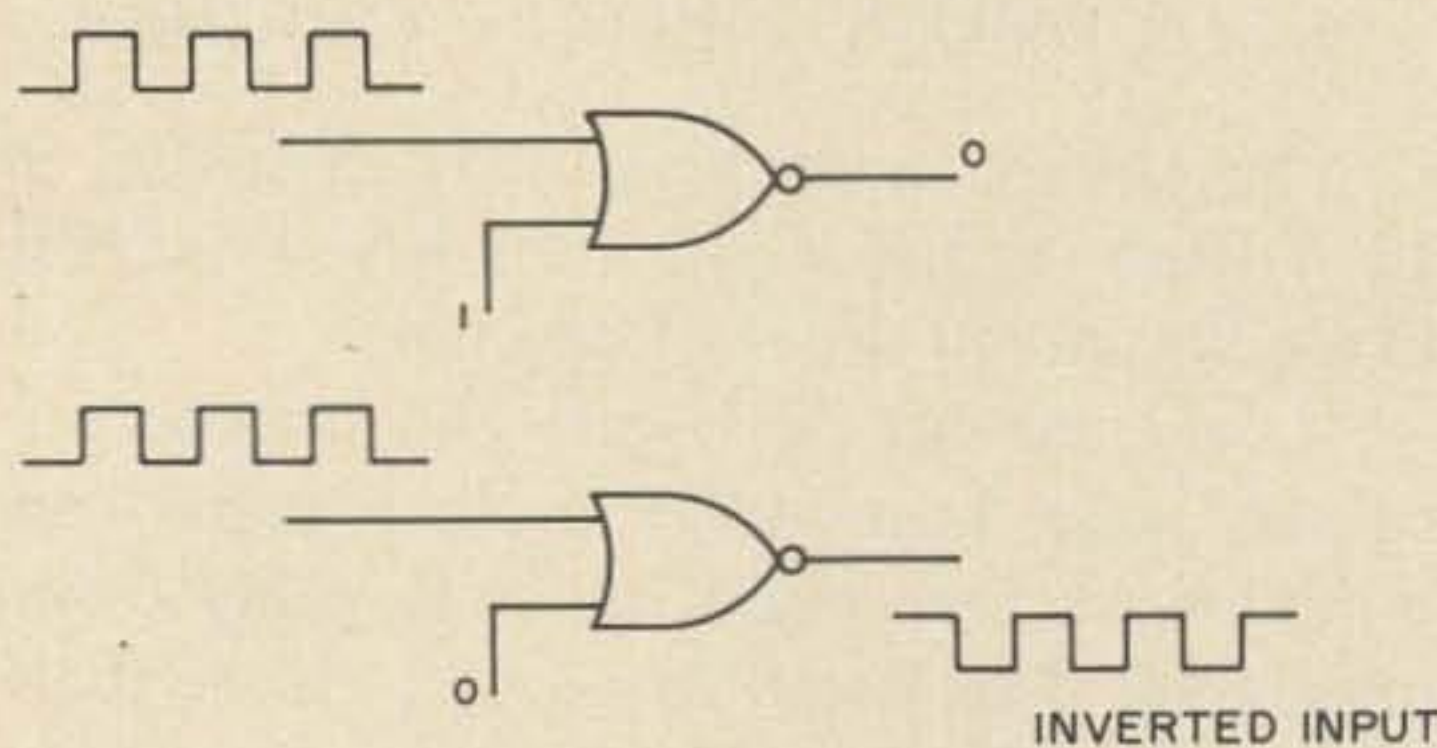
Fig. 11. NOR gate.
