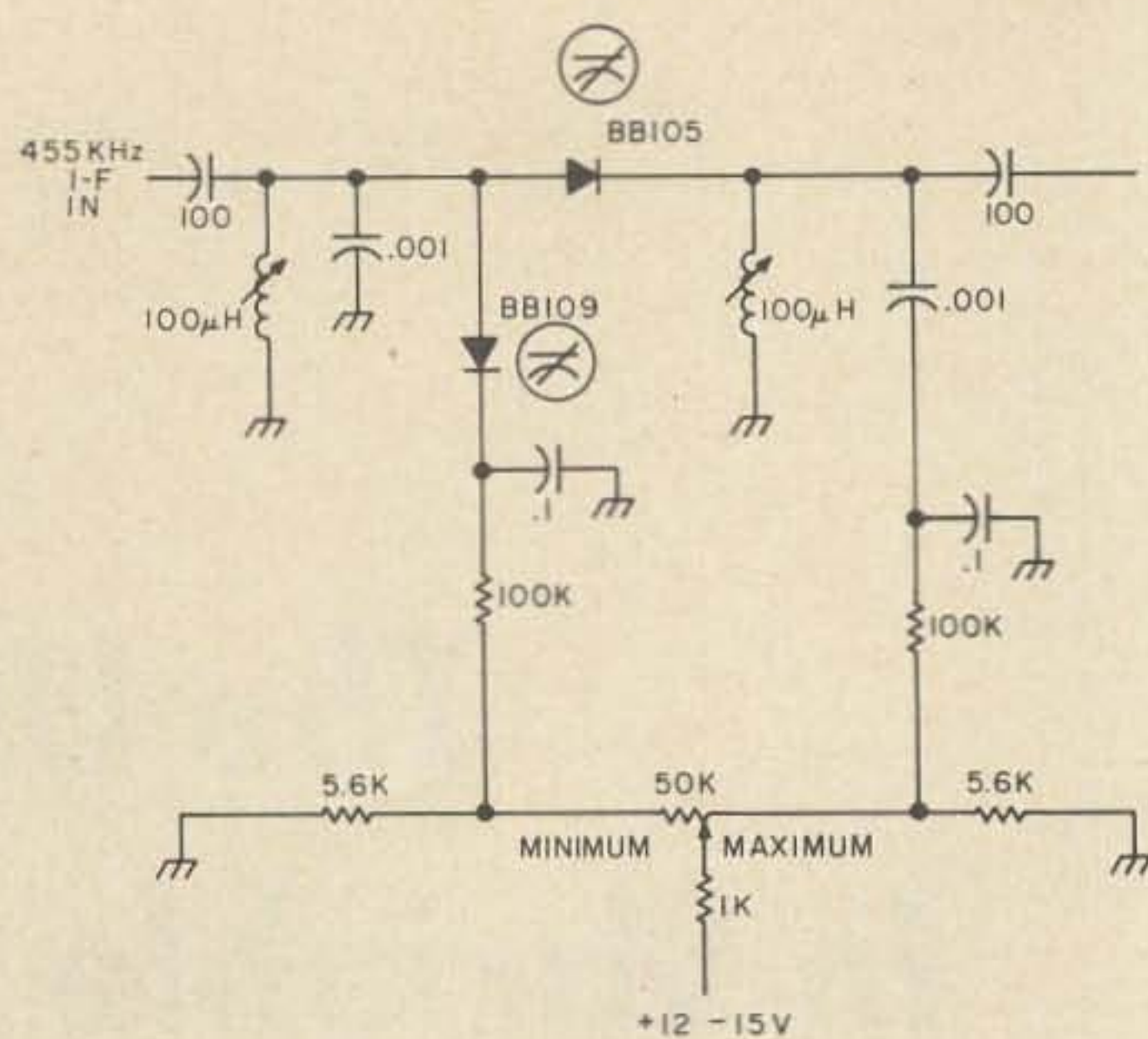
Fig. 3. Variable selectivity circuit with compensation.
