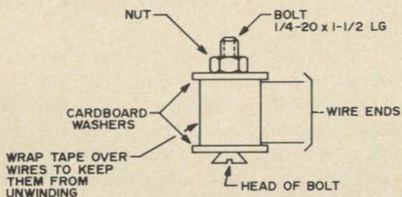
Fig. 1. Tom's electromagnet.
