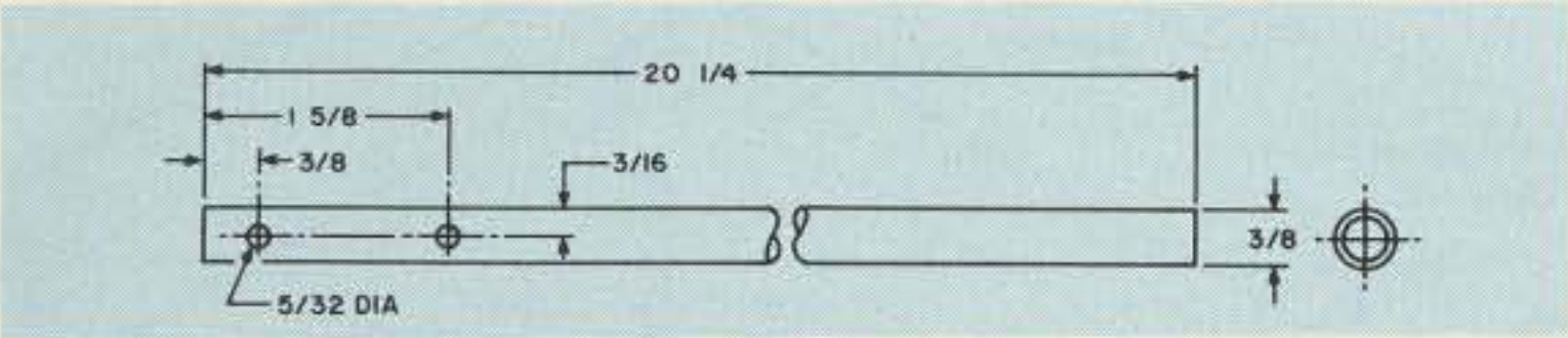
Fig. 19. Construction detail of the short radial. Four are required.
