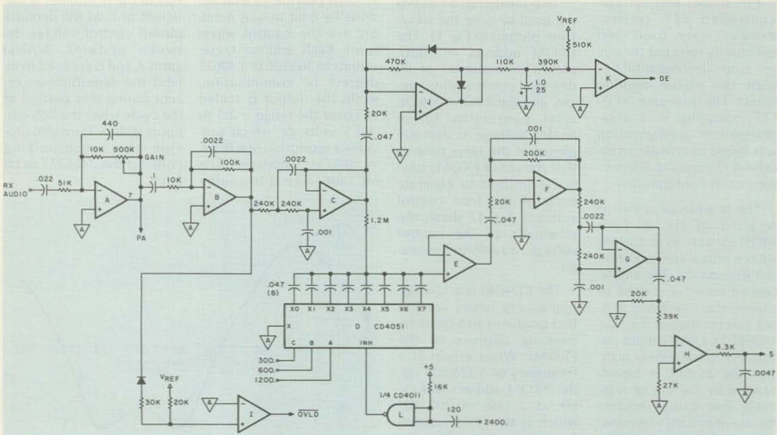
Fig. 13. Audio signal processor circuit schematic. Notes: All op amps are 1/2 LM1458 except H, which is 1/2 CA3240. All diodes are 1N4148. Logic power is V_{dd} = +5 , V_{ee} = -6 , V_{ss} = \text{L} . Op amp power is +5 and -6 V dc.
