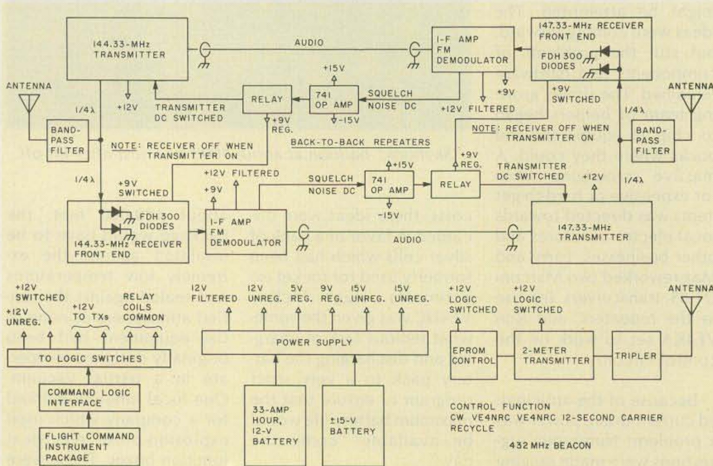
Fig. 1. Flight package.
