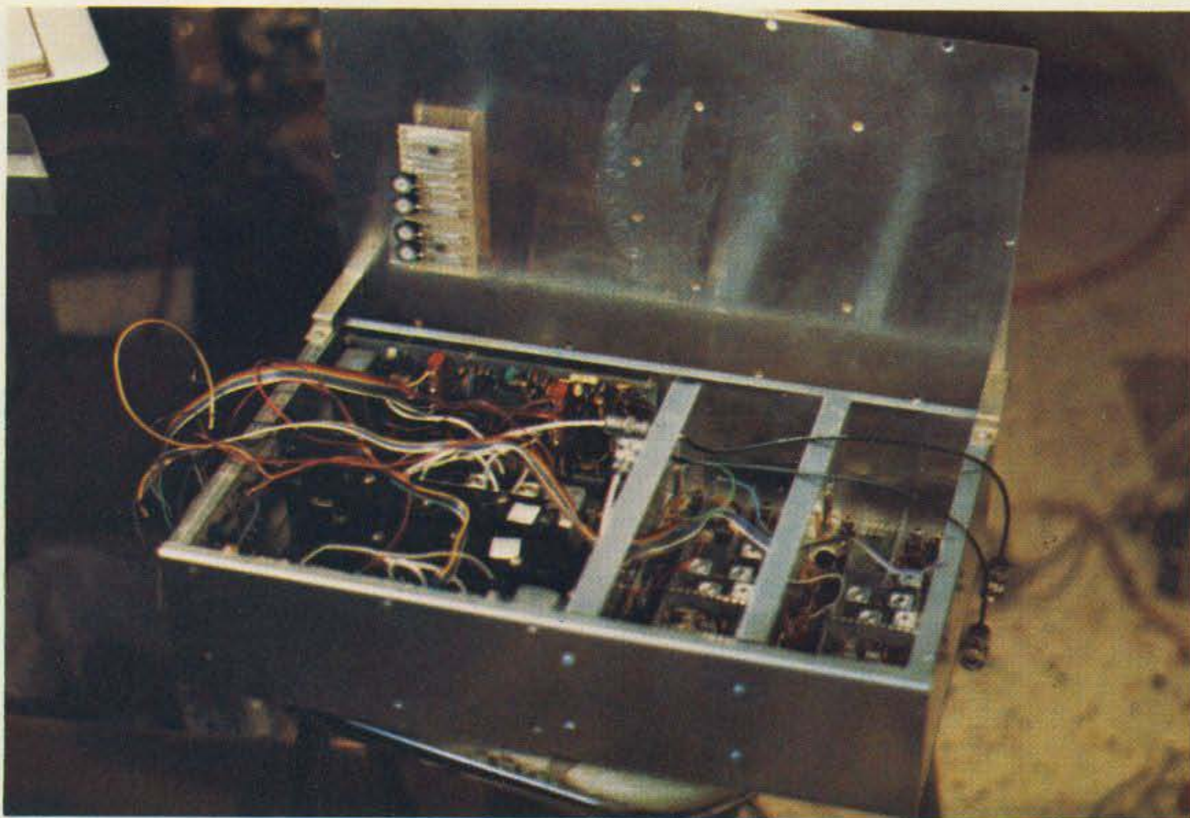
The repeater package with two receivers in the left-hand compartment and the transmitters in two separate compartments on the right.
