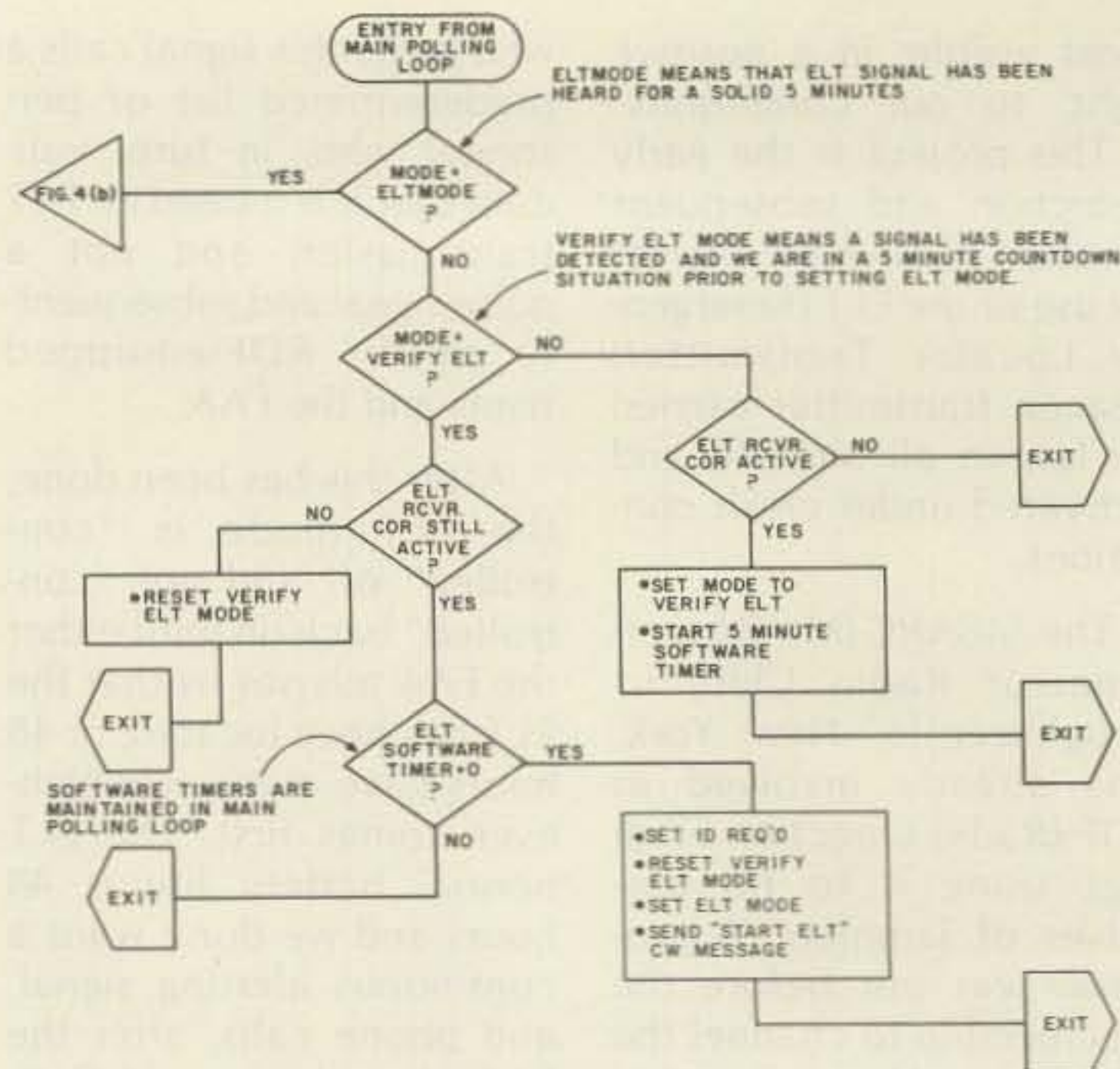
Fig. 4(a). System flowchart.
