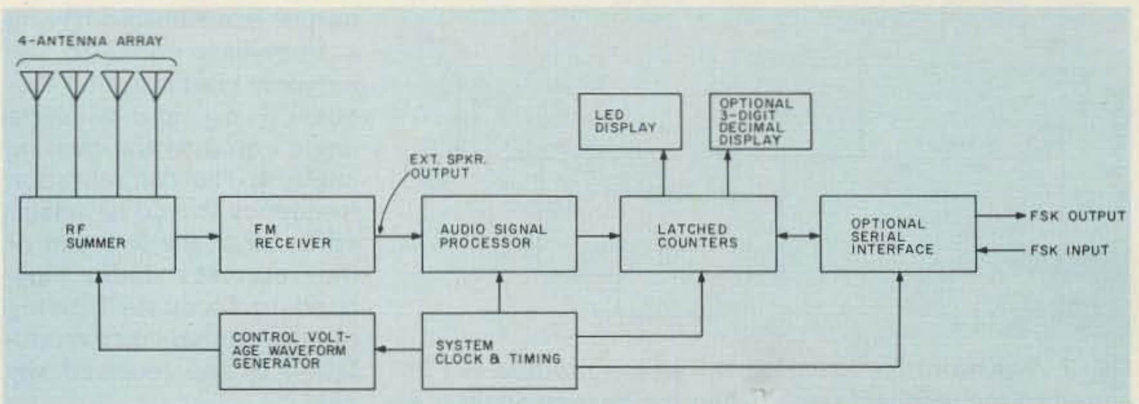
Fig. 1. Block diagram of the complete direction-finding system.
