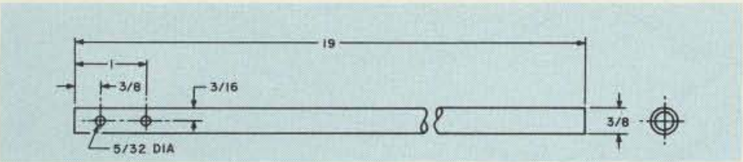
Fig. 20. Vertical element dimensions. Four are required.
