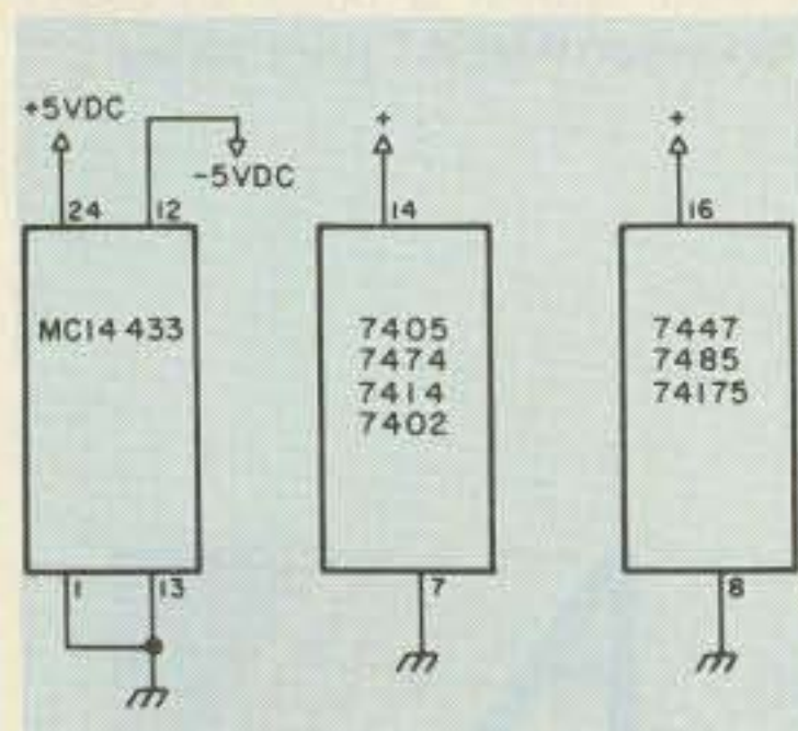
Fig. 5. Supply connections for integrated circuits.
