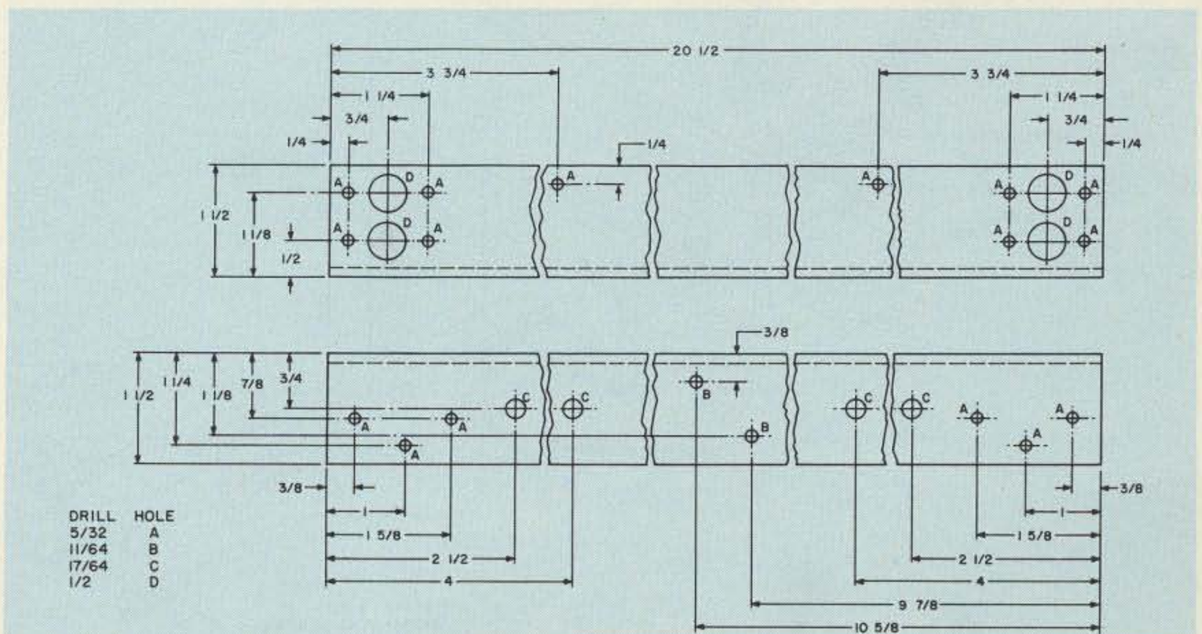
Fig. 23. Side arm construction detail. Two are required.
