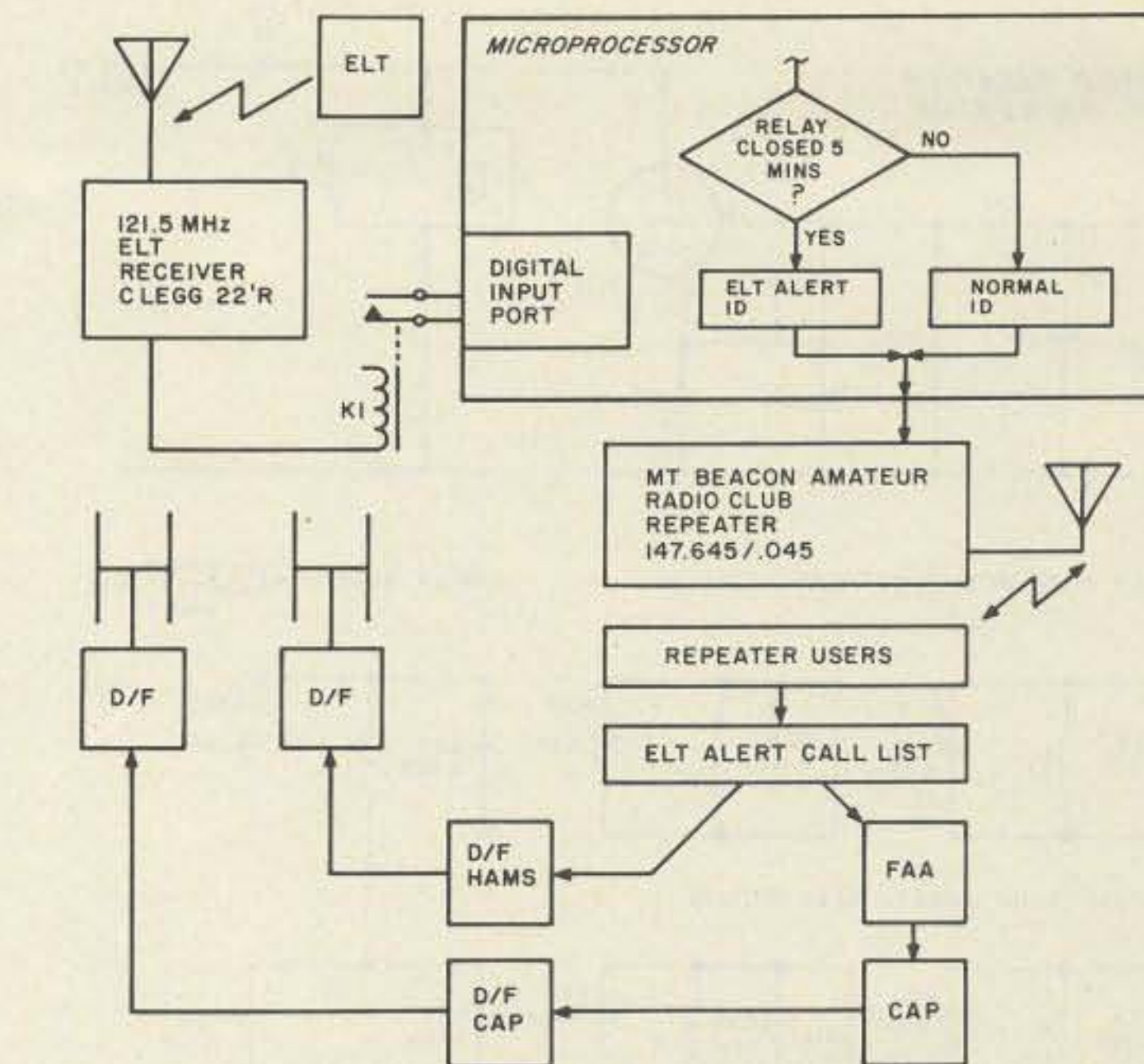
Fig. 1. Emergency Locator Transmitter (ELT) alerting system.
