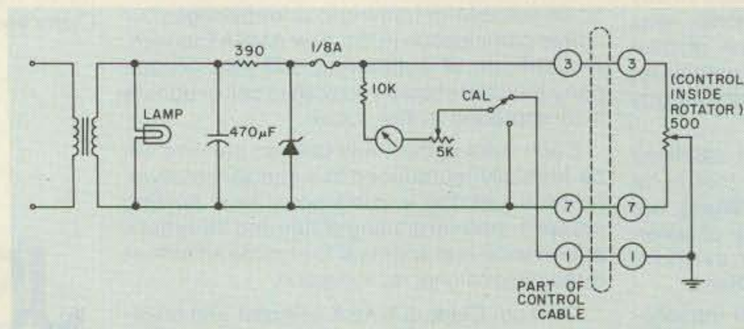
Fig. 6. Unmodified sensing circuit of the Ham III rotator. Wiper of control in rotator is connected to earth ground.
