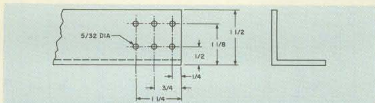
Fig. 24. Drill guide dimensions. Make this tool from stock left over from the center support and side arms.
