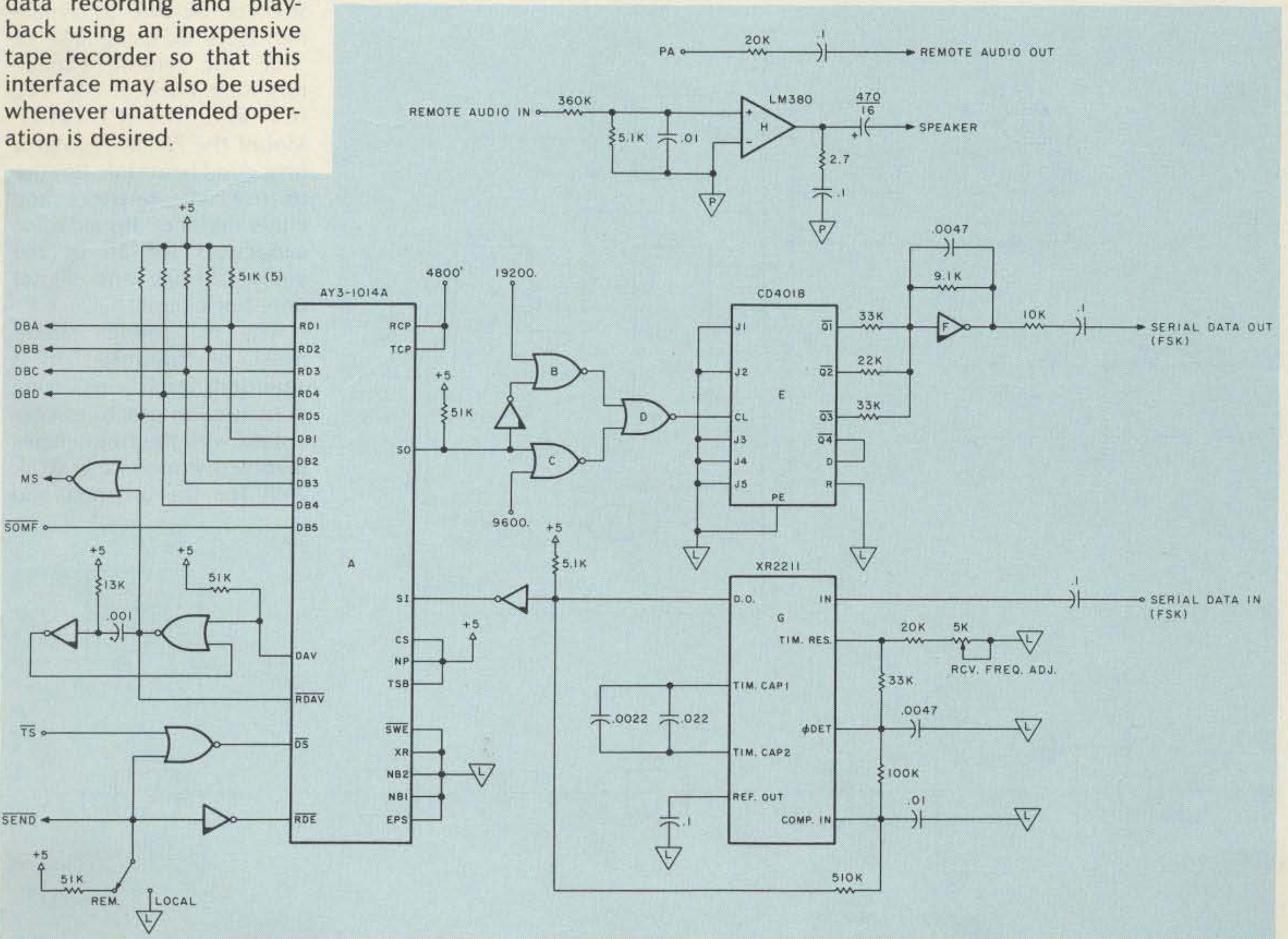
Fig. 16. Optional serial interface circuit schematic. Notes: NOR gates are 1/4 CD4001. Inverters are 1/6 74C903. Digital logic power is V_{cc} = V_{dd} = +5 , V_{ss} = GND = \nabla . Amplifier H power is +13 switched (sw); ground is \nabla .
