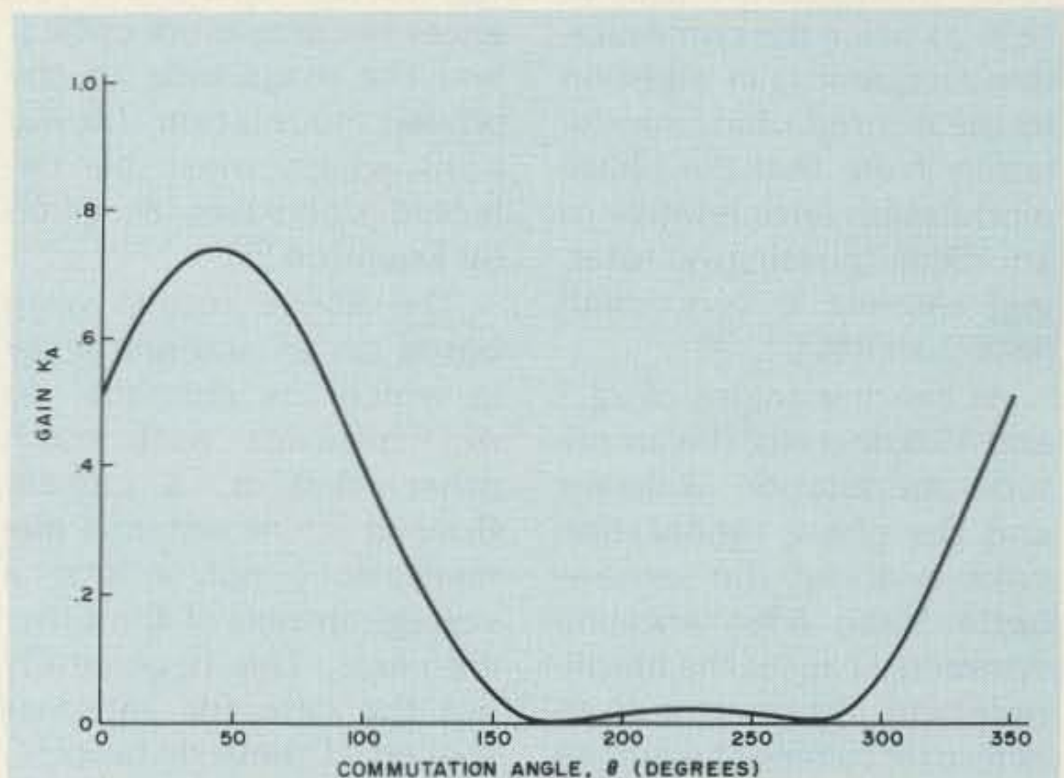
Fig. 5. Theoretical gain variation for antenna "A" required to produce an equivalent continuously rotating antenna signal.
