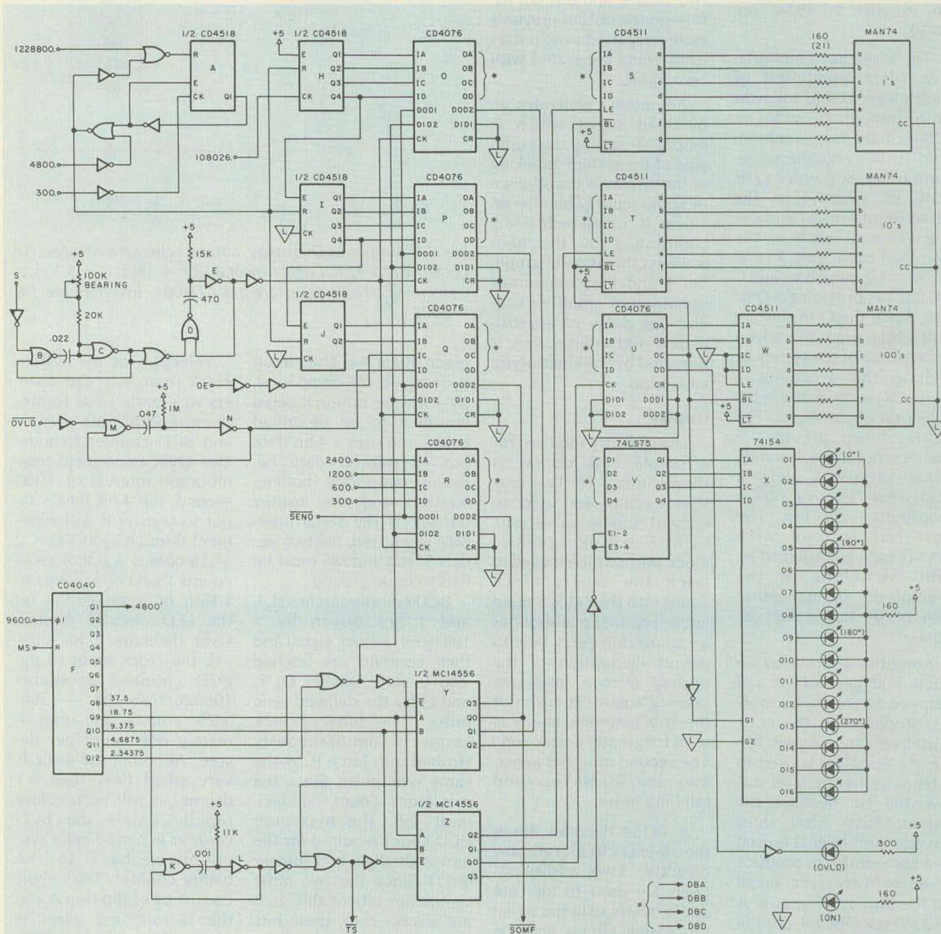
Fig. 15. Schematic of the circuit used to provide circular LED display and a three-digit decimal display. A data bus technique is employed which is compatible with the optional serial interface. Notes: Connect 4-bit data bus *. All LEDs are MIL32 R. Digital logic power is V_{dd} = V_{cc} = +5 , V_{ss} = GND = \text{ground symbol} . All NOR gates are 1/4 CD4001. All inverters are 1/6 CD4069 except \nabla are 1/6 74C903. Schematic is drawn for operation with serial interface. For no serial interface, add jumpers SEND to \nabla , MS to \nabla .
