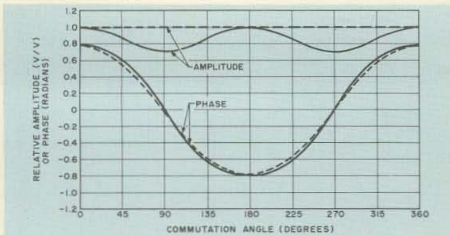
Fig. 6. Amplitude and phase modulation for an uncoupled antenna array of size 1/4 wavelength and a bearing angle of 0 degrees. The dashed lines represent the ideal (continuously rotating antenna) case.
