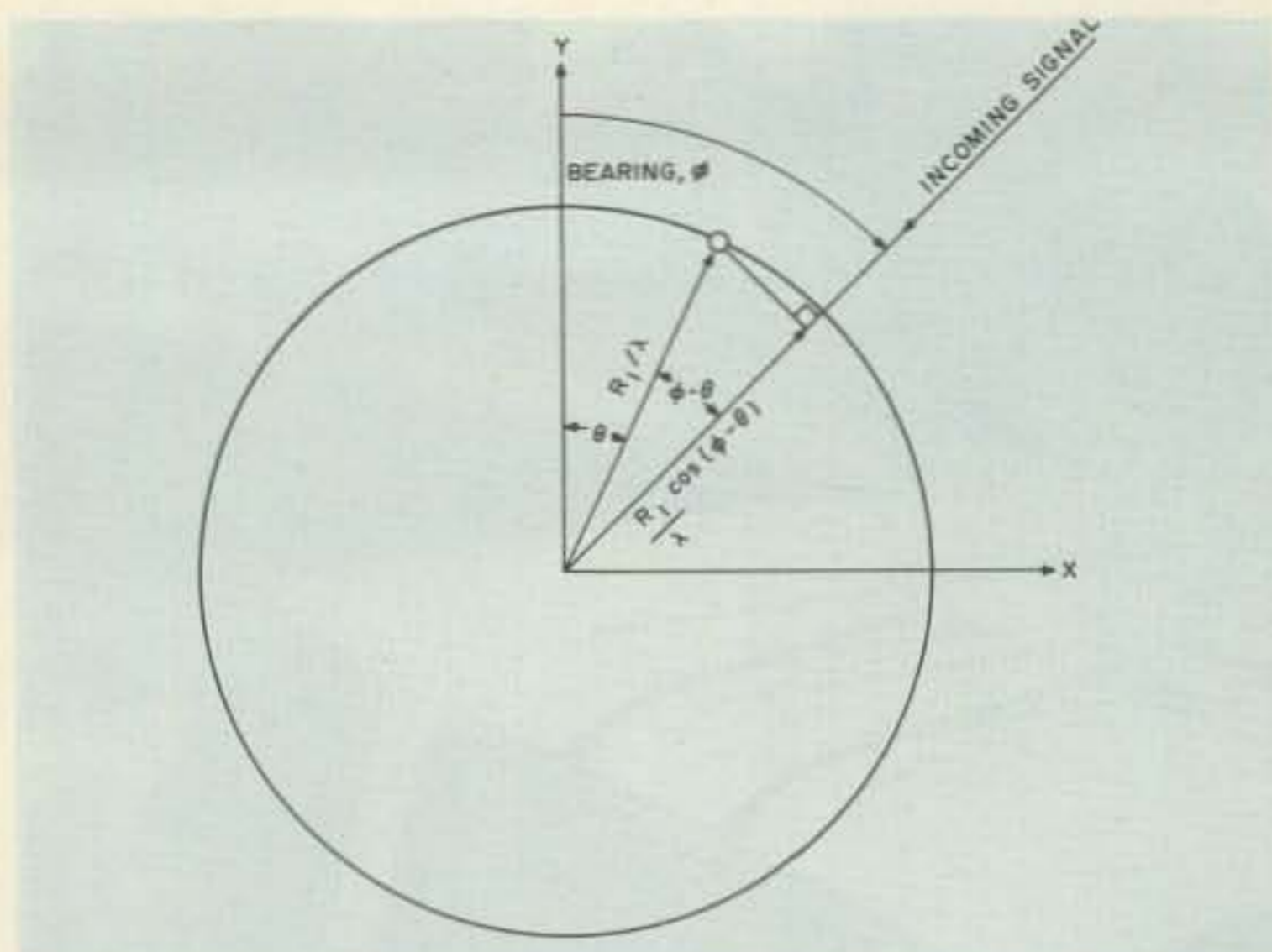
Fig. 2. Geometry used to derive the signal received by a rotating antenna.
