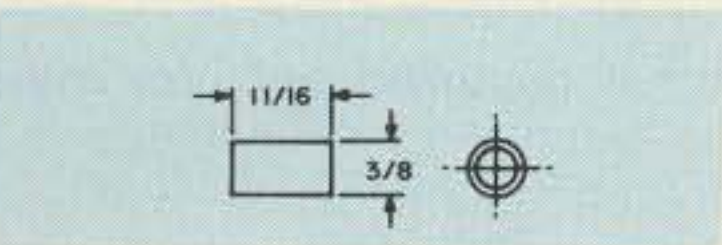
Fig. 21. Suction cup spacer. Four of these are required for mounting the antenna on a car roof.
