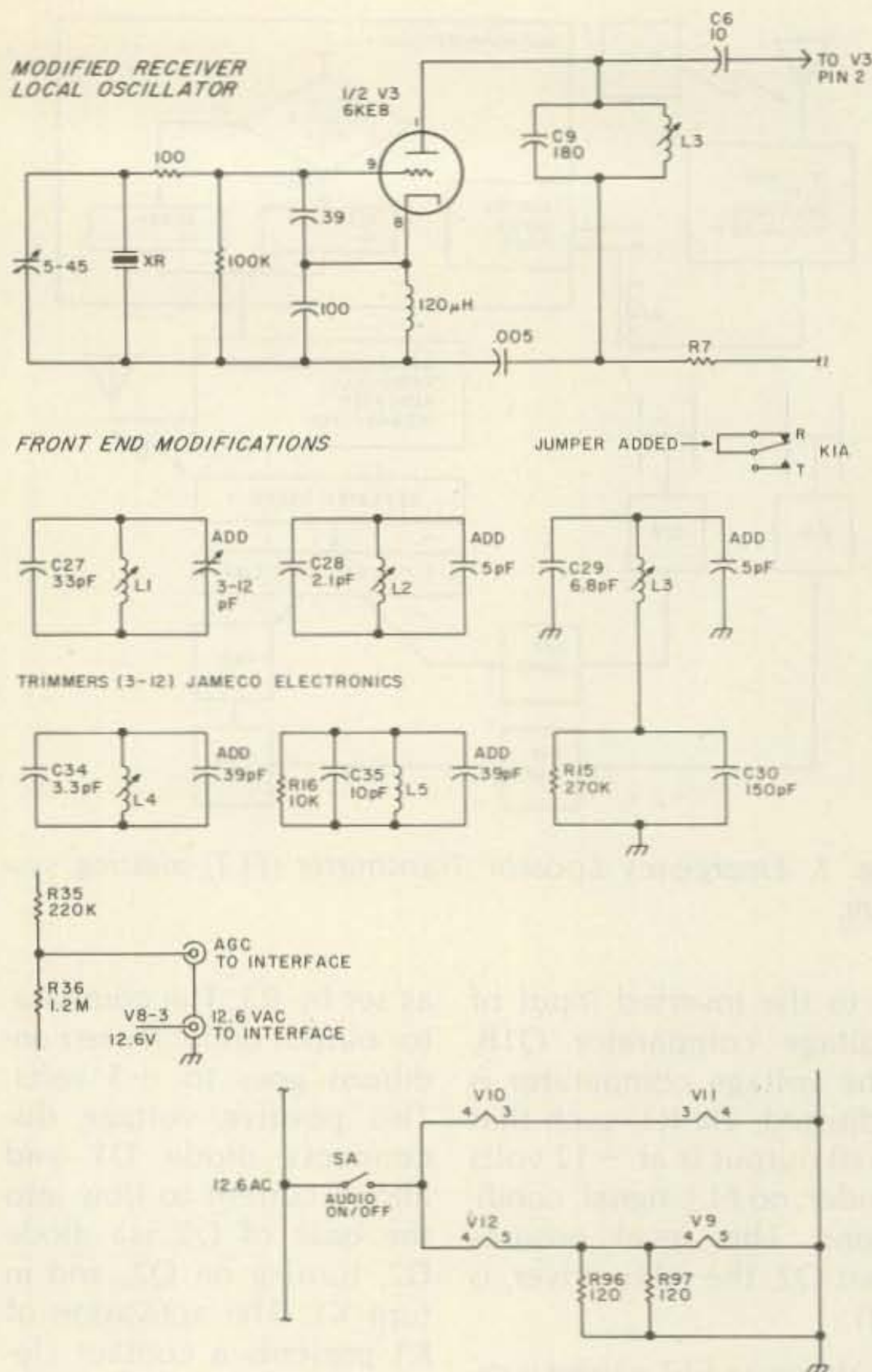
Fig. 3. Modifications to Clegg 22'er for 121.5-MHz ELT reception. XR = 8.262500 MHz for 121.5-MHz input, use International Crystal Manufacturing Co. catalog #433478 (10 North Lee, Oklahoma City OK 73102). Modifications include removal of V13, V14, and V15. Do not remove V12. This turns off audio and reduces heat generated by unused tubes. A small pancake fan was mounted on top of the cabinet to provide cooling required for 24-hour operation.
