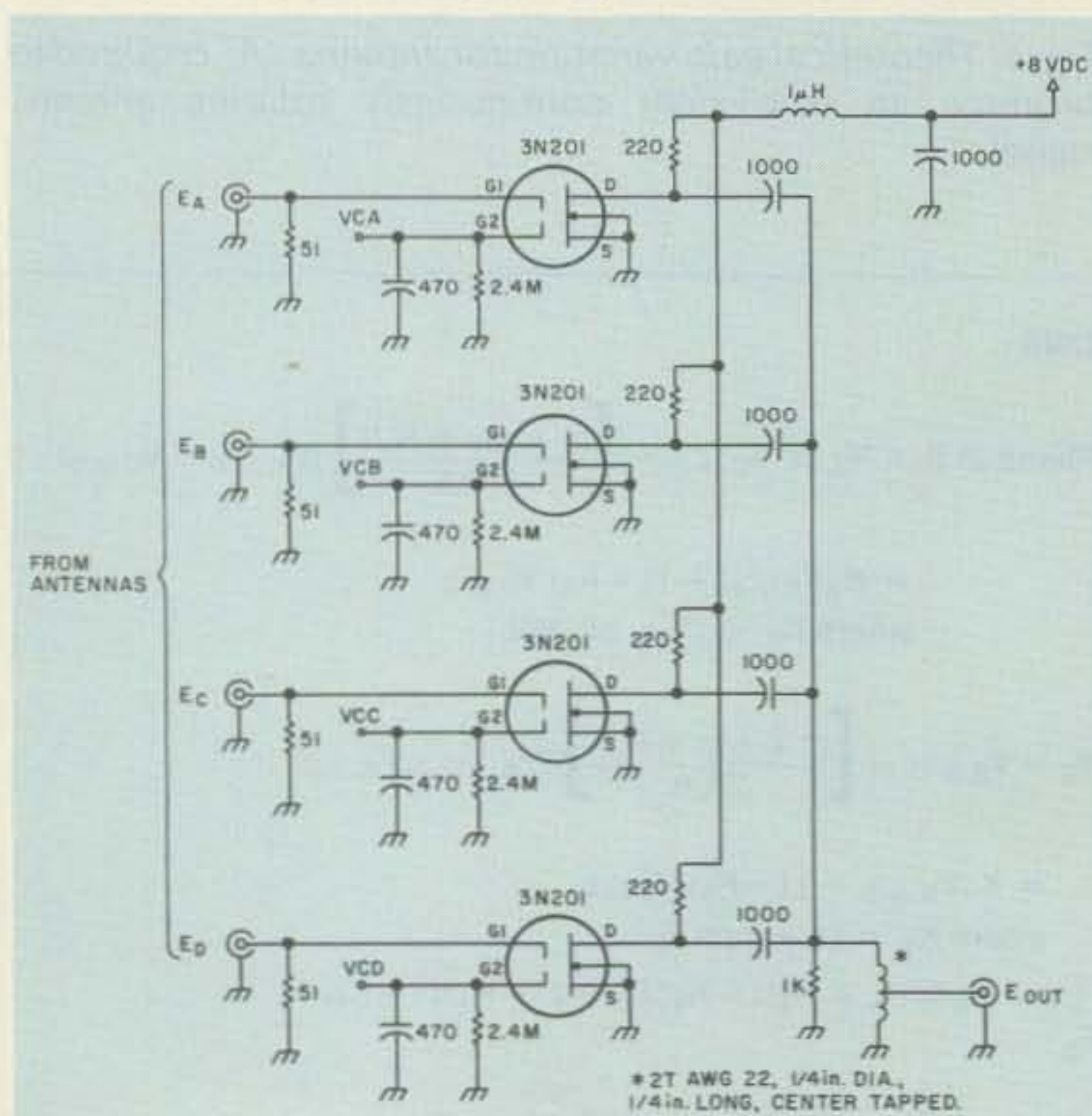
Fig. 8. Rf summer circuit schematic.
