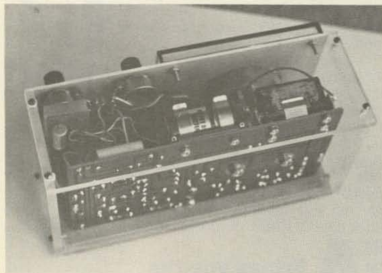
Photo B. The IM-17 mounted in a home-built Plexiglas housing.
