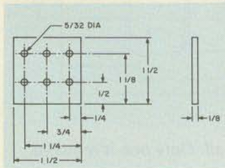
Fig. 25. Teflon insulator construction. Use the drill guide and a block of wood when drilling this material.
