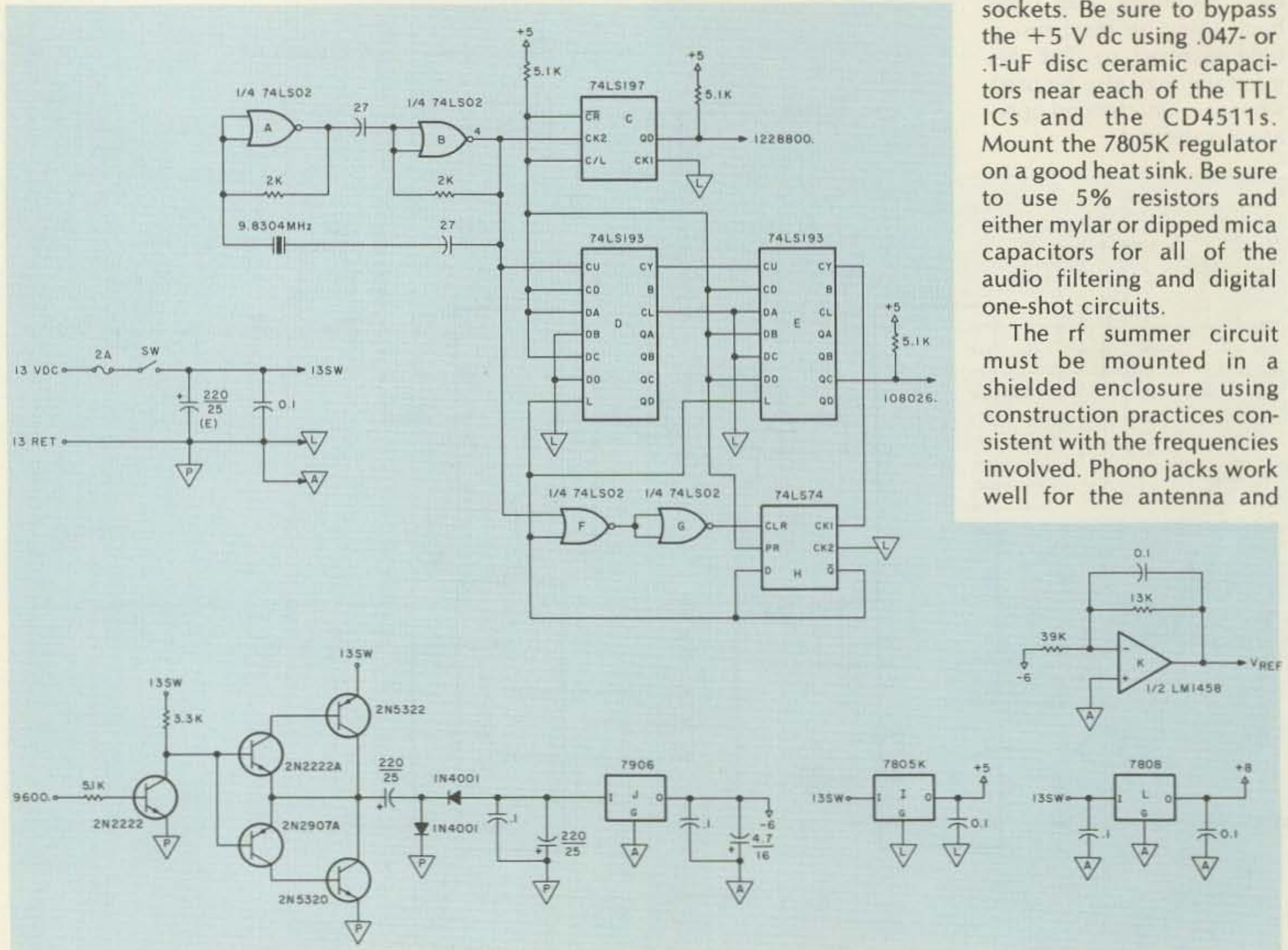
Fig. 17. Schematic of the power supply and clock circuitry. Notes: Power to LM1458 is +5 and -6 V dc. Logic power is V_{cc} = +5 , GND = \text{ground} .
