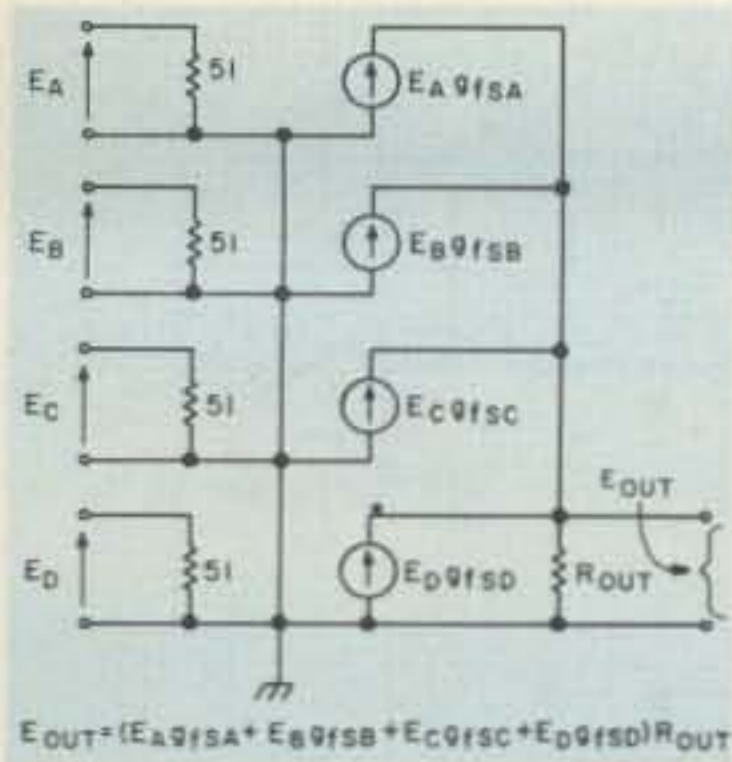
Fig. 9. Equivalent circuit of the rf summer.
