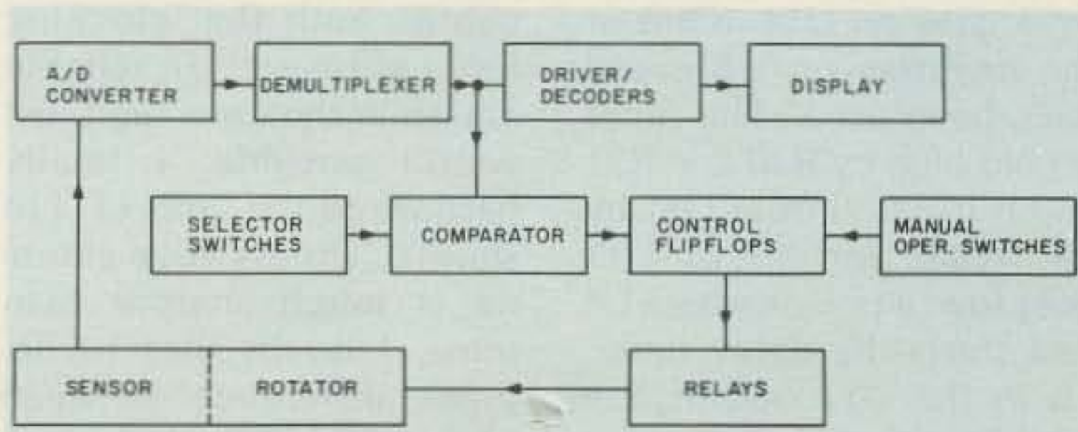
Fig. 1. Automatic rotator control block diagram.
