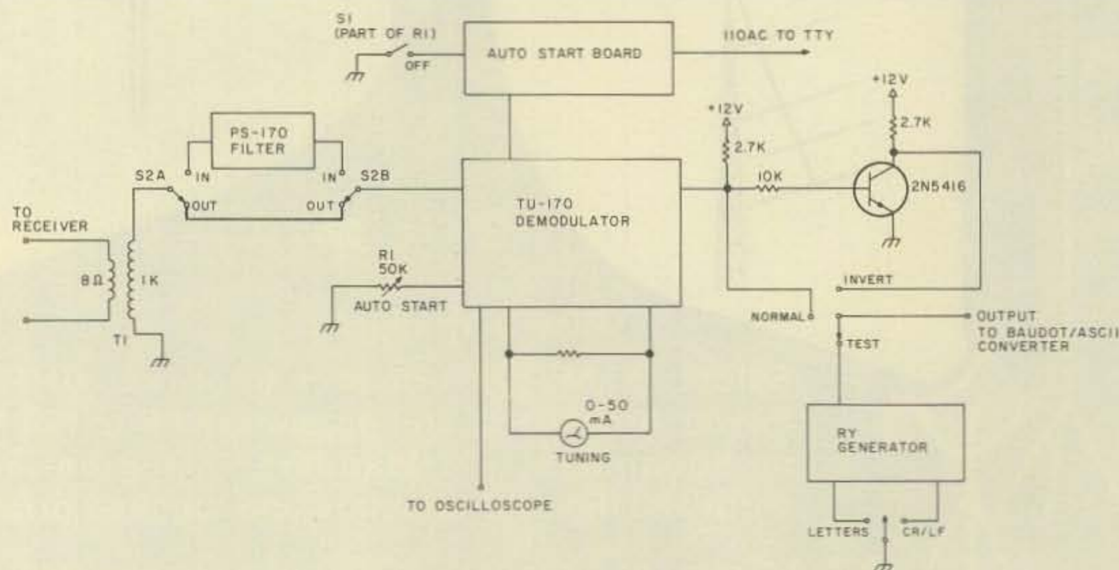
Fig. 2. Block diagram of the TU.
