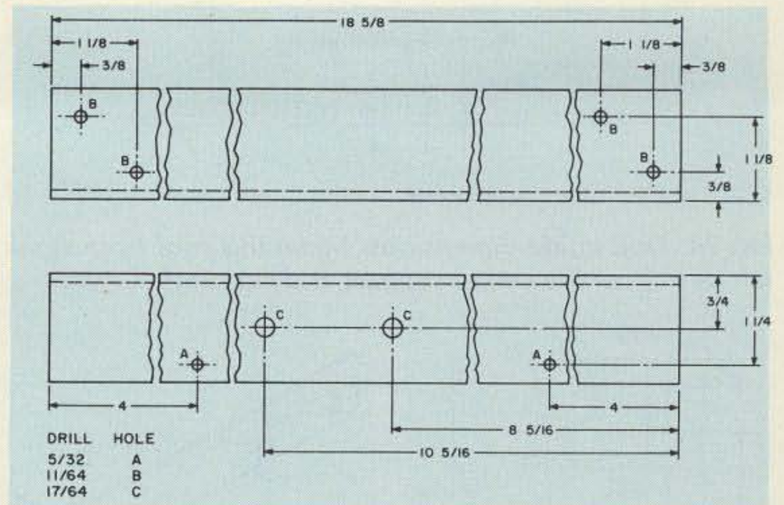
Fig. 22. Center support detail. Only one is required.
