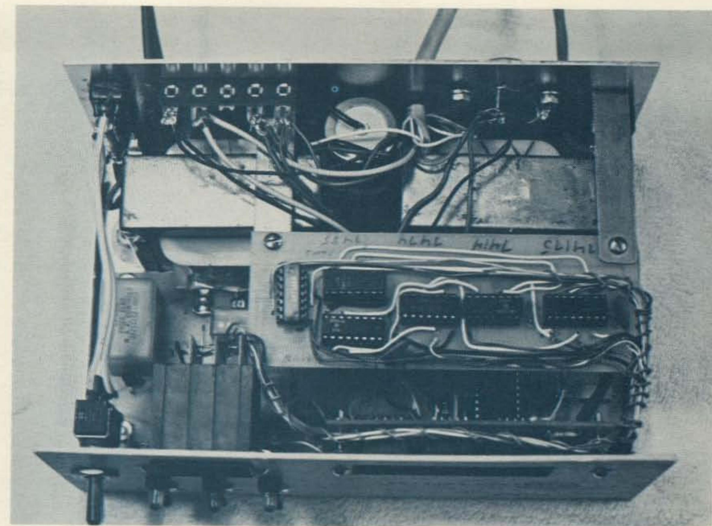
Photo B. Interior view. A 25.2-V transformer at upper left provides ac for rotator operation. At upper right is a 12.6-V transformer for control operation. Connections to the rotator assembly are made on the terminal strip at upper left. After the photo was taken, I installed a molex connector and eliminated the terminal strip. The ac power switch and thumbwheel switches are at lower left. The six ICs mounted on a separate circuit board which is double-decked over the main board are the de-multiplexers, comparators, and inverters.
