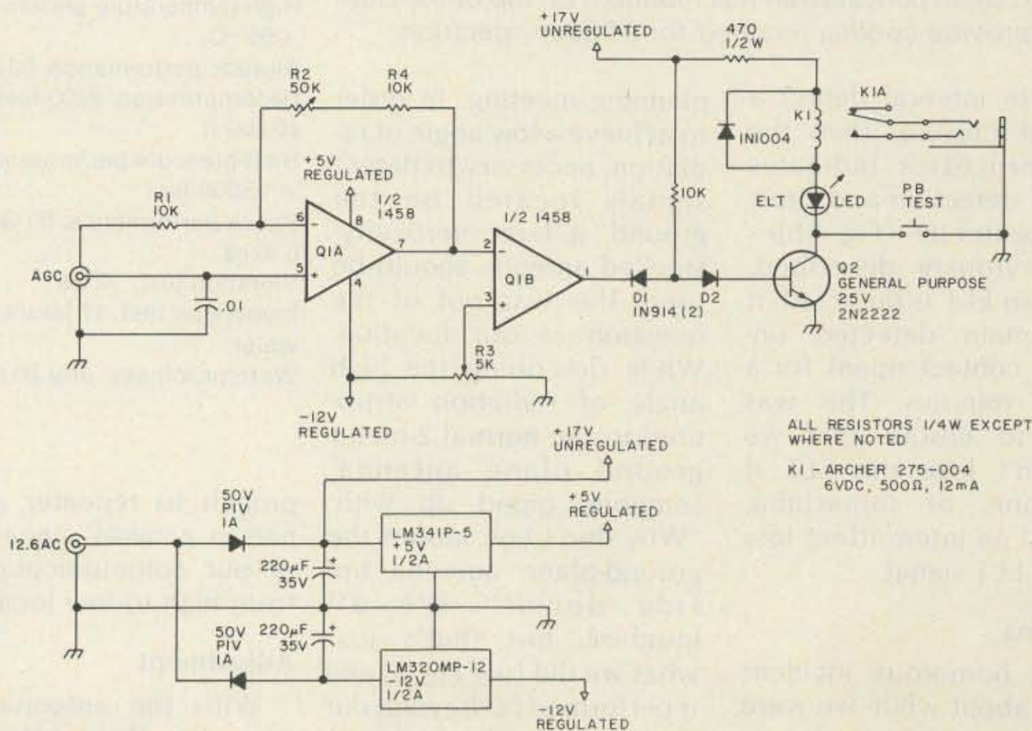
Fig. 2. Interface from Clegg 22'er to microprocessor.
