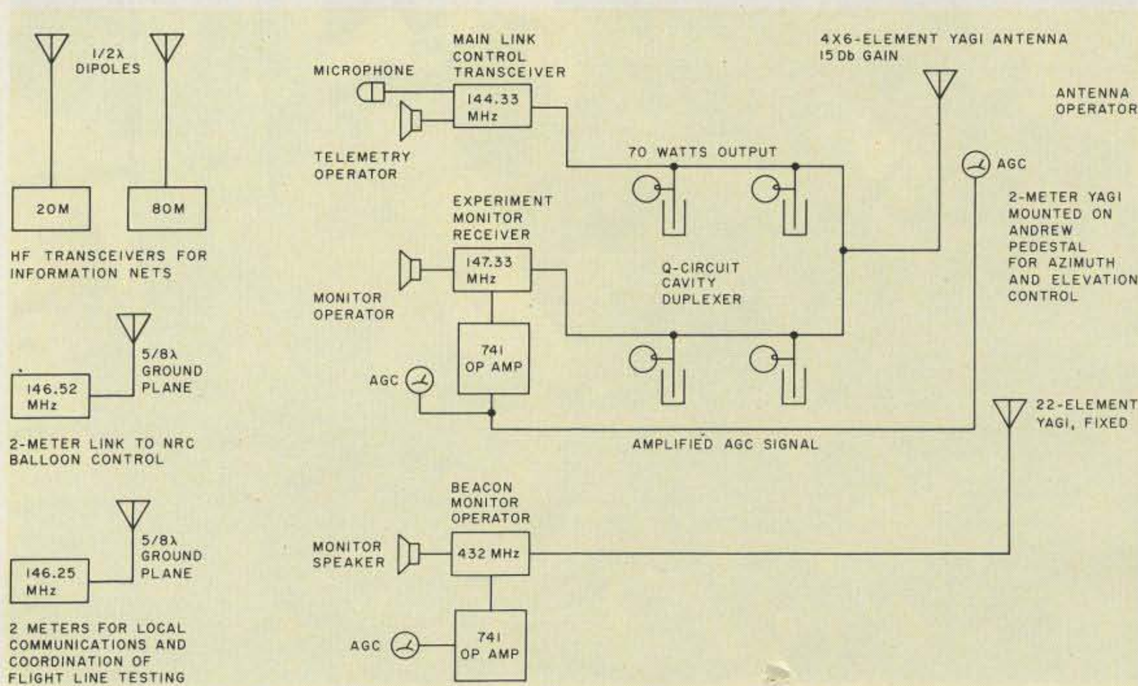
Fig. 2. Ground station.
