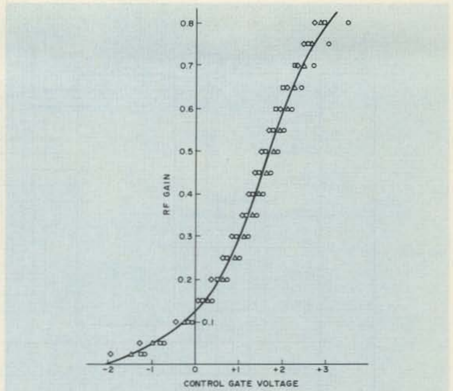
Fig. 10. Rf gain variation with control gate voltage for four typical field-effect transistors. The curve is a seventh-order polynomial fit to the measured data.
