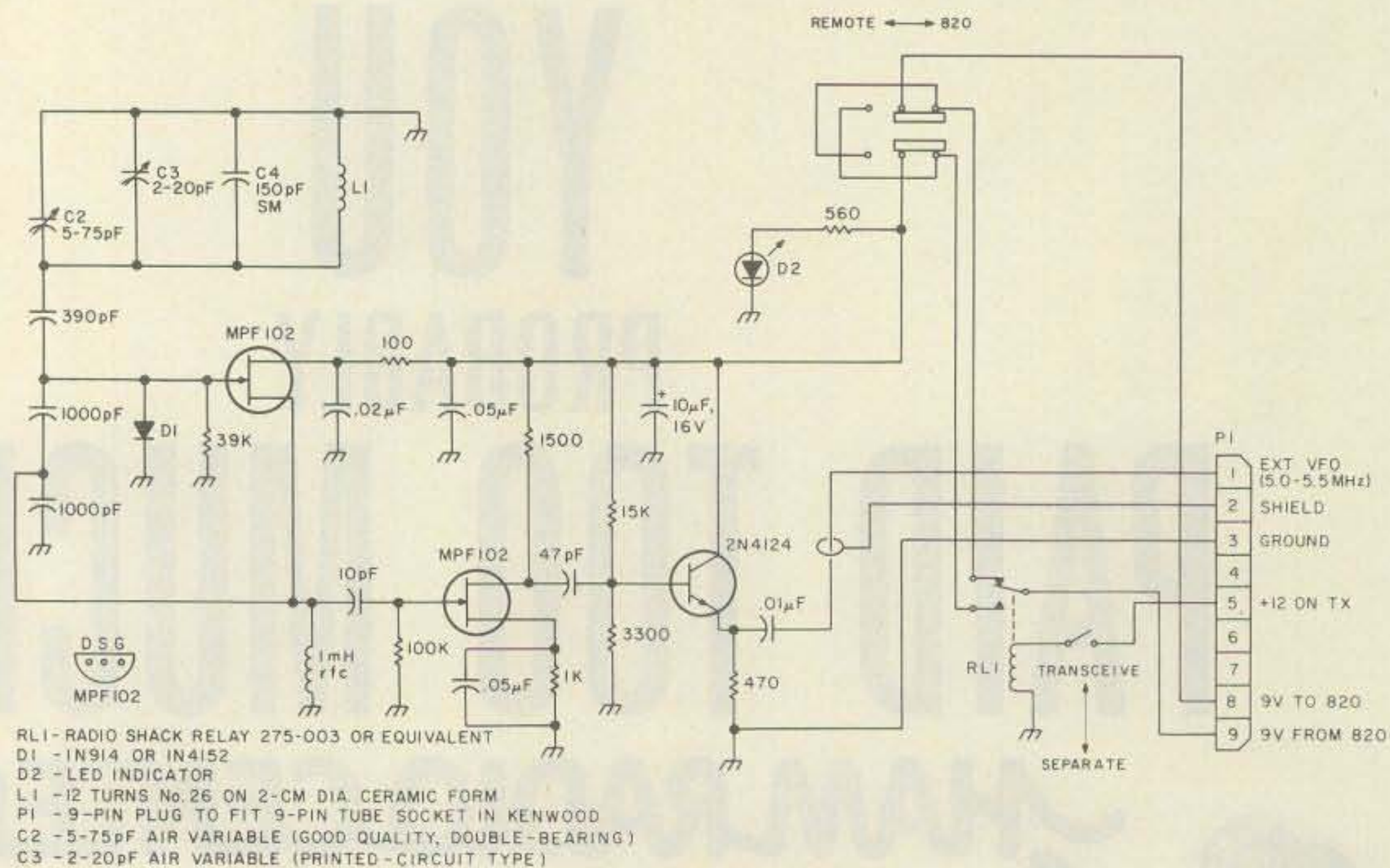
Fig. 1. Schematic for the Kenwood TS-820S remote vfo.
