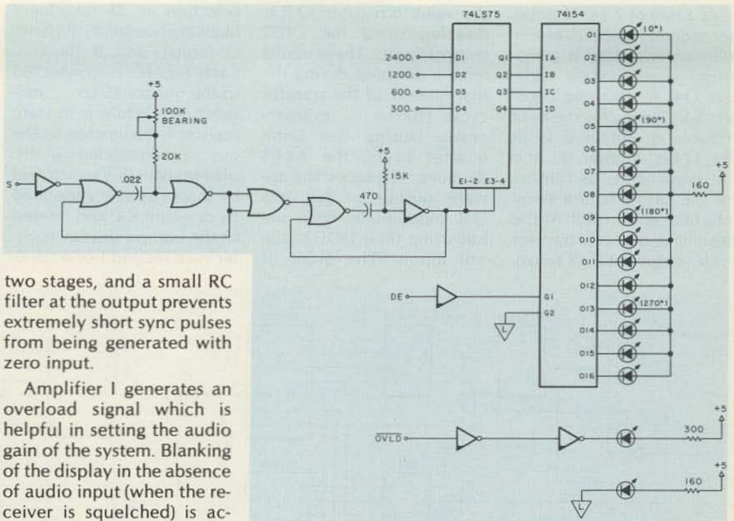
Fig. 14. Simple LED display circuit schematic. Notes: All LEDs are MIL32 R. Logic power is V_{cc} = V_{dd} = +5 , V_{ss} = GND = \nabla . NOR gates are 1/4 CD4001. Inverters are 1/6 74C903.
