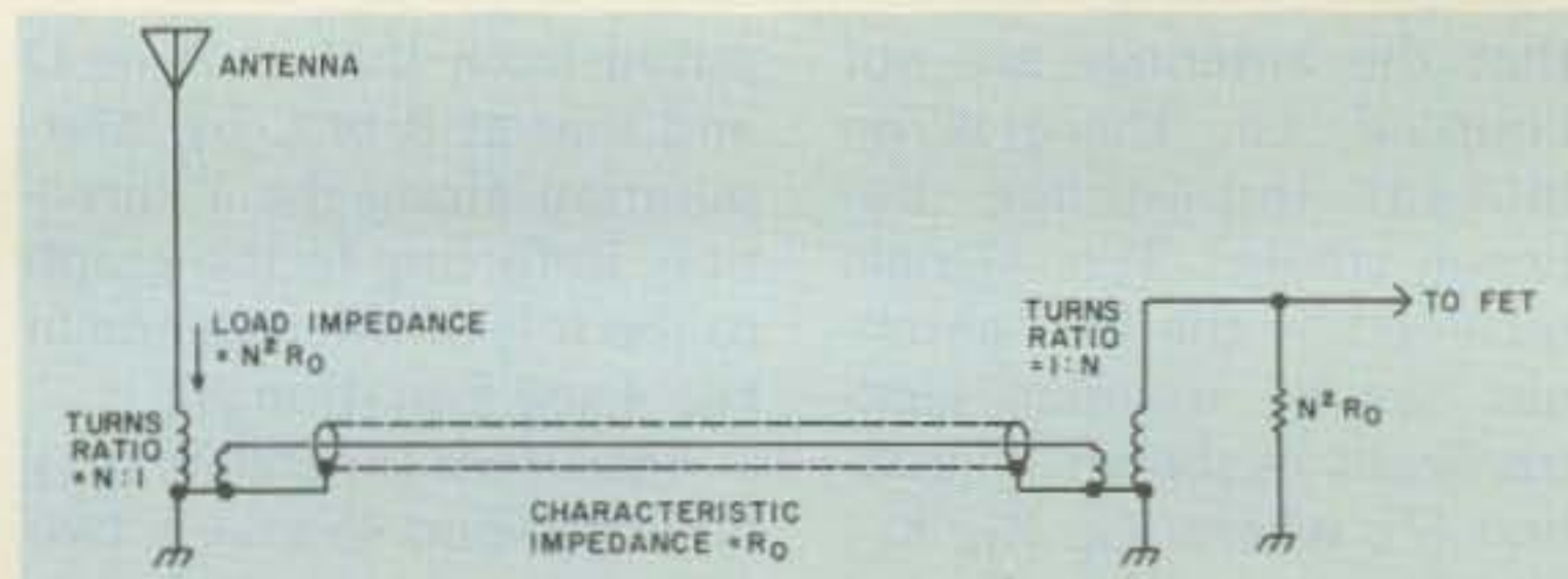
Fig. 7. Use of impedance transformers to minimize the effect of mutual impedance coupling between array antennas.
