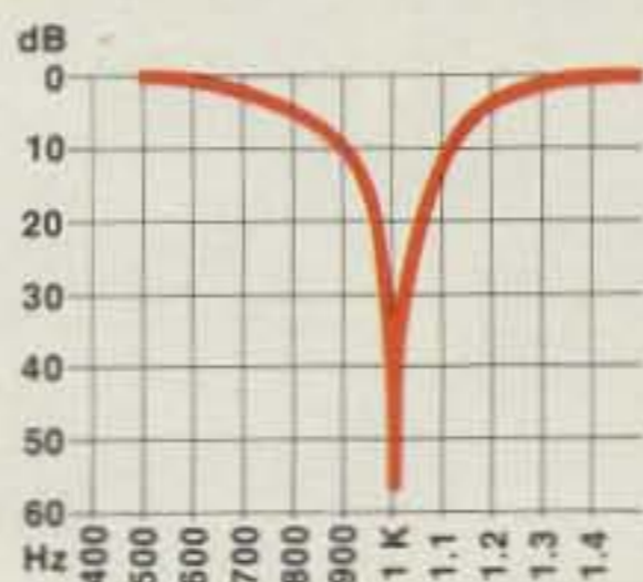
NOTCH FILTER PERFORMANCE ADJUSTED TO 1 kHz POINT.
