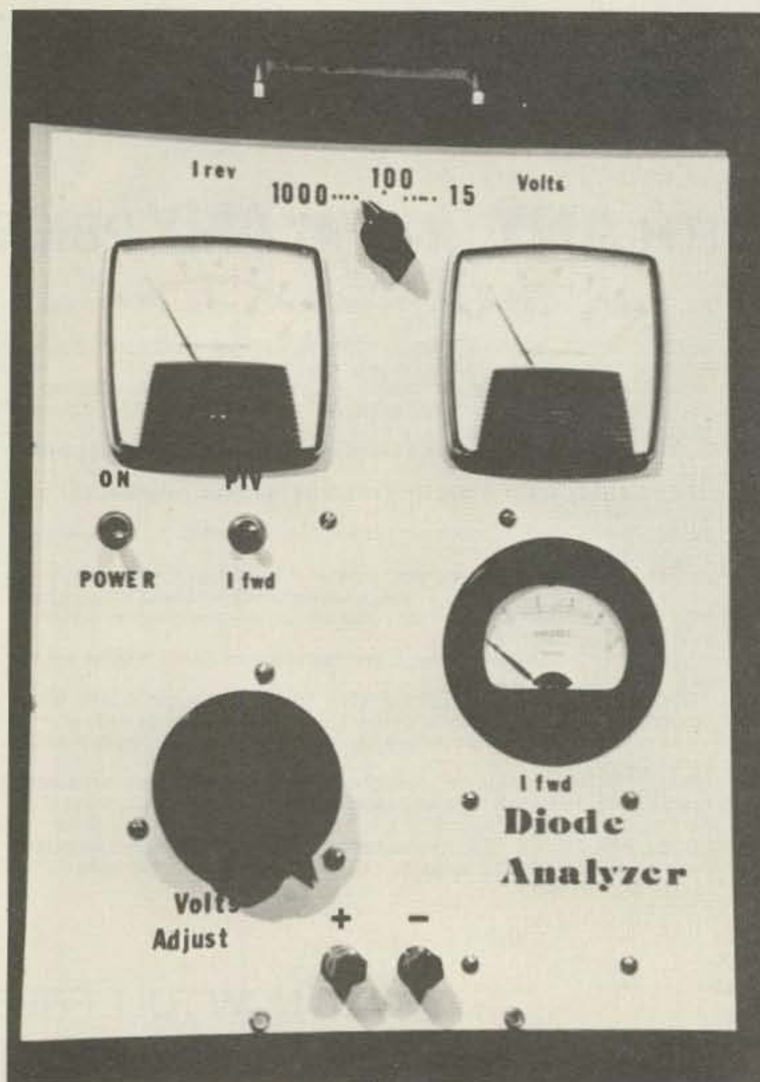
Front panel of the diode analyzer.
