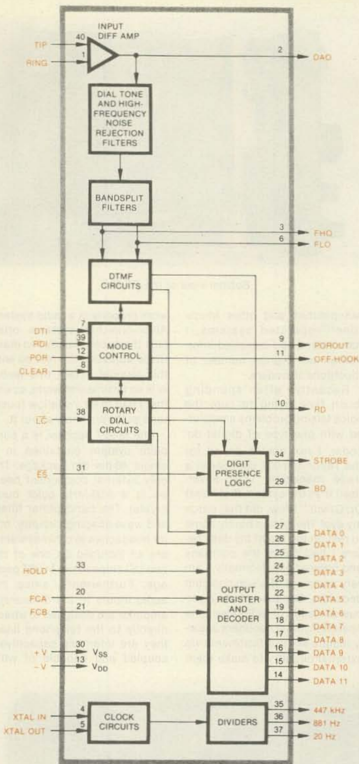
Fig. 1(a). The M-927 block diagram.
