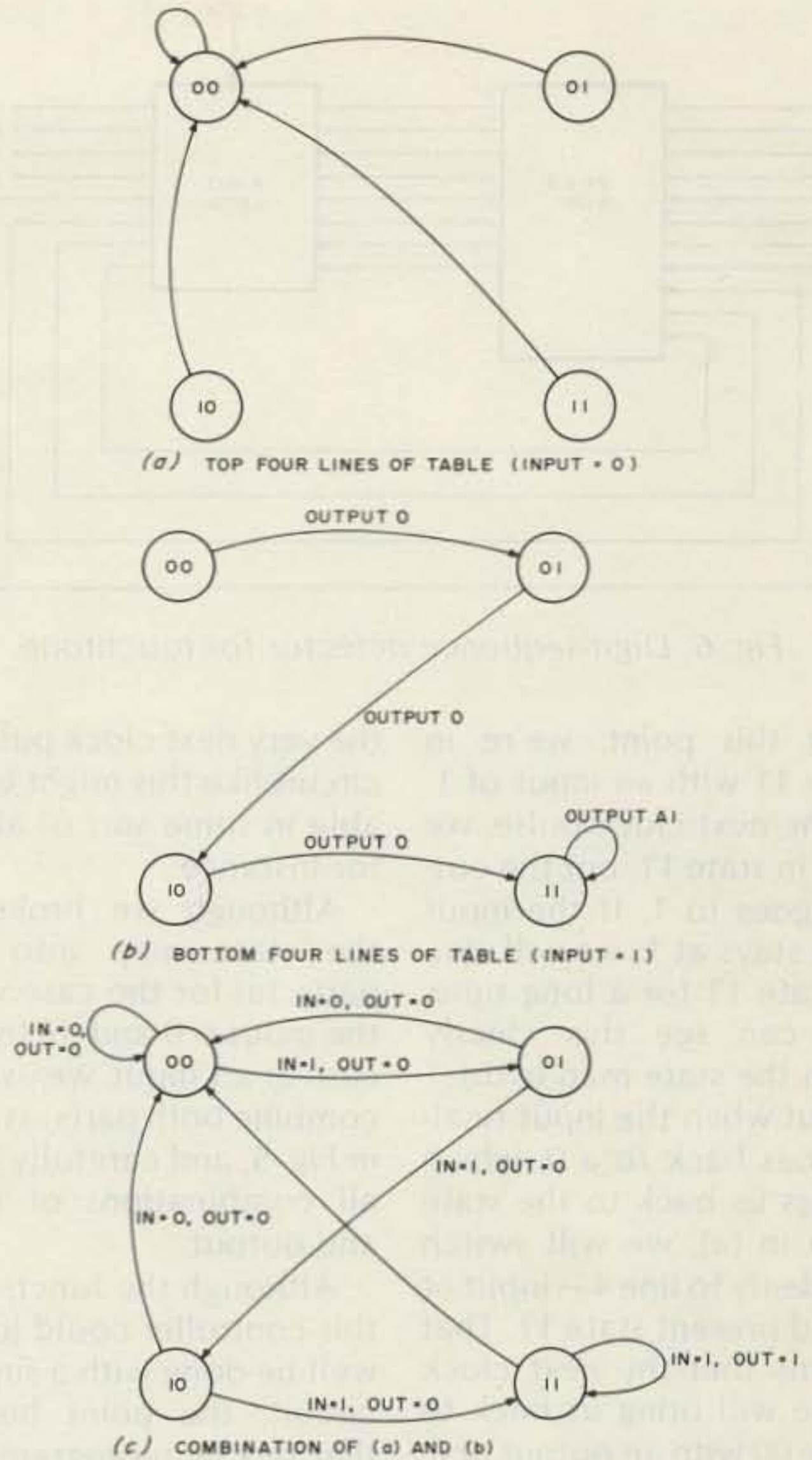
Fig. 5. State map for Fig. 4.
