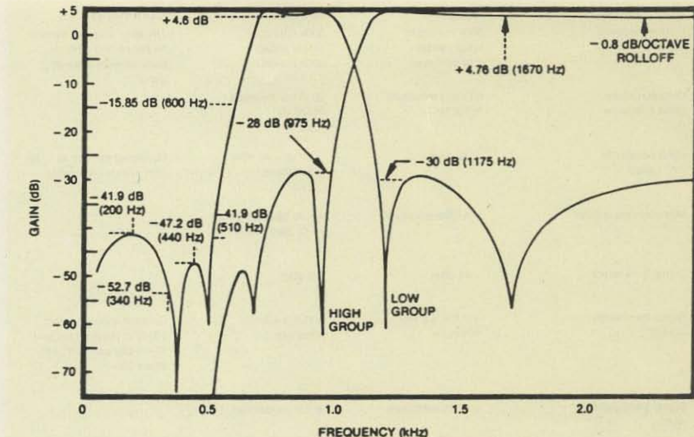
Fig. 2. Bandpass filter characteristics of the M-927.
