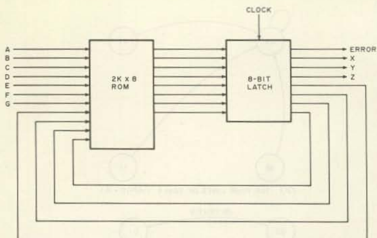
Fig. 6. Digit-sequence detector for touchtone.
