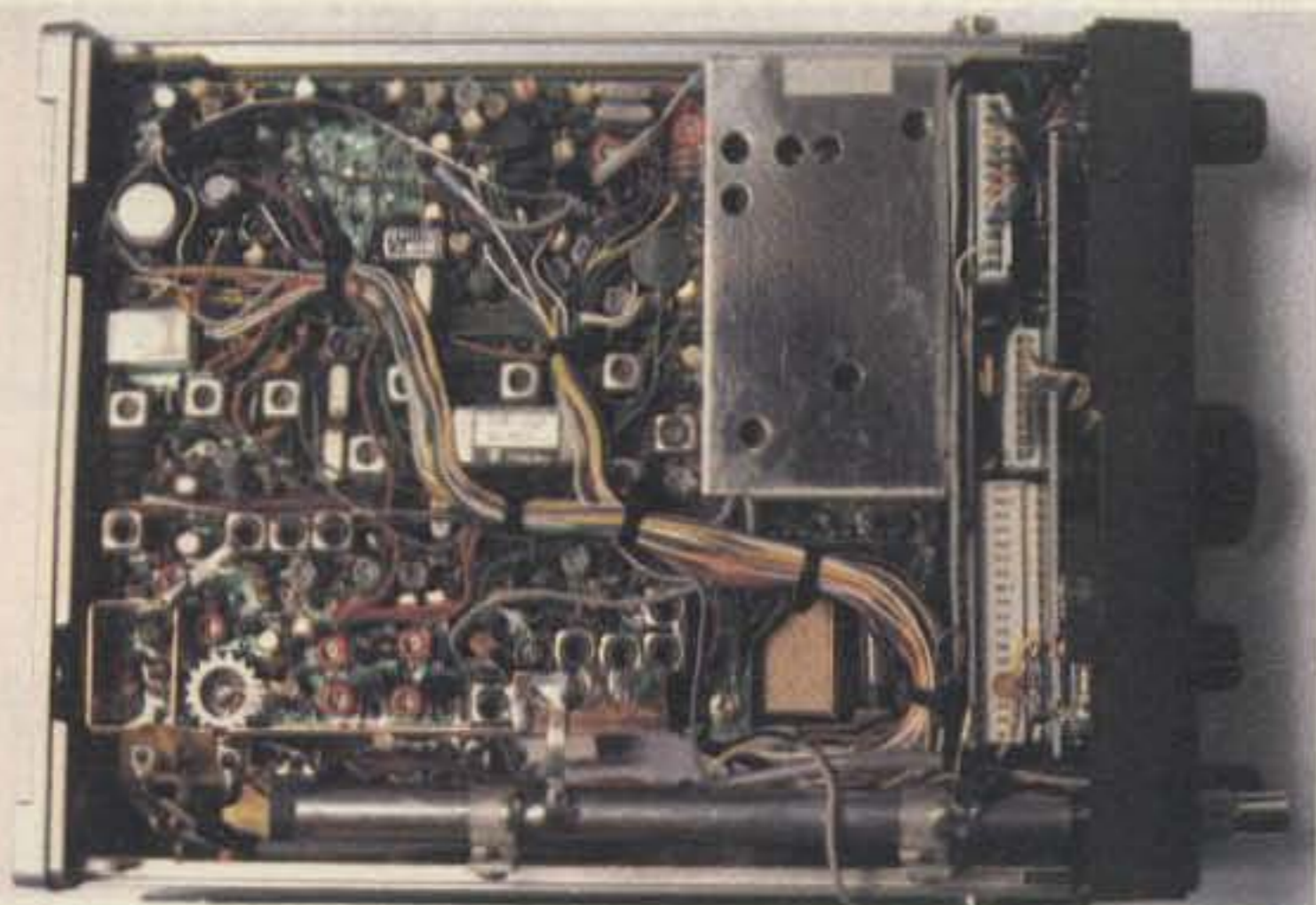
Top view of the FT-290.
