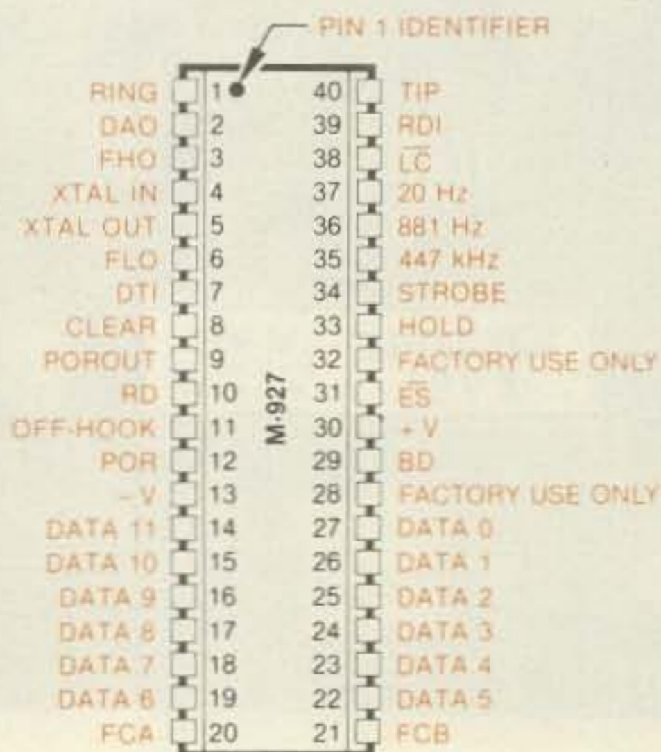
Fig. 1(b). Pinout of the M-927.
