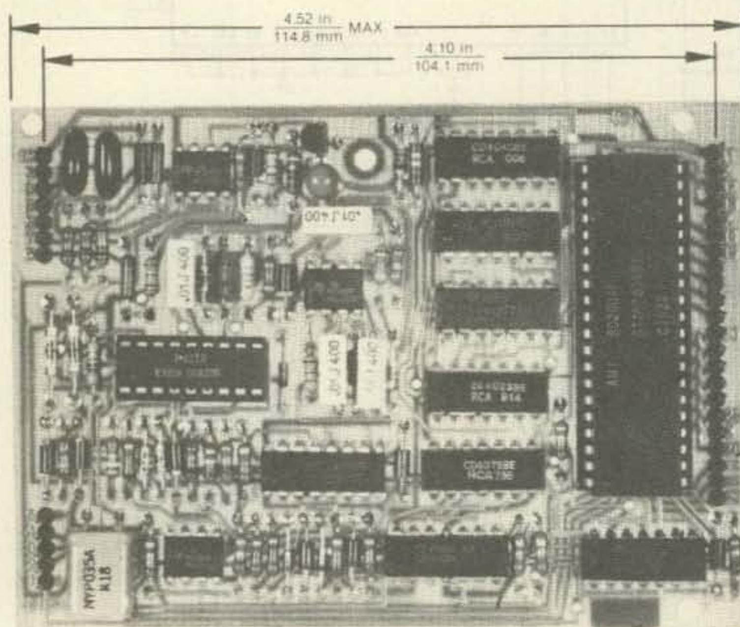
Photo B. The M-937 touchtone decoder.
