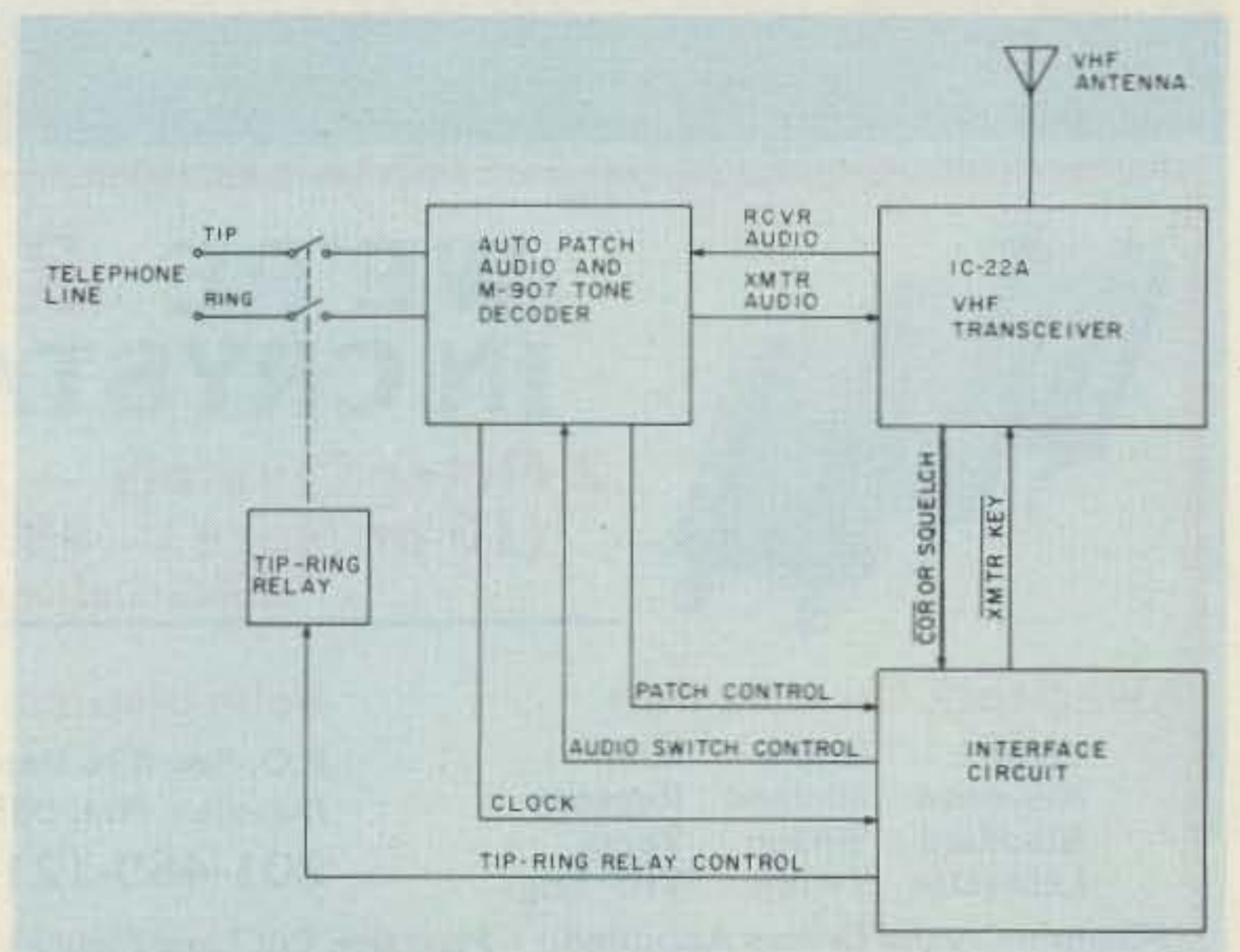
Fig. 3. Block diagram.
