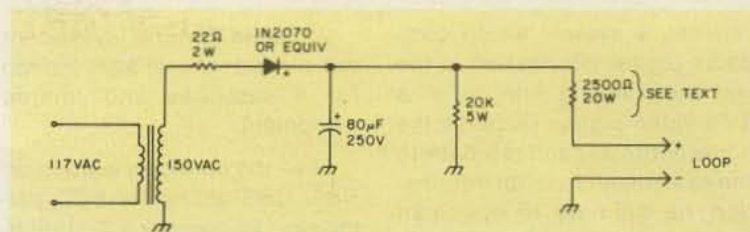
Fig. 1. A local loop supply.
