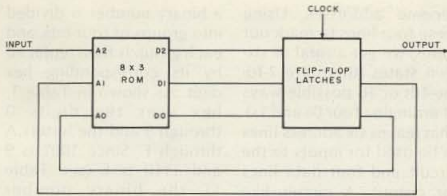
Fig. 4. A more complex controller.
