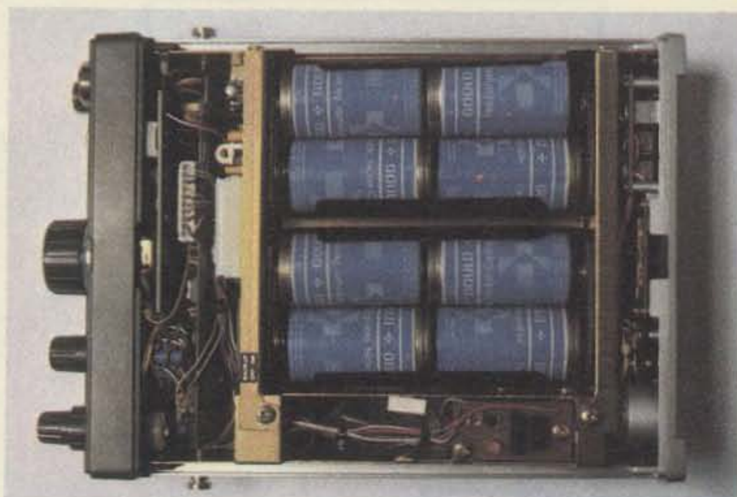
Bottom view of the FT-290.
