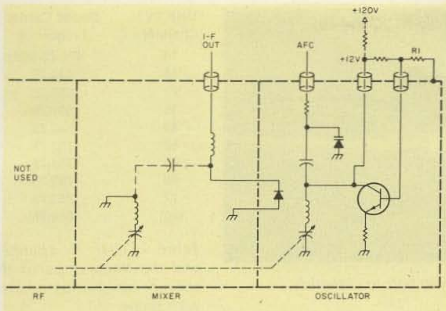
Fig. 1. Typical schematic of oscillator and mixer sections of UHF converters. Power supply is either 12 volts or 120 volts through a dropping resistor. The afc circuit can be used for frequency modulation or fine tuning, and the detector diode is used to monitor relative power output.
