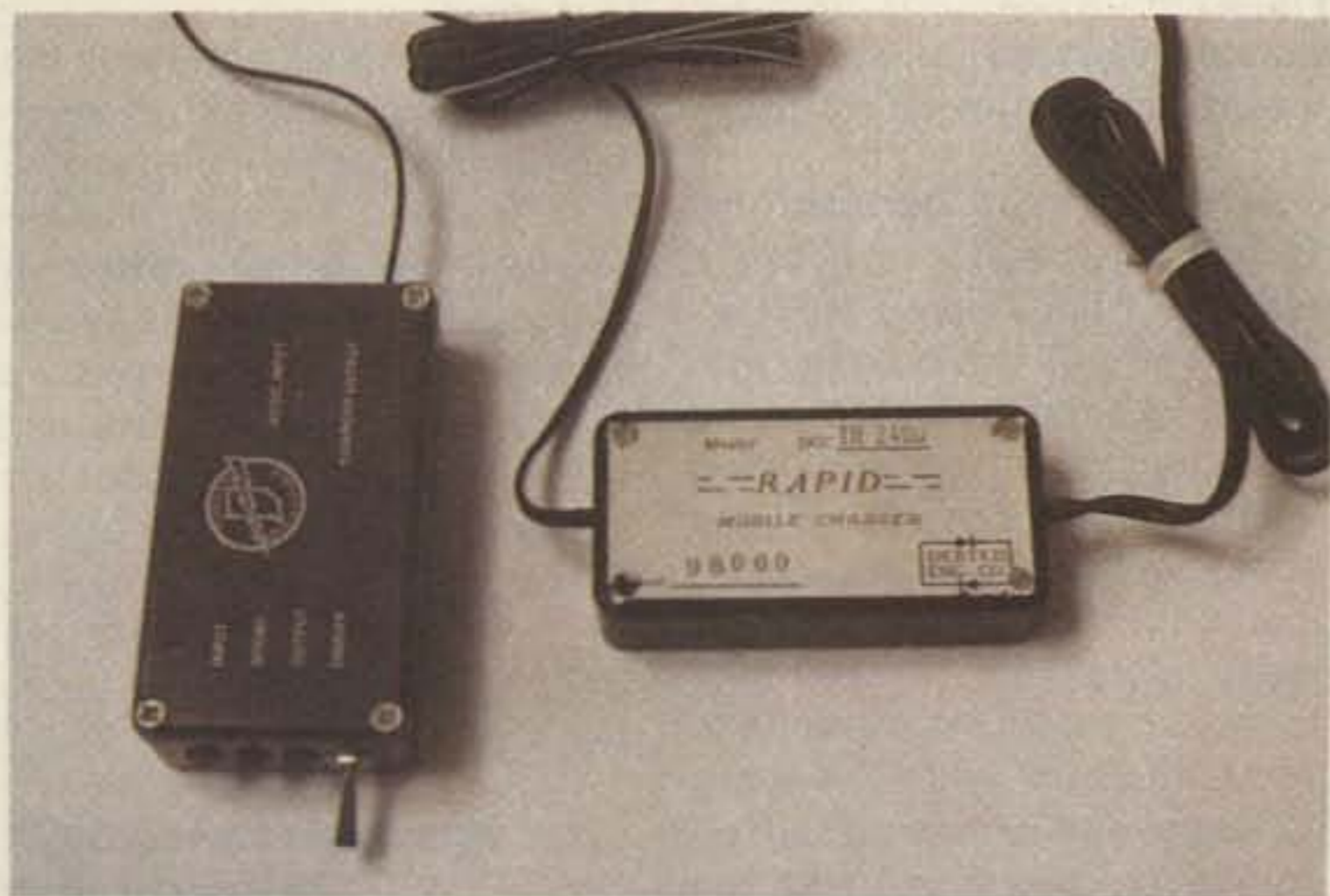
The Debco Deb-Ted Rapid Mobile Charger and the Indiana Quick Charge QC-500 charger.
