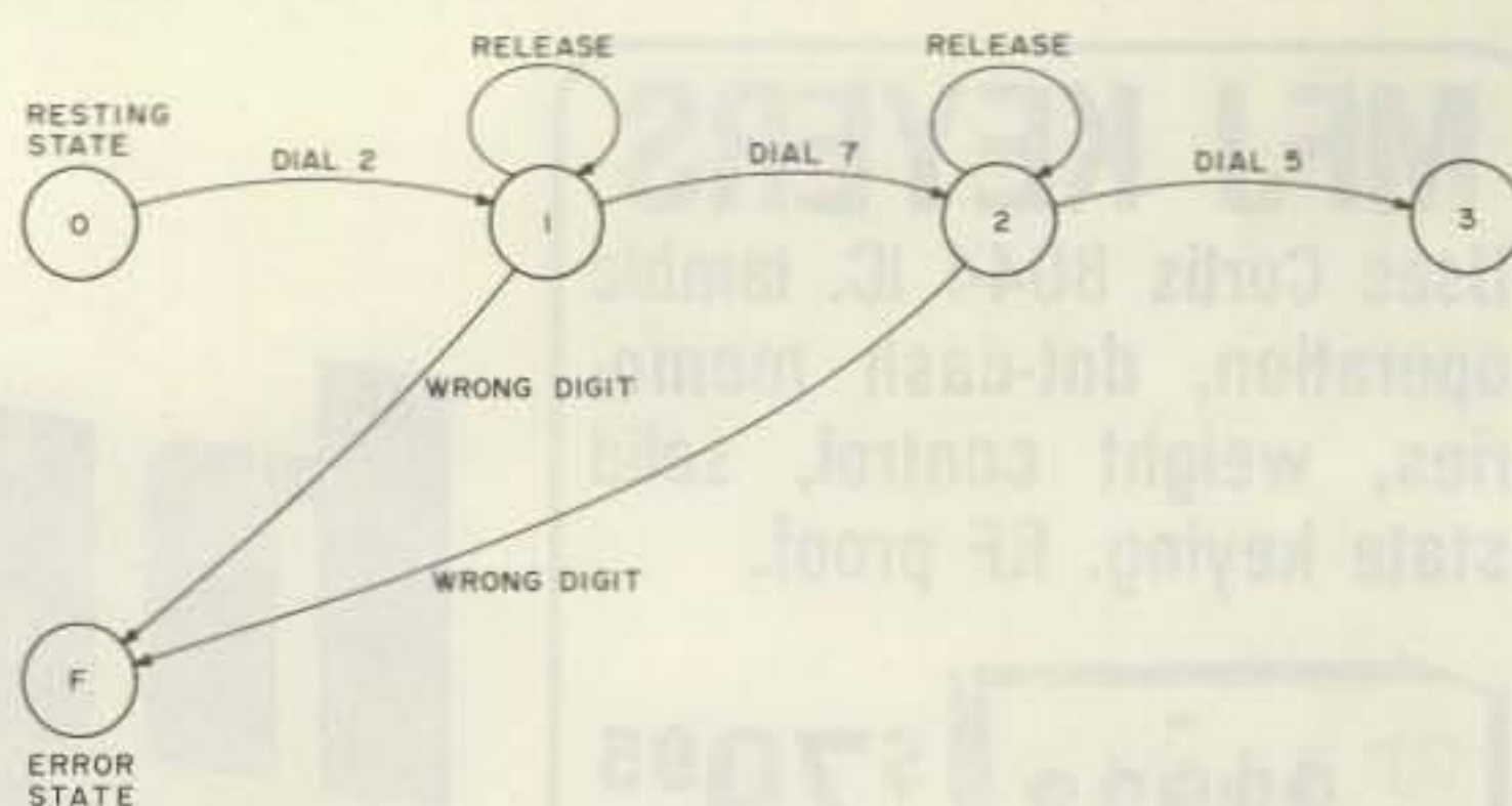
Fig. 8. Partial state map for touchtone-sequence detector.
