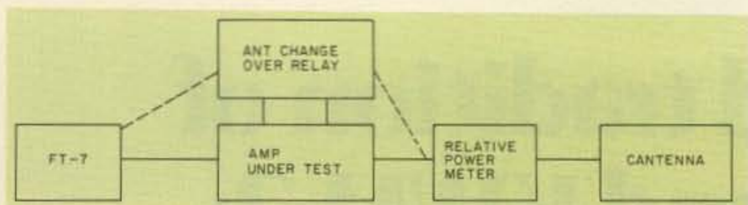
Fig. 4. Passive-grid amplifier test setup for common-grid configuration.
