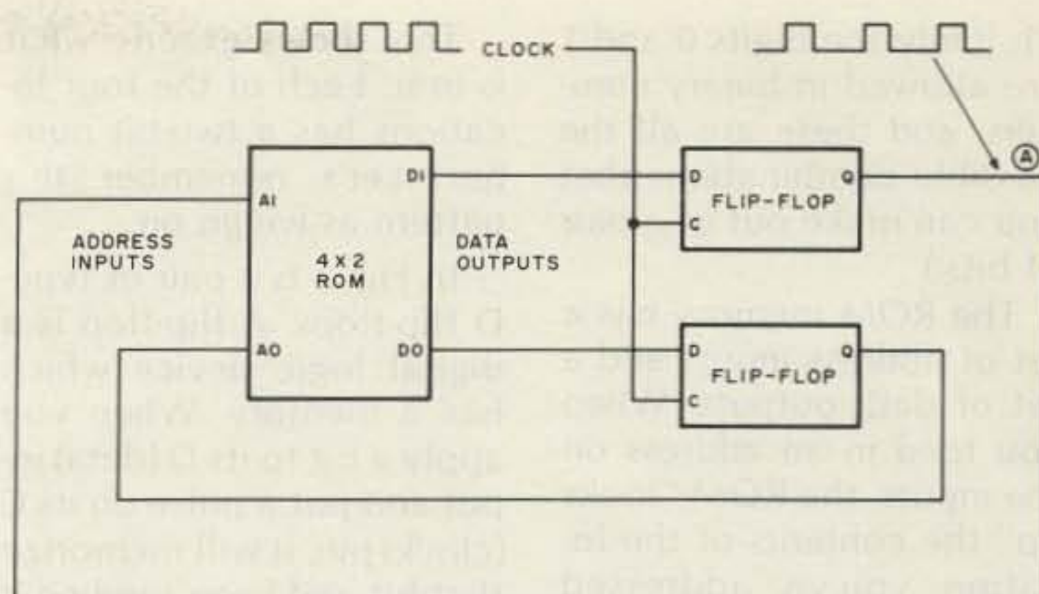
Fig. 2. A very simple micro-programmed sequential circuit.
