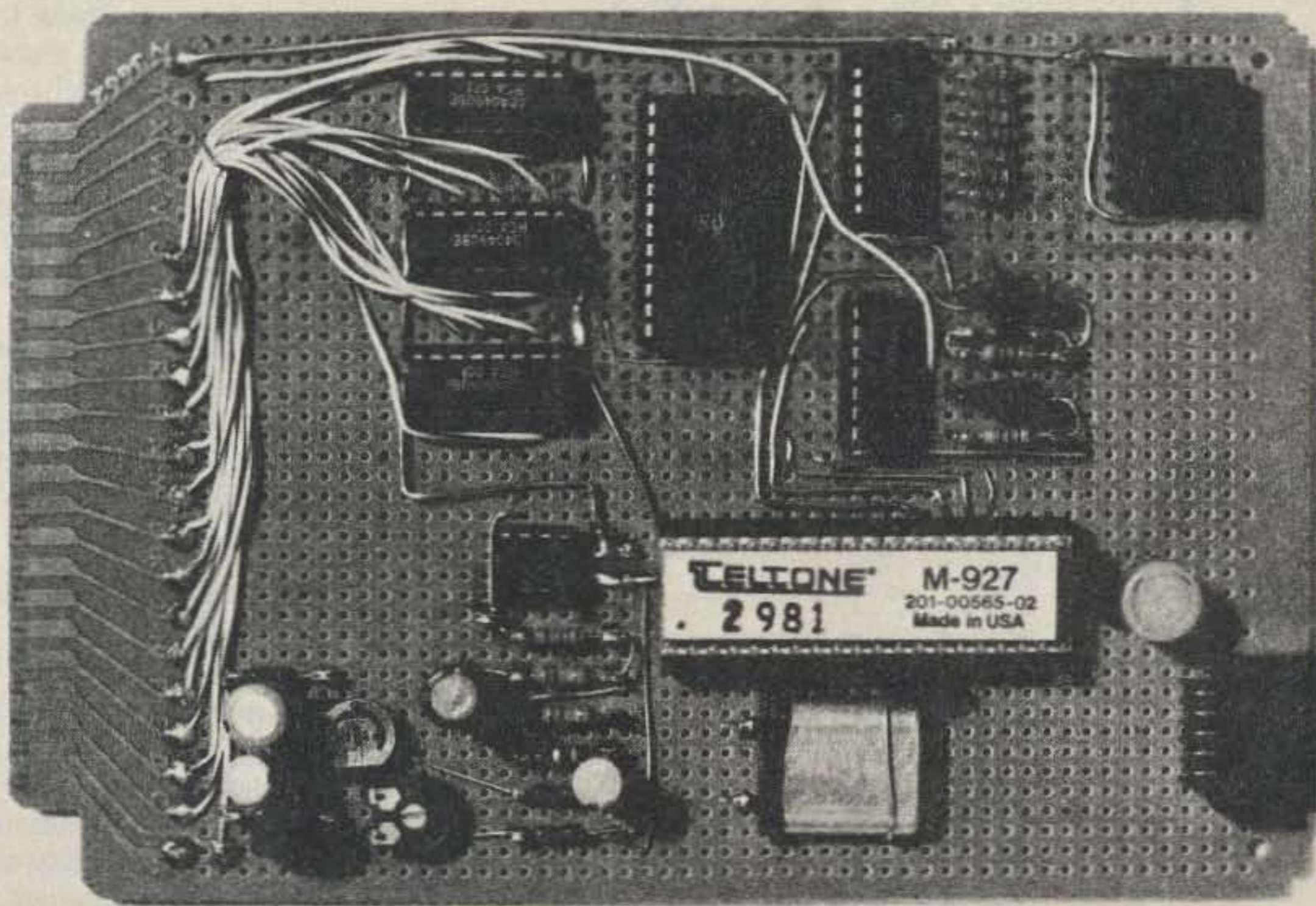
Photo A. The assembled tone decoder board. (Photo by Vic Klein WA4THR)
