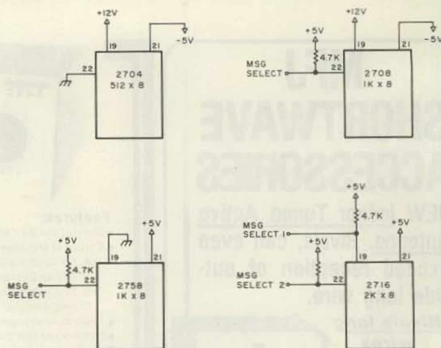
Fig. 10. Four different EPROMs can be used.
