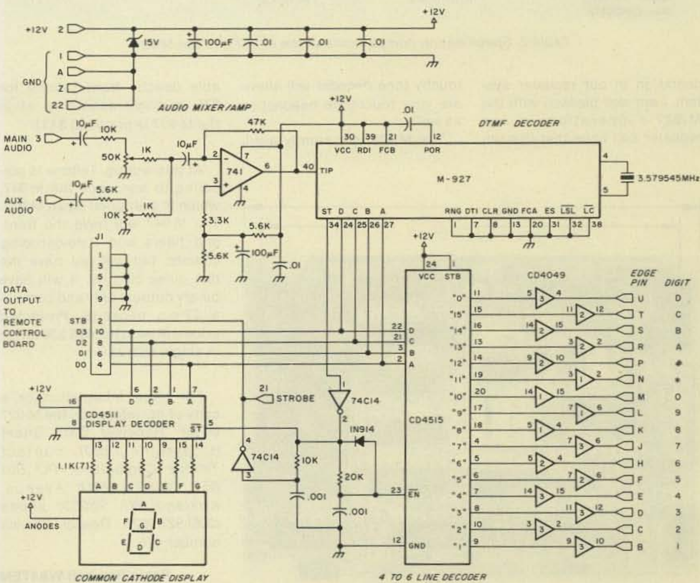
Fig. 3. The tone decoder board schematic.
