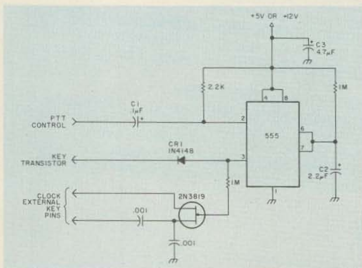
Fig. 2. Clock timer. C1 through C3 are tantalum.
