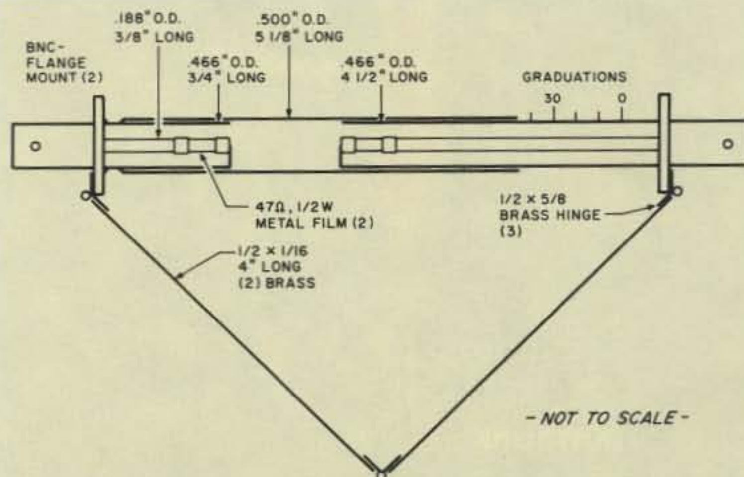
Fig. 6. Attenuator assembly shown in cross section.
