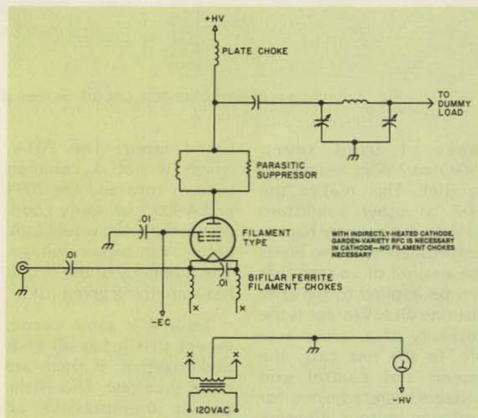
Fig. 1. Grounded-grid amplifier test circuit.
