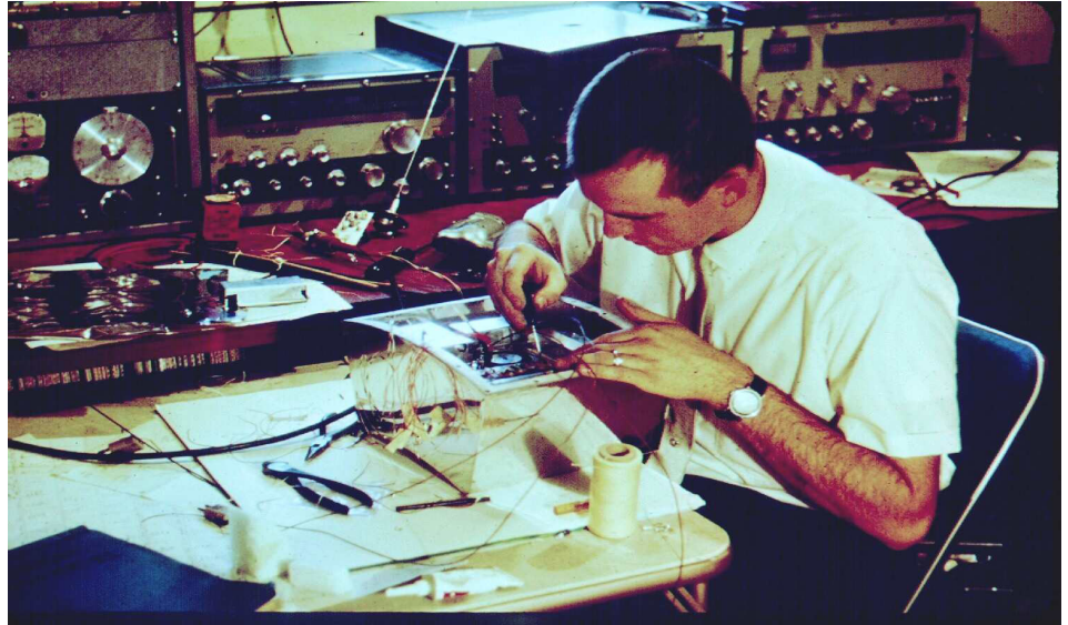
Lance Ginner, K6GSJ, performs the final wiring of the flight model OSCAR-I satellite on a card table set in the ham shack of his California home. [Photo courtesy of Project OSCAR.]
