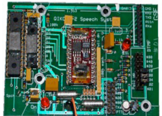
Figure 11 - DTMF speech board on QIKCOM-2
