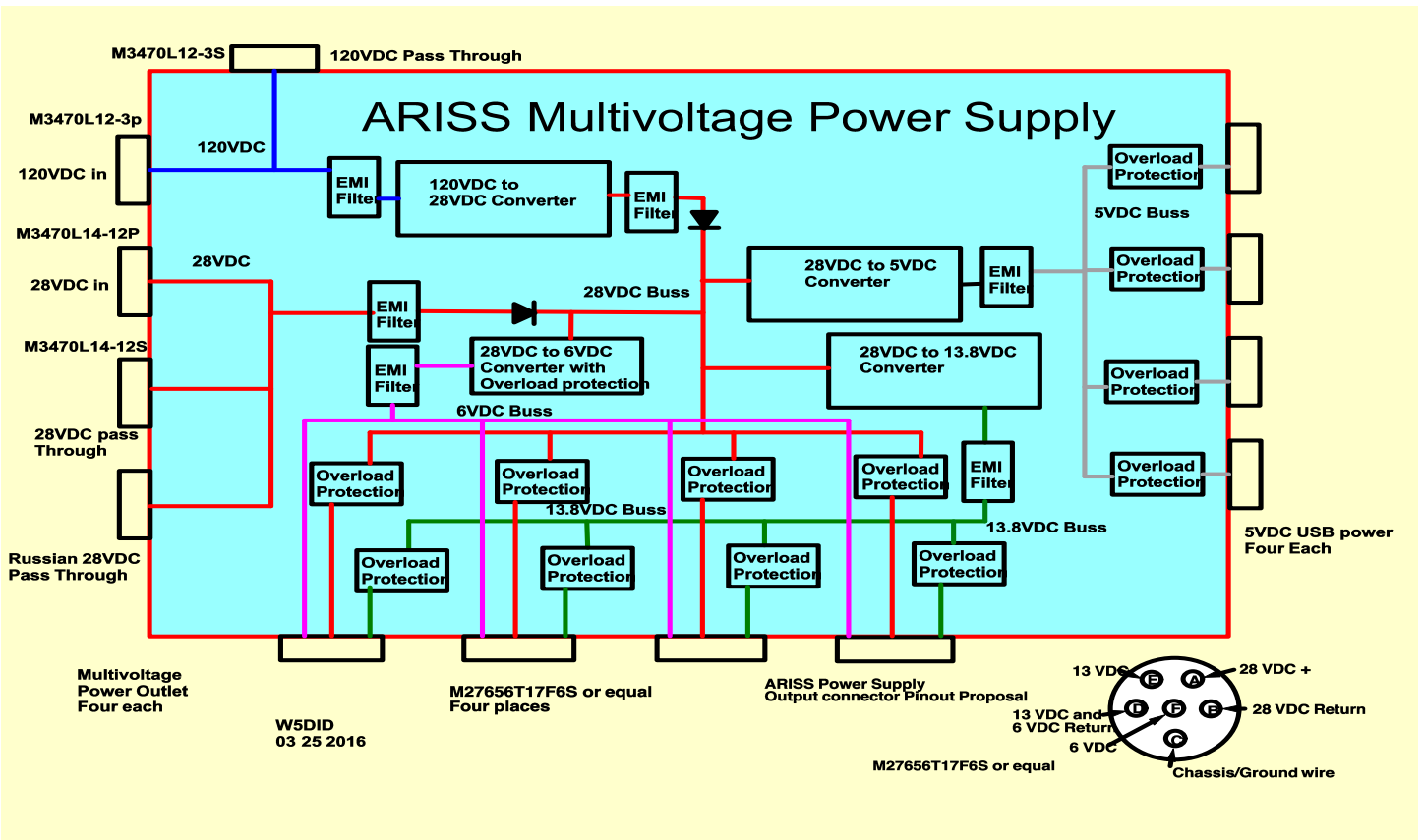
Figure 2 - Low voltage power supply more details
