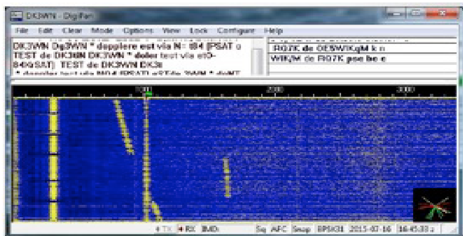
Figure 4 - Downlink waterfall shows stations with and without Doppler shift correction.
