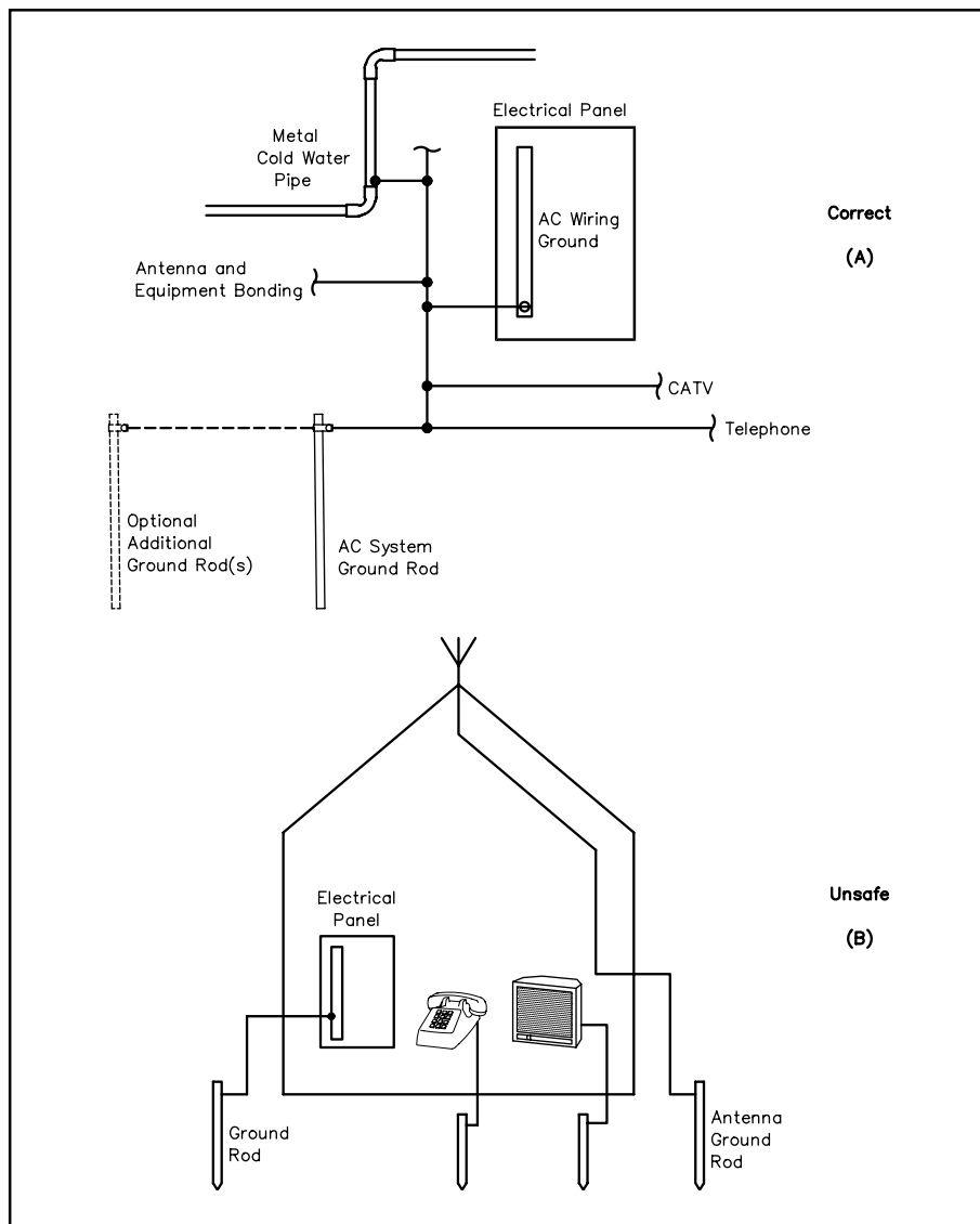
Fig 9.3—At A, proper bonding of all grounds to electrical service panel. Installation shown at B is unsafe—the separate grounds are not bonded. This could result in a serious accident or electrical fire.
