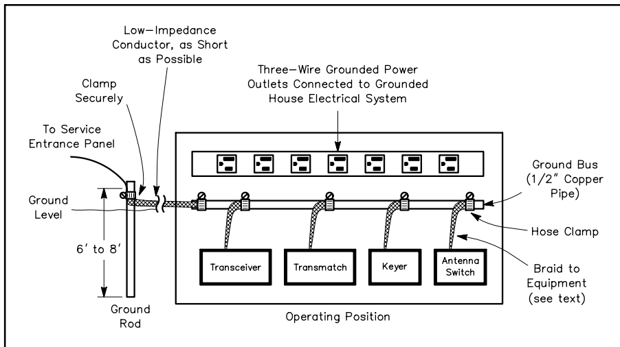
Fig 9.6—An effective station ground bonds the chassis of all equipment together with low-impedance conductors and ties into a good earth ground. Note that the ground bus is in turn bonded to the service entrance panel. This connection should be made by a licensed electrician with #6 AWG (minimum size) copper wire.
