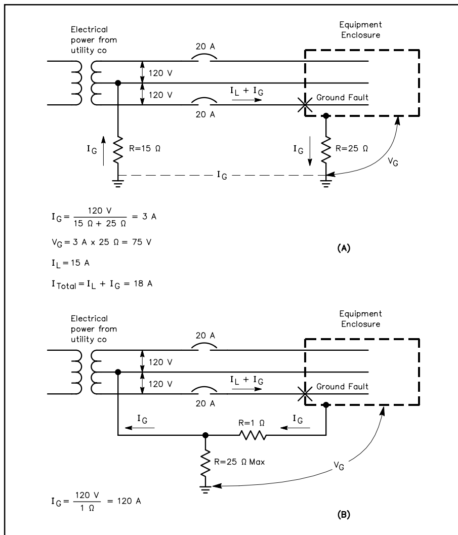
Fig 9.4— These drawings show the importance of properly bonded ground rods. In the system shown in A, the 20-A breaker will not trip. In the system in B, the 20-A circuit breaker trips instantly. There is an equipment internal short to ground—the ground rod is properly bonded back to the power system ground.
