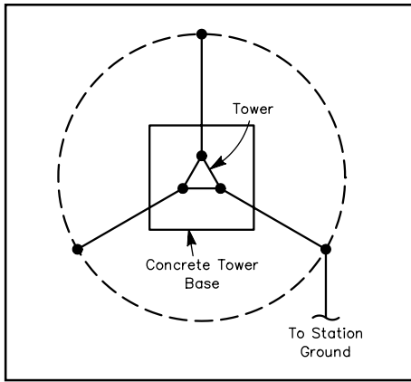
Fig 9.5—Schematic of a properly grounded tower. A bonding conductor connects each tower leg to a ground rod and a buried (1 ft deep) bare, tinned copper ring (dashed line), which is also connected to the station ground and then to the ac safety ground. Locate ground rods on the ring, as close as possible to their respective tower legs. All connectors should be compatible with the tower and conductor materials to prevent corrosion. See text for conductor sizes and details of lightning and voltage transient protection.
