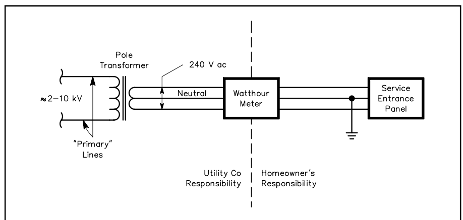
Fig 9.1—Typical division of responsibility for maintenance of electrical power conductors and equipment. The meter is supplied by the utility company.
