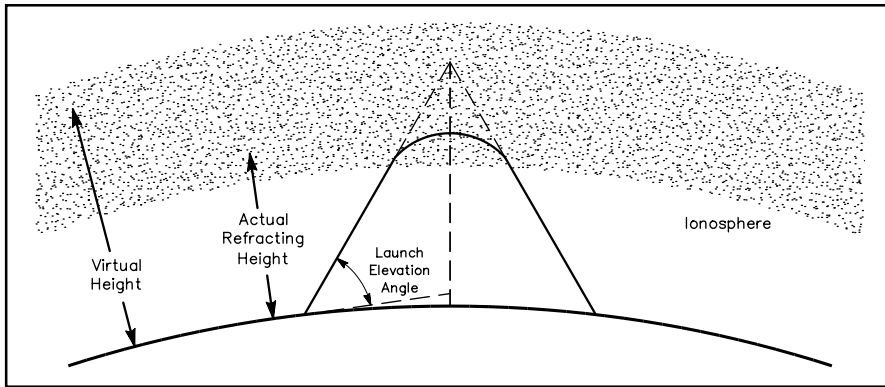
Fig 21.7 —Gradual refraction in the ionosphere allows radio signals to be propa-gated long distances. It is often convenient to imagine the process as a reflection with an imaginary reflection point at some virtual height above the actual refracting region. The other figures in this chapter show ray paths as equivalent reflections, but you should keep in mind that the actual process is a gradual refraction.
