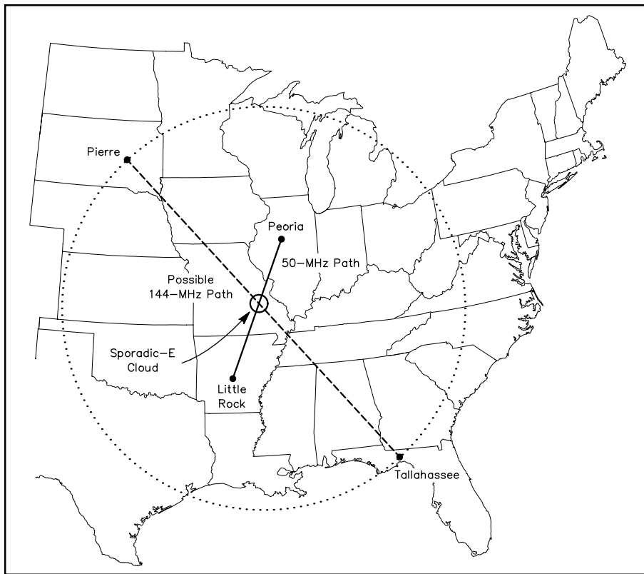
Fig 21.15—50 MHz sporadic-E contacts of 700 km (435 mi) or shorter (such as between Peoria and Little Rock) indicate that the MUF on longer paths is above 144 MHz. Using the same sporadic-E region reflecting point, 144-MHz contacts of 2200 km (1400 mi), such as between Pierre and Tallahassee, should be possible.
