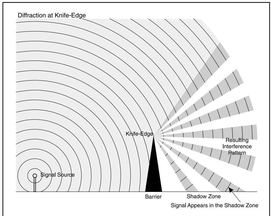
Fig 21.4—Radio, light and other waves are diffracted around the sharp edge of a solid object that is large in terms of wavelengths. Diffraction results from interference between waves right at the knife-edge and those that are passing above it. Some signals appear behind the knife-edge as a consequence of the interference pattern. Hills or mountains can serve as natural knife-edges at radio frequencies.
