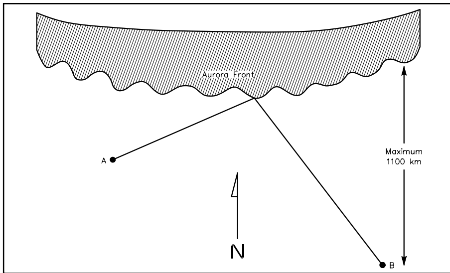
Fig 21.16—Point antennas generally north to make oblique long-distance contacts on 28 through 432 MHz via aurora scattering. Optimal antenna headings may shift considerably to the east or west depending on the location of the aurora.
