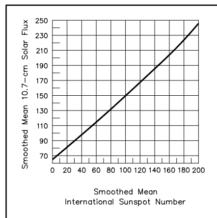
Fig 21.12 —Approximate conversion between solar flux and sunspot number.
