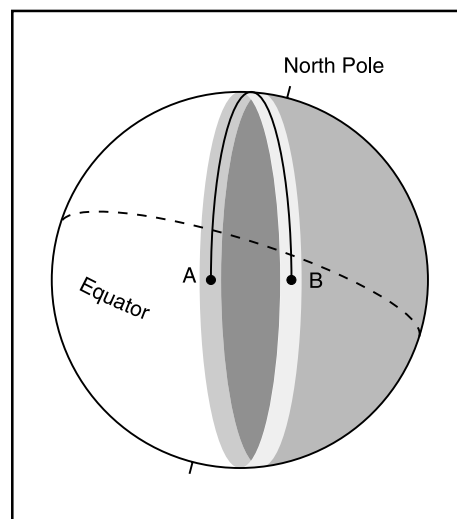
Fig 21.18—The gray line encircles the Earth, but the tilt at the equator to the poles varies over 46° with the seasons. Long-distance contacts can often be made halfway around the Earth along the gray line, even as low as 1.8 and 3.5 MHz. The strength of the signals, characteristic of gray-line propagation, indicates that multiple Earth-ionosphere hops are not the only mode of propagation, since losses in many such hops would be very great. Chordal hops, where the signals are confined to the ionosphere for at least part of the journey, are involved.
