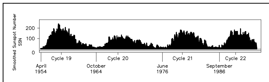
Fig 21.11 —Average monthly sunspot numbers for Solar Cycles 19 to 22.
