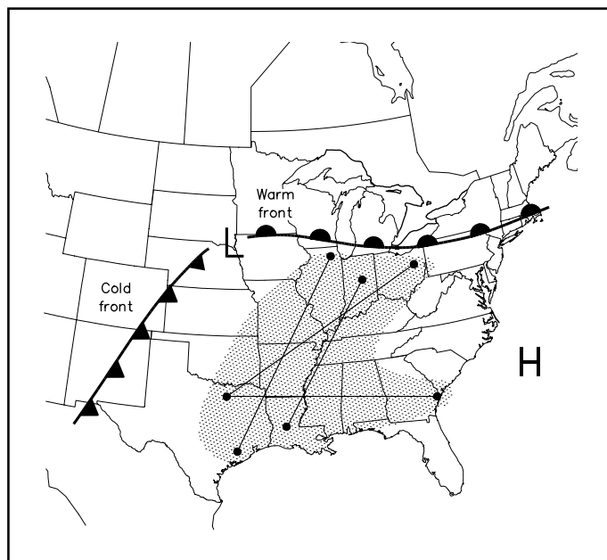
Fig 21.28 —Surface weather map for June 2, 1980, with a typical spring wave cyclone over the southeastern quarter of the US. The shaded portion shows where ducting conditions existed.
