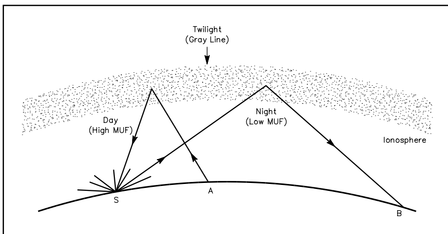
Fig 21.20 —Backscatter path across the gray line. Stations A and B are too close to make contact via normal ionospheric refraction, but may hear each other's signals scattered from point S. Station A makes use of a high-angle refraction on the day side of the gray line, where the MUF is high. Station B makes use of a night-time refraction, with a lower MUF and lower angle of propagation. Note that station A points away from B to complete the circuit.
