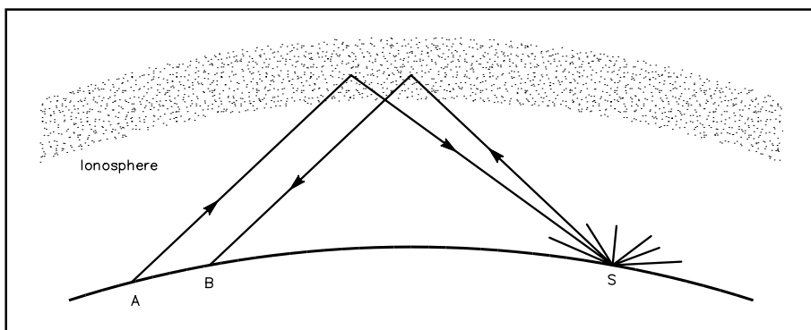
Fig 21.19 —Schematic of a simple backscatter path. Stations A and B are too close to make contact via normal F-layer ionospheric refraction. Signals scattered back from a distant point on the Earth's surface (S), often the ocean, may be accessible to both and create a backscatter circuit.
