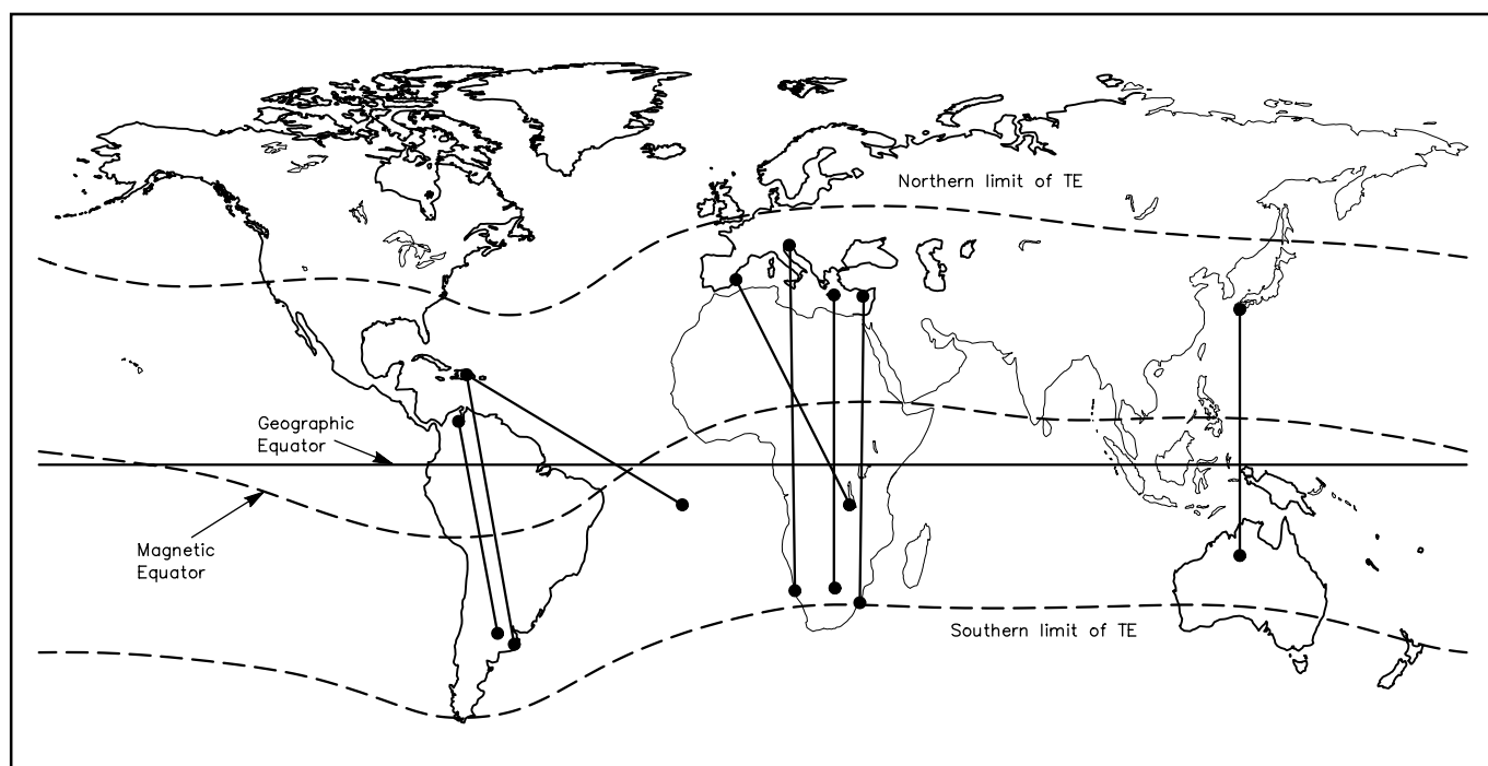
Fig 21.21—Transequatorial spread-F propagation takes place between stations equidistant across the geomagnetic equator. Distances up to 8000 km (5000 mi) are possible on 28 through 432 MHz. Note the geomagnetic equator is considerably south of the geographic equator in the Western Hemisphere.
