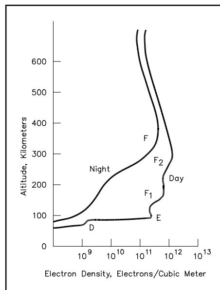
Fig 21.14—Typical electron densities for the various ionospheric regions.
