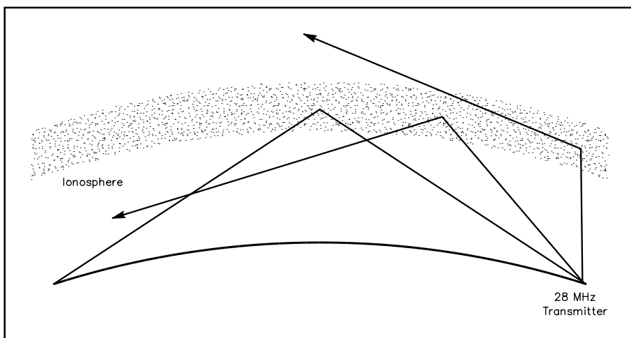
Fig 21.10—Signals at the MUF propagated at a low angle to the horizon provide the longest possible one-hop distances. In this example, 28-MHz signals entering the ionosphere at higher angles are not refracted enough to bring them back to Earth.
