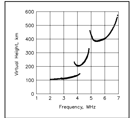
Fig 21.8 —Simplified vertical incidence ionogram showing echoes returned from the E, F 1 and F 2 layers. The critical frequencies of each layer (4.1, 4.8 and 6.8 MHz) can be read directly from the ionogram scale.
