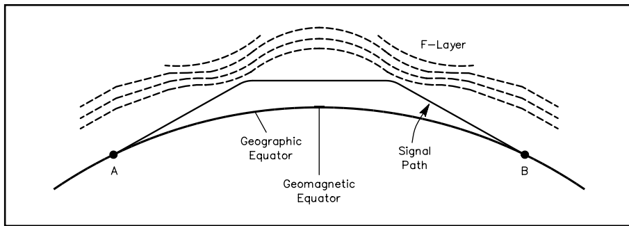
Fig 21.22—Cross-section of a transequatorial spread-F signal path, showing the effects of ionospheric bulging and a double refraction above the normal MUF.
