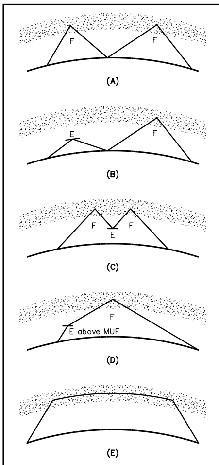
Fig 21.17—Multihop paths can take many different configurations, including a mixture of E- and F-layer hops. (A) Two F-layer hops. Five or more consecutive F-layer hops are possible. (B) An E-layer hookup to the F layer. (C) A top-side E-layer reflection can shorten the distance of two F-layer hops. (D) Refraction in the E layer above the MUF is insufficient to return the signal to Earth, but it can go on to be refracted in the F layer. (E) The Pedersen ray, which originates from a signal launched at a relatively high angle above the horizon into the E or F region, may result in a single-hop path, 5000 km (3100 mi) or more. This is considerably further than the normal 4000-km (2500 mi) maximum F-region single-hop distance, where the signal is launched at a very low takeoff angle. The Pedersen ray can easily be disrupted by any sort of ionospheric gradient.
