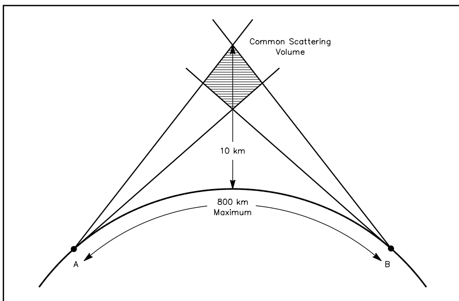
Fig 21.24—Tropospheric-scatter path geometry. The lower boundary of the common scattering volume is limited by the take-off angle of both stations. The upper boundary of 10 km (6 mi) altitude is the limit of efficient scattering in the troposphere. Signal strength increases with the scattering volume.
