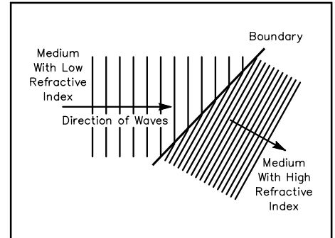
Fig 21.3—Radio waves are refracted as they pass at an angle between dissimilar media. The lines represent the crests of a moving wave front and the distance between them is the wavelength. The direction of the wave changes because one end of the wave slows down before the other as it crosses the boundary between the two media. The wavelength is simultaneously shortened, but the wave frequency (number of crests that pass a certain point in a given unit of time) remains constant.
