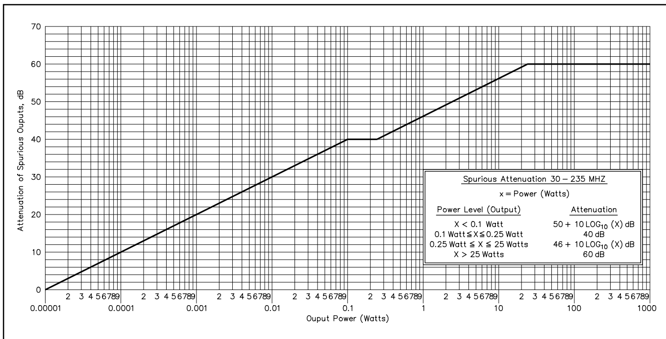
Fig 29.4 —Required attenuation of spurious outputs, 30-235 MHz.
