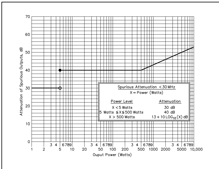
Fig 29.3 —Required attenuation of spurious outputs below 30 MHz is related to output power.
