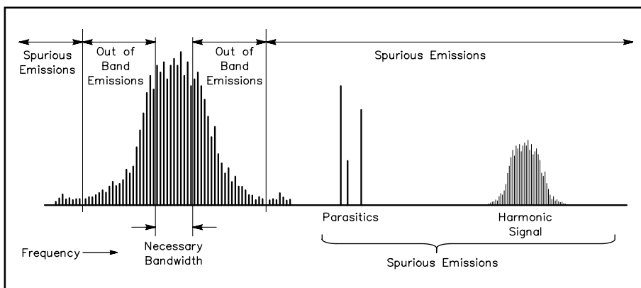
Fig 29.2—Some of the modulation products are outside the necessary bandwidth. These are out-of-band emissions, but they are not considered spurious emissions. On the other hand, these out-of-band emissions must not interfere with other stations [97.307(b)]. The harmonics and parasitics shown in this figure are spurious emissions, and they must be reduced to the levels specified in Part 97. The FCC states that all spurious emissions must be reduced “to the greatest extent practicable” [97.307(c)]. Further, if any spurious emission, including chassis or power-line radiation, causes harmful interference to the reception of another radio station, the licensee of the interfering amateur station is required to take steps to eliminate the interference.
