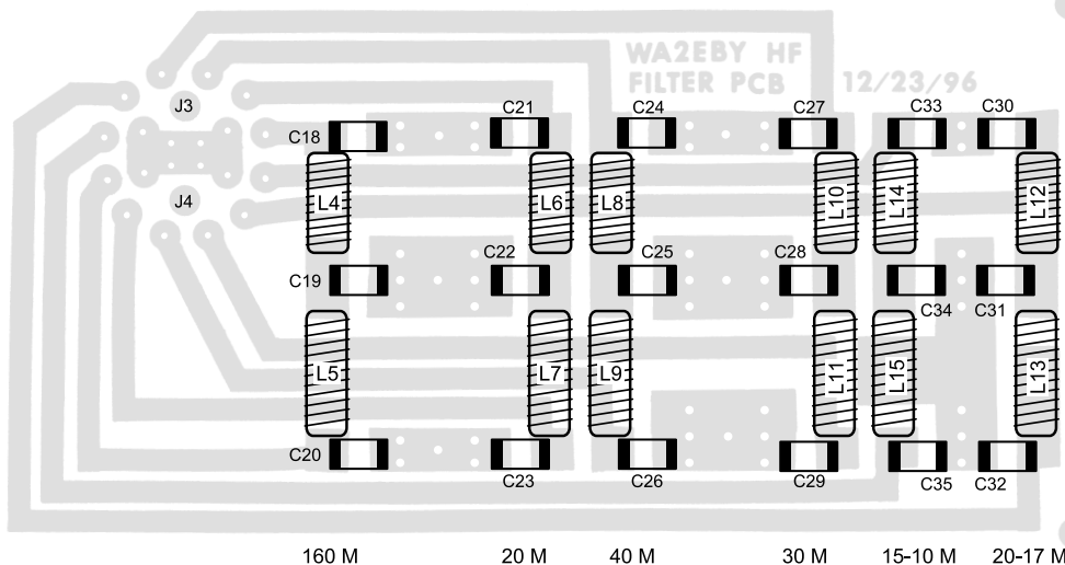
Filter Board Parts-Placement Diagram
