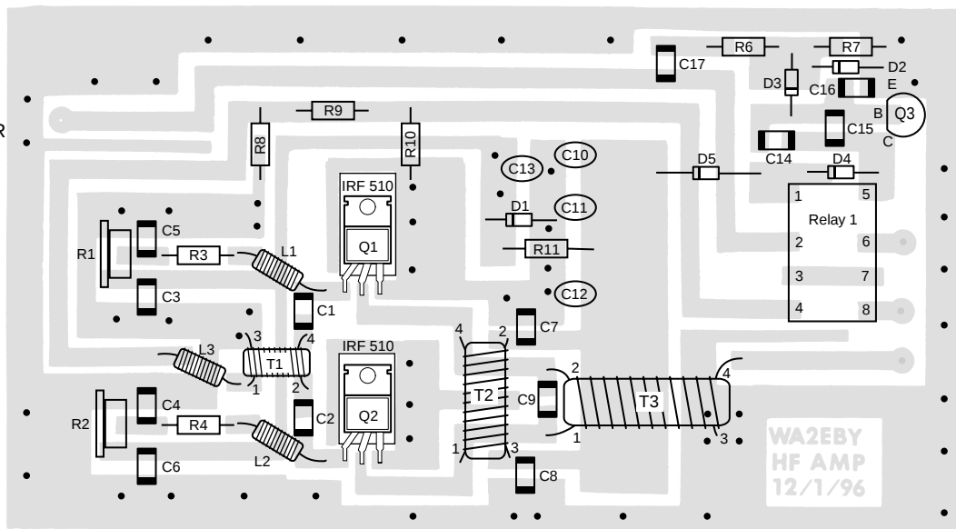
Amplifier Board Parts-Placement Diagram
