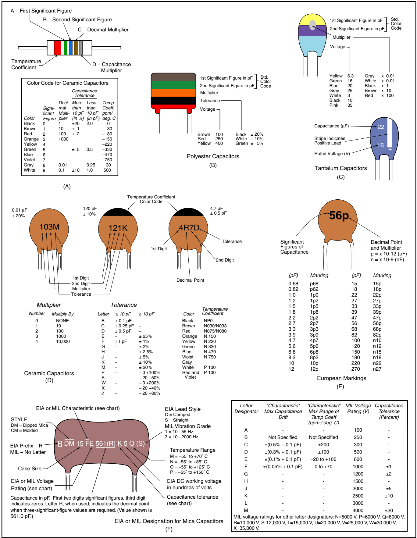
Fig 24.3—Capacitors can be identified by color codes and markings. Shown here are identifying markings found on many common capacitor types.
