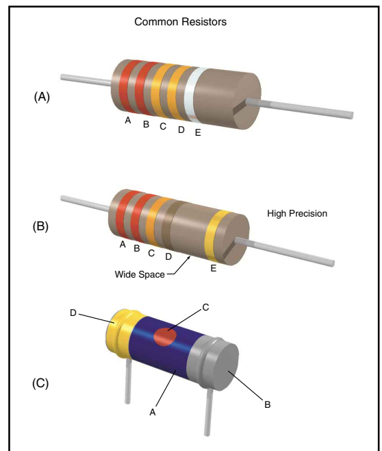
Fig 24.1—Color coding and body size for fixed resistors. The color code is given in Table 24.2. The colored areas have the following significance. A—First significant figure of resistance in ohms. B—Second significant figure. C—Decimal multiplier. D—Resistance tolerance in percent. If no color is shown the tolerance is ±20%. E—Relative percent change in value per 1000 hours of operation; Brown, 1%; Red 0.1%; Orange 0.01%; Yellow 0.001%.
