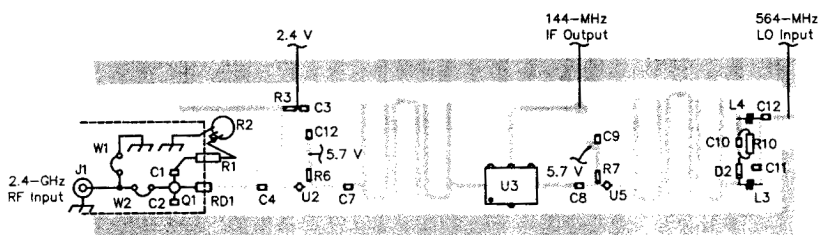
Fig 6—Parts-placement diagram for the Teflon microwave board.
