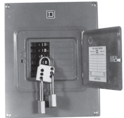
Fig 3.2 — If the switch box feeding power to your shack is equipped with a lock-out hole, use it. With a lock through the hole on the box, the power cannot be accidentally turned back on. (Photo courtesy of American ED-CO)
