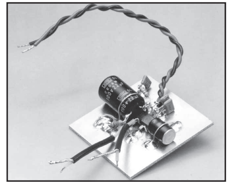
Fig 8.11—The example audio amplifier of Fig 8.10 built using ground-plane construction.
