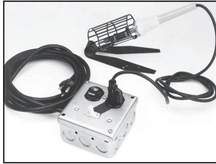
Fig 8.7—An incandescent-light dimmer controls soldering-iron tip temperature. Only one of the duplex outlets is connected through the dimmer.
