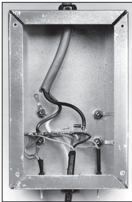
Fig 8.5—View of the soldering-station chassis underside with the bottom plate removed. #24 hookup wire is adequate for all connections. Make sure no possibility of a short circuit exists.
