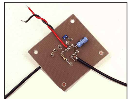
Fig 8.15—The audio amplifier built using terminal-and-wire construction.
