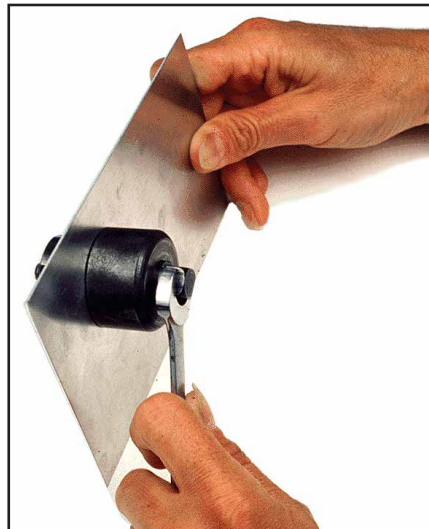
Fig 8.3 —A socket punch is used to easily punch a hole in sheet metal.
