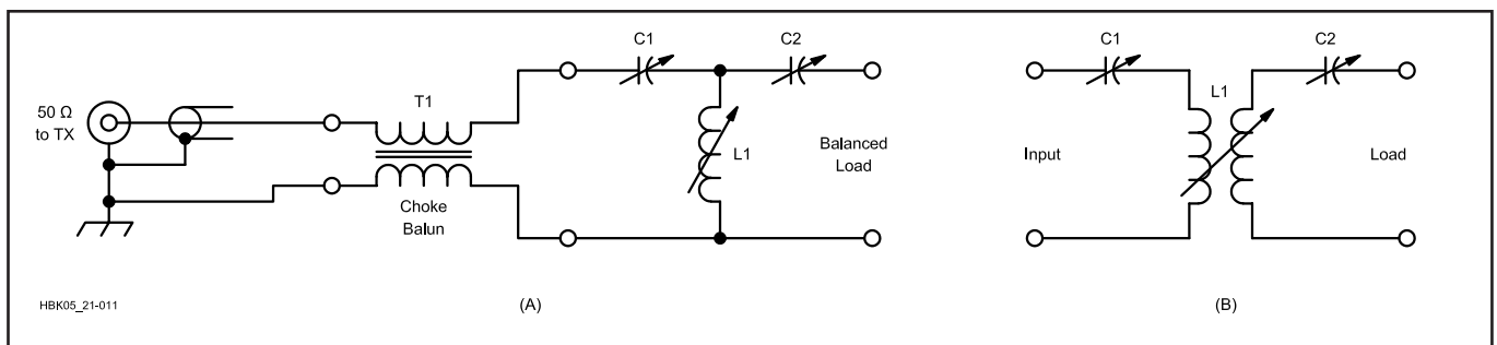
Fig 21.11 —Antenna tuner network in T configuration. This network has become popular because it has the capability of matching a wide range of impedances. At A, the balun transformer at the input of the antenna tuner preserves balance when feeding a balanced transmission line. At B, the T configuration is shown as two L networks back to back.
