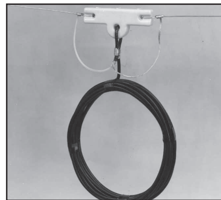
Fig 21.15—RF choke formed by coiling the feed line at the point of connection to the antenna. The inductance of the choke isolates the antenna from the remainder of the feed line.
