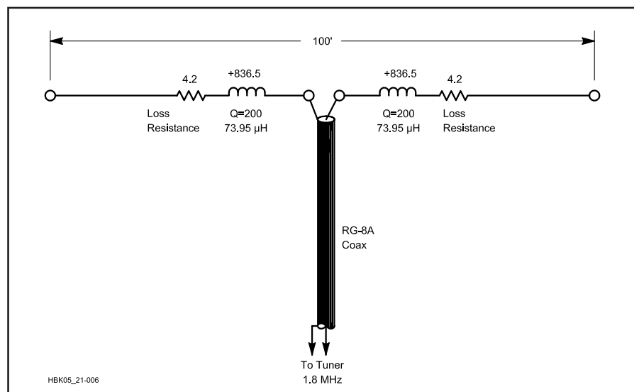
Fig 21.6—The efficiency of the dipole in Table 21.3 can be improved at 1.8 MHz with a pair of inductors inserted symmetrically at the feed point. Each inductor is assumed to have a Q of 200. By resonating the dipole in this fashion the system efficiency, when fed with RG8A coax, is almost 12 dB better than using this same antenna without the resonator. The disadvantage is that the formerly multiband antenna can only be used on a single band.
