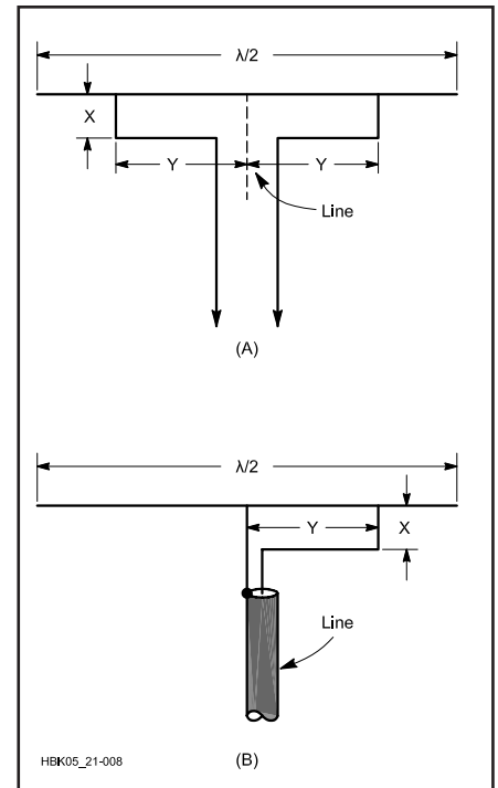
Fig 21.8—The T match (A) and gamma match (B).
