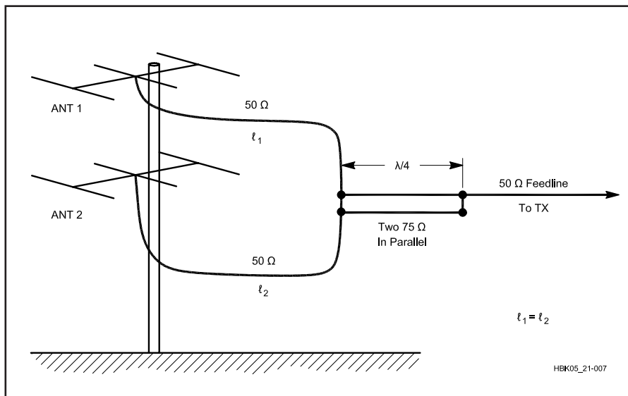
Fig 21.7—Array of two stacked Yagis, illustrating use of quarter-wave matching sections. At the junction of the two equal lengths of 50\text{-}\Omega feed line the impedance is 25 \Omega . This is transformed back to 50 \Omega by the two paralleled 75\text{-}\Omega , quarter-wave lines, which together make a net characteristic impedance of 37.5 \Omega . This is close to the 35.4 \Omega value computed by the formula.
