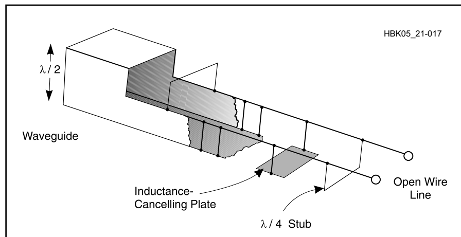
Fig 21.17 —At its cutoff frequency a rectangular waveguide can be analyzed as a parallel two-conductor transmission line supported from top and bottom by an infinite number of quarter-wavelength stubs.
