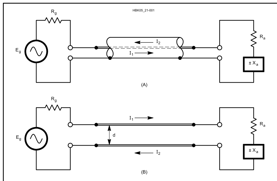
Fig 21.1—In A, coaxial cable transmission line connecting signal generator having source resistance R_g to reactive load R_a \pm jX_a , where X_a is either a capacitive (–) or inductive (+) reactance. Velocity factor (VF) and characteristic impedance ( Z_0 ) are properties of the line, as discussed in the text. B shows open-wire balanced transmission line.
