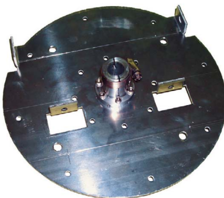
Fig 23.60—A modified antenna base plate assembly. See the text for a description.
