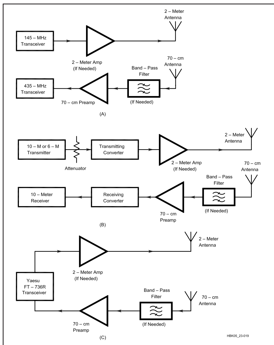
Fig 23.19—Several different Mode-V/U satellite-station configurations for OSCAR 29 are shown here. At A, separate VHF/UHF multimode transceivers are used for transmitting and receiving. The configuration shown at B uses transmitting and receiving converters or transverters with HF equipment. At C, a multimode, multiband transceiver can perform both transmitting and receiving functions, full duplex, in one package.
