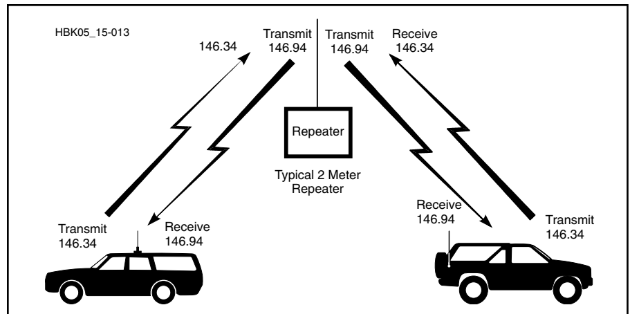
Fig 18.1 — Typical 2-m repeater, showing mobile-to-mobile communication through a repeater station. Usually located on a hill or tall building, the repeater amplifies and retransmits the received signal on a different frequency.
