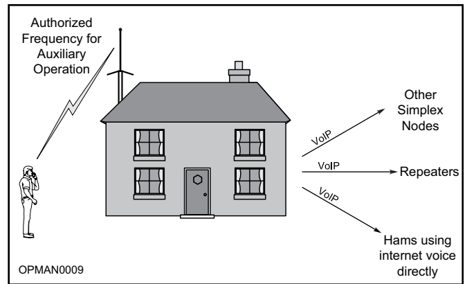
Fig 18.16 — A diagram of a VoIP simplex node. If a control operator is not physically present at the station location and the node is functioning with wireless remote control, the control link must follow the rules for auxiliary operation.
