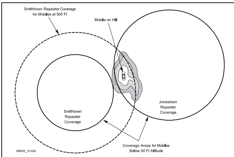
Fig 18.14 — When two repeaters operate on the same frequencies, a well-situated operator can key up both repeaters simultaneously. A directional antenna may help.
