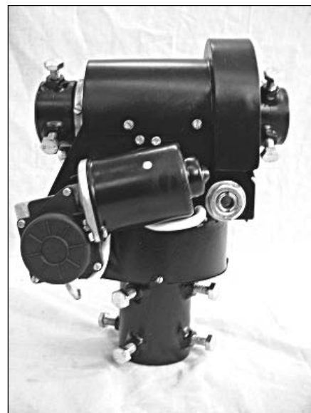
Fig 28 — An az/el rotator made by Alfa Radio.
