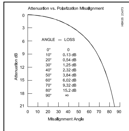
Fig 62 — Attenuation caused by misalignment of a linearly polarized signal with the polarization angle of a receiving antenna. The attenuation increases rapidly for alignment errors greater than 45°.
