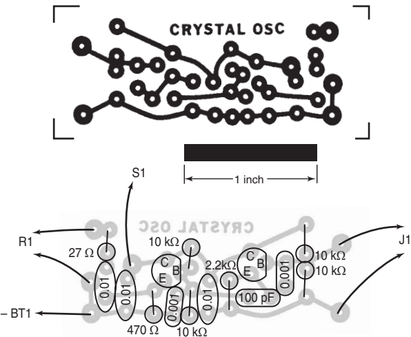
Crystal-Controlled Signal Source
