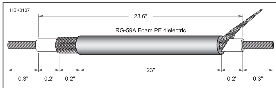
Fig 50 — Feed cables stripping dimensions.
