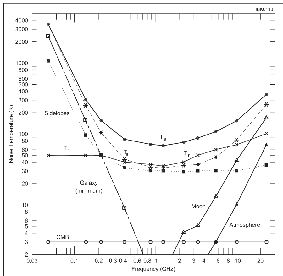
Fig 64 — Typical contributions to system noise temperature T_s as function of frequency. See text for definitions and descriptions of the various sources of noise.
