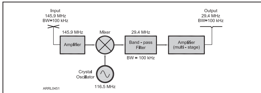
Fig 3 — A simplified block diagram of a linear transponder.
