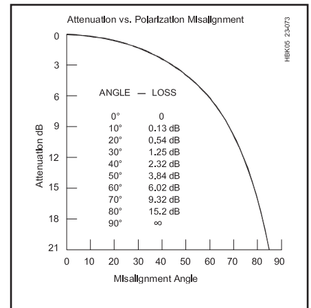
Fig 62 — Attenuation caused by misalignment of a linearly polarized signal with the polarization angle of a receiving antenna. The attenuation increases rapidly for alignment errors greater than 45^\circ .
