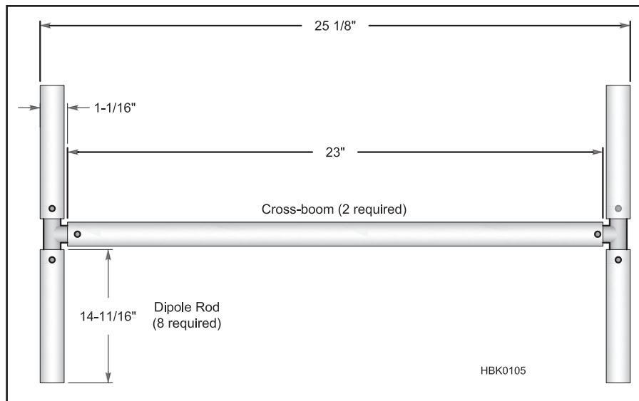
Fig 48 — Dimensions of the dipoles and cross booms. The antenna requires two cross booms, with a dipole at each end of each cross boom (four dipoles total).
