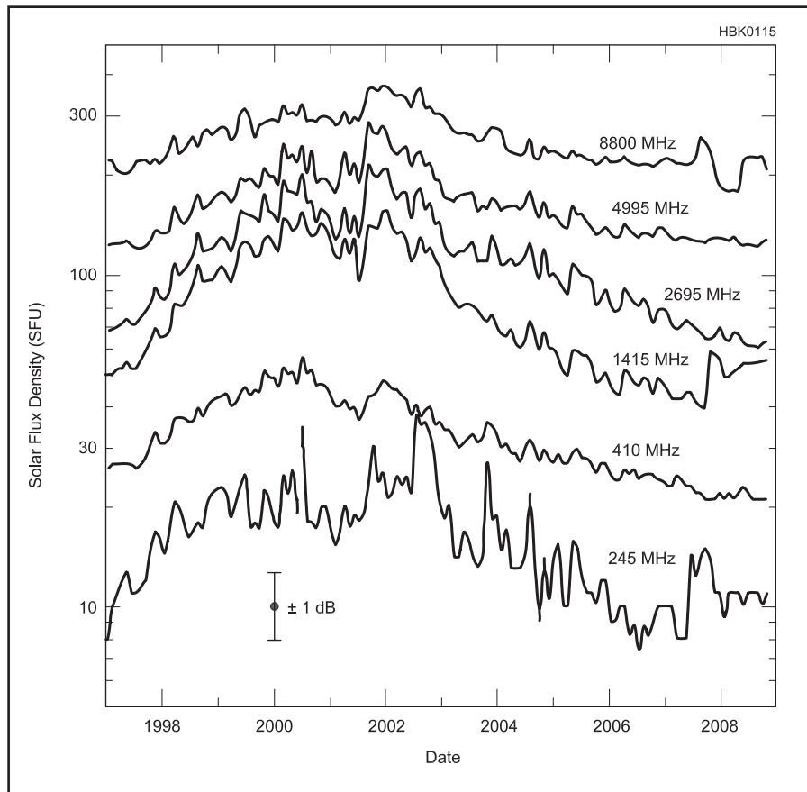
Fig 74 — Monthly median values of solar flux density at six frequencies, over the 11 years of solar cycle 23. Original data are from the Sagamore Hill Observatory in Massachusetts. At the lower frequencies, and especially near solar maximum, day-to-day and even hour-to-hour upward variations can be an order of magnitude larger than those in the monthly medians.
