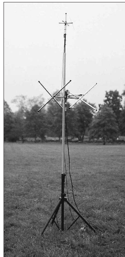
Fig 52 — The EZ-Lindenblad as a portable or Field Day antenna. A 70 cm antenna is on the top.
