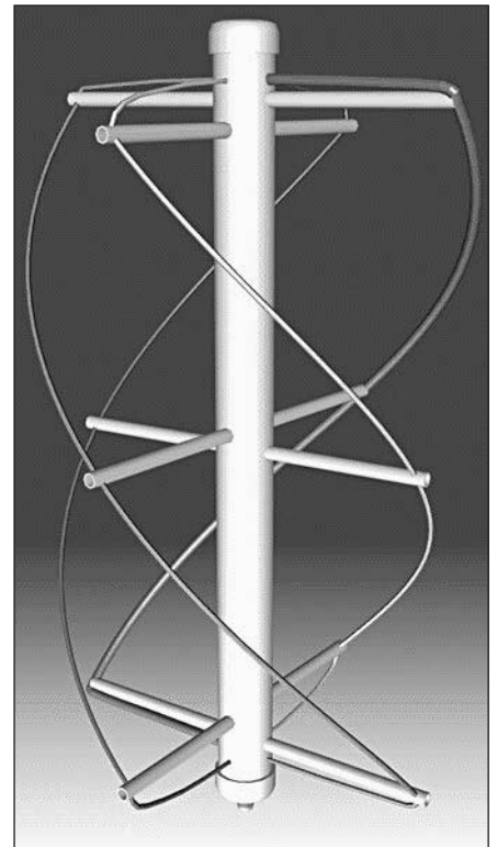
Fig 14 — The quadrifilar helicoidal antenna is comprised of four equal-length conductors (filars) wound in the form of a corkscrew (helix) and fed in quadrature.
