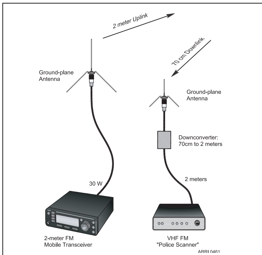
Fig 46 — Let's say that you want to work the low-orbiting FM birds, but you only have a 2 meter FM transceiver for the uplink and only a VHF FM "police scanner" receiver for the 70 cm downlink. You could use a downconverter for the 70 cm downlink, stepping the signal down to 2 meters for reception with the scanner.
