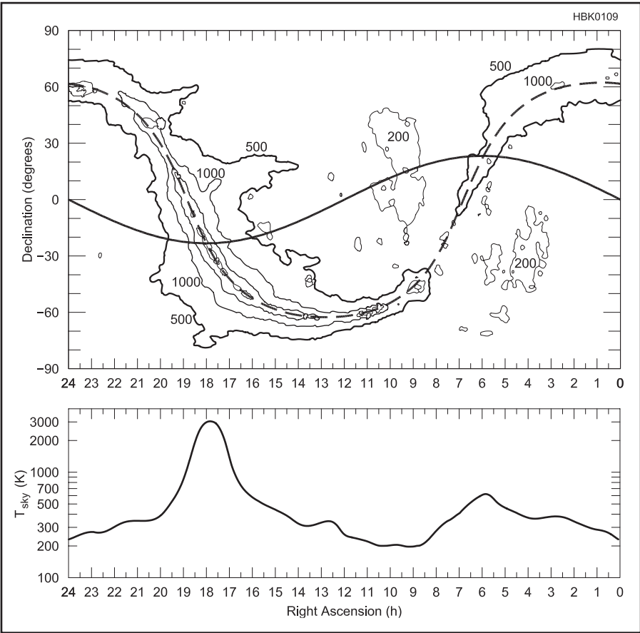
Fig 63 — Top: All-sky contour map of sky background temperature at 144 MHz. The dashed curve indicates the plane of our Galaxy, the Milky Way; the solid sinusoidal curve is the plane of the ecliptic. The Sun follows a path along the ecliptic in one year; the moon moves approximately along the ecliptic ( \pm 5^\circ ) each month. Map contours are at noise temperatures 200, 500, 1000, 2000 and 5000 K. Bottom: One-dimensional plot of sky background temperature at 144 MHz along the ecliptic, smoothed to an effective beamwidth 15^\circ .
