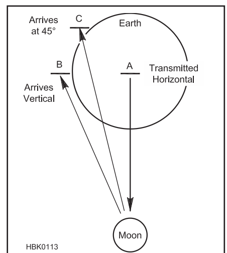
Fig 68 — The spherical Earth creates spatial polarization offsets for well-separated stations with horizon-oriented linear polarization. Here, a signal transmitted horizontally at A arrived with vertical polarization at B and midway between horizontal and vertical at C. When combined with Faraday rotation, offsets close to 45° can lead to apparent one-way propagation. See text for details.
