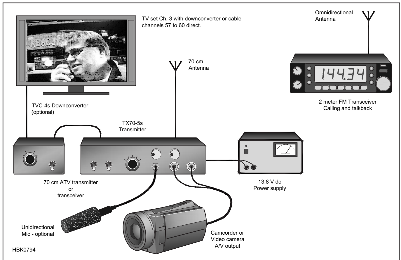
Fig 9 — Block diagram of a basic 70 cm AM ATV station with an optional downconverter. A TV set can be used without a downconverter, but it's better to have one for weak signal DX and if the video carrier frequency is more than 1 MHz from the cable channel frequency. If receiving an AM or DTV crossband repeater output on 33 or 23 cm, the downconverter would be connected to its own antenna and not through the TR relay in the transmitter. This makes it possible to see your own video coming back.
