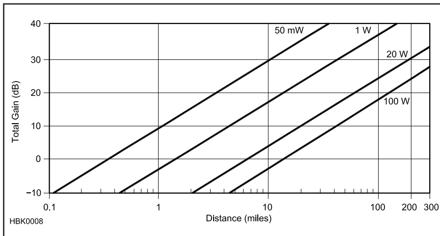
Fig 7 — This graph shows the possible line-of-sight distances for P5 (snow free) video reception for various analog AM ATV transmitter levels in the 70 cm band. Power levels shown are in PEP. The Total Gain is calculated by adding the antenna gain (dBd) for both the receive and transmit antennas and then subtracting the feed line loss (in dB) at both ends. For other bands: 33 cm, subtract 6 dB; 23 cm, subtract 9 dB; and 13 cm, subtract 15 dB. For FM ATV (4 MHz deviation, 5.5 MHz sound), add 12 dB. For ATSC 8-VSB digital TV, the sudden loss of picture “cliff effect” distance is found by adding 26 dB. If the noise figure of the first stage in the downconverter is greater than 2 dB, subtract for each dB over 2. See the example in Table 1.
