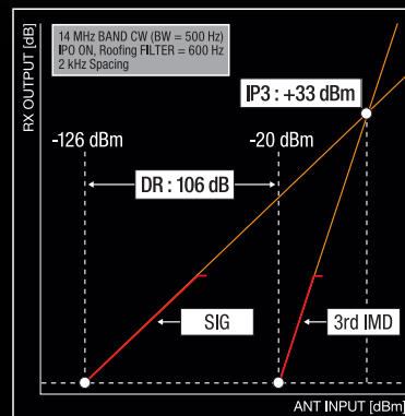
3rd Order Dynamic Range / IP3 (2kHz Spacing)
