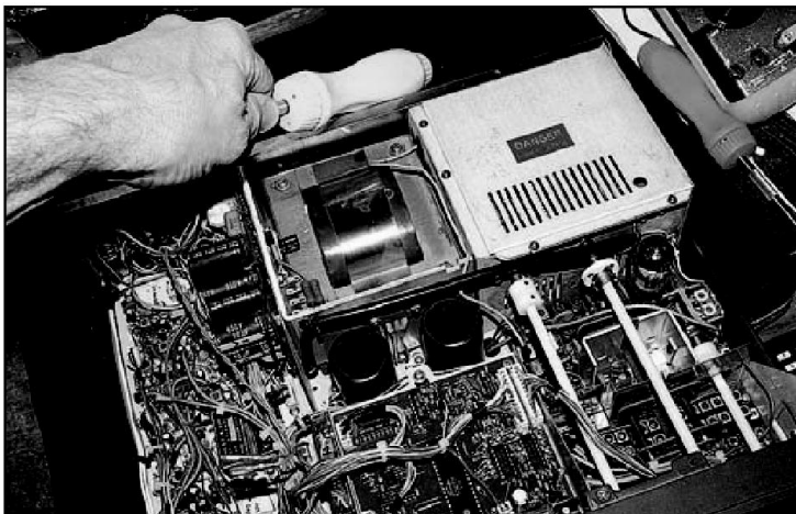
Figure 2 — Only hit the chassis hard enough to get the bounce effect (see text) on the scope pattern. In all testing use good common sense.
