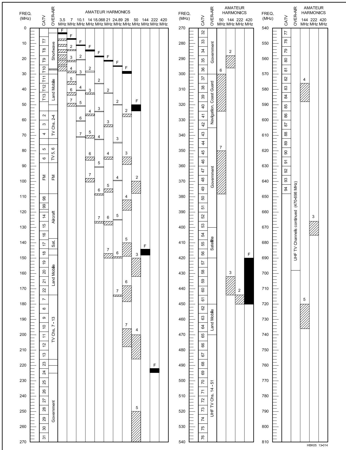
This chart shows CATV and broadcast channels used in the United States and their relationship to the harmonics of MF, HF, VHF and UHF amateur bands. Over-the-air UHF TV channels 52-69 (698-890 MHz) have been reallocated to other services. (F denotes a fundamental frequency for amateur signals.)
