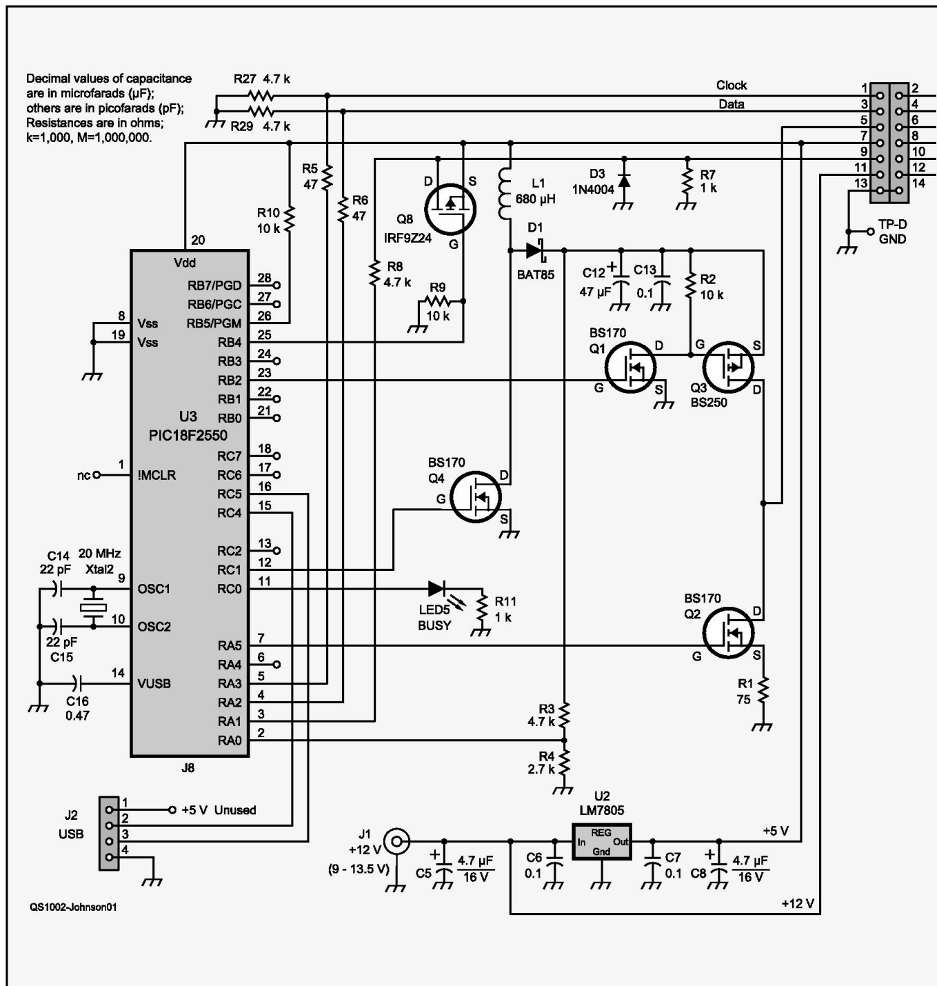
Figure 1 — Schematic diagram of the USB interface portion of the PIC-EL. Although the display subassembly is functionally equivalent to the version in May 2007 QST, there are a few differences in detail.
