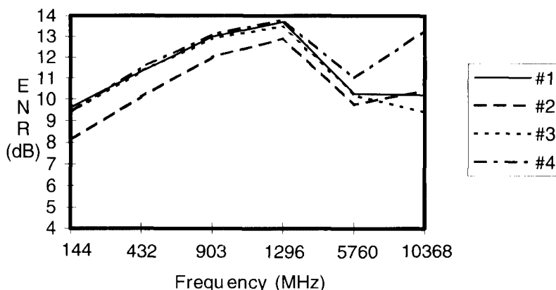
Fig 11—ENR of the PC-board noise sources (Fig 10).
