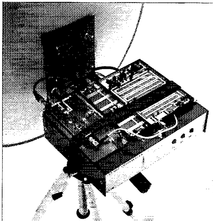
Fig 2—A complete 5760-MHz station and 24-inch dish antenna, less IF transceiver and 12-V power supply, mounts on an inexpensive camera tripod and is ready to go anywhere!
