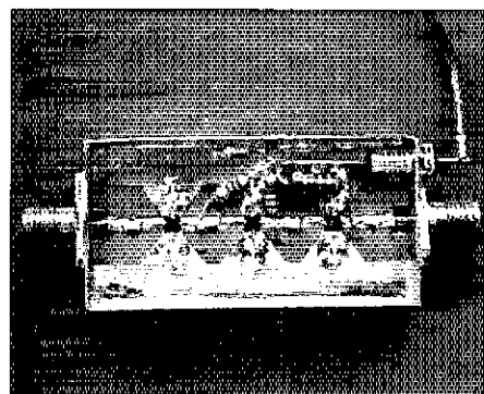
Fig 3—This simple utility amplifier, suitable for 903, 1296, 2304, 3456 and 5760-MHz transmitting and receiving use, consists of three MMICs, three ordinary resistors and five chip capacitors.
