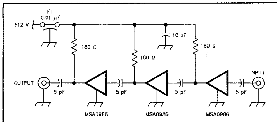
Fig 4—Schematic of the utility amplifier. Chip capacitors and MMICs are available in small quantities from Down East Microwave, Microwave Components of Michigan, and several other sources.
