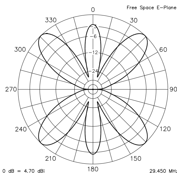
Fig 19—Free-space E-Plane radiation pattern for a 100-foot dipole at three times its full-wave resonant frequency of 29.45 MHz. The pattern has returned to six lobes, with a peak gain of 4.70 dBi.
