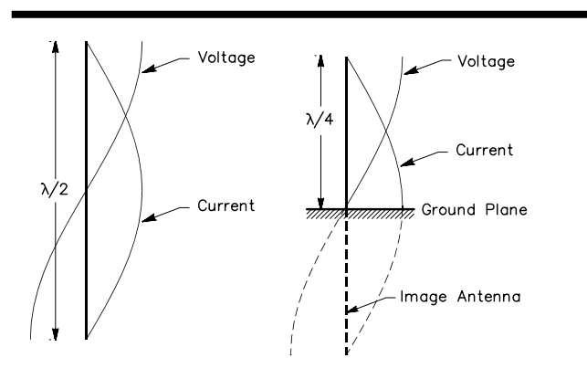
Fig 22 —The \lambda/2 dipole antenna and its \lambda/4 ground-plane counterpart. The “missing” quarter wavelength is supplied as an image in “perfect” (that is, high-conductivity) ground.
