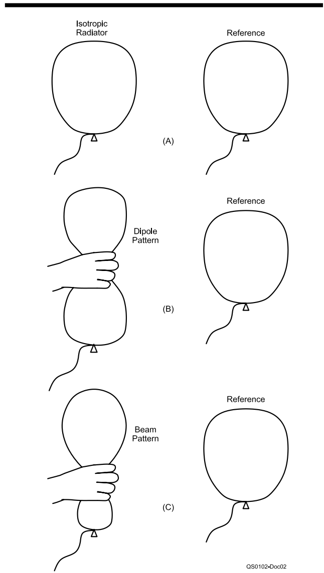
Fig 13—Demonstrating antenna pattern gain with balloons. Take a balloon, blow it up so that it is roughly circular in shape and then declare that this is a radiation pattern from an isotropic radiator. Next, blow up another balloon to the same size and shape and tell the audience that this will be the "reference" antenna (A). Then, squeeze the first balloon in the middle to form a sort of figure-8 shape and declare that this is a dipole and compare the maximum size to that of the reference "antenna" (B). The dipole can be seen to have some "gain" over the reference isotropic. Next, squeeze the end of the first balloon to come up with a sausage-like shape to demonstrate the sort of pattern a beam antenna creates (C).
