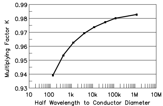
Fig 8—Effect of antenna diameter on length for half-wavelength resonance, shown as a multiplying factor, K, to be applied to the free-space, half-wavelength.
