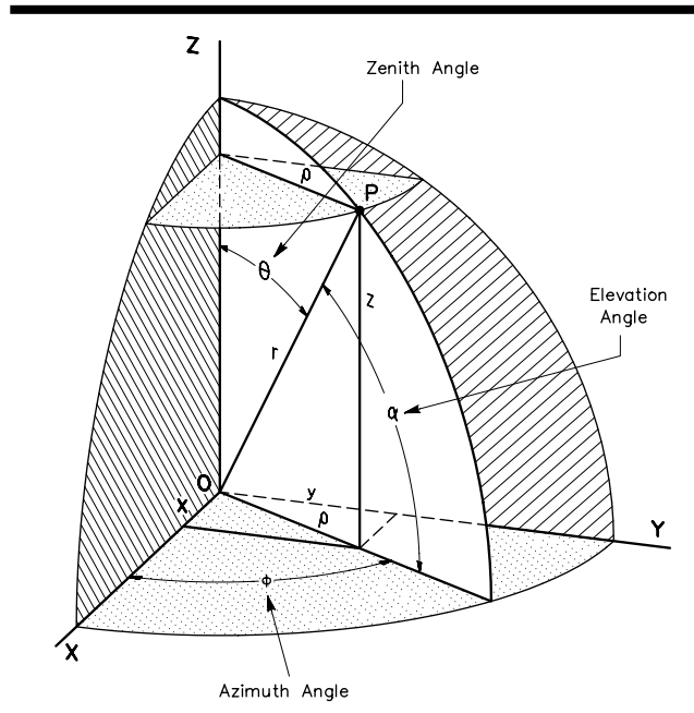
Fig 21 —Diagram showing polar representation of a point P lying on an imaginary sphere surrounding a point-source antenna. The various angles associated with this coordinate system are shown referenced to the x, y and z-axes.
