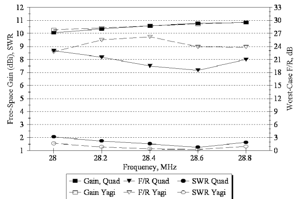
10-M Optimized Monoband Quad vs Yagi 5-Ele. Quad/5-Ele. Yagi -- 26' Booms
