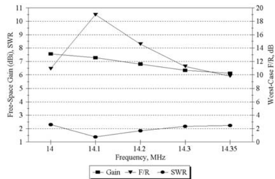
Fig 17 —Computed performance of the pentaband two-element quad on 20 meters. With the simple direct-feed system, the SWR rises to about 2.3:1 at the low end of the band. A gamma match can bring the SWR down to 1:1 at 14.1 MHz, if desired.
