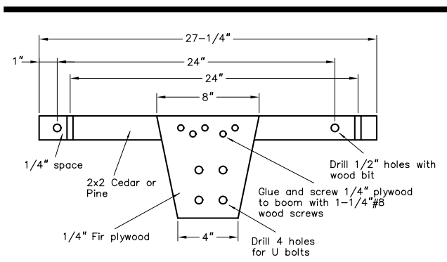
Fig 18—Dimensions for the boom-to-mast bracket for VE7CA's portable two-element 6-meter quad.
