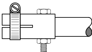
Fig 8 —The joint between two sections of \frac{5}{8} -inch tubing is made from a \frac{1}{2} -inch copper pipe coupling, bolted to one section and hose clamped to the other.
