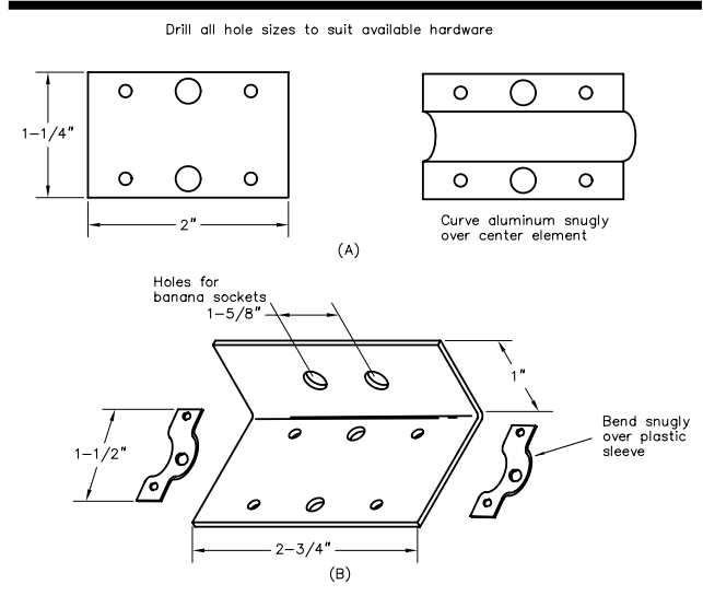
Fig 26 —At A, details for the reflector and director element-to-boom brackets, made of 1/16 -inch plate aluminum. At B, details for the driven-element bracket. These are screwed to the square boom.
