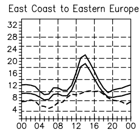
Fig 27—Propagation prediction chart for East Coast of US to Europe. This appeared in December 1994 QST, where an average 2800-MHz (10.7-cm) solar flux of 83 was assumed for the mid-December to mid-January period. On 10% of these days, the highest frequency propagated was predicted at least as high as the uppermost curve (the Highest Possible Frequency, or HPF, approximately 21 MHz), and for 50% of the days as high as the middle curve, the MUF. The broken lines show the Lowest Usable Frequency (LUF) for a 1500-W CW transmitter.
