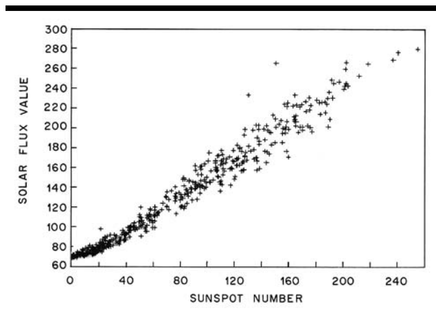
Fig 16 —Scatter diagram or X-Y plot of monthly mean sunspot numbers and monthly mean 2800MHz solar flux values. Data values are from February 1947 through February 1987. Each “+” mark represents the intersection of data for a given month. If the correlation between sunspot number and flux values were consistent, all the marks would align to form a smooth curve.
