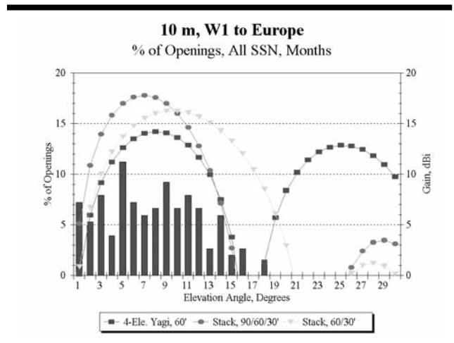
Fig 33—10-meter graph of the percentage of all openings versus elevation angles, together with overlay of elevation patterns over flat ground for three 10-meter antenna systems. Stacked antennas have wider “footprints” in elevation angle coverage for this example from New England to Europe.
