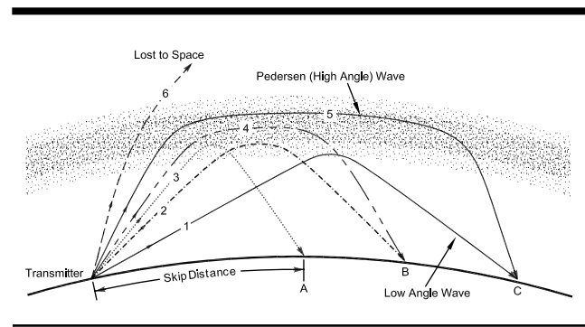
Fig 24 —Very simplified smooth-Earth/ionosphere diagram showing how the ground range from transmitter to receiver can vary as the elevation angle is gradually raised. The Pedersen wave, launched at a relatively high angle, has the same ground range as the low-angle wave #1, but is weaker because it travels for a long distance in the ionosphere.
