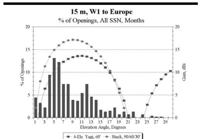
Fig 34—15-meter graph of the percentage of all openings versus elevation angles, together with overlay of elevation patterns over flat ground for two 15-meter antenna systems. Like 10 meters, 15-meter stacked antennas have wider footprints in elevation angle coverage for this example from New England to Europe.
