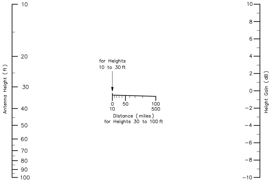
Fig 12—Nomogram for determining antenna-height gain.
