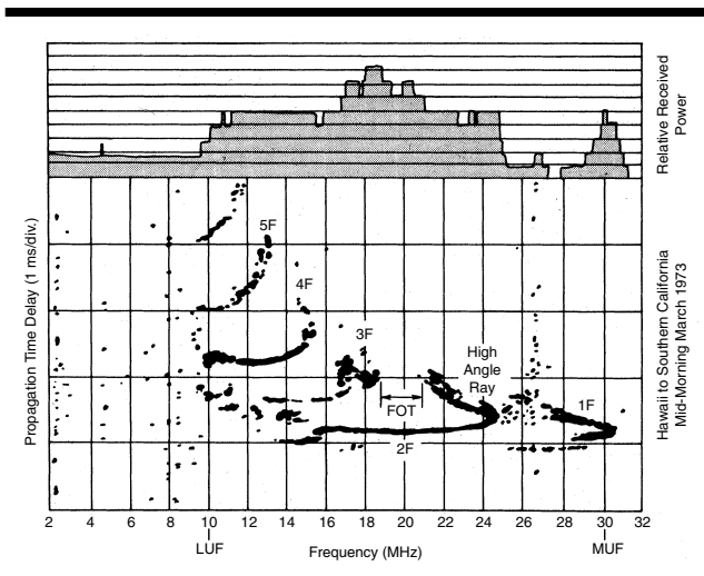
Fig 23 —HF oblique-sounder ionogram. This is a typical chirpsounder measurement on a 2500-mile path from Hawaii to southern California during midmorning in March at a medium level of solar activity. Six possible modes (hops) are shown. The “FOT” is the frequency of optimum traffic, considered most reliable for this path/time.
