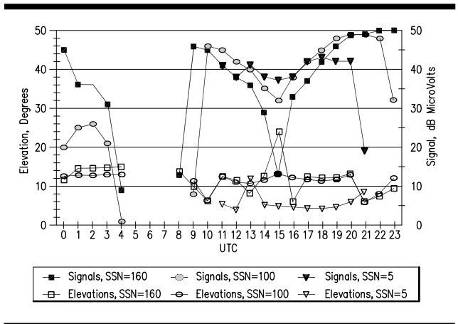
Fig 32—October 20-meter signals and elevation angles for the full range of solar activity, from W1 to England. The elevation angle does not closely follow the level of solar activity. What is important in designing a station capable of covering all levels of solar activity is to have flexibility in antenna elevation pattern response — to cover a wide range of possible angles.
