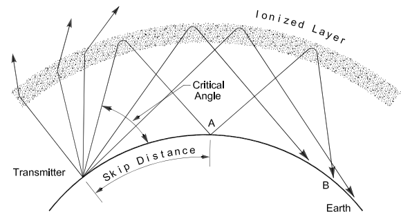
Fig 25—Behavior of waves encountering a simple curved ionospheric layer over a curved Earth. Rays entering the ionized region at angles above the critical angle are not bent enough to be returned to Earth, and are lost to space. Waves entering at angles below the critical angle reach the Earth at increasingly greater distances as the launch angle approaches the horizontal. The maximum distance that may normally be covered in a single hop is 4000 km. Greater distances are covered with multiple hops.
