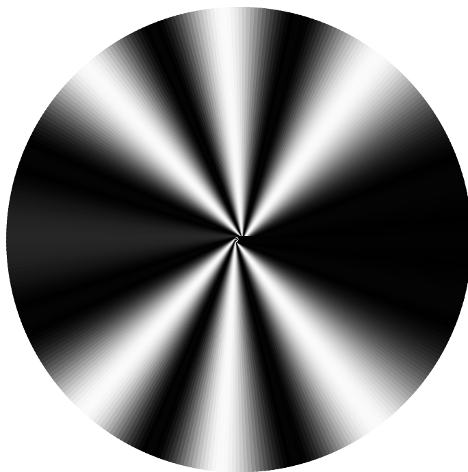
(e) Two sources - interference pattern
