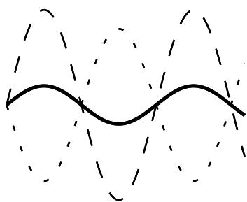
(b) Out of phase - cancellation
