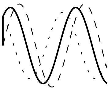
(c) 120 degree phase difference
