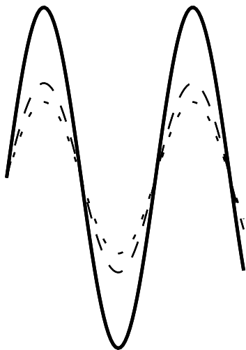
(a) In phase - addition
