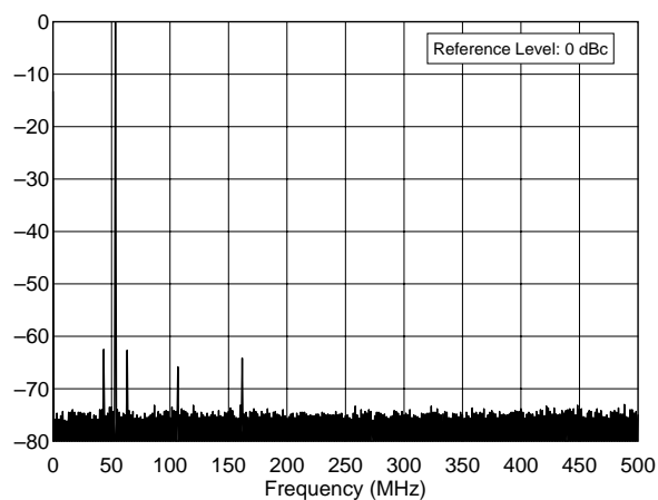
ICOM IC-756 Pro II, s/n 01164 50.0 MHz Band, Spectral Purity, 100 W F:\SHARED\PROD_REV\TESTS\IC756P2\756P2S6M.TXT
