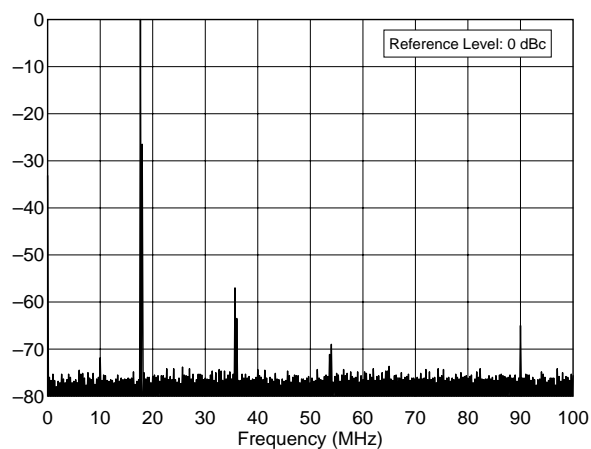
ICOM IC-756 Pro II, s/n 01164 18.1 MHz Band, Spectral Purity, 100 W F:\SHARED\PROD_REV\TESTS\IC756P2\756P2S17.TXT
