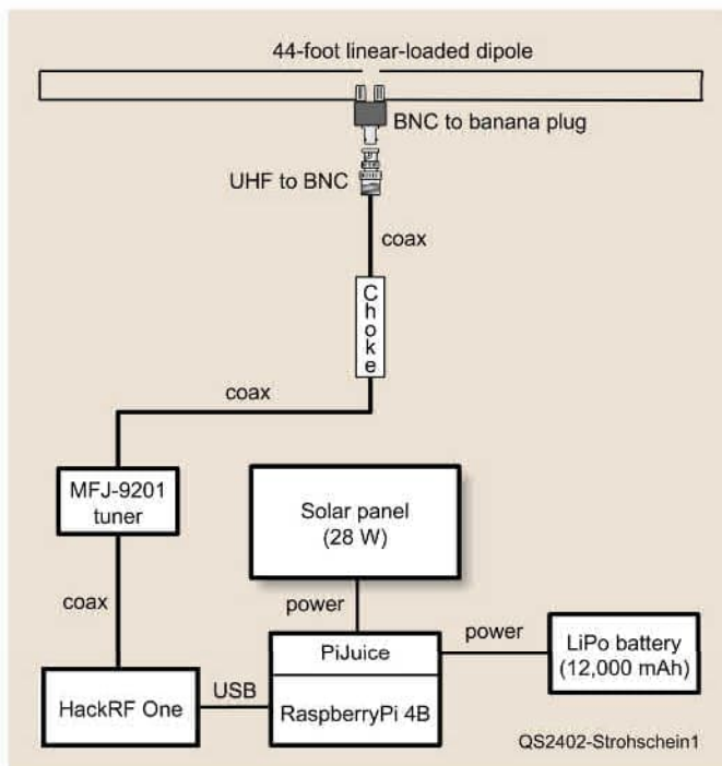
Figure 1 — A diagram of PASCOR.
