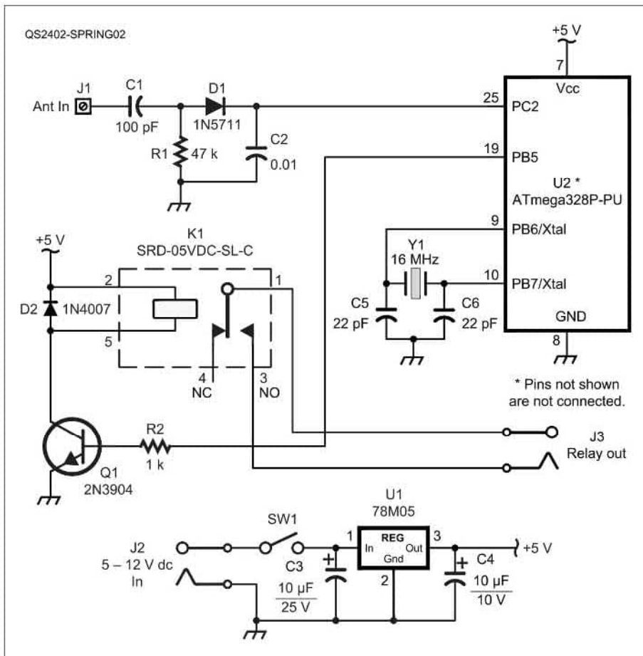
Figure 2 — The Arduino-based RF sensing schematic.
