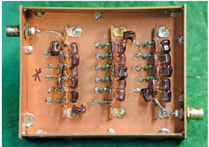
Figure 1 — The receive-only filter.
