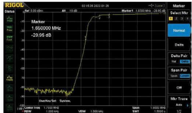
Figure 7 — Response of the transmit filter.
