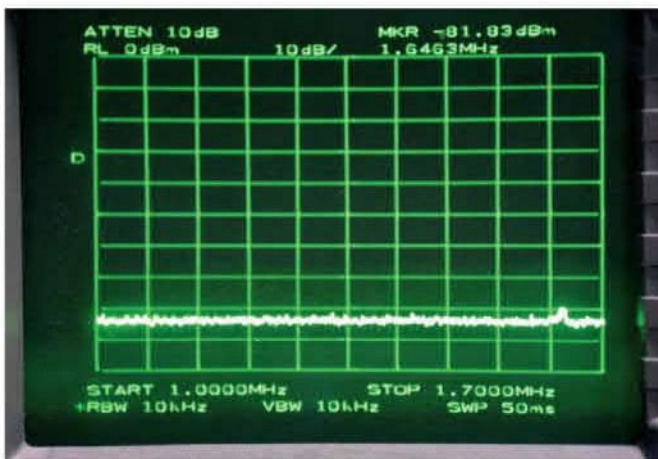
Figure 5 — AM band signals through the receive filter.
