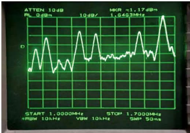
Figure 4 — AM band signals without filter.
