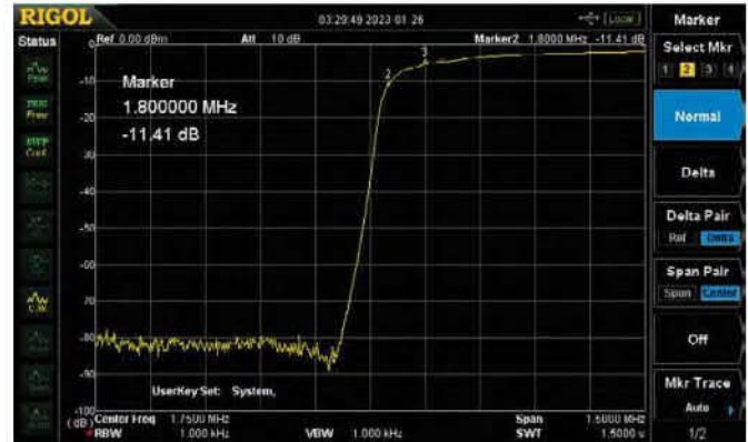
Figure 6 — The measured response of a 13-pair receive-only filter. Marker 1 at 1650 kHz is buried in the noise. Marker 2 shows the bottom end, and marker 3 shows the center of the 160-meter band. The loss in the 160-meter band doesn't affect reception, as both signal and noise will be attenuated.
