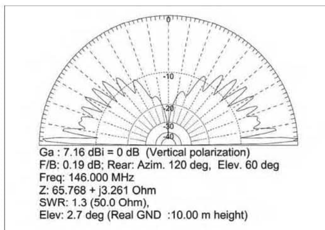
Figure 2 — The modified Astroplane's radiation pattern.
