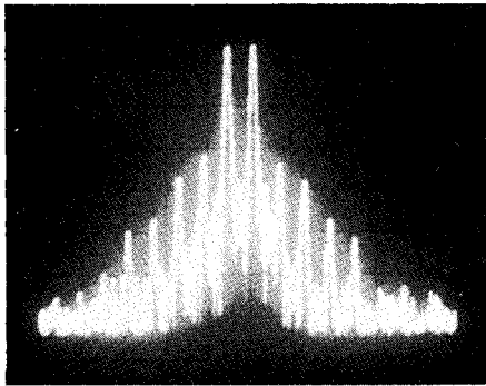
Fig 4—Spectral display of the FT-736R during 220.2-MHz, two-tone intermodulation distortion (IMD) testing. Third-order products are approximately 32 dB below PEP output, and fifth-order products are approximately 37 dB down. Vertical divisions are each 10 dB; horizontal divisions are each 2 kHz. The transceiver was being operated at 22 W PEP output.
