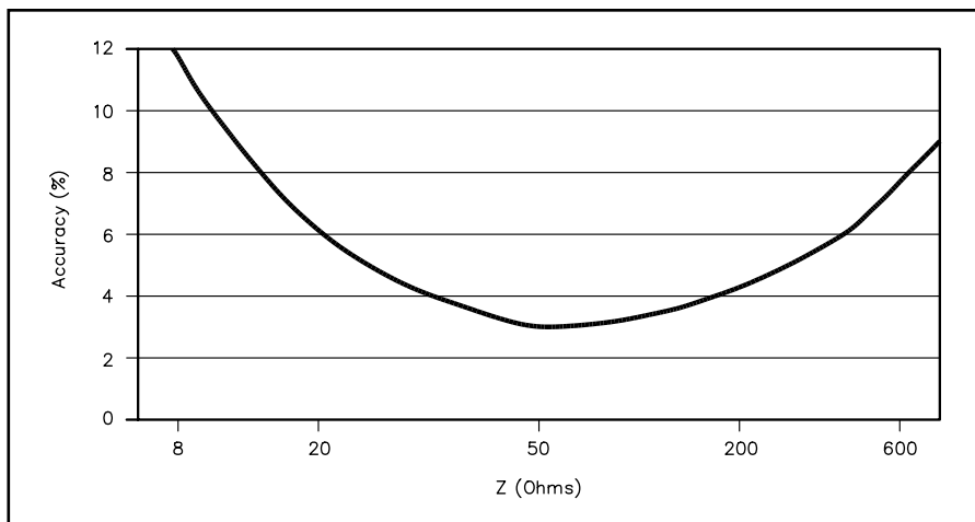
Figure 4—Here's a plot of impedance accuracy for the Autek RF5, as provided by the manufacturer. The plot shows the accuracy you can expect at 50 MHz with negligible lead length and an impedance below 100 Ω. At higher impedances, the meter's output capacitance makes the impedance appear smaller.
