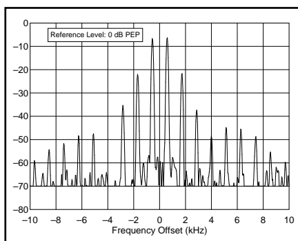
Figure 2— Worst-case spectral display of the IC-746 transmitter during two-tone intermodulation distortion (IMD) testing on VHF. The worst-case third-order product is approximately 22 dB below PEP output, and the worst-case fifth-order product is approximately 36 dB down. The transmitter was being operated at 100 W output at 144.200 MHz.
