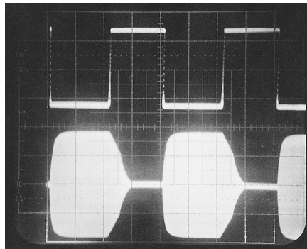
Figure 6—Keying waveform for the Ten-Tec 1340 showing the first two dits. The equivalent keying speed is 60 WPM. The upper trace is the actual key closure; the lower trace is the RF envelope. Horizontal divisions are 10 ms. The transmitter is being operated at 4 W output at 7.020 MHz.
