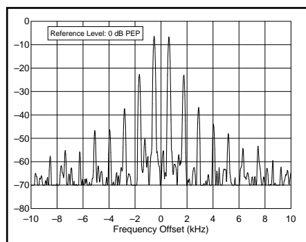
Figure 1—Worst-case spectral display of the IC-746 transmitter during two-tone intermodulation distortion (IMD) testing on HF. The worst-case third-order product is approximately 23 db below PEP output, and the worst-case fifth-order product is approximately 37 dB down. The transmitter was being operated at 100 W output at 28.350 MHz.
