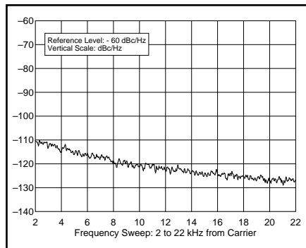
Figure 5—Worst-case tested spectral display of the IC-746 transmitter output during composite-noise testing on VHF. Power output is 100 W at 144.020 MHz. The carrier, off the left edge of the plot, is not shown. The plot shows composite transmitted noise 2 to 22 kHz from the carrier.
