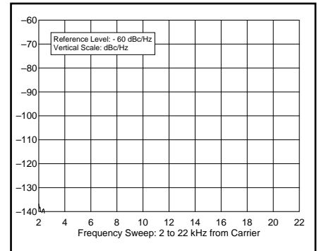
Figure 7—Spectral display of the Ten-Tec 1340 transmitter output during composite-noise testing. The carrier, off the left edge of the plot, is not shown. This plot shows composite transmitted noise 2 to 22 kHz from the carrier. Note that the only noise on this plot is the two small "pips" near the left edge of the graph. This level of composite noise is lower than any transmitter that has been previously tested in the ARRL Lab. The transceiver is being operated at 4 W PEP at 7.020 MHz.
