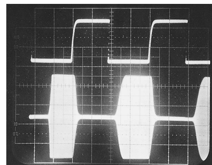
Figure 3— CW keying waveform for the IC-746 showing the first two dits in semi-break-in mode. The equivalent keying speed is 60 WPM. The upper trace is the actual key closure; the lower trace is the RF envelope. Horizontal divisions are 10 ms. The transmitter is being operated at 100 W output at 14.2 MHz. Note that the first dit is slightly shortened. Full-break-in operation (QSK) results in a nearly identical shape for the first dit, with slight shortening indicated on subsequent dits.
