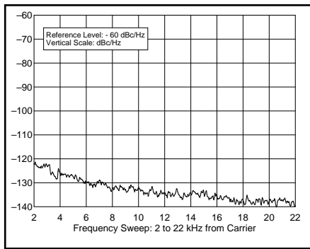
Figure 4—Worst-case tested spectral display of the IC-746 transmitter output during composite-noise testing on HF. Power output is 100 W at 14.020 MHz. The carrier, off the left edge of the plot, is not shown. The plot shows composite transmitted noise 2 to 22 kHz from the carrier.
