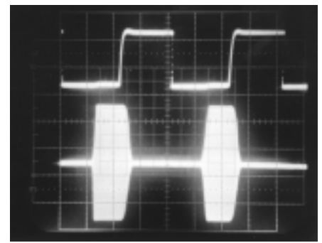
Figure 3—CW keying waveform for the IC-756PRO showing the first two dits in full-break-in (QSK) mode. The equivalent keying speed is 60 WPM. The upper trace is the actual key closure; the lower trace is the RF envelope. Horizontal divisions are 10 ms. The transceiver was being operated at 100 W output at 14.2 MHz. Note that both dits are somewhat shortened. Only the first dit is shortened in semi-break-in mode.
