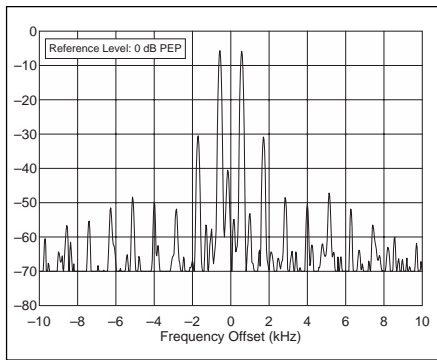
Figure 1—Worst-case spectral display of the IC-756PRO transmitter during two-tone intermodulation distortion (IMD) testing on HF. The worst-case third-order product is approximately 31 dB below PEP output, and the worst-case fifth-order is approximately 49 dB down. The transmitter was being operated at 100 W output at 28.350 MHz.
