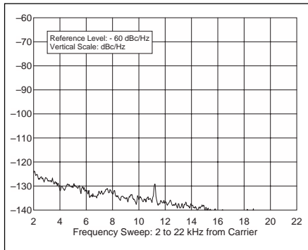
Figure 4—Worst-case tested HF spectral display of the IC-756PRO transmitter output during composite-noise testing at 14 MHz. Power output is 100 W. The carrier, off the left edge of the plot, is not shown. This plot shows composite transmitted noise 2 to 22 kHz from the carrier.
