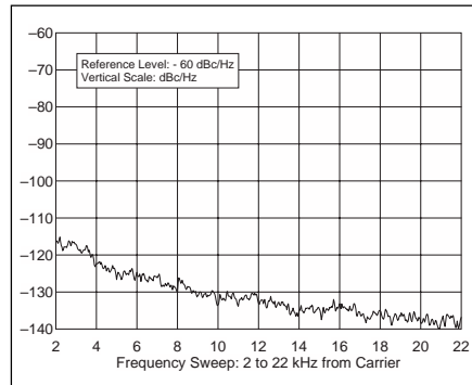
Figure 5—Spectral display of the IC-756PRO transmitter output during composite-noise testing at 50.2 MHz. Power output is 100 W. The carrier, off the left edge of the plot, is not shown. This plot shows composite transmitted noise 2 to 22 kHz from the carrier.
