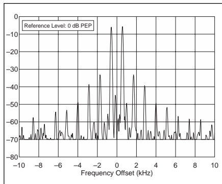
Figure 2—Spectral display of the IC-756PRO transmitter during two-tone intermodulation distortion (IMD) testing on 6 meters. The third-order product is approximately 34 dB below PEP output, and the fifth-order is approximately 40 dB down. The transmitter was being operated at 100 W output at 50.200 MHz.
