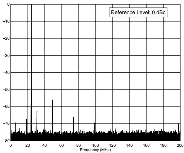
IC-706 / SN: 02104 28.0 MHz Band, Spectral Purity, 100 W F:\SHARED\PROD_REVTESTS\IC706S10.TXT
