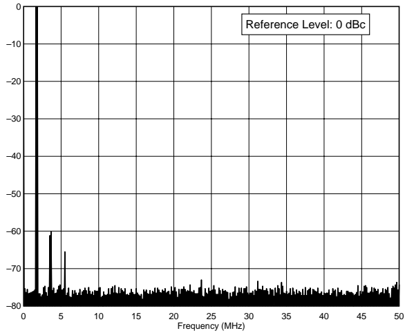
IC-706 / SN: 02104 1.8 MHz Band, Spectral Purity, 100 W F:\SHARED\PROD_REV\TESTS\IC706SLO.TXT
