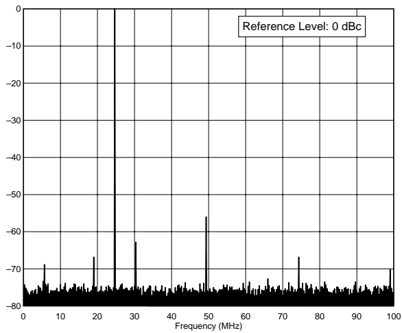
IC-706 / SN: 02104 24.9 MHz Band, Spectral Purity, 100 W F:\SHARED\PROD_REVTESTS\IC706S12.TXT
