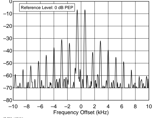
IC-706 / 02104 14.250 MHz, Transmit IMD, 100 W F:\SHARED\PROD_REV\TESTS\IC706\IC706I20.TXT
