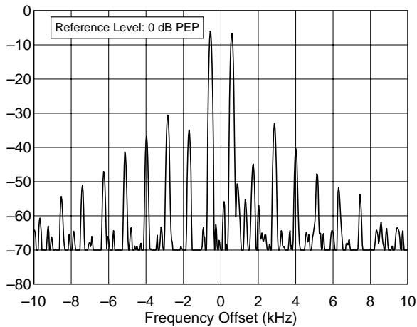
IC-706 / 02104 7.250 MHz, Transmit IMD, 100 W F:\SHARED\PROD_REV\TESTS\IC706\IC706I40.TXT
