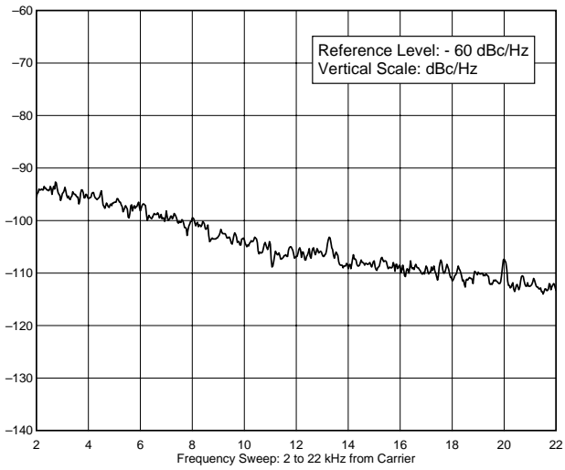
IC-706 Composite Noise Frequency = 144.02 MHz
