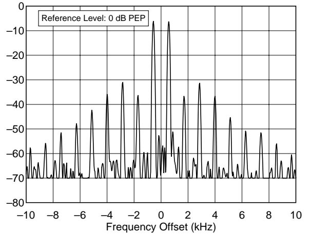
IC-706 / 02104 10.120 MHz, Transmit IMD, 100 W F:\SHARED\PROD_REV\TESTS\IC706\IC706I30.TXT
