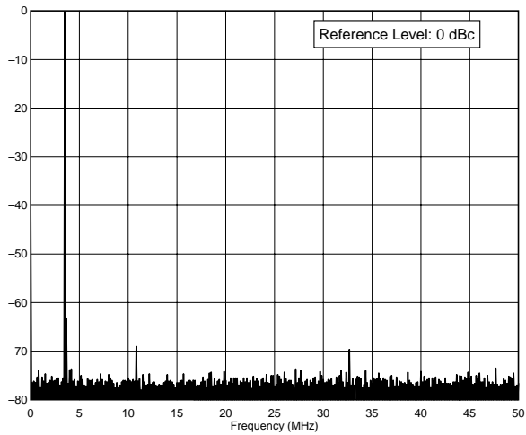
IC-706 / SN: 02104 3.5 MHz Band, Spectral Purity, 100 W F:\SHARED\PROD_REV\TESTS\IC706S80.TXT
