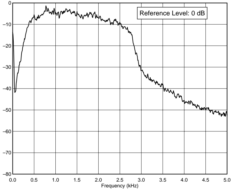
IC-706 14 MHz Rcv Bandpass USB Normal Filter P:\TESTS\IC706\IC706BP1.TXT
