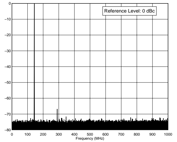
IC-706 / SN: 02104 144.0 MHz Band, Spectral Purity, 10 W F:\SHARED\PROD_REVTESTS\IC706S2M.TXT
