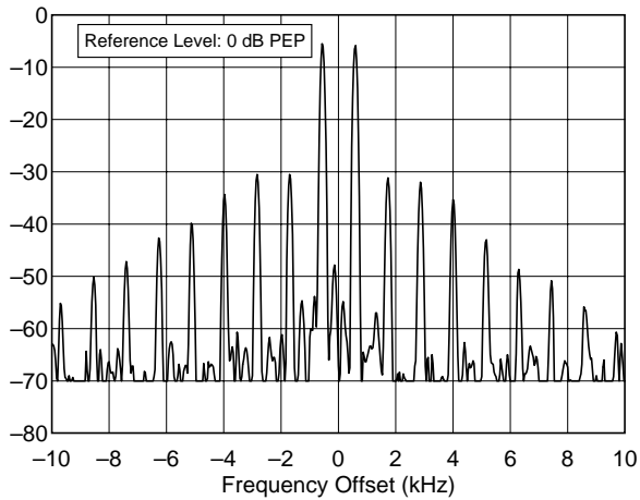
IC-706 / 02104 24.950 MHz, Transmit IMD, 100 W F:\SHARED\PROD_REV\TESTS\IC706\IC706i12.TXT
