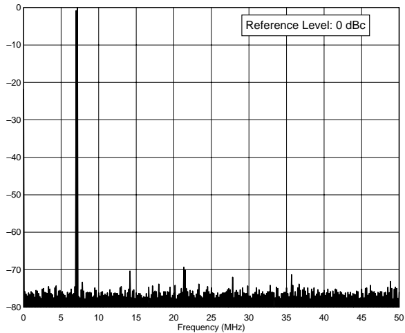
IC-706 / SN: 02104 7.0 MHz Band, Spectral Purity, 100 W F:\SHARED\PROD_REV\TESTS\IC706S40.TXT
