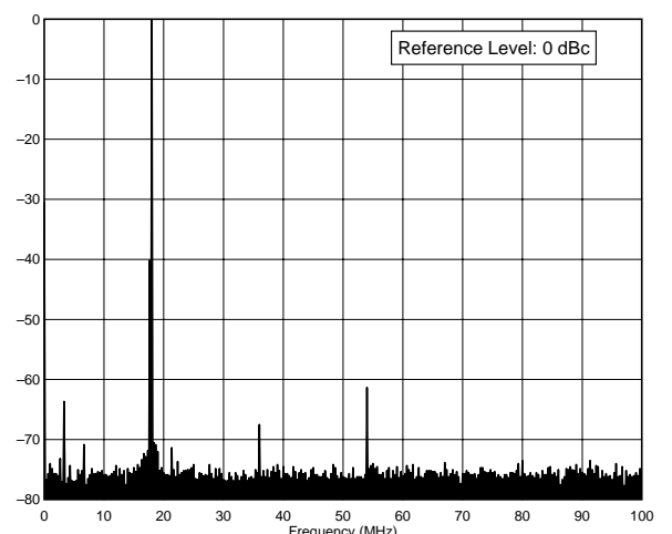
IC-706 / SN: 02104 18.1 MHz Band, Spectral Purity, 100 W F:\SHARED\PROD_REV\TESTS\IC706S17.TXT
