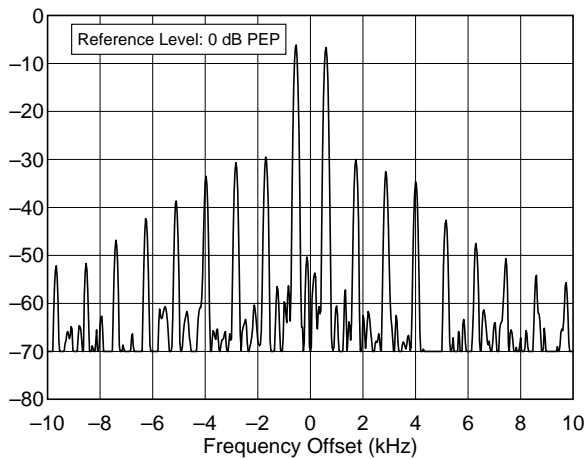
IC-706 / 02104 28.350 MHz, Transmit IMD, 100 W F:\SHARED\PROD_REV\TESTS\IC706\IC706i10.TXT
