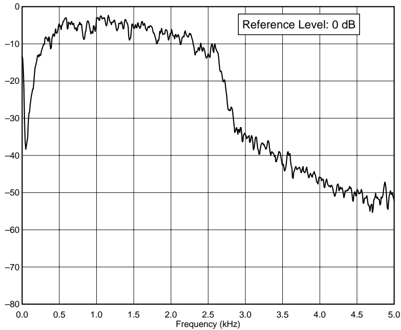
IC-706 14 MHz Rcv Bandpass CW Wide Filter P:\TESTS\IC706\IC706BP2.TXT
