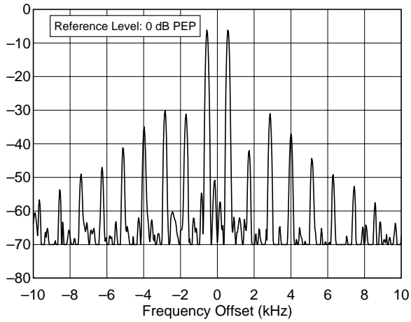
IC-706 / 02104 21.250 MHz, Transmit IMD, 100 W F:\SHARED\PROD_REV\TESTS\IC706\IC706i15.TXT
