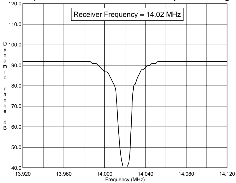
Swept Two-Tone, Third-Order IMD Dynamic Range
