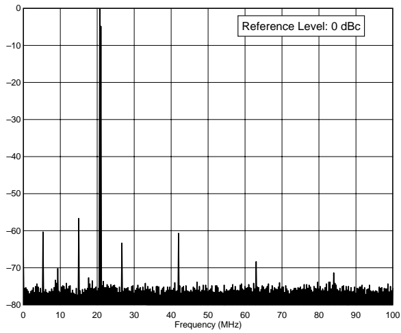
IC-706 / SN: 02104 21.0 MHz Band, Spectral Purity, 100 W F:\SHARED\PROD_REVTESTS\IC706S15.TXT
