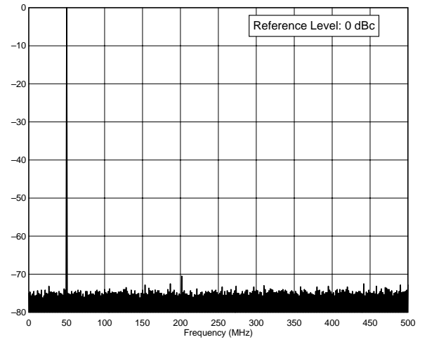
IC-706 / SN: 02104 50.0 MHz Band, Spectral Purity, 100 W F:\SHARED\PROD_REVTESTS\IC706S6M.TXT
