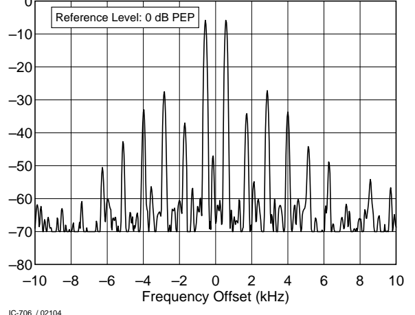
IC-706 / 02104 18.120 MHz, Transmit IMD, 100 W F:\SHARED\PROD_REV\TESTS\IC706\IC706I17.TXT
