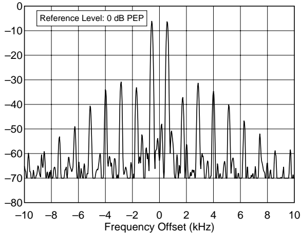
IC-706 / 02104 1.850 MHz, Transmit IMD, 100 W F:\SHARED\PROD_REV\TESTS\IC706\IC706I10.TXT
