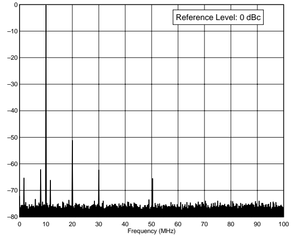
IC-706 / SN: 02104 10.1 MHz Band, Spectral Purity, 100 W F:\SHARED\PROD_REV\TESTS\IC706S30.TXT
