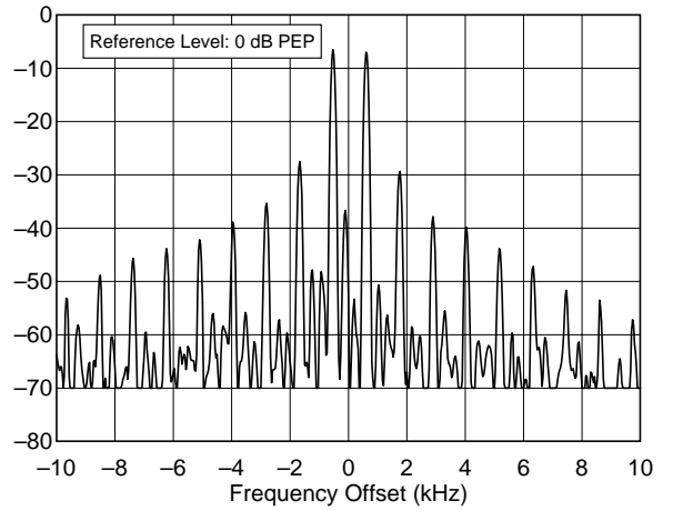
IC-706 / 02104 50.200 MHz, Transmit IMD, 82 W F:\SHARED\PROD_REV\TESTS\IC706\IC706i6M.TXT
