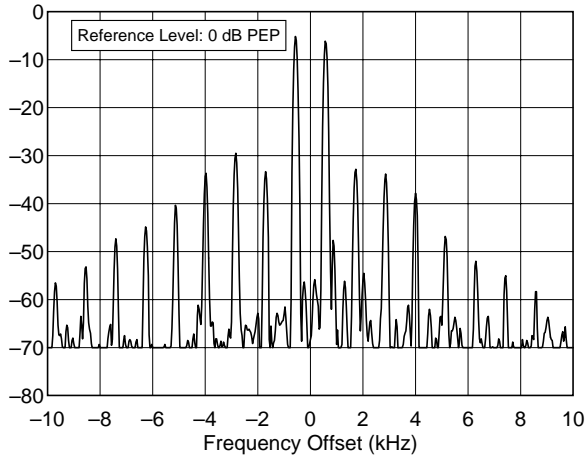
IC-706 / 02104 3.900 MHz, Transmit IMD, 100 W F:\SHARED\PROD_REV\TESTS\IC706\IC706I80.TXT
