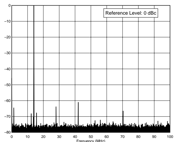
IC-706 / SN: 02104 14.0 MHz Band, Spectral Purity, 100 W F:\SHARED\PROD_REV\TESTS\IC706S20.TXT
