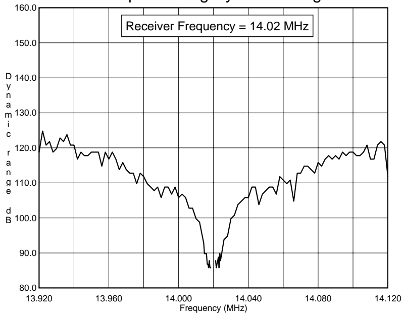
Swept Blocking Dynamic Range
