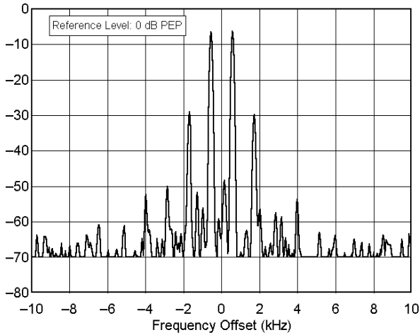
ICOM IC-706 MkII ser no 02995 1.860 MHz, Transmit IMD, 100 W F:\SHARED\PROD_REV\TESTS\IC-706\INC706100.TXT
