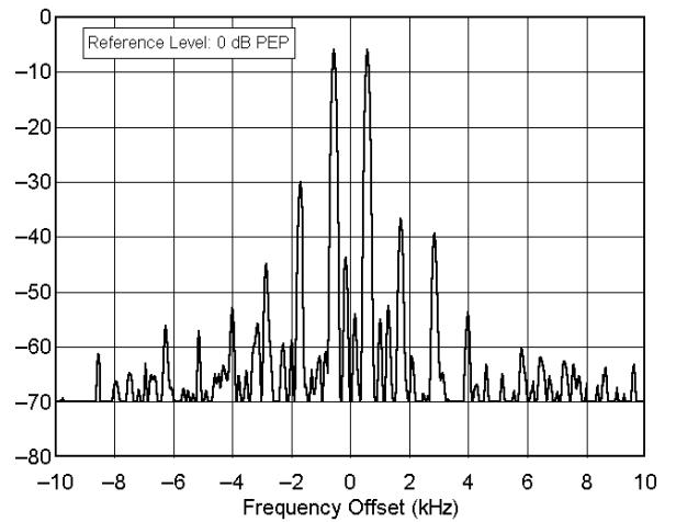
ICOM IC-706 MkII ser no 02995 50.200 MHz, Transmit IMD, 100 W F:\SHARED\PROD_REV\TESTS\IC-706\INC706I6M.TXT
