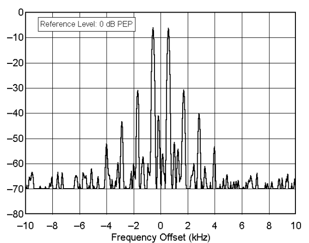
ICOM IC-706 MkII ser no 02995 18.120 MHz, Transmit IMD, 100 W F:\SHARED\PROD_REV\TESTS\IC-706\INC706117.TXT
