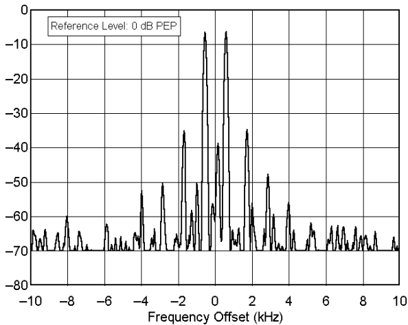
ICOM IC-706 MkII ser no 02995 7.250 MHz, Transmit IMD, 100 W F:\SHARED\PROD_REV\TESTS\IC-706\INC706140.TXT
