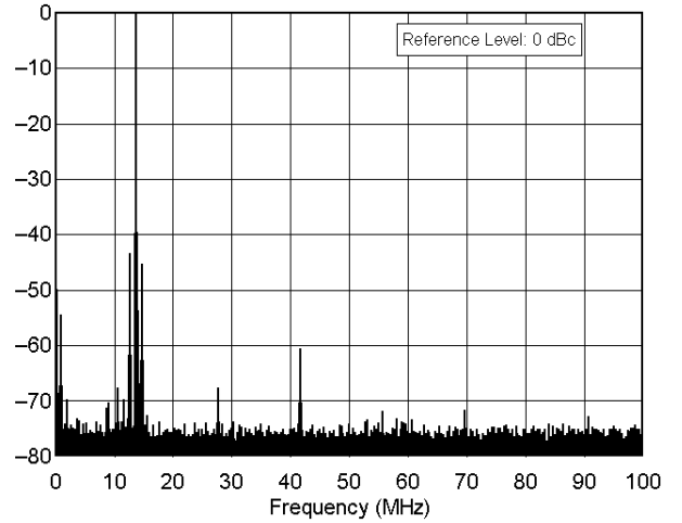
IC-706 MkII ser no 02995 14.0 MHz Band, Spectral Purity, 100 W F:\SHARED\PROD_REVTESTS\SVC-706\INC706S20.TXT
