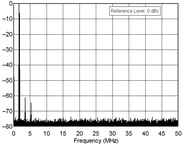
IC-706 MkII ser no 02995 1.8 MHz Band, Spectral Purity, 100 W F:\SHARED\PROD_REVTESTS\SVC-706\INC706SLO.TXT
