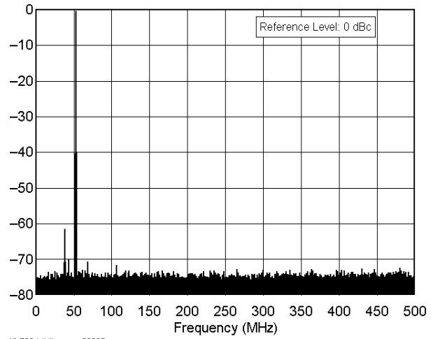
IC-706 MkII ser no 02995 50.0 MHz Band, Spectral Purity, 100 W F:\SHARED\PROD_REV\TESTS\IC-706\INC706S6M.TXT
