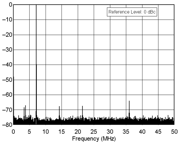
IC-706 MkII ser no 02995 7.0 MHz Band, Spectral Purity, 100 W F:\SHARED\PROD_REVTESTS\SVC-706\INC706S40.TXT
