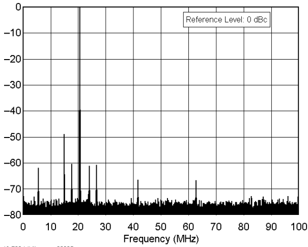
IC-706 MkII ser no 02995 21.0 MHz Band, Spectral Purity, 100 W F:\SHARED\PROD_REV\TESTS\IC-706\INC706S15.TXT
