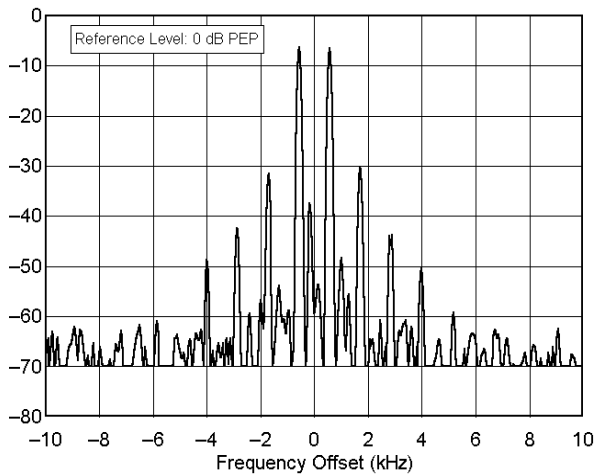
ICOM IC-706 MkII ser no 02995 21.250 MHz, Transmit IMD, 100 W F:\SHARED\PROD_REV\TESTS\IC-706\INC706I15.TXT
