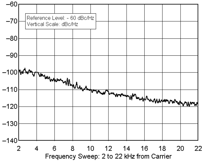
ICOM IC-706 MkII ser no 02995 14.020 MHz, Phase Noise, 100 W F:\SHARED\PROD_REV\TESTS\IC-706\IC706P20.TXT
