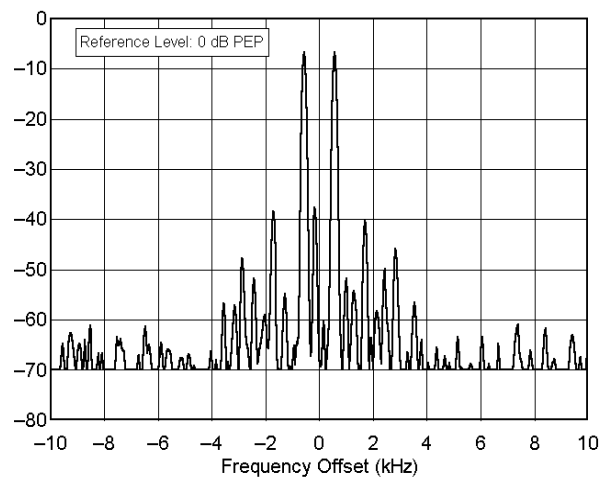
ICOM IC-706 MkII ser no 02995 14.250 MHz, Transmit IMD, 100 W F:\SHARED\PROD_REV\TESTS\IC-706\INC706200.TXT
