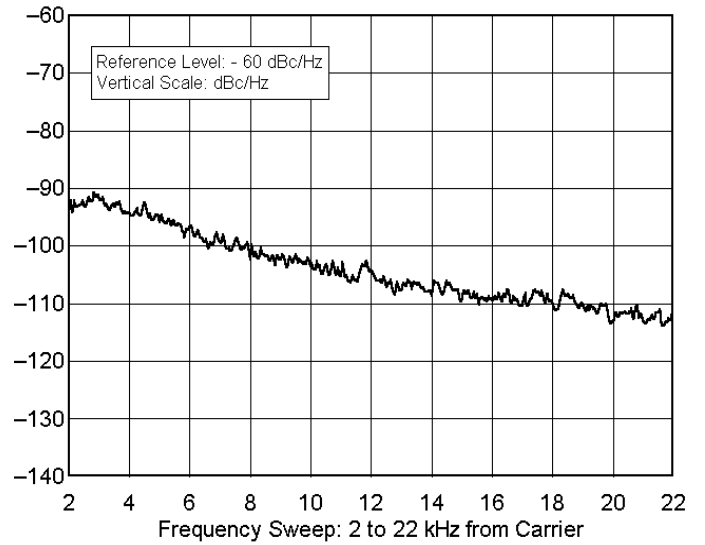
ICOM IC-706 MkII ser no 02995 144.020 MHz, Phase Noise, 20 W F:\SHARED\PROD_REV\TESTS\IC-706\IC706P2M.TXT
