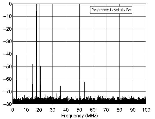
IC-706 MkII ser no 02995 18.1 MHz Band, Spectral Purity, 100 W F:\SHARED\PROD_REVTESTS\SVC-706\INC706S17.TXT
