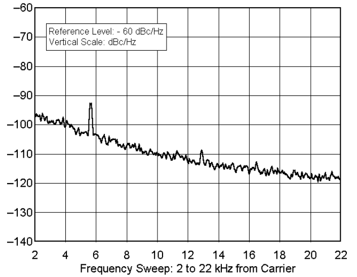
ICOM IC-706 MkII ser no 02995 50.020 MHz, Phase Noise, 100 W F:\SHARED\PROD_REV\TESTS\IC-706\IC706P6M.TXT
