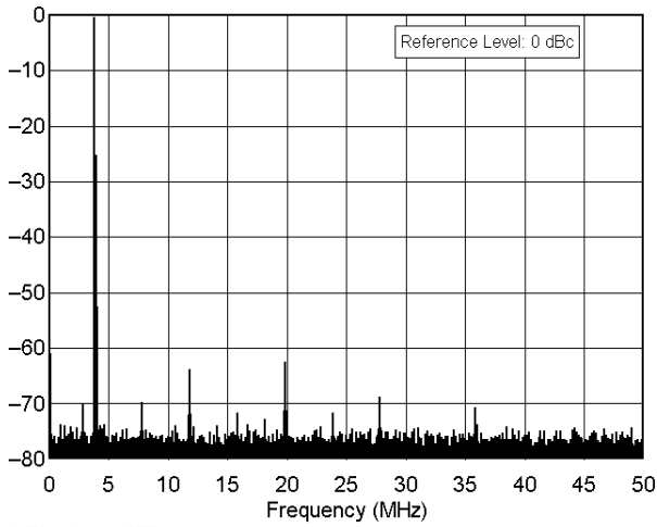
IC-706 MkII ser no 02995 3.5 MHz Band, Spectral Purity, 100 W F:\SHARED\PROD_REVTESTS\SVC-706\INC706S80.TXT
