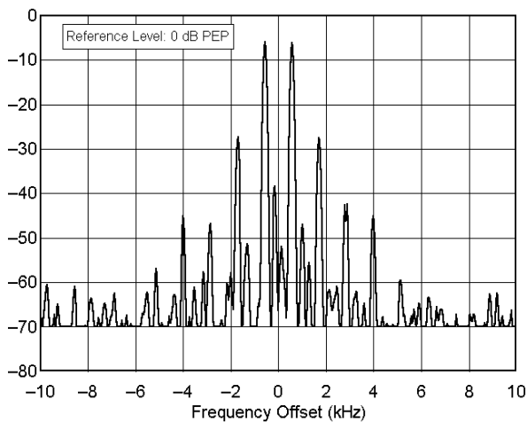
ICOM IC-706 MkII ser no 02995 24.950 MHz, Transmit IMD, 100 W F:\SHARED\PROD_REV\TESTS\IC-706\INC706I12.TXT
