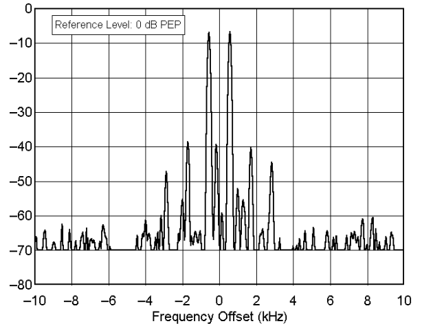
ICOM IC-706 MkII ser no 02995 10.120 MHz, Transmit IMD, 100 W F:\SHARED\PROD_REV\TESTS\IC-706\INC706130.TXT
