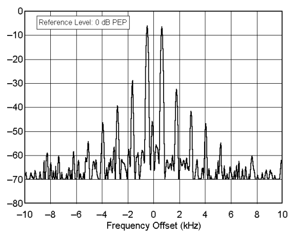
ICOM IC-706 MkII ser no 02995 144.200 MHz, Transmit IMD, 20 W F:\SHARED\PROD_REV\TESTS\IC-706\INC706I2M.TXT
