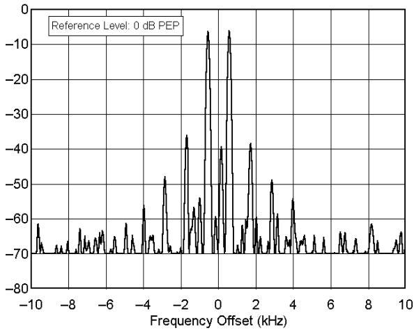
ICOM IC-706 MkII ser no 02995 3.900 MHz, Transmit IMD, 100 W F:\SHARED\PROD_REV\TESTS\IC-706\INC706180.TXT
