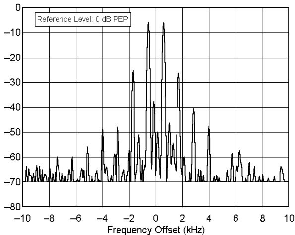
ICOM IC-706 MkII ser no 02995 28.350 MHz, Transmit IMD, 100 W F:\SHARED\PROD_REV\TESTS\IC-706\INC706I10.TXT
