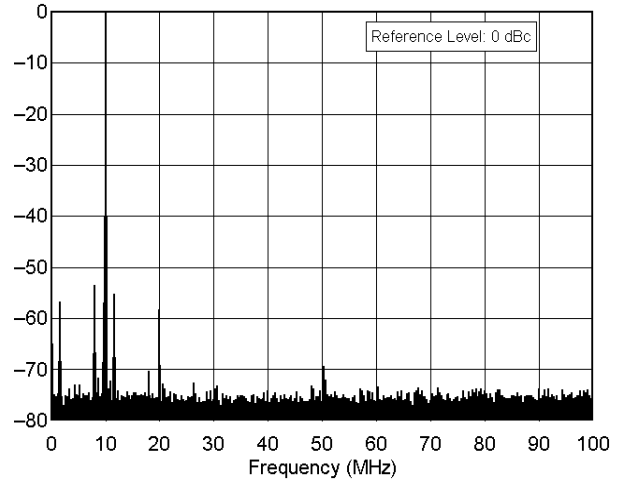
IC-706 MkII ser no 02995 10.1 MHz Band, Spectral Purity, 100 W F:\SHARED\PROD_REVTESTS\SVC-706\INC706S30.TXT
