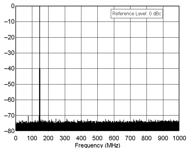
IC-706 MkII ser no 02995 144.0 MHz Band, Spectral Purity, 100 W F:\SHARED\PROD_REV\TESTS\IC-706\INC706S2M.TXT
