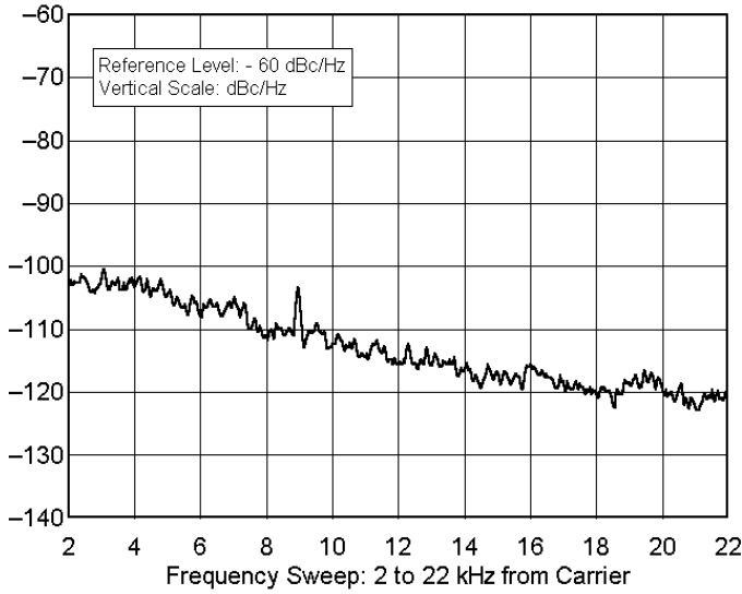
ICOM IC-706 MkII ser no 02995 3.520 MHz, Phase Noise, 100 W F:\SHARED\PROD_REV\TESTS\IC-706\IC706P80.TXT
