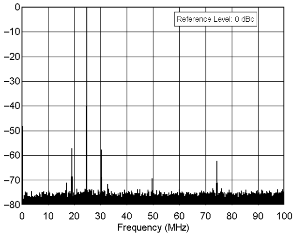
IC-706 MkII ser no 02995 24.9 MHz Band, Spectral Purity, 100 W F:\SHARED\PROD_REV\TESTS\IC-706\INC706S12.TXT
