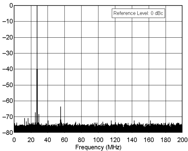
IC-706 MkII ser no 02995 28.0 MHz Band, Spectral Purity, 100 W F:\SHARED\PROD_REV\TESTS\IC-706\INC706S10.TXT
