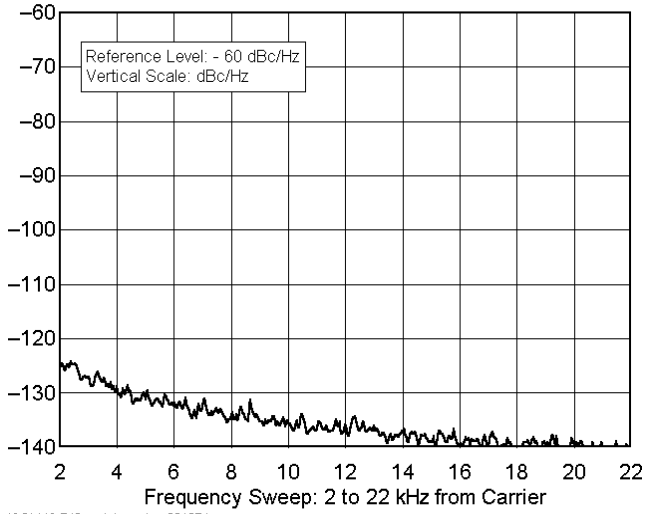
ICOM IC-746 serial number 001674 3.520 MHz, Phase Noise, 100 W F:\SHARED\PROD_REVTESTS\IC746\IC746P80.TXT
