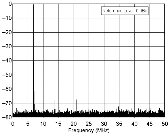
ICOM IC-746 serial number 001674 7.0 MHz Band, Spectral Purity, 100 W F:\SHARED\PROD_REV\TESTS\IC746\IC746S40.TXT
