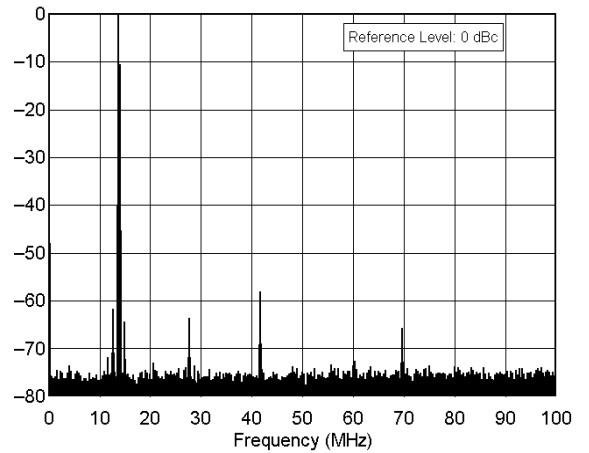
ICOM IC-746 serial number 001674 14.0 MHz Band, Spectral Purity, 100 W F:\SHARED\PROD_REV\TESTS\IC746\IC746S20.TXT
