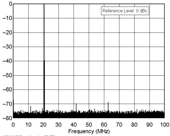
ICOM IC-746 serial number 001674 21.0 MHz Band, Spectral Purity, 100 W F:\SHARED\PROD_REV\TESTS\IC746\IC746S15.TXT
