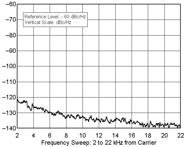
ICOM IC-746 serial number 001674 14.020 MHz, Phase Noise, 100 W F:\SHARED\PROD_REVTESTS\IC746\IC746P20.TXT
