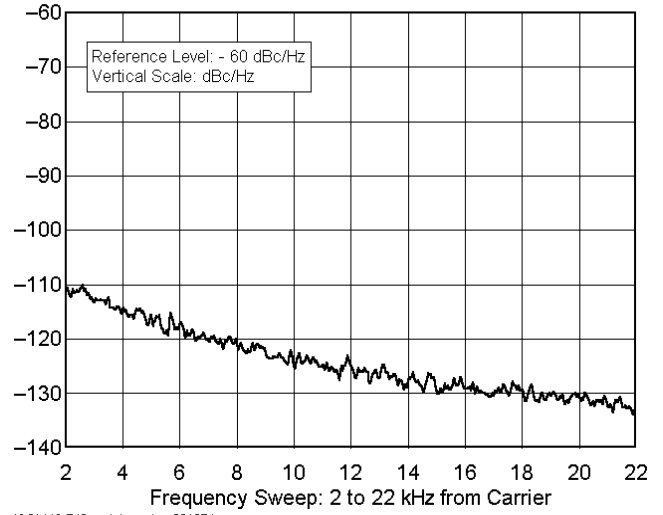
ICOM IC-746 serial number 001674 50.020 MHz, Phase Noise, 100 W F:\SHARED\PROD_REVTESTS\IC746\IC746P6M.TXT
