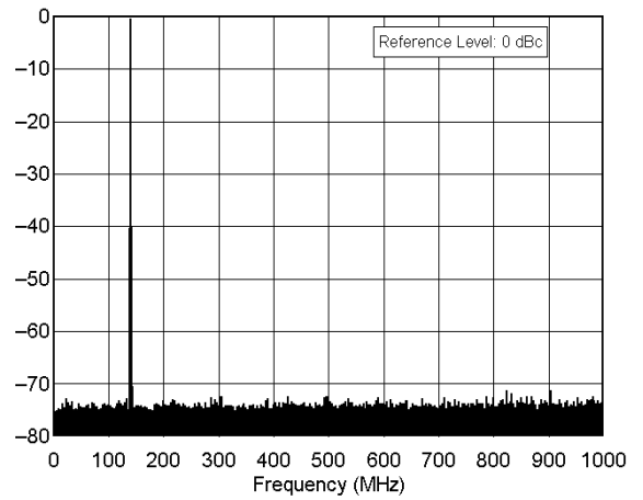
ICOM IC-746 serial number 001674 144.0 MHz Band, Spectral Purity, 100 W F:\SHARED\PROD_REV\TESTS\IC746\IC746S2M.TXT
