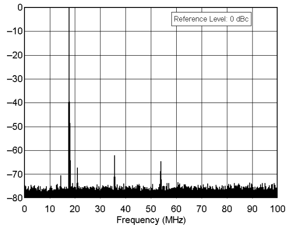
ICOM IC-746 serial number 001674 18.1 MHz Band, Spectral Purity, 100 W F:\SHARED\PROD_REV\TESTS\IC746\IC746S17.TXT
