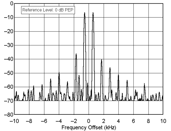
ICOM IC-746 serial number 001674 10.120 MHz, Transmit IMD, 100 W F:\SHARED\PROD_REV\TESTS\VC746\IC746120.TXT
