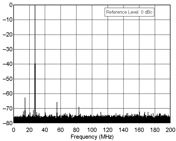
ICOM IC-746 serial number 001674 28.0 MHz Band, Spectral Purity, 100 W F:\SHARED\PROD_REV\TESTS\IC746\IC746S10.TXT
