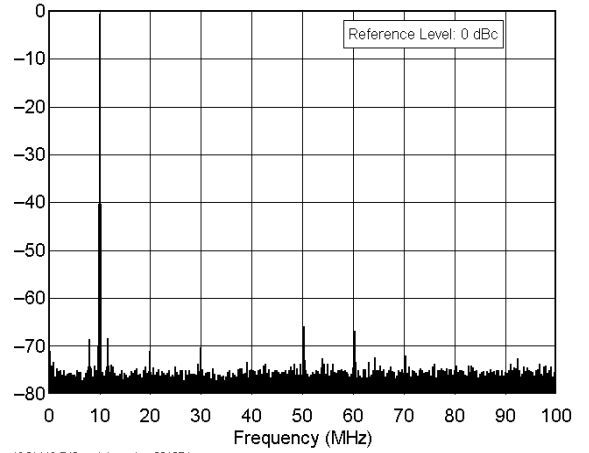
ICOM IC-746 serial number 001674 10.1 MHz Band, Spectral Purity, 100 W F:\SHARED\PROD_REV\TESTS\IC746\IC746S30.TXT
