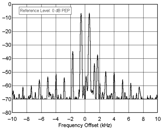
ICOM IC-746 serial number 001674 7.250 MHz, Transmit IMD, 100 W F:\SHARED\PROD_REV\TESTS\VC746\IC746750.TXT
