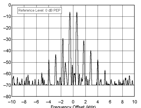
ICOM IC-746 serial number 001674 18.120 MHz, Transmit IMD, 100 W F:\SHARED\PROD_REV\TESTS\VC746\IC746120.TXT
