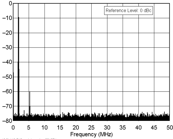
ICOM IC-746 serial number 001674 1.8 MHz Band, Spectral Purity, 100 W F:\SHARED\PROD_REV\TESTS\IC746\IC746SLO.TXT
