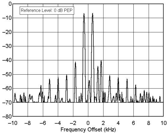
ICOM IC-746 serial number 001674 3.900 MHz, Transmit IMD, 100 W F:\SHARED\PROD_REV\TESTS\VC746\IC746390.TXT
