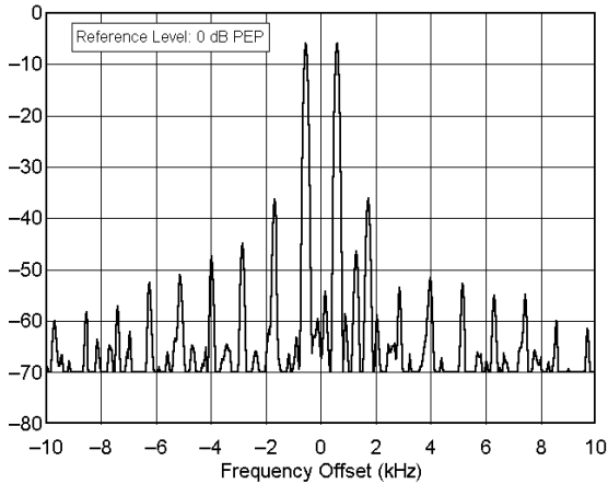
ICOM IC-746 serial number 001674 1.850 MHz, Transmit IMD, 100 W F:\SHARED\PROD_REV\TESTS\VC746\IC746180.TXT
