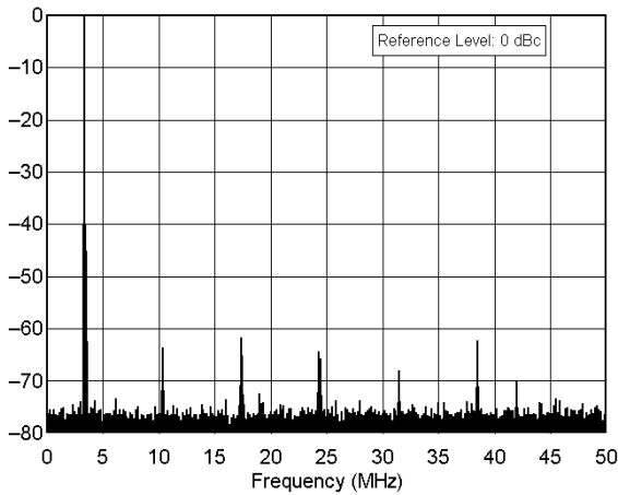
ICOM IC-746 serial number 001674 3.5 MHz Band, Spectral Purity, 100 W F:\SHARED\PROD_REV\TESTS\IC746\IC746S80.TXT
