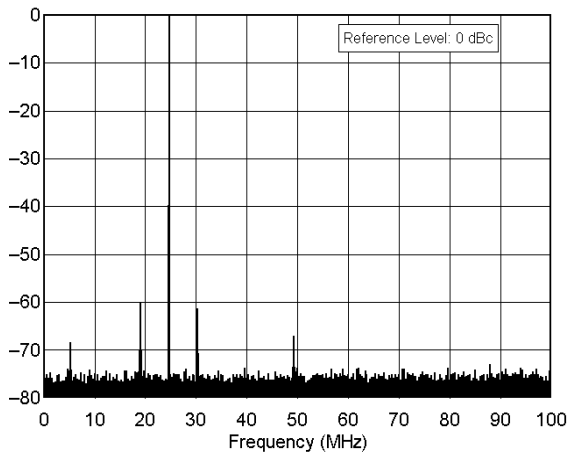
ICOM IC-746 serial number 001674 24.9 MHz Band, Spectral Purity, 100 W F:\SHARED\PROD_REV\TESTS\IC746\IC746S12.TXT
