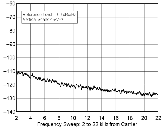
ICOM IC-746 serial number 001674 144.020 MHz, Phase Noise, 100 W F:\SHARED\PROD_REVTESTS\IC746\IC746P2M.TXT
