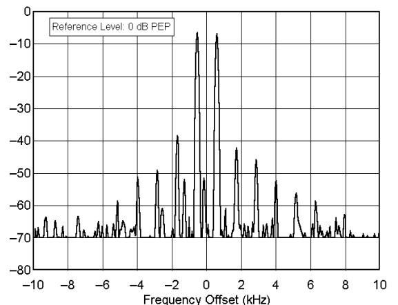
ICOM IC-746 serial number 001674 14.250 MHz, Transmit IMD, 100 W F:\SHARED\PROD_REV\TESTS\VC746\IC746250.TXT
