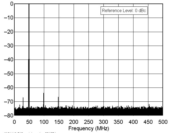
ICOM IC-746 serial number 001674 50.0 MHz Band, Spectral Purity, 100 W F:\SHARED\PROD_REV\TESTS\IC746\IC746S6M.TXT
