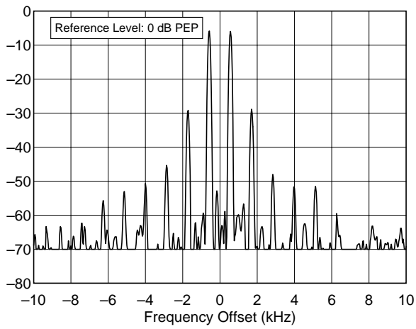
FT-1000MP 21.250 MHz, Transmit IMD, 100 W F:\SHARED\PROD_REV\TESTS\FT1000\FT100115.TXT
