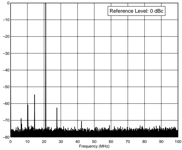
FT-1000MP 21.0 MHz Band, Spectral Purity, 100 W F:\SHARED\PROD_REV\TESTS\FT1000\FT100S15.TXT
