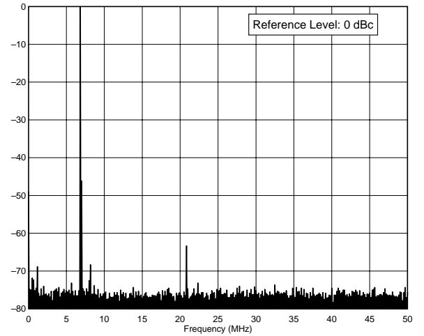
FT-1000MP 7.0 MHz Band, Spectral Purity, 100 W F:\SHARED\PROD_REV\TESTS\FT1000\FT100S40.TXT
