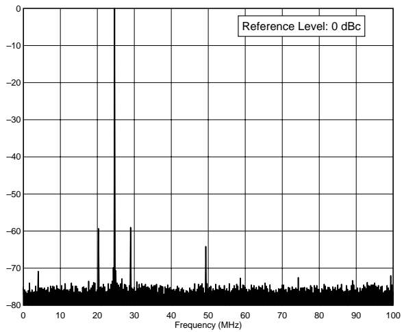
FT-1000MP 24.9 MHz Band, Spectral Purity, 100 W F:\SHARED\PROD_REV\TESTS\FT1000\FT100S12.TXT
