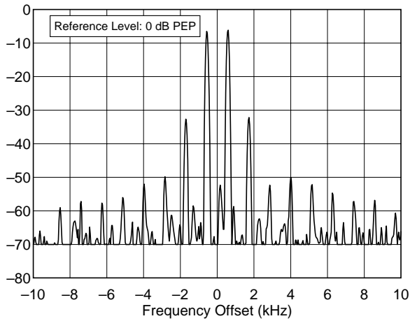
FT-1000MP 7.250 MHz, Transmit IMD, 100 W F:\SHARED\PROD_REV\TESTS\FT1000\FT100140.TXT
