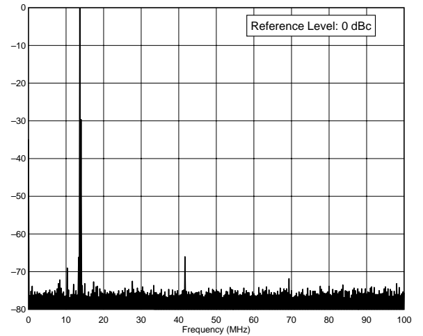
FT-1000MP 14.0 MHz Band, Spectral Purity, 100 W F:\SHARED\PROD_REV\TESTS\FT1000\FT100S20.TXT
