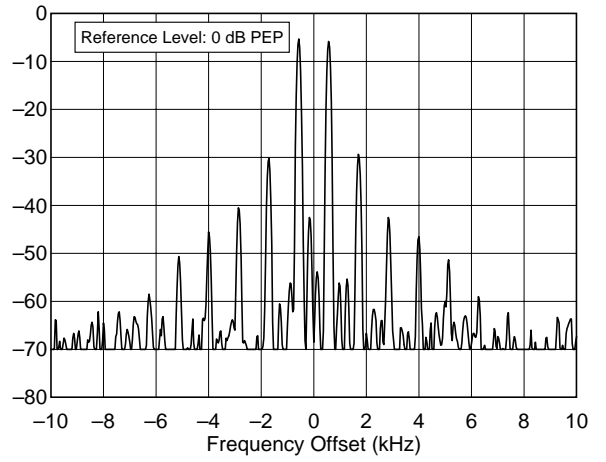
FT-1000MP 28.350 MHz, Transmit IMD, 100 W F:\SHARED\PROD_REV\TESTS\FT1000\FT100110.TXT
