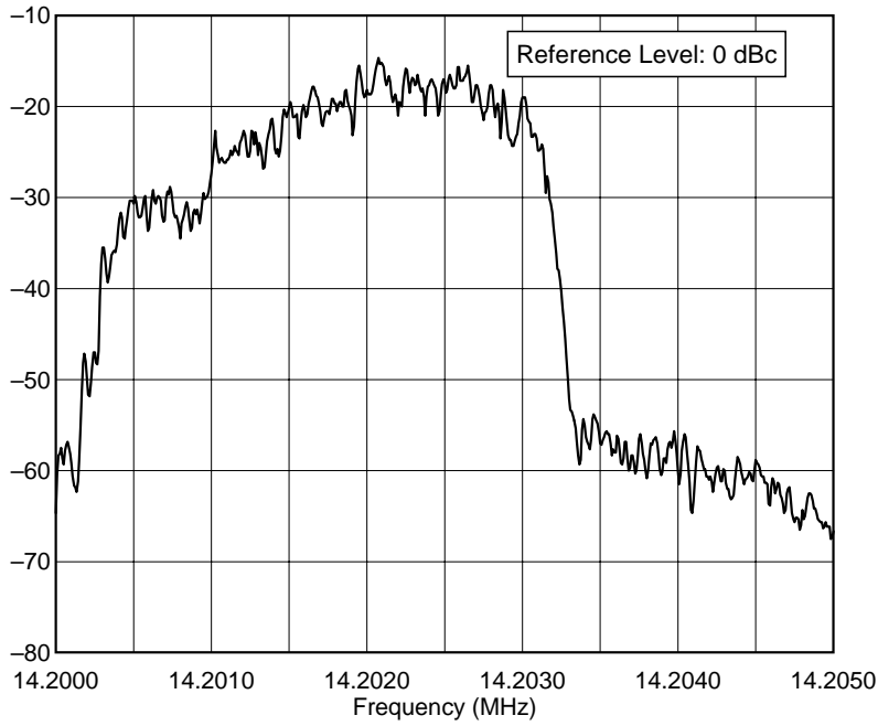
Yaesu FT-1000MP 14.2 MHz USB Xmit Bandpass, EDSP Mic Setting 1 P:\TESTS\FT1000\FT1KXM1.TXT
