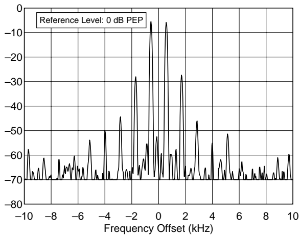
FT-1000MP 24.950 MHz, Transmit IMD, 100 W F:\SHARED\PROD_REV\TESTS\FT1000\FT100112.TXT
