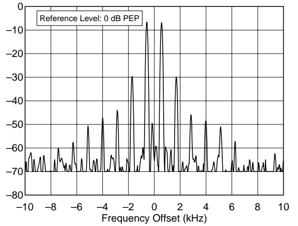
FT-1000MP 14.250 MHz, Transmit IMD, 100 W F:\SHARED\PROD_REV\TESTS\FT1000\FT100120.TXT
