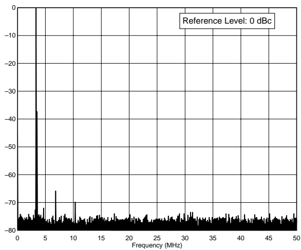
FT-1000MP 3.5 MHz Band, Spectral Purity, 100 W F:\SHARED\PROD_REV\TESTS\FT1000\FT100S80.TXT
