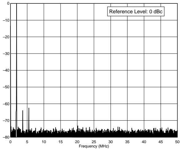
FT-1000MP 1.8 MHz Band, Spectral Purity, 100 W F:\SHARED\PROD_REV\TESTS\FT1000\FT100SLO.TXT
