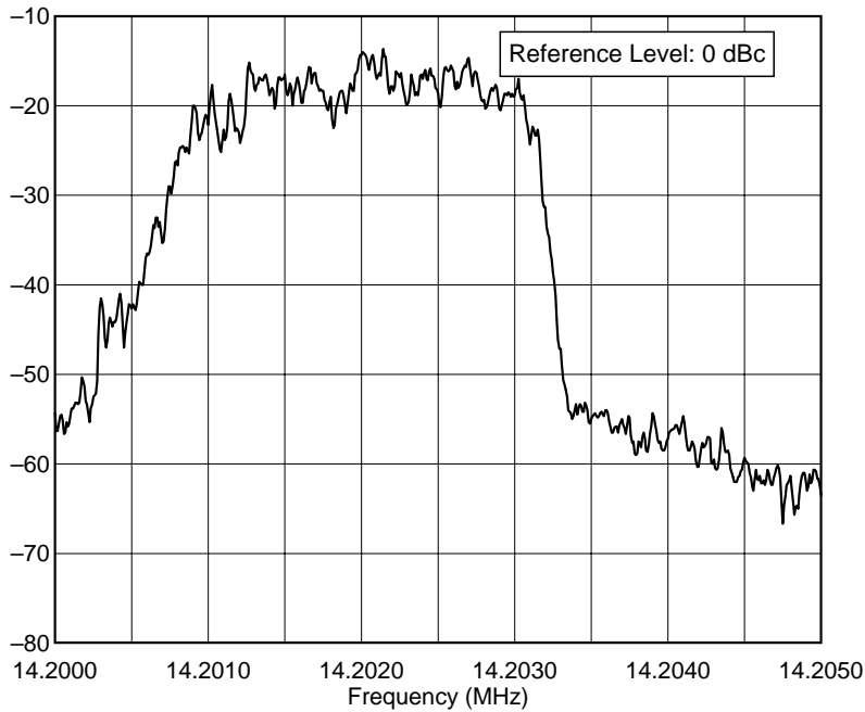
Yaesu FT-1000MP 14.2 MHz USB Xmit Bandpass, EDSP Mic Setting 2 P:\TESTS\FT1000\FT1KXM2.TXT
