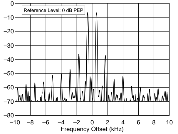
FT-1000MP 10.120 MHz, Transmit IMD, 100 W F:\SHARED\PROD_REV\TESTS\FT1000\FT100130.TXT
