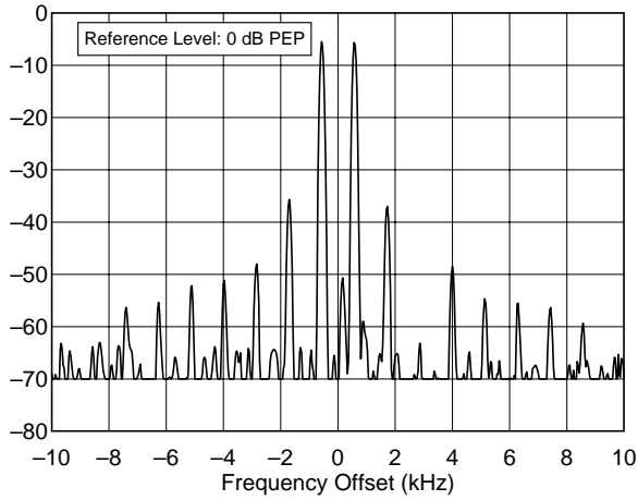
FT-1000MP 1.850 MHz, Transmit IMD, 100 W F:\SHARED\PROD_REV\TESTS\FT1000\FT10010I.LO.TXT
