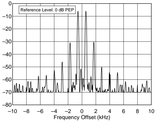
FT-1000MP 18.120 MHz, Transmit IMD, 100 W F:\SHARED\PROD_REV\TESTS\FT1000\FT100117.TXT
