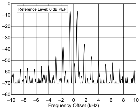
FT-1000MP 3.900 MHz, Transmit IMD, 100 W F:\SHARED\PROD_REV\TESTS\FT1000\FT100180.TXT
