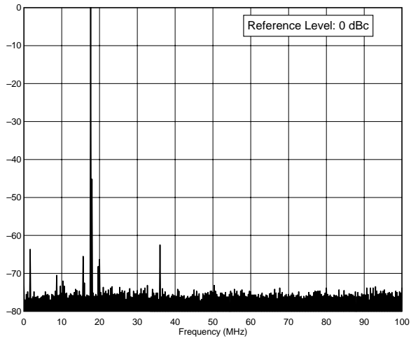
FT-1000MP 18.1 MHz Band, Spectral Purity, 100 W F:\SHARED\PROD_REV\TESTS\FT1000\FT100S17.TXT
