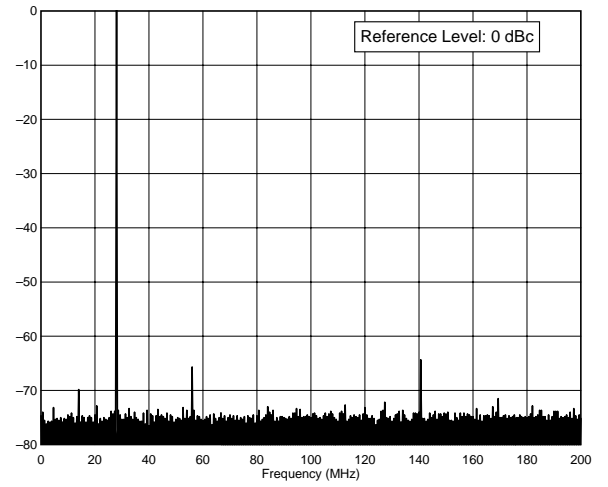
FT-1000MP 28.0 MHz Band, Spectral Purity, 100 W F:\SHARED\PROD_REV\TESTS\FT1000\FT100S10.TXT
