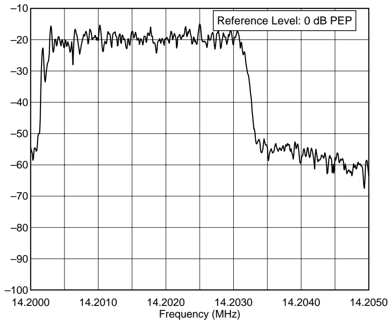
Yaesu FT-1000MP 14.2 MHz USB Xmit Bandpass, EDSP 300-3100 Hz P:\TESTS\FT1000\FT1KX3.TXT
