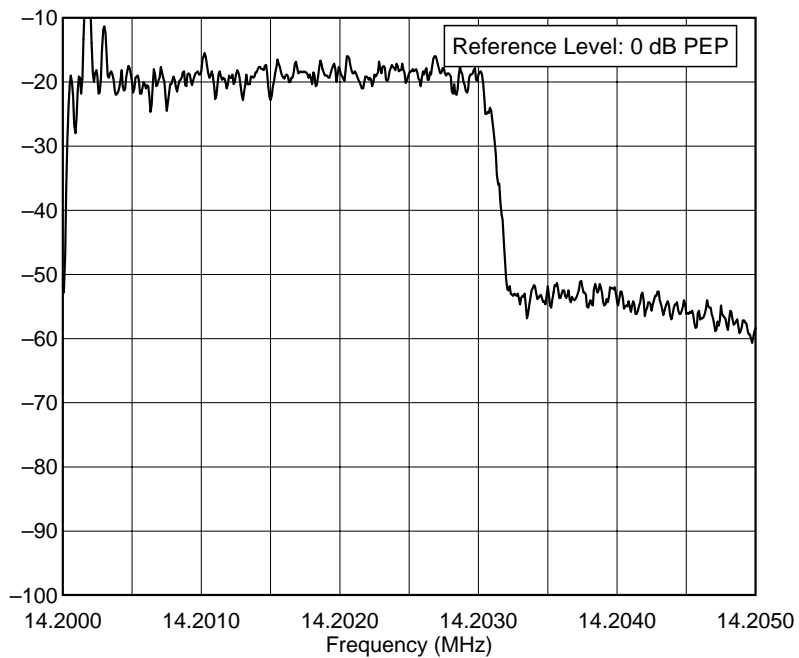
Yaesu FT-1000MP 14.2 MHz USB Xmit Bandpass, EDSP 100-3100 Hz P:\TESTS\FT1000\FT1KX1.TXT
