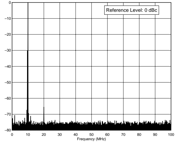
FT-1000MP 10.1 MHz Band, Spectral Purity, 100 W F:\SHARED\PROD_REV\TESTS\FT1000\FT100S30.TXT
