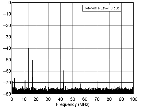
Yaesu FT-847 sn 8C020205 14.0 MHz Band, Spectral Purity, 100 W F:\SHARED\PROD_REV\TESTS\F\T847\F\T847S20.TXT
