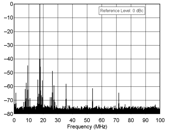
Yaesu FT-847 sn 8C020205 18.1 MHz Band, Spectral Purity, 100 W F:\SHARED\PROD_REV\TESTS\F\T847\F\T847S17.TXT
