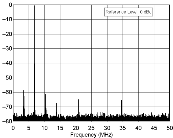
Yaesu FT-847 sn 8C020205 7.0 MHz Band, Spectral Purity, 100 W F:\SHARED\PROD_REV\TESTS\F\T847\F\T847S40.TXT
