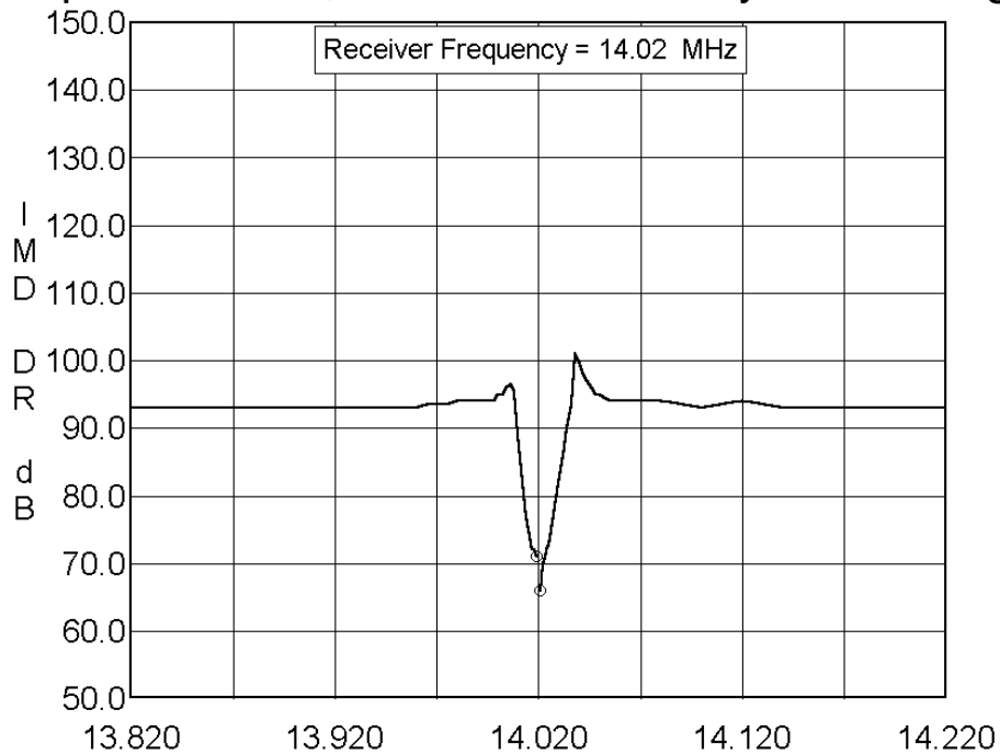
Swept Two-Tone, Third-Order IMD Dynamic Range
