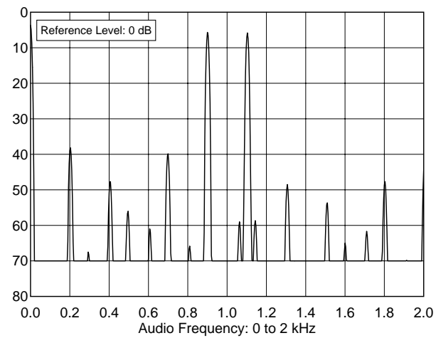
COM IC-718 s/n 001069q 4.020 MHz, In-Band Receiver IMD, S9+60 signals :\MYDOCU-1\PRODREV\TESTDATA\ICOM\IC718\IC718IB6.TXT
