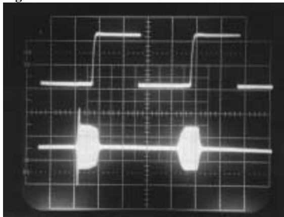
First and second dits, semi-QSK, 20W
