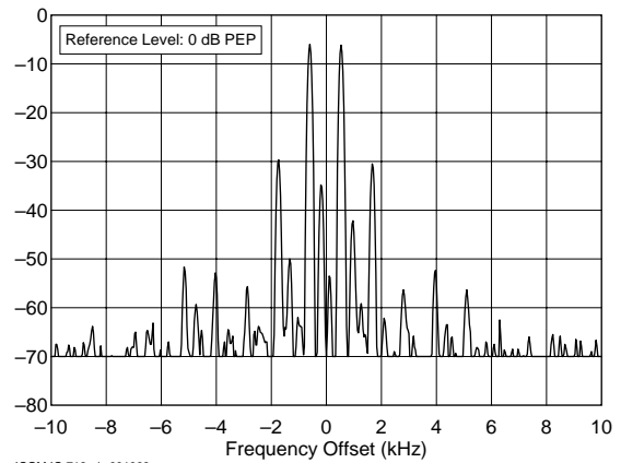
ICOM IC-718 s/n 001069 10.120 MHz, Transmit IMD, 100 W C:\TESTS\IC718\IC718I30.TXT
