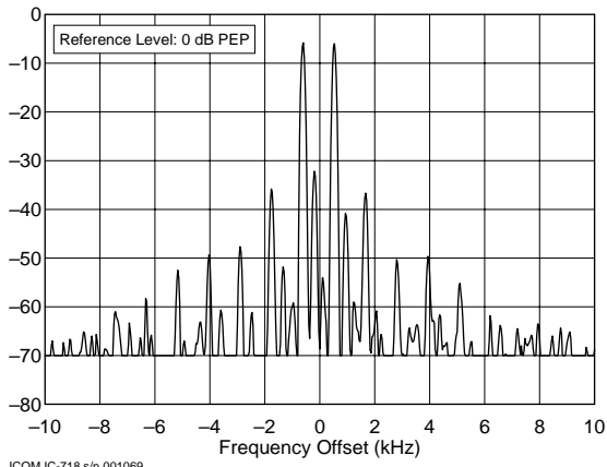
ICOM IC-718 s/n 001069 14.250 MHz, Transmit IMD, 100 W C:\TESTS\IC718\IC718I20.TXT
