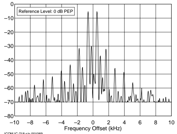
ICOM IC-718 s/n 001069 21.250 MHz, Transmit IMD, 100 W C:\TESTS\IC718\IC718I15.TXT
