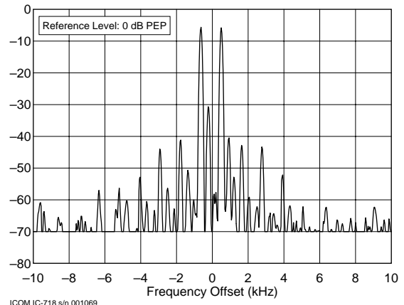
ICOM IC-718 s/n 001069 24.950 MHz, Transmit IMD, 100 W C:\TESTS\IC718\IC718I12.TXT
