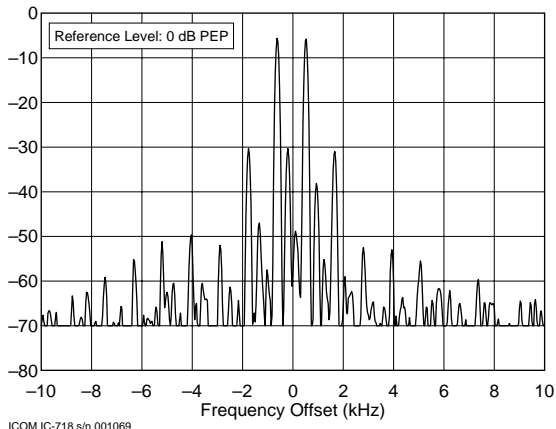
ICOM IC-718 s/n 001069 18.120 MHz, Transmit IMD, 100 W C:\TESTS\IC718\IC718I17.TXT
