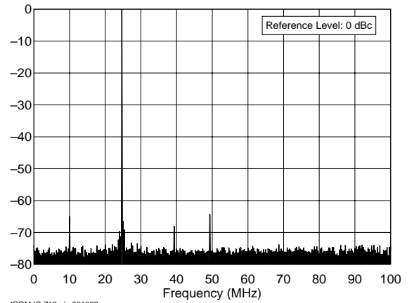
ICOM IC-718 s/n 001069 24.9 MHz Band, Spectral Purity, 100 W C:\TESTS\IC718\IC718S12.TXT
