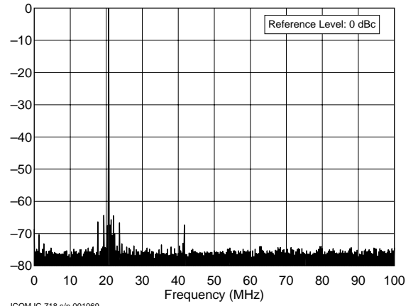
ICOM IC-718 s/n 001069 21.0 MHz Band, Spectral Purity, 100 W C:\TESTS\IC718\IC718S15.TXT
