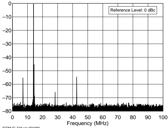
ICOM IC-718 s/n 001069 14.0 MHz Band, Spectral Purity, 100 W C:\TESTS\IC718\IC718S20.TXT
