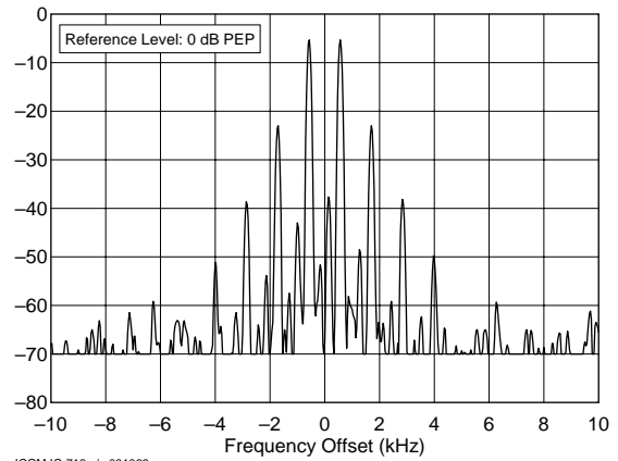
ICOM IC-718 s/n 001069 7.250 MHz, Transmit IMD, 100 W C:\TESTS\IC718\IC718I40.TXT
