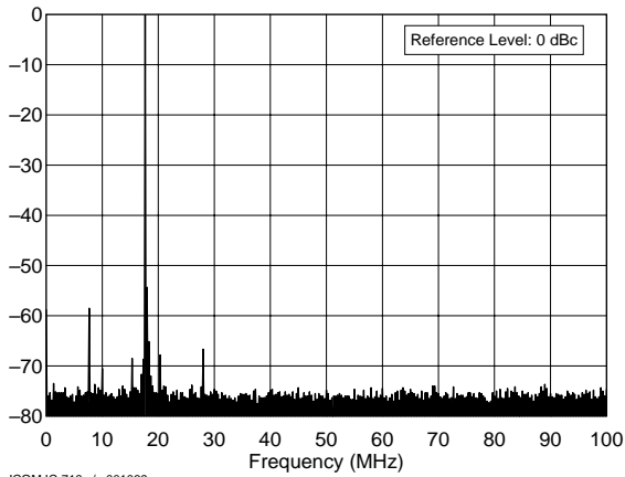
ICOM IC-718 s/n 001069 18.1 MHz Band, Spectral Purity, 100 W C:\TESTS\IC718\IC718S17.TXT
