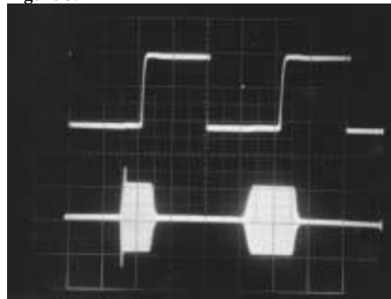
First and second dits, semi-QSK, 25W (Four vertical divisions on this photo represent 100W)
