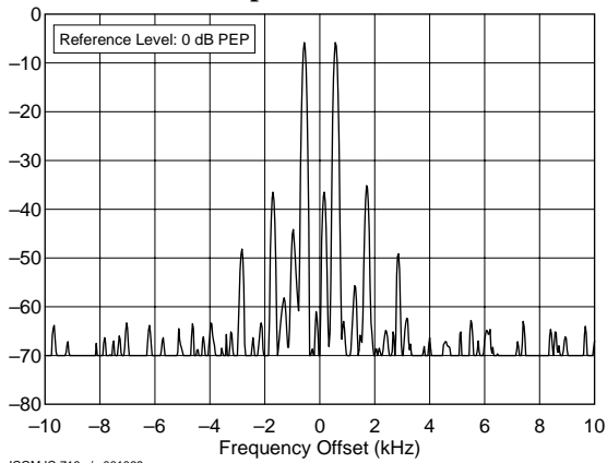
ICOM IC-718 s/n 001069 1.850 MHz, Transmit IMD, 100 W C:\TESTS\IC718\IC718I10.TXT
