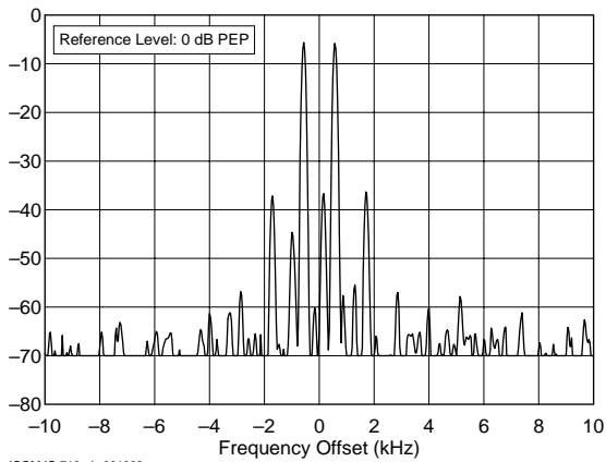
ICOM IC-718 s/n 001069 3.900 MHz, Transmit IMD, 100 W C:\TESTS\IC718\IC718I80.TXT
