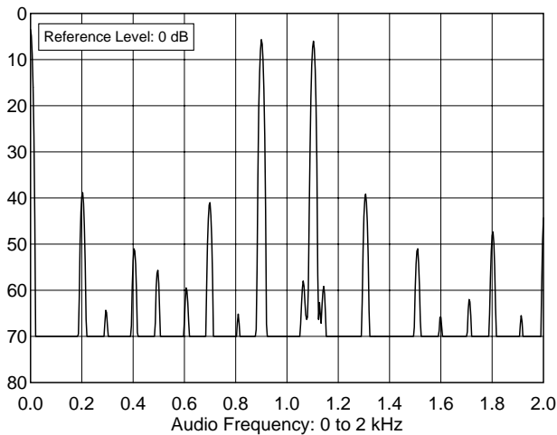
COM IC-718 s/n 001069q 4.020 MHz, In-Band Receiver IMD, S9 signals :\MYDOCU-1\PRODREV\TESTDATA\ICOM\IC718\IC718IBF.TXT
