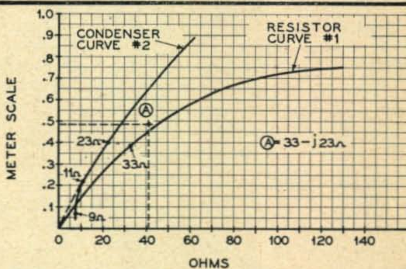
Fig. 9. The "Matchmaker" will not read correctly when the load is largely reactive. The magnitude of some tests taken at 3.5 mc are shown above.
