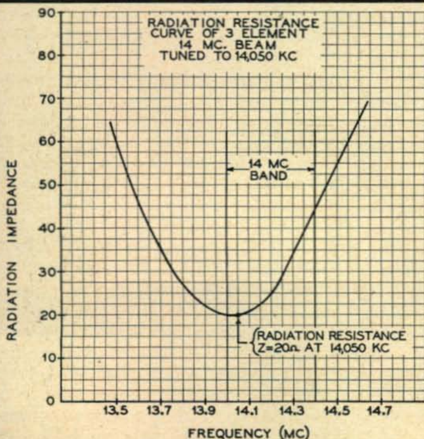
Fig. 8. Your final graph should look something like this. The radiation resistance is the value at the lowest meter reading.
