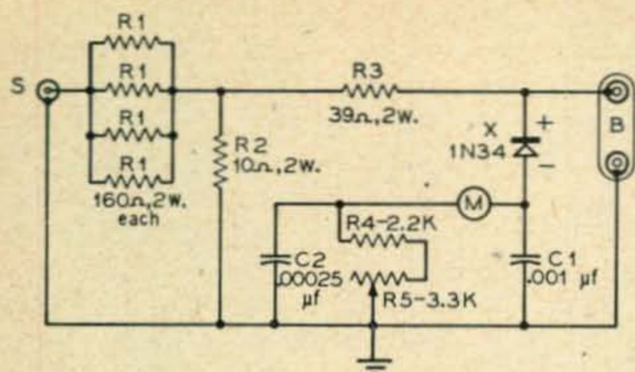
Fig. 5. Schematic of the "Matchmaker." This unit operates on the same basic principle as a low range shunt reading d.c. ohmmeter. The following values of 1 watt composition resistors are necessary for calibration: 5.6, 12, 22, 33, 55, 68, 82, 100, 220 and 350.
