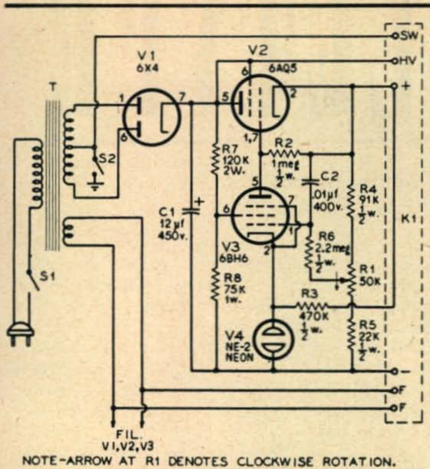
Fig. 2. Circuit schematic of the "Minipak" regulated voltage power supply.
