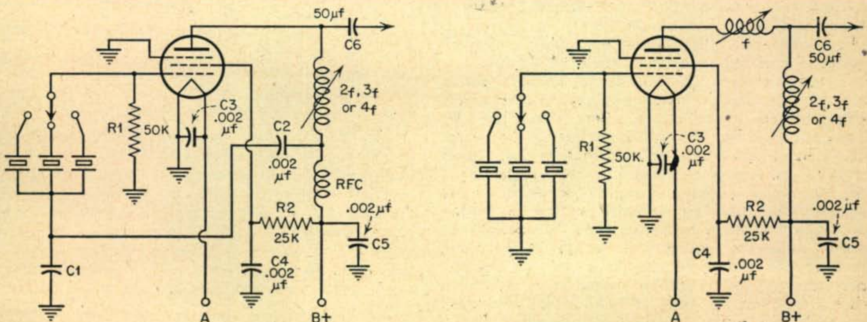
Fig. 1 (left). A method of operating quick-heating tubes with the filament at ground potential. For the value of C1 see text. Fig. 2 (right). A harmonic oscillator using tubes similar to the 2E30.
