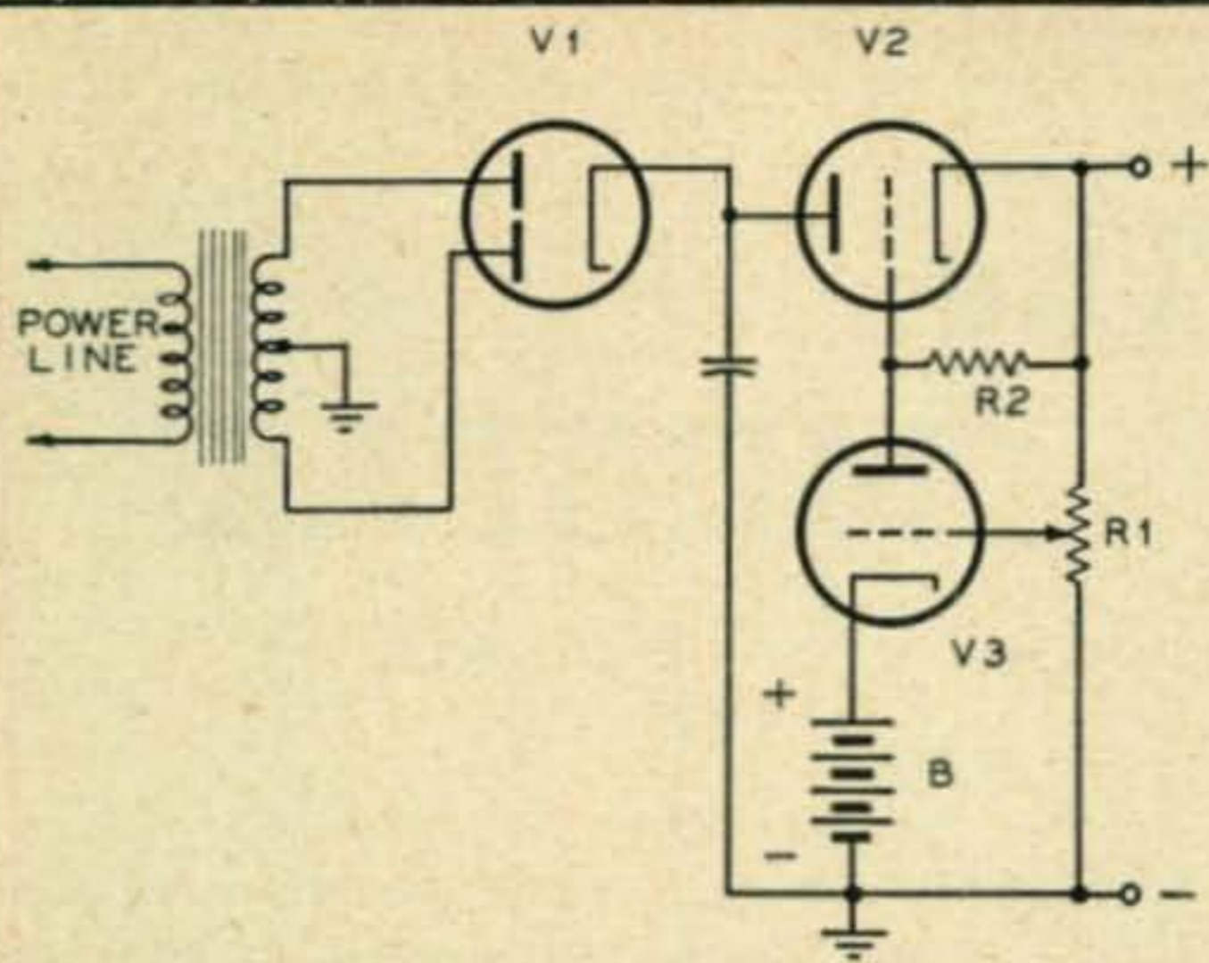
Fig. 1. Basic current regulator circuit schematic.
