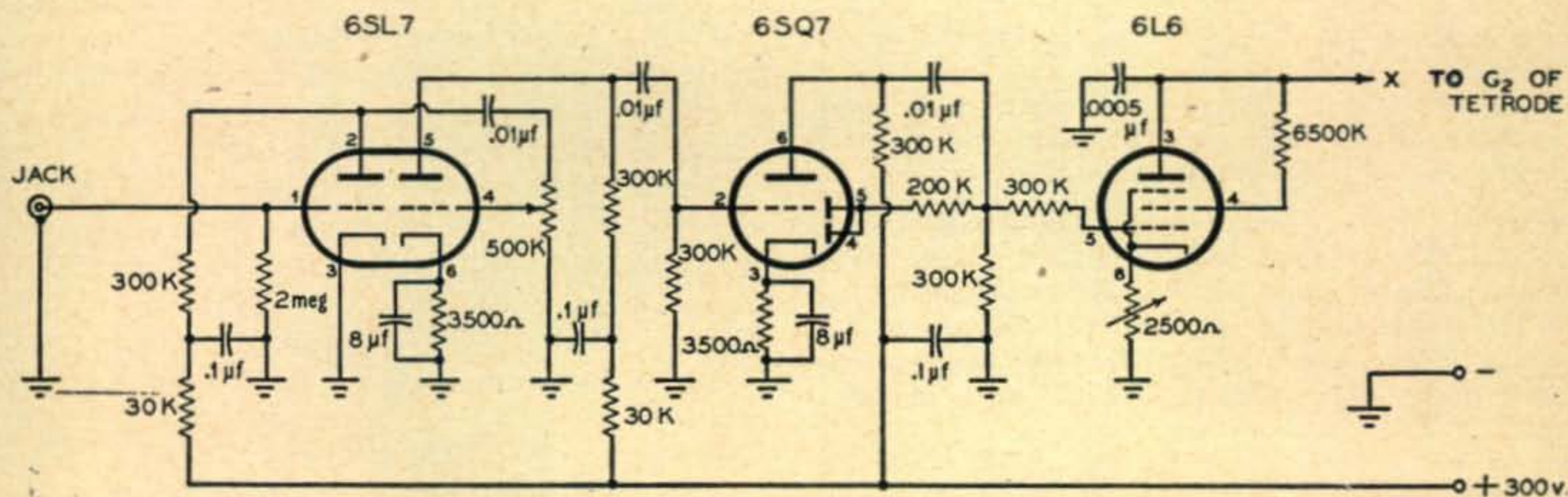
SPEECH AMPLIFIER AND 6L6 MODULATOR TO MODULATE SCREEN OF TETRODES
