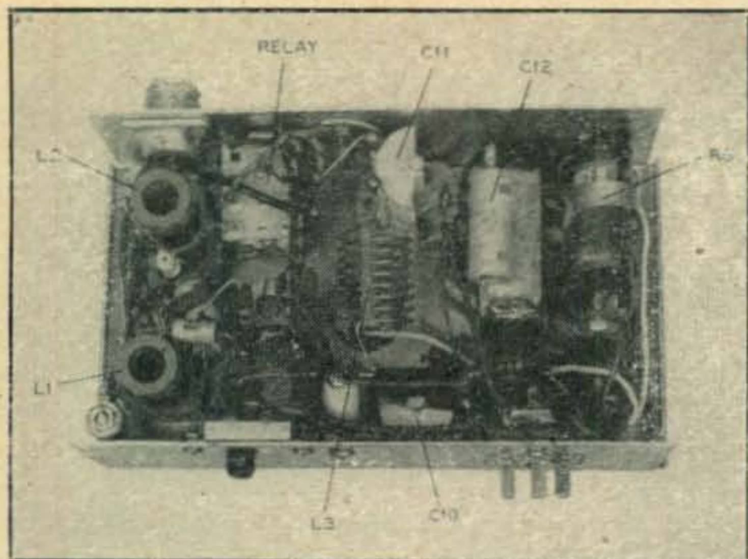
Under chassis view of the 28-28 showing the location of the important components
