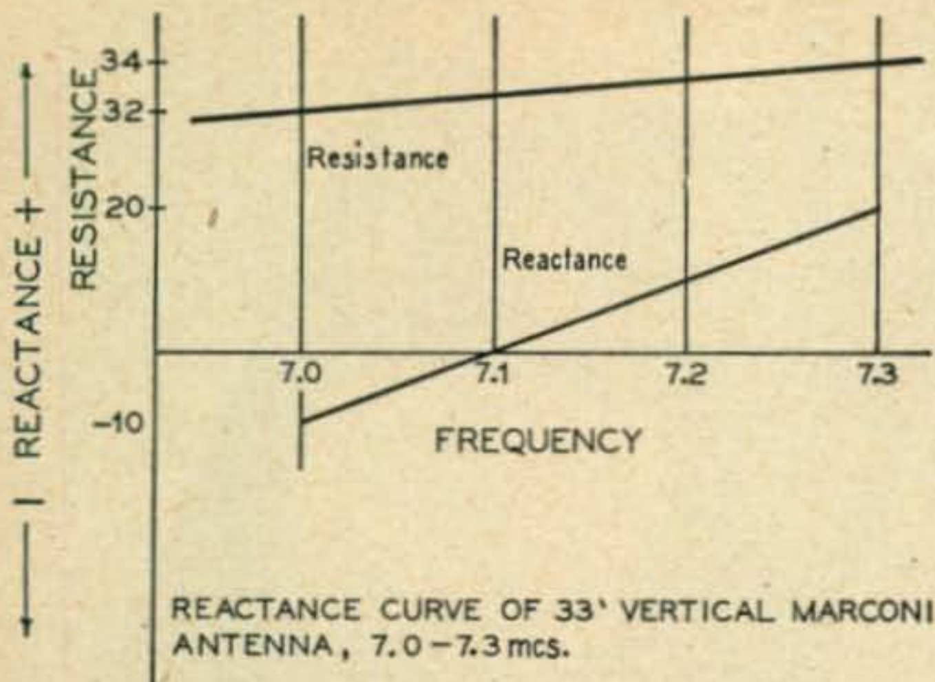
Fig. 2. Determining the radiation resistance at antenna resonance.
