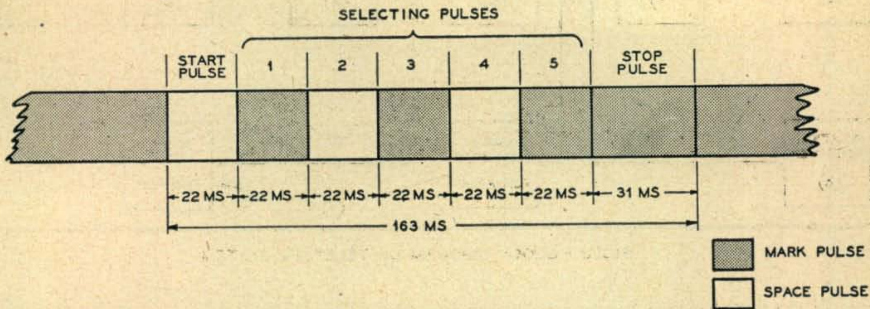
FIG. 1. - TELETYPE CODE FOR LETTER "Y"
