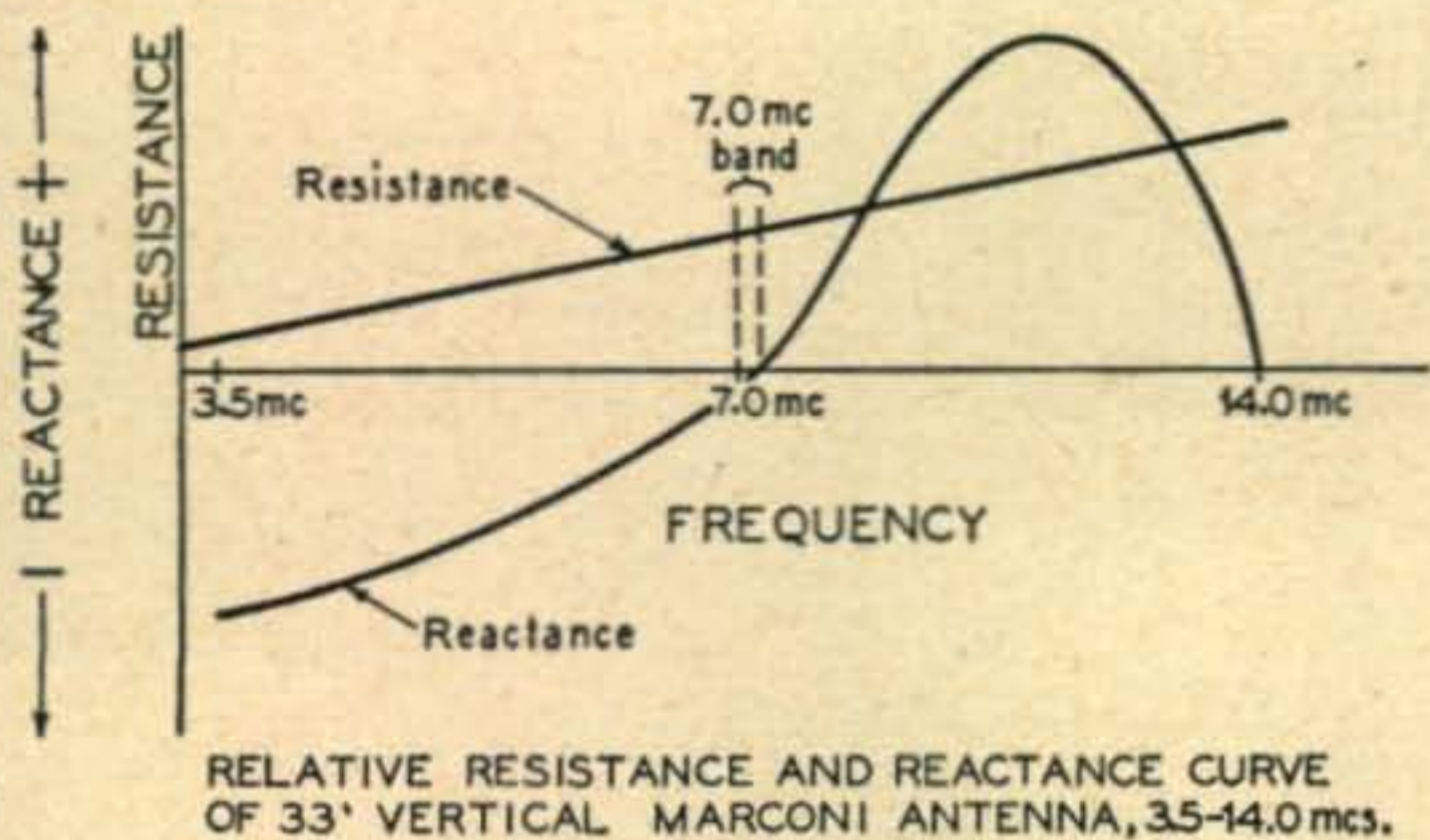
Fig. 1. Typical plot covering the three principal amateur bands.
