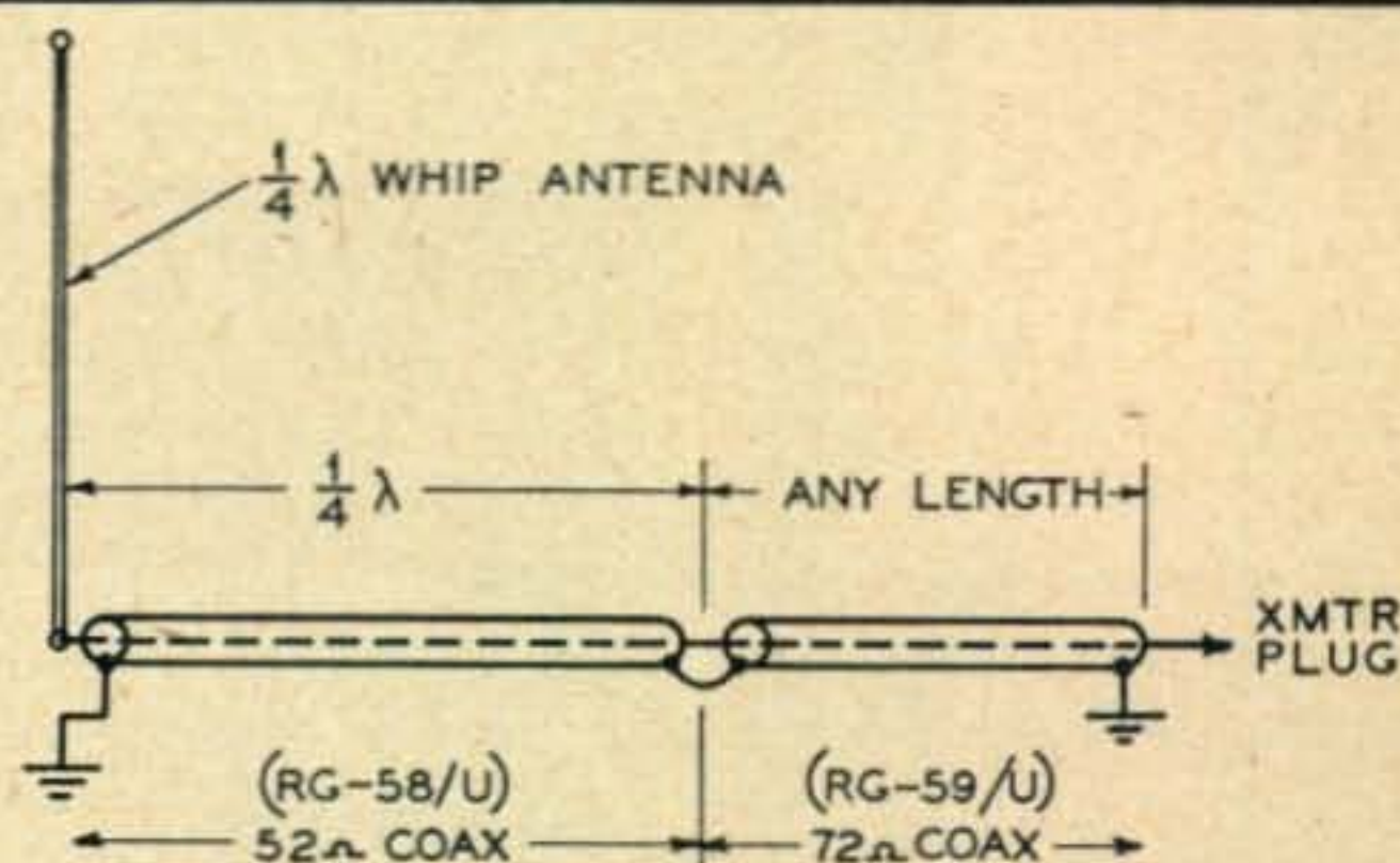
Fig. 2. Quarter wave matching section as used to match a resonant whip to 72-ohm line. The car body is used as ground.
