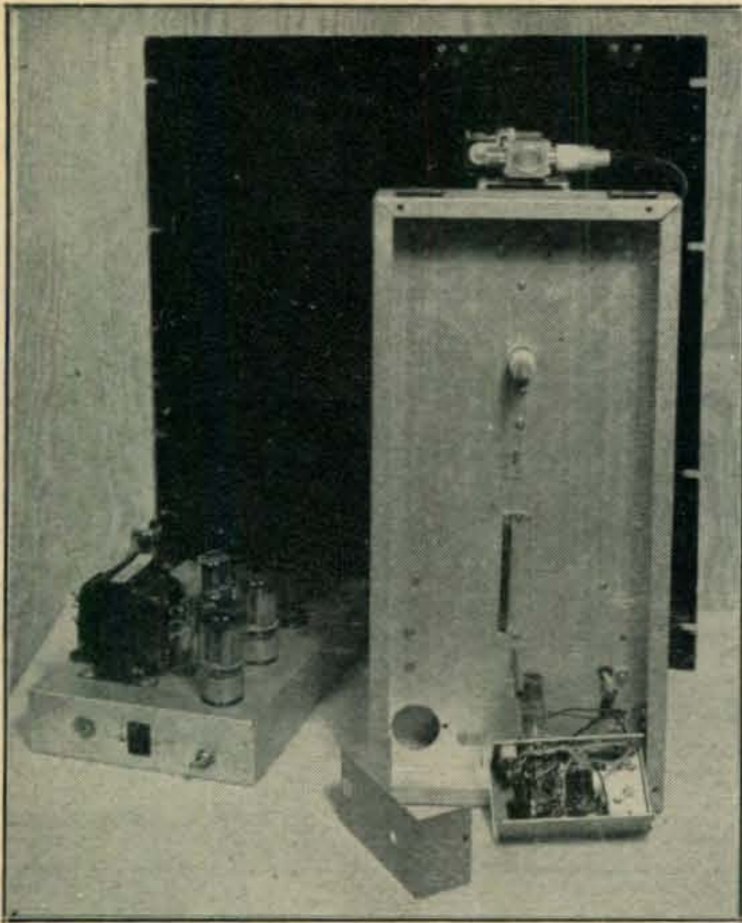
Underneath the final amplifier chassis is the small aluminum box containing the 25 mc crystal oscillator.
