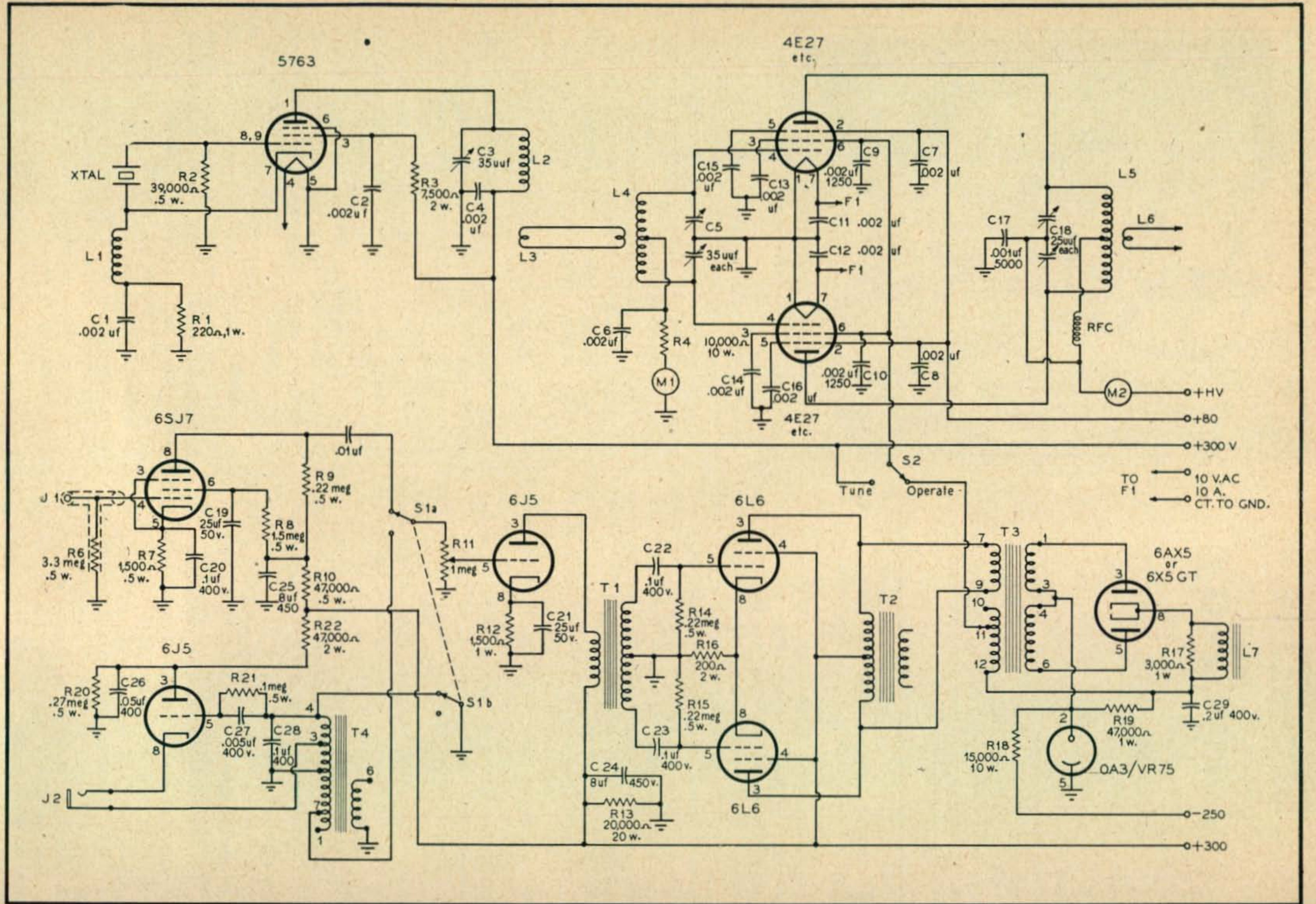
Fig. 1. Circuit schematic of the complete six-meter transmitter.
