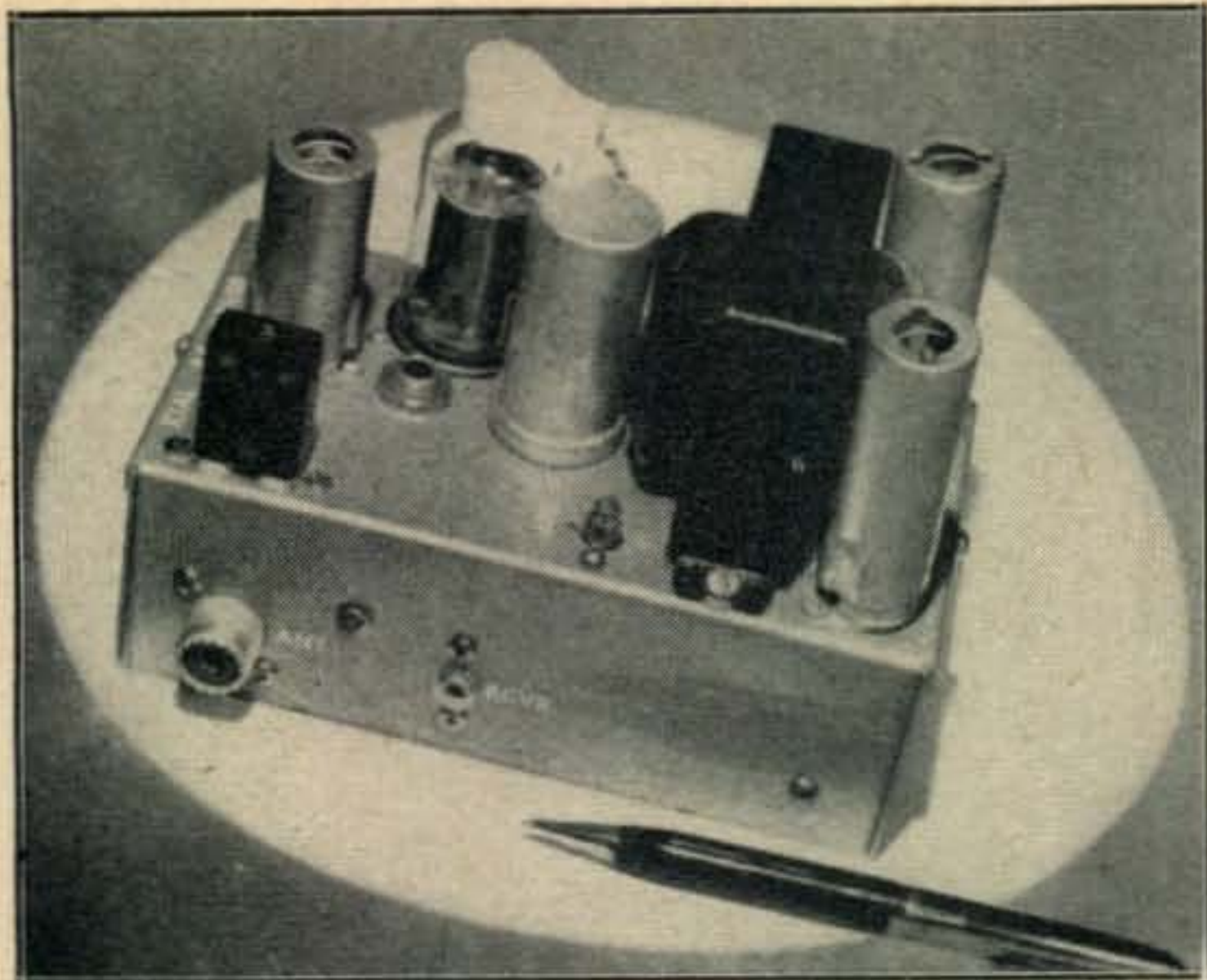
This view shows the metering jack next to the 2E26 and next to the 6J6 r-f driver. The antenna coupling adjusting capacitor C11 is in the center near the modulation transformer.
