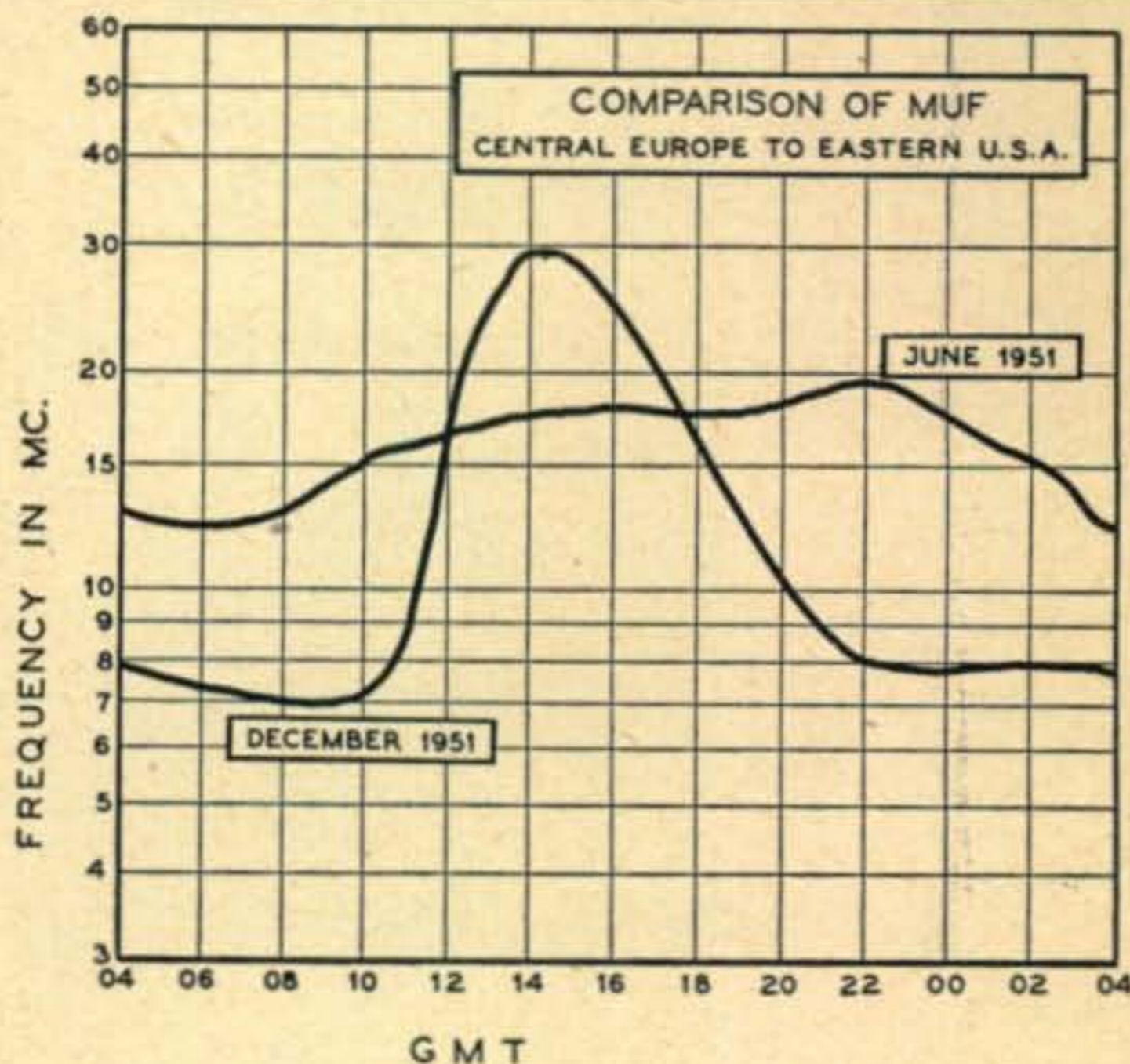
Fig. 1. MUF characteristics at the winter and summer solstice.
