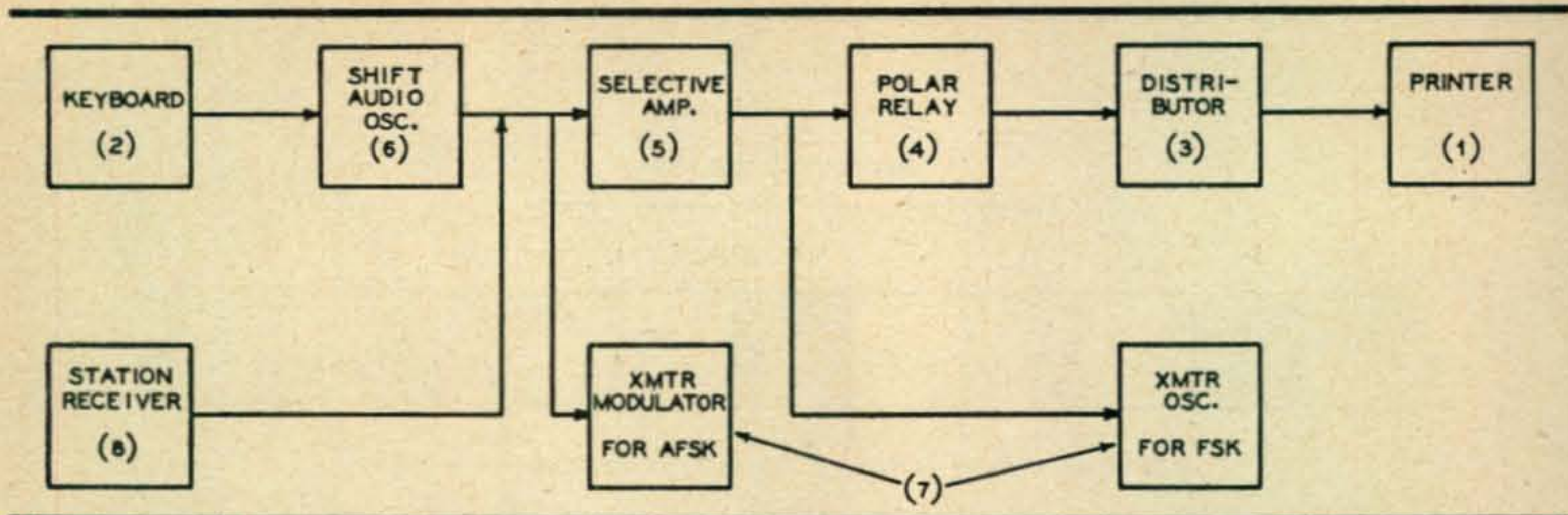
FIG. 2 - BLOCK DIAGRAM OF TELETYPE SYSTEM
