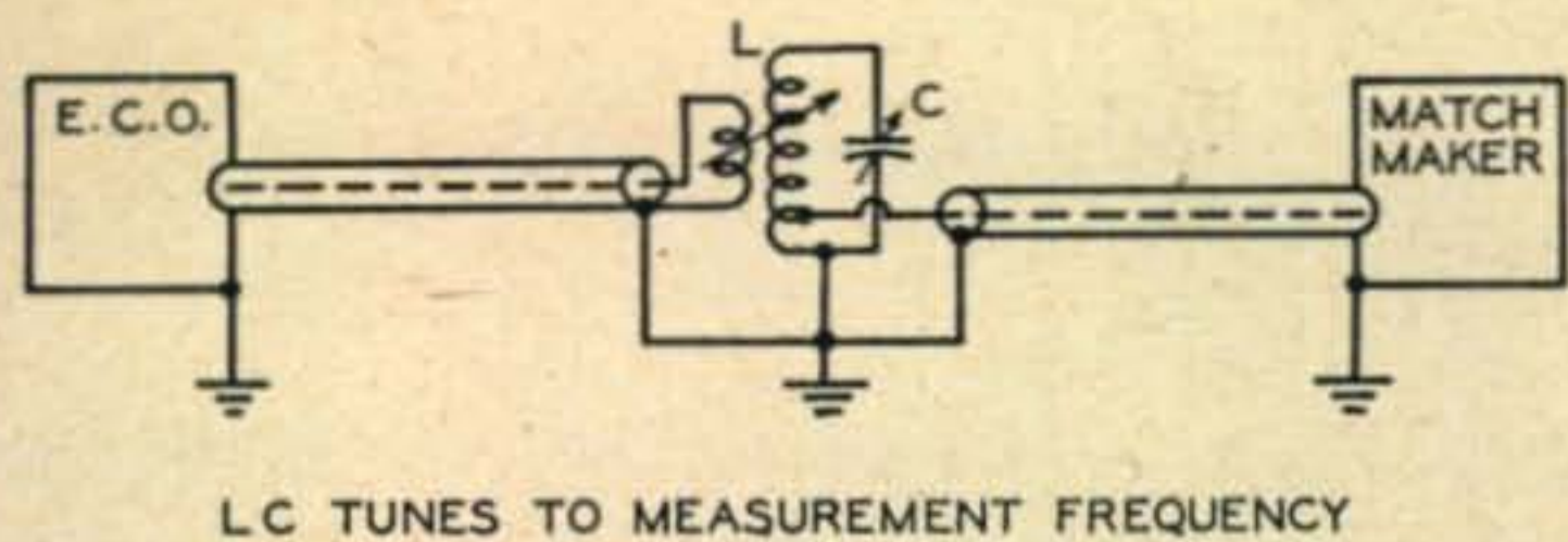
Fig. 7. A method of coupling permitting control of the r-f input.
