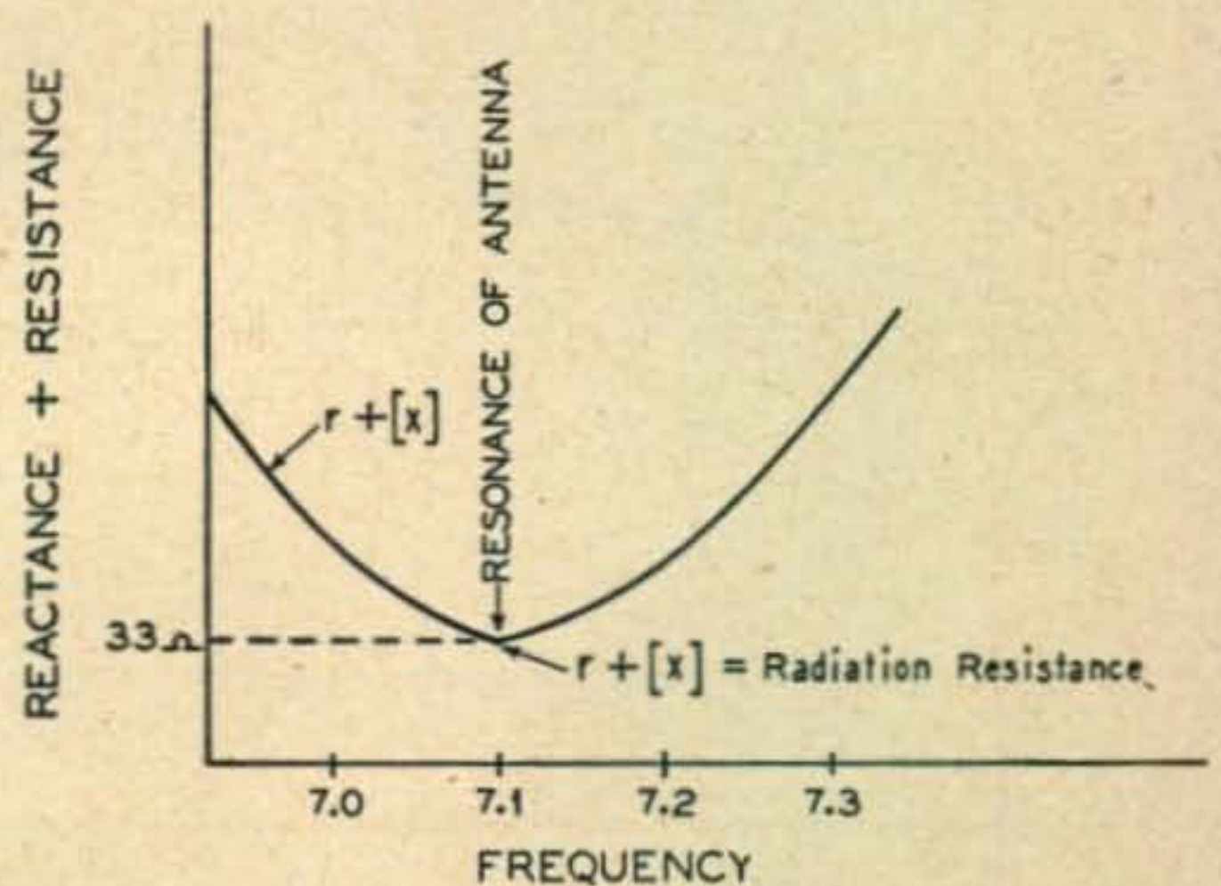
Fig. 3. Obtaining the absolute values.
