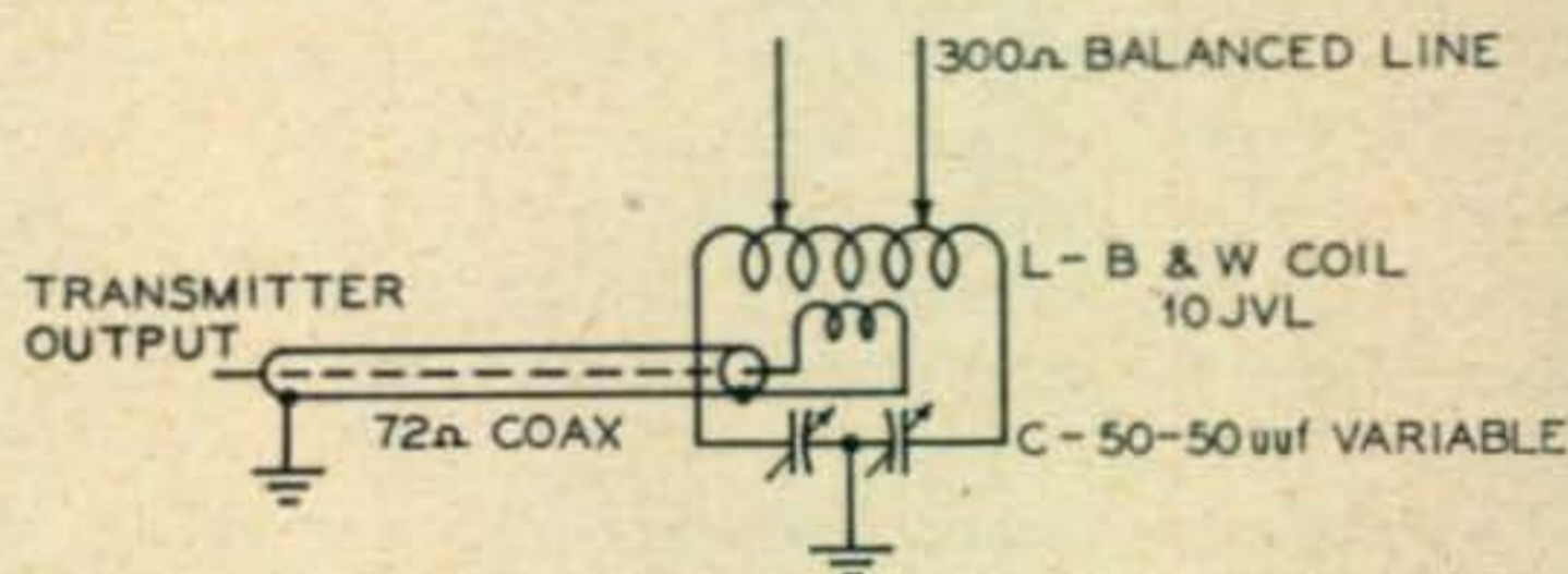
FIGURE 3a. BALANCED RESONANT TUNER
