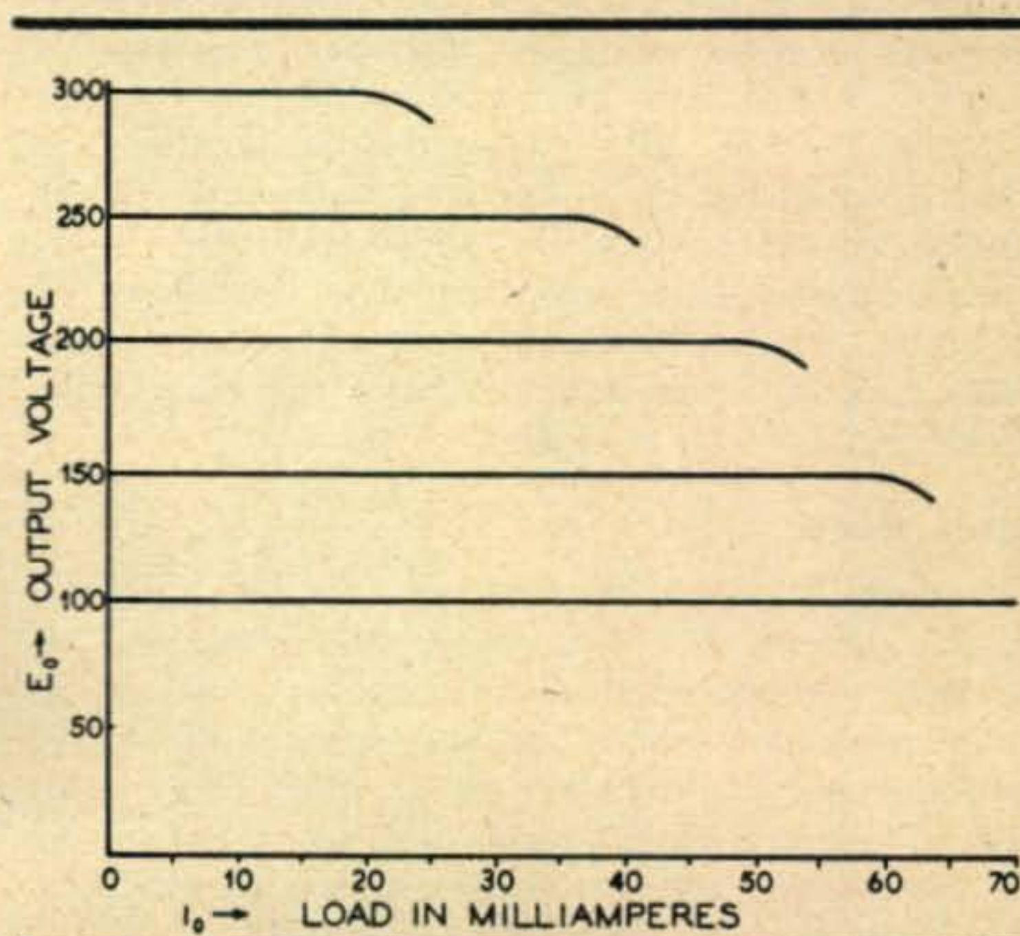
Fig. 3. Voltage output regulation curve under various conditions of load.
