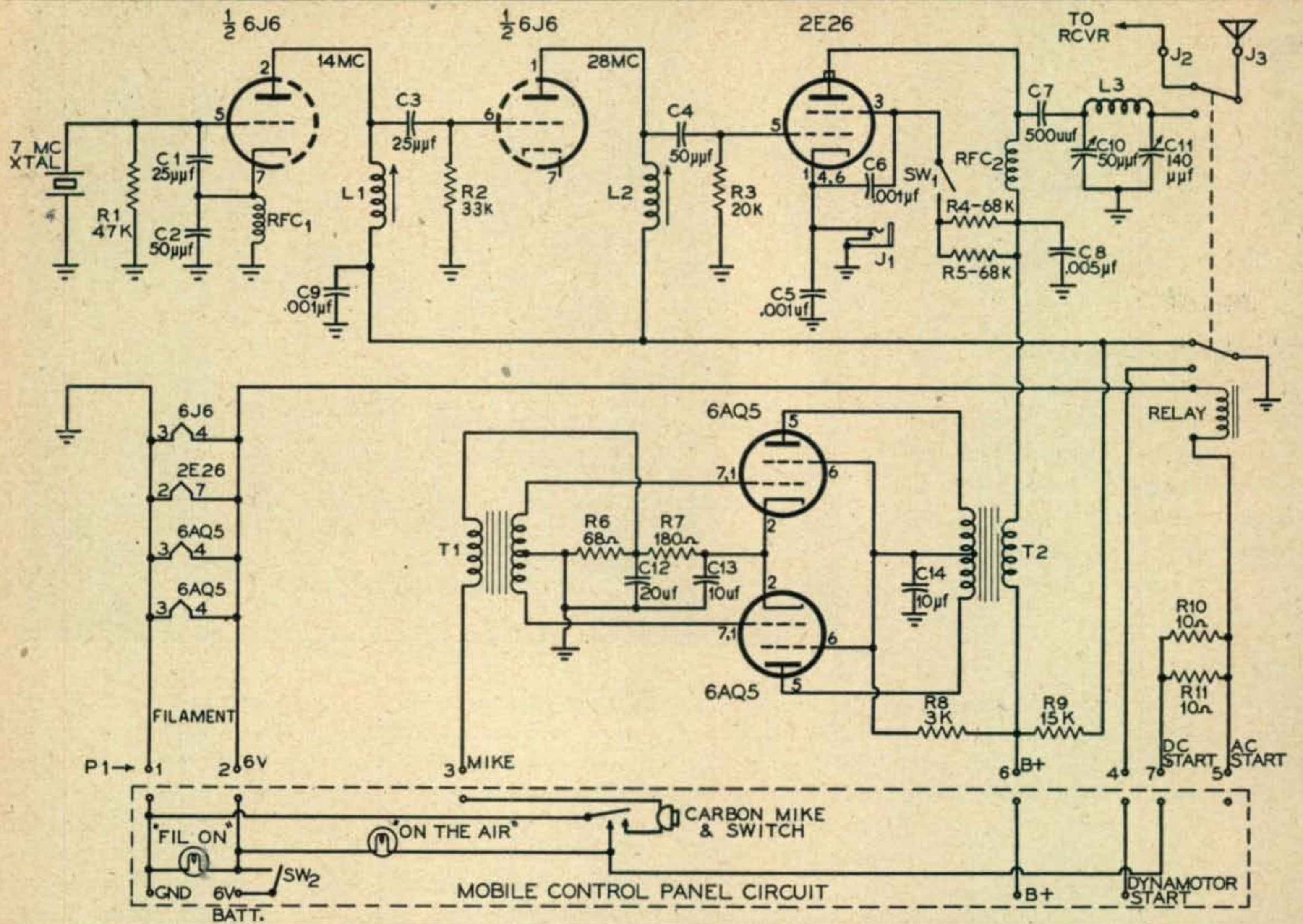
Fig. 1. Wiring schematic of the 28 watt 10 meter transmitter.
