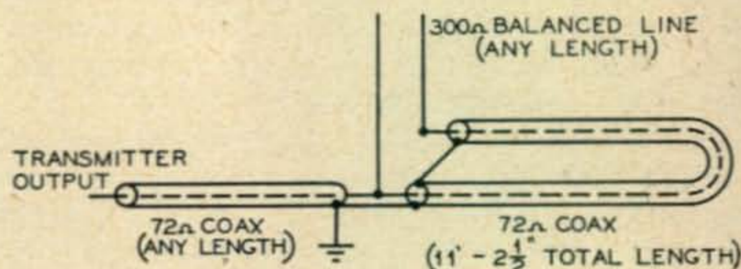
FIGURE 3b. THE BALUN
