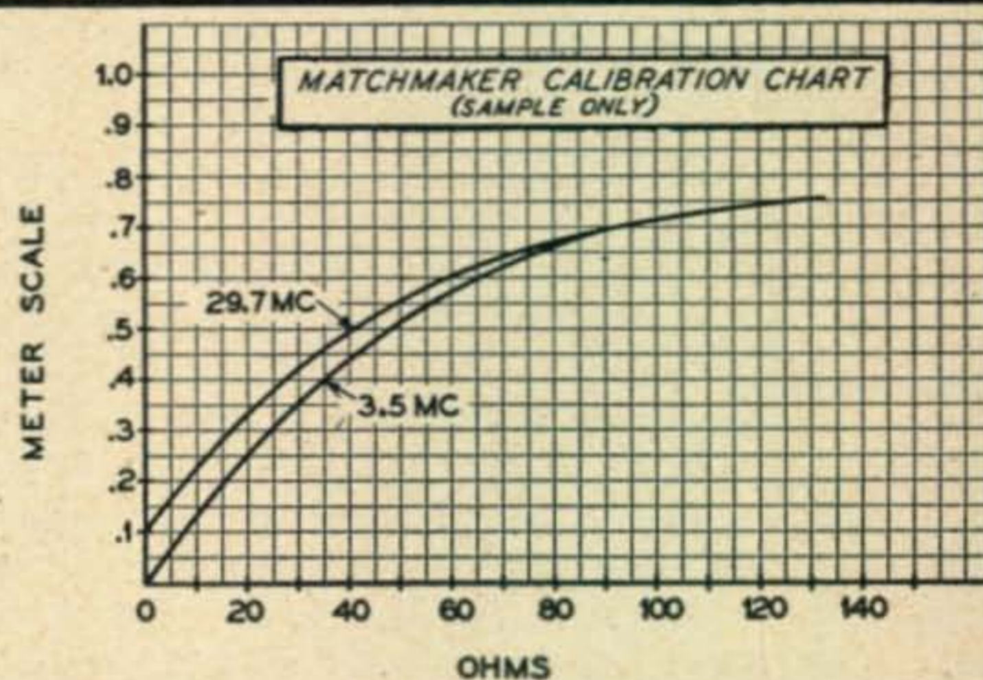
Fig. 6. Typical calibration chart also showing the shift in calibration due to the use of inductive resistors. If expensive non-inductive resistors are employed this shift will disappear.
