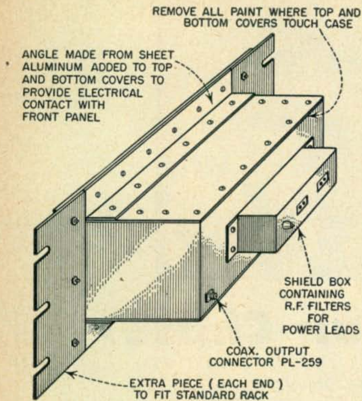
Fig. 1. Although the TU-10B is a good foundation for a shield around the final it will need the various finishing touches outlined above to be really effective in reducing harmonics.
