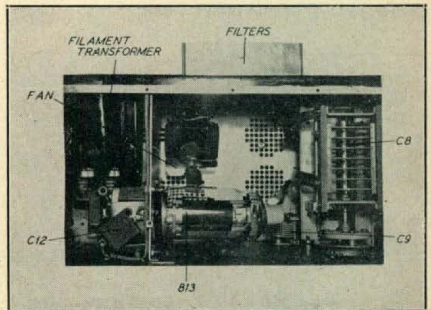
Inside view of final with top plate removed. Note how internal shield has been moved to the left. Low inductance copper strip leads can be seen running to 813 and plate tuning condenser.
