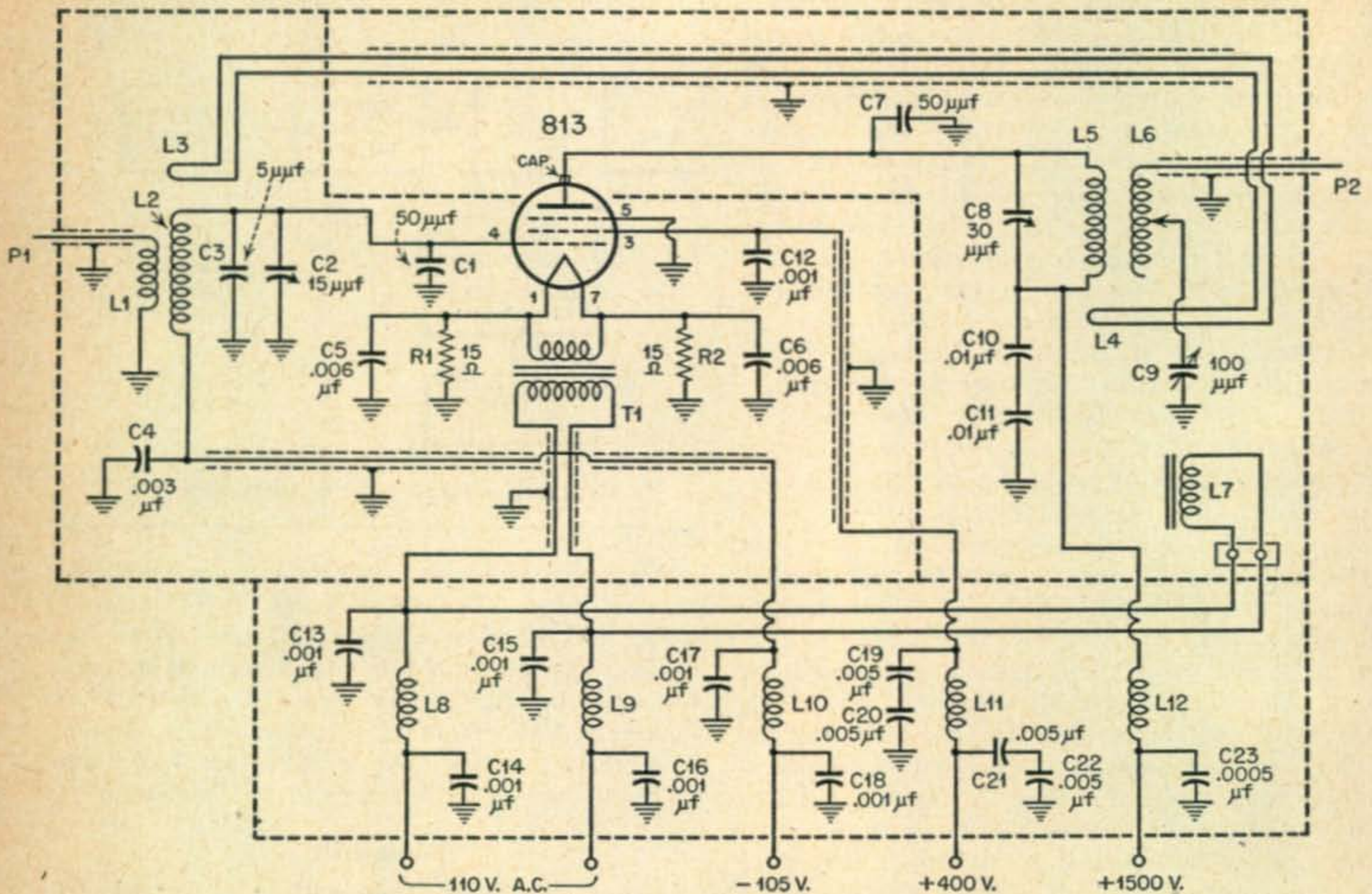
Schematic of the 20 meter final in the TU-10B cabinet.
