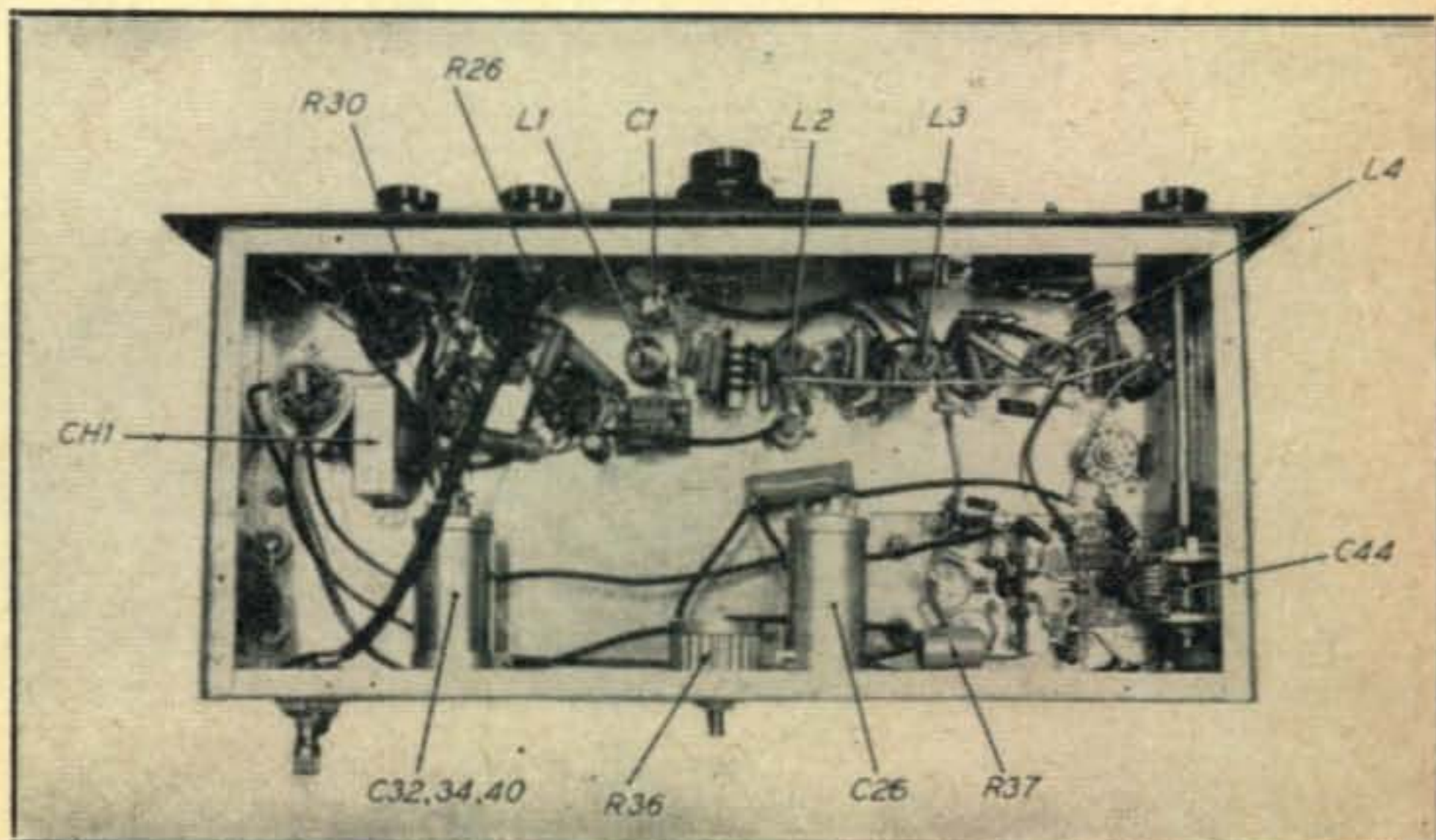
Fig. 3. Underneath the chassis. There are no cramped corners and the parts are located largely as convenience dictates, keeping in mind the necessity of separating the r-f input and output circuits to avoid feedback.
