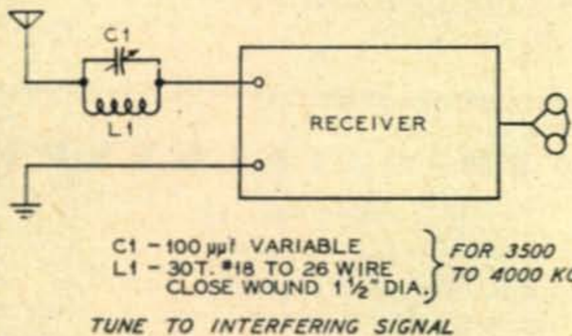
Fig. 3. Simple wave trap for decreasing strength of nearby interfering signals.
