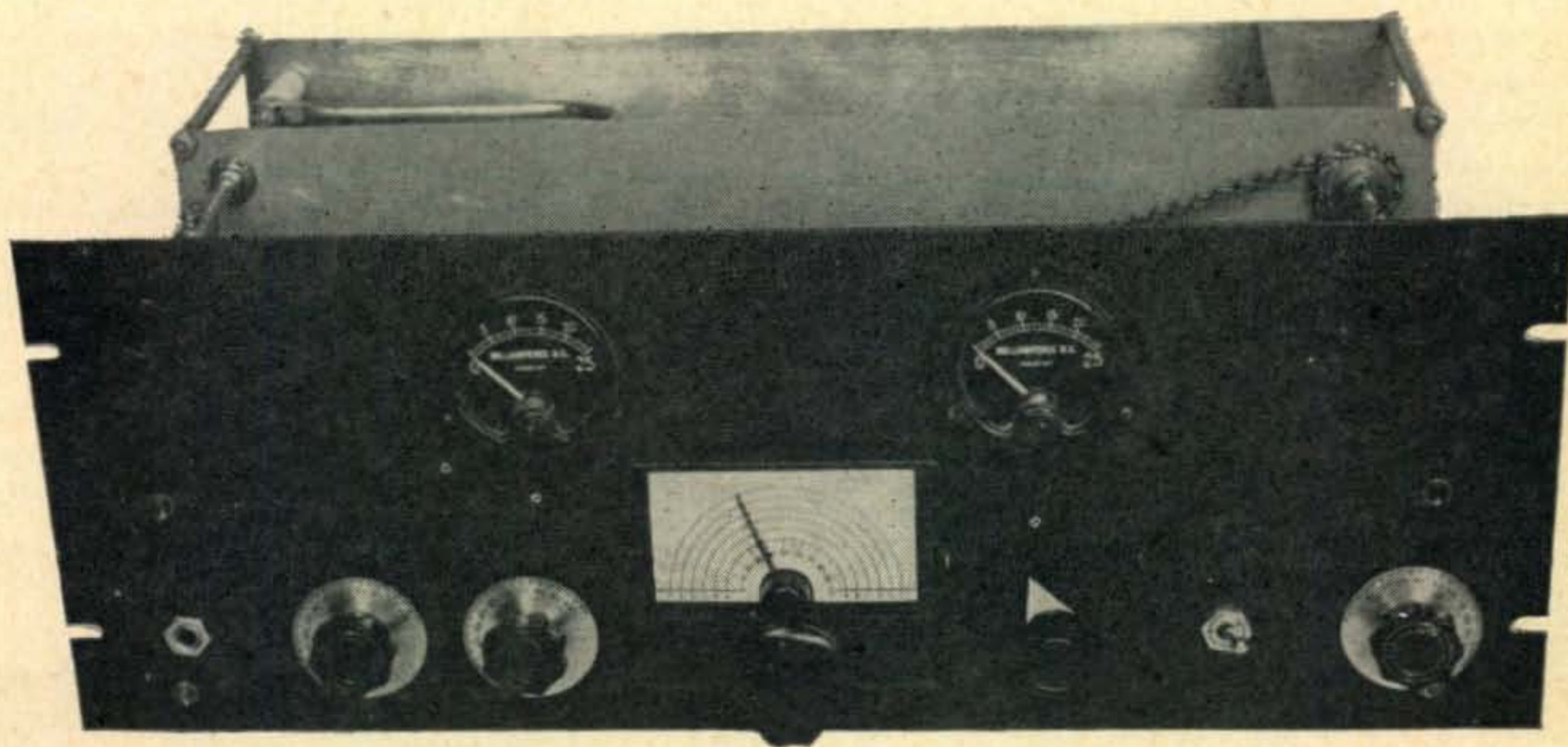
Fig. 1. Front view showing front panel layout. Although the left-hand meter has only a 25 milliampere scale, a 10X shunt is used providing 250 milliampere operation.
