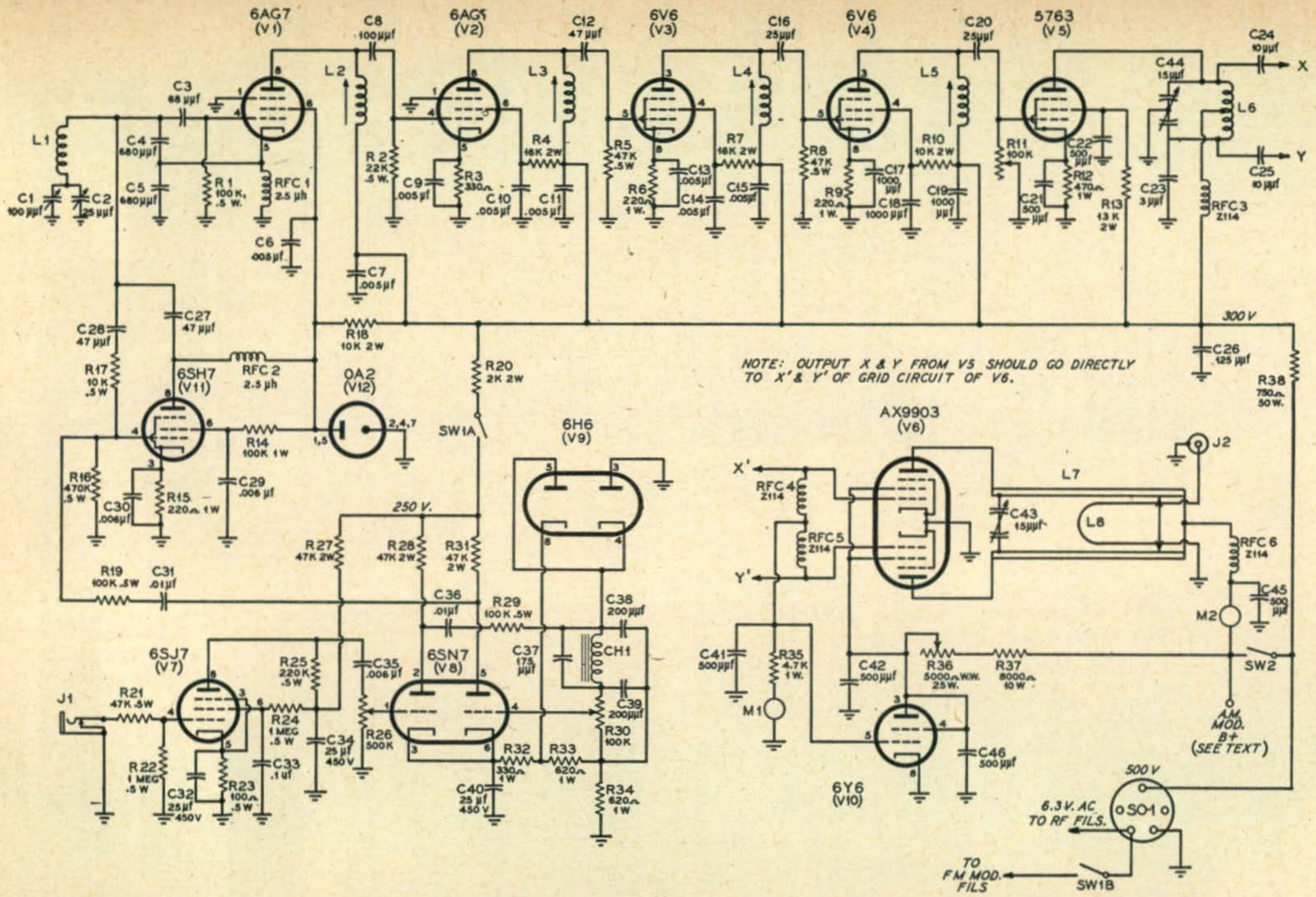
Circuit diagram for the VFO controlled 100 watt two meter transmitter.
