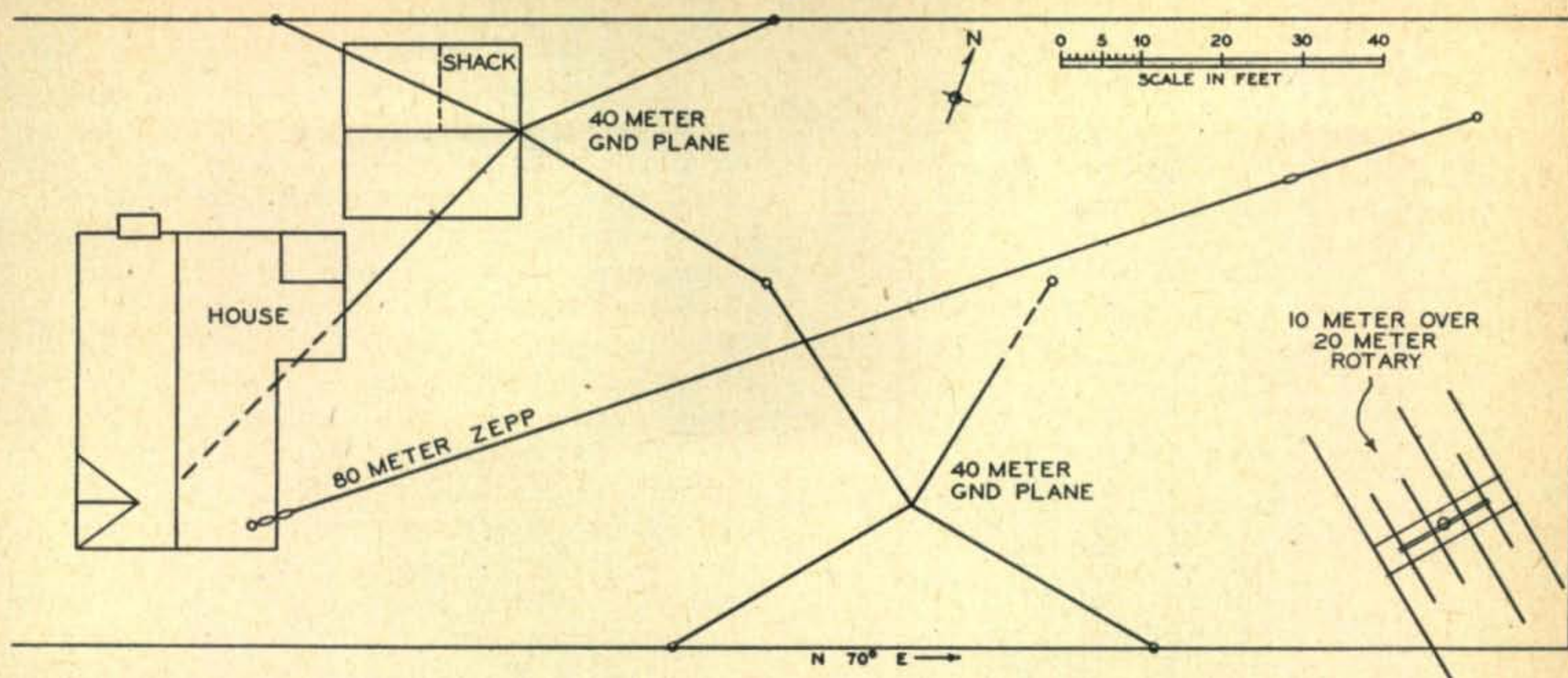
Fig. 2. A view of the W6MVQ antenna layout.
