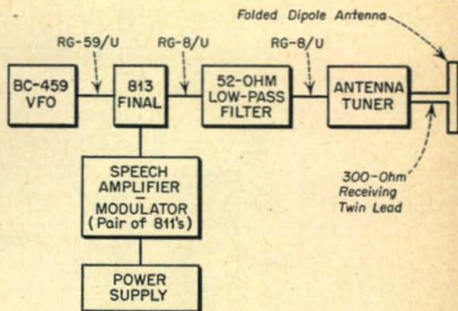
Block diagram of the transmitter.
