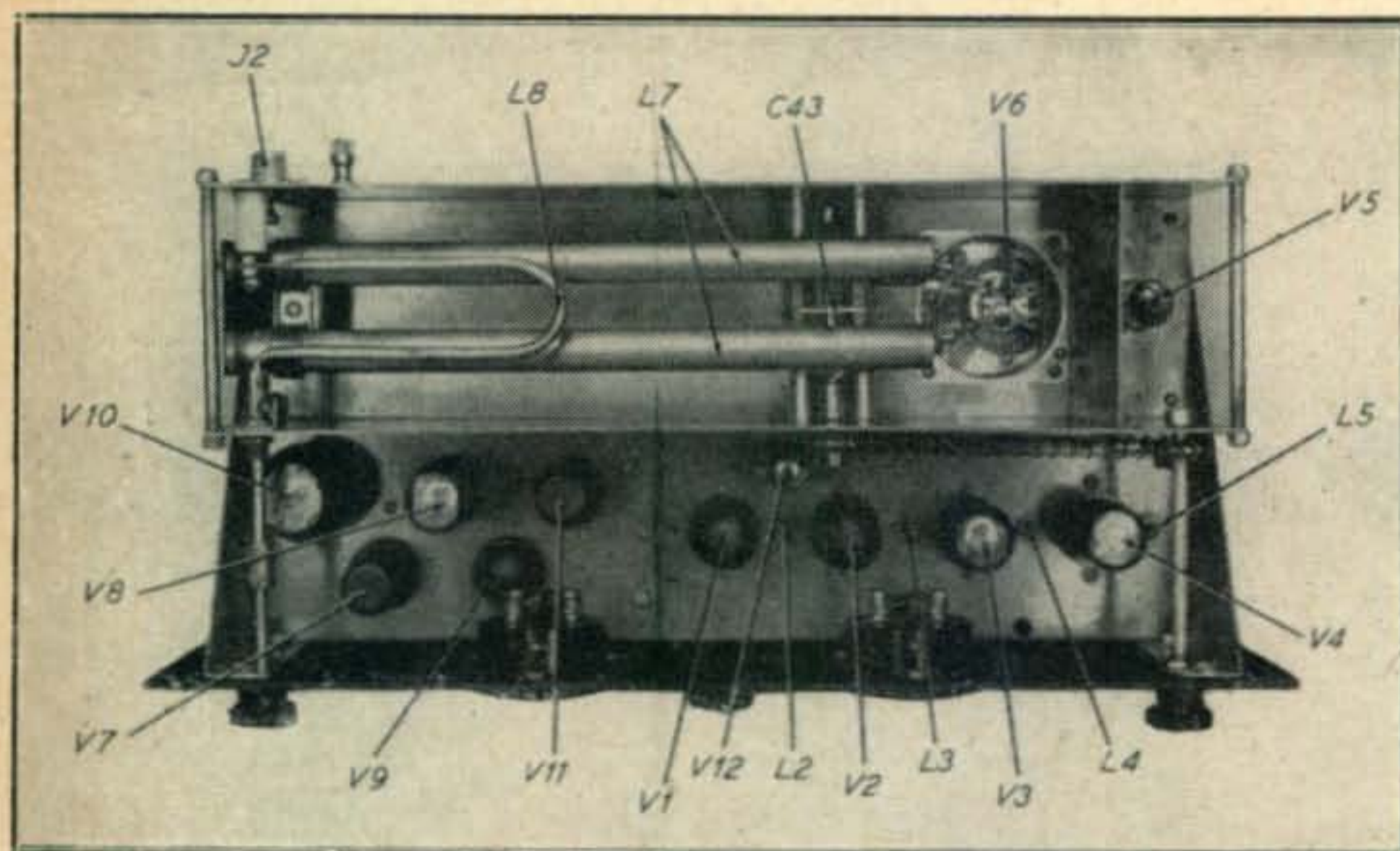
Fig. 2. Top view of chassis showing efficient use of space. Note the chain drive arrangement for tuning the final amplifier plate circuit and the antenna pickup coil arrangement.
