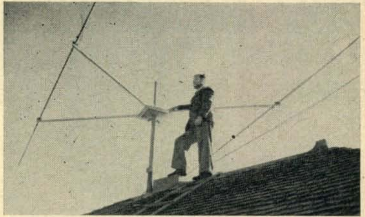
Don, VK2NO surveys the terrain from the rooftop of VK2CM. The beam is a two-element rotary of the G8PO type which is somewhat like the 8JK except that it has electrically reversible phased elements for a controllable front-to-back ratio.
