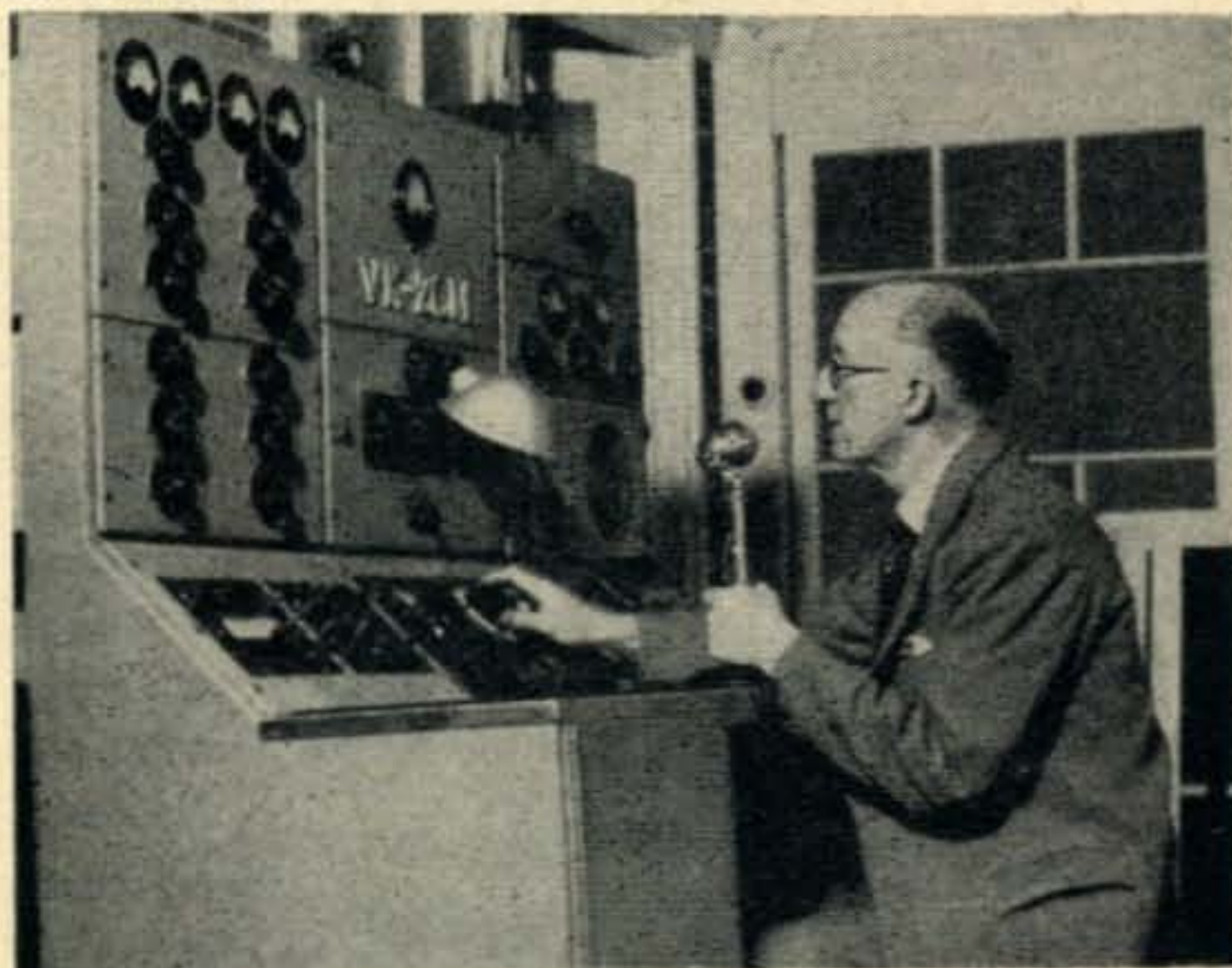
This is the No. 1 Australian amateur; Charles D. Maclurcan, VK2CM as seen in his 1953 shack. The receiver is a National HRO and to the left are the 6-meter converter and "R9-er." Below the meters on the top left section are separate finals for the transmitters which vary from 807's to 829's and 813's. Class AB2 807's are used in the modulator. A surplus "Command" unit is built into the right-hand panel as a VFO from 80 through 10 meters.
