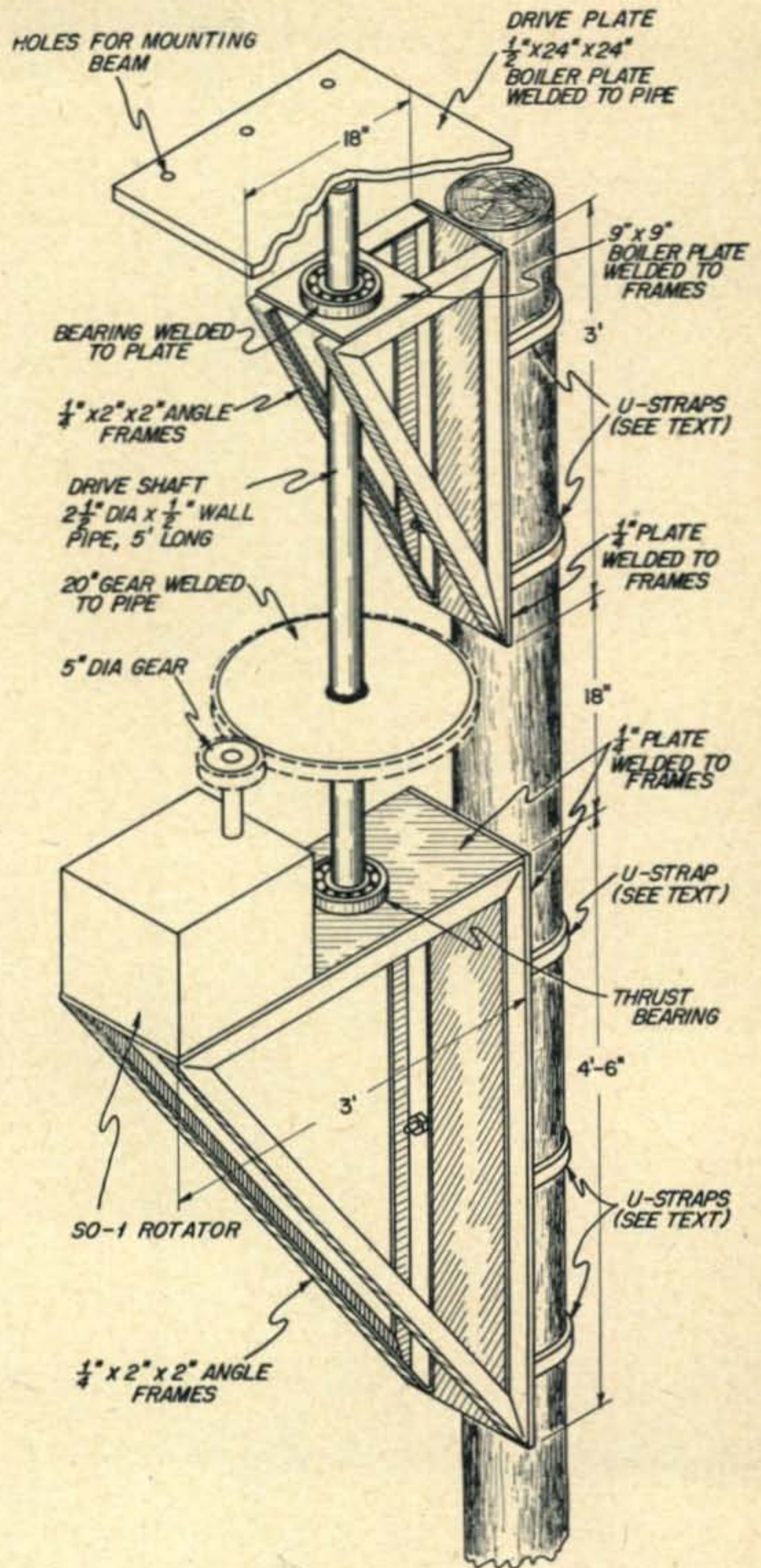
Fig. 4. Construction of the platforms to support the rotator, shaft bearings and drive shaft. All principal metal joints are welded.
