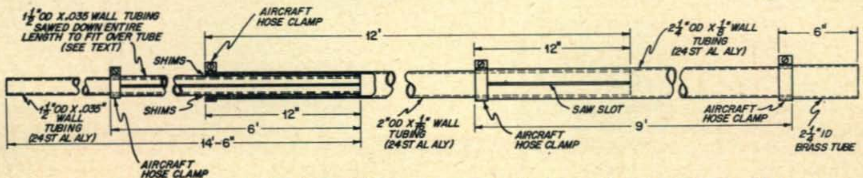
Fig. 3. In order to obtain the rigidity necessary at 40-meters, the elements should be constructed as shown above. This is one side of the radiator. The director/reflector does not have the six-inch brass tube at the right, but is continuous and unbroken.
