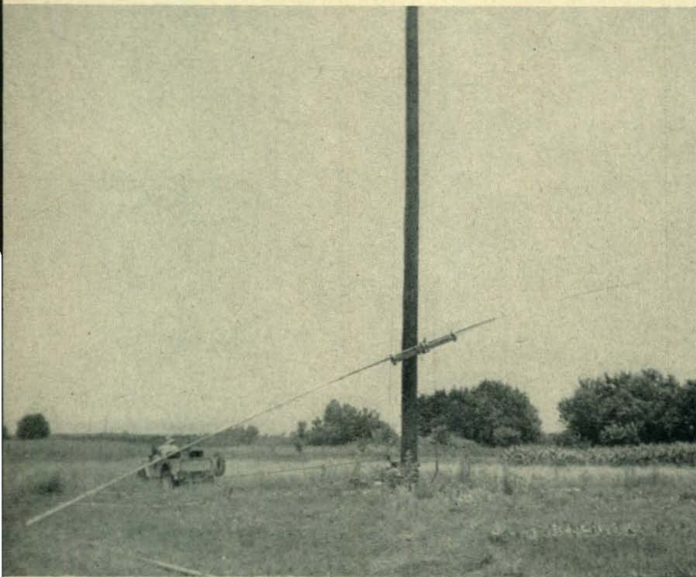
Figure 5: This picture serves the dual purpose of showing the construction of the sixty-seven foot, self-supporting element and the method of getting the various components to the top of the telephone pole. Hal, W9LM, is driving the Jeep. John, W9APE, is perched on top of the pole, thirty feet above the top of the picture, waiting for the element to reach him.
