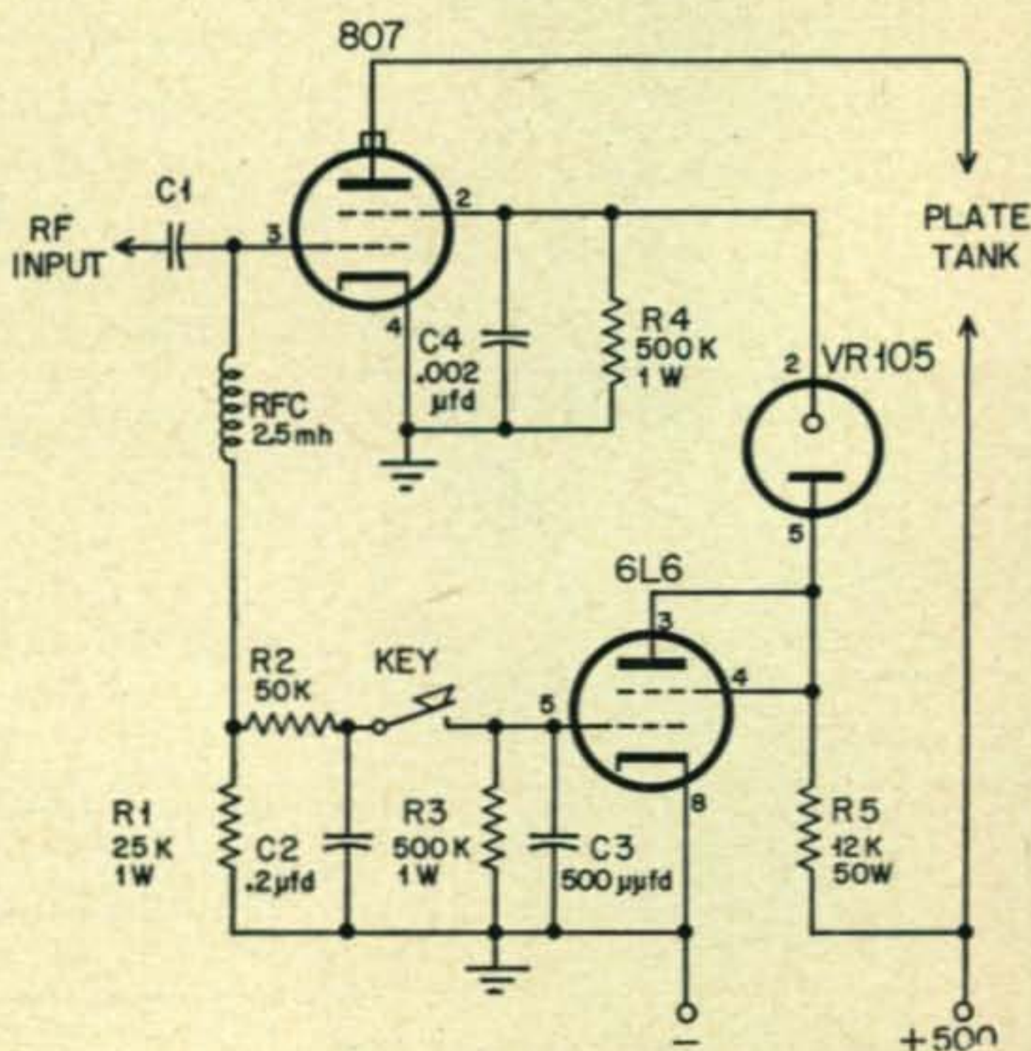
Fig. 1. This is the method of obtaining control-tube bias from the amplifier grid current. The revised circuit appears on page 63.
