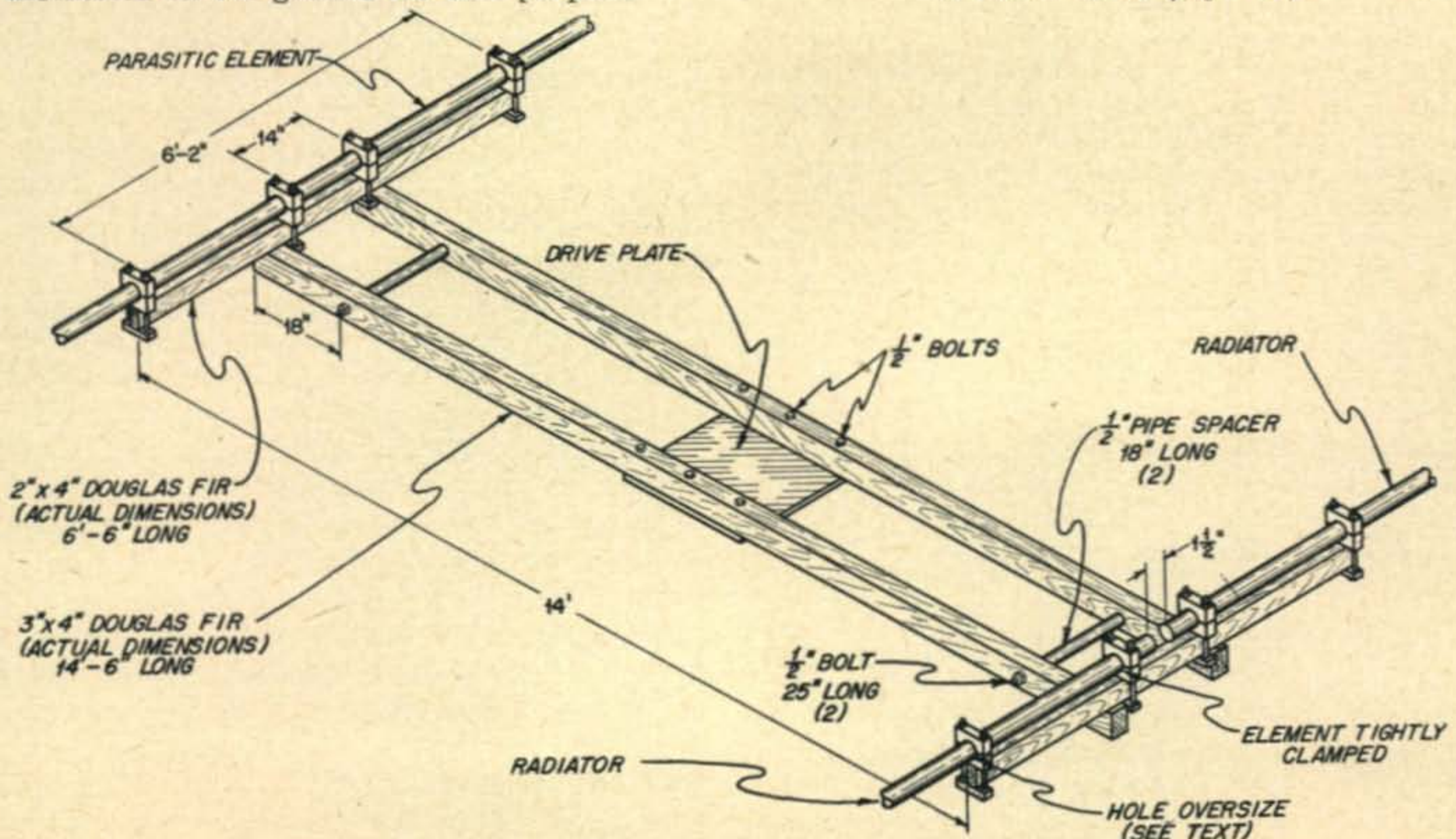
Assembled drawing of the W9LM 40-meter rotary beam antenna. The parasitic element is quite responsive to frequency change. It reacts as director on the low end of the band and as a reflector on the high end of the band.
