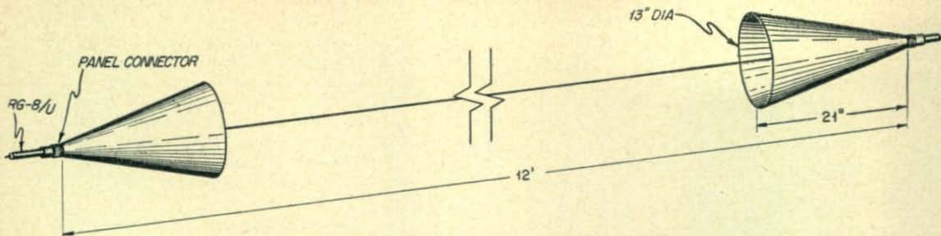
Fig. 1. Working arrangement of a simple "G-String."
