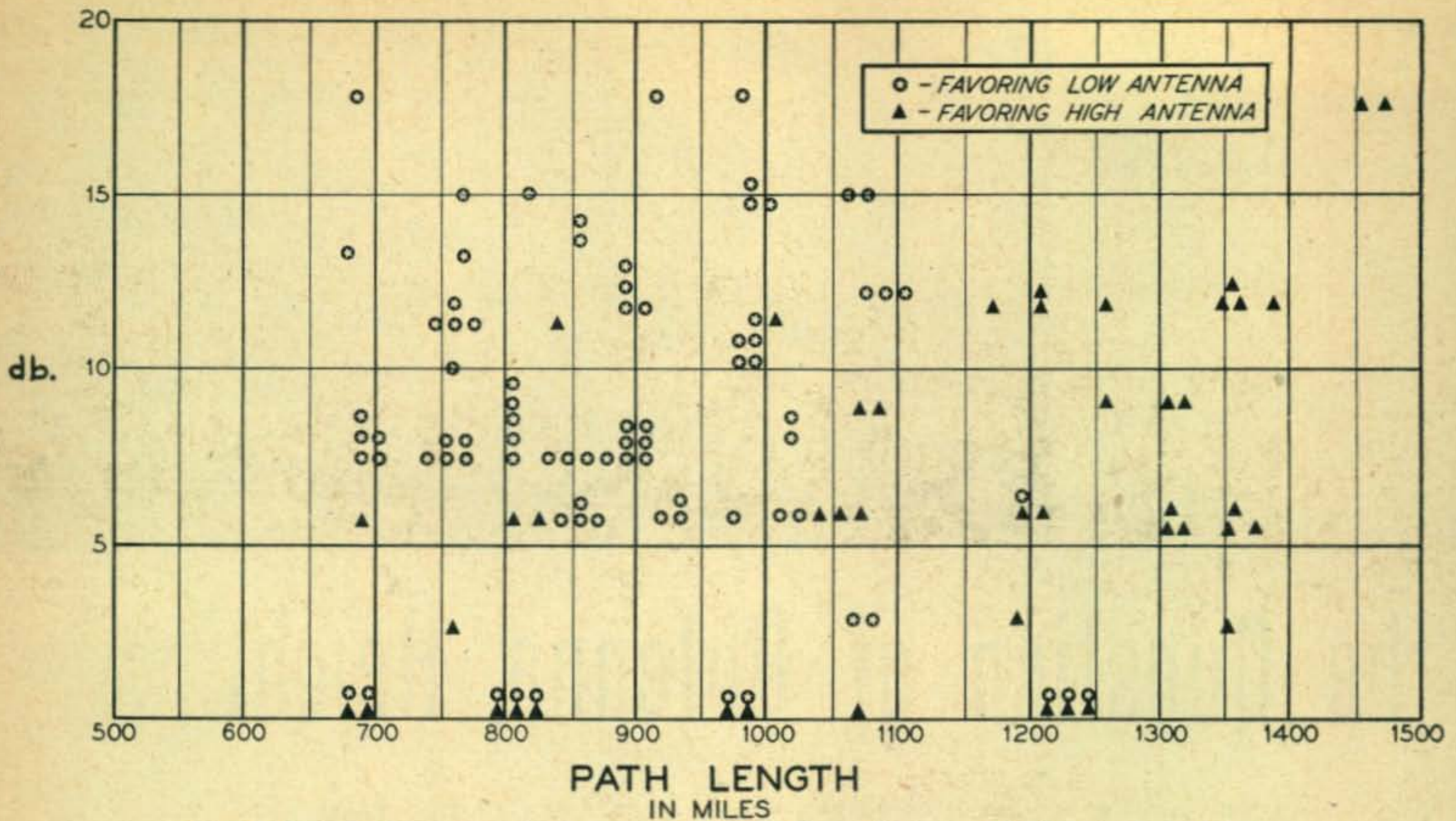
Fig. 2. Rough plotting method used after the mileage between the terminals had been worked out. "Non-standard" reports (i.e., observations favoring the high antenna in the predominantly low antenna readings) may be due to a change in layer height.
