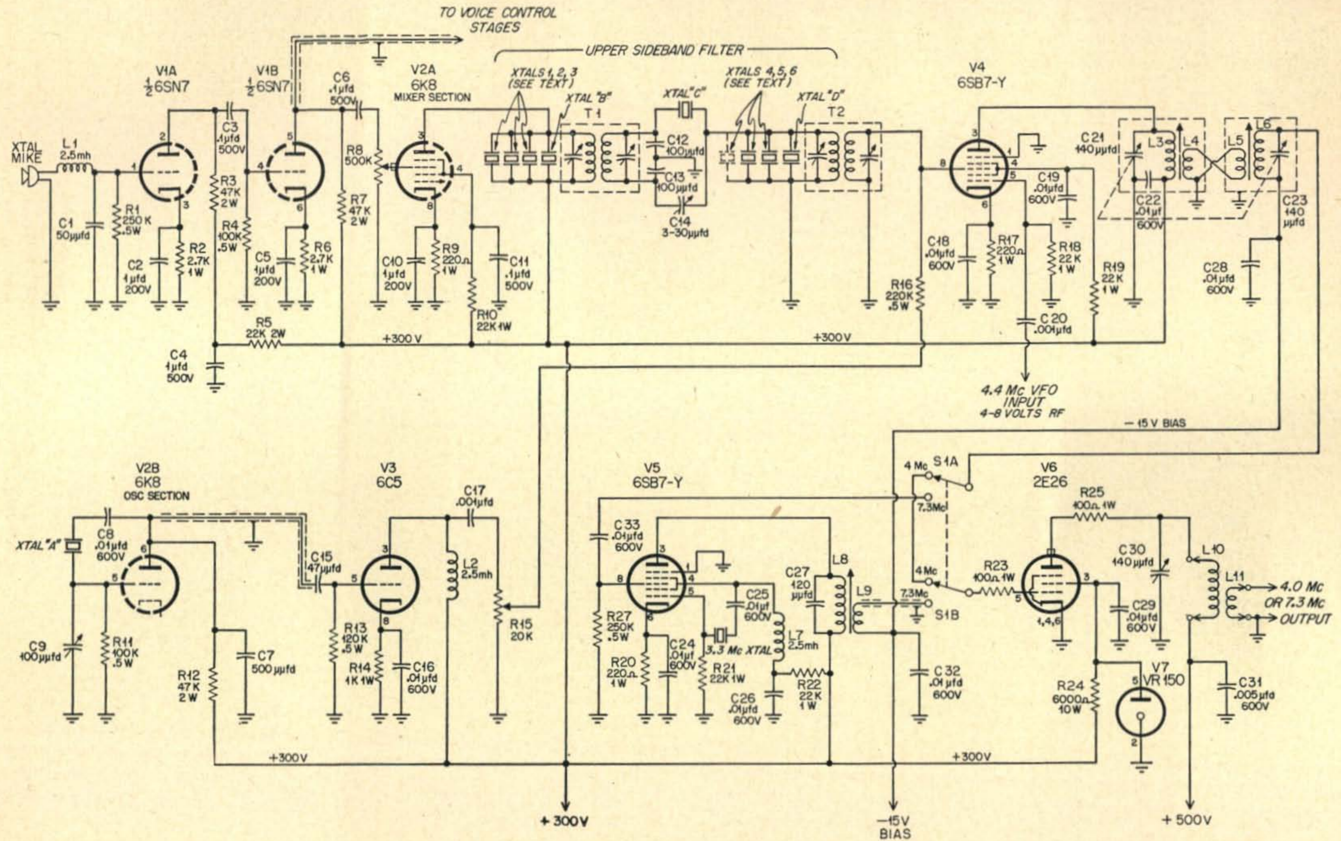
Fig. 2. This is the two-band crystal-type single-sideband exciter as modified by W2MTJ from the original design by WIJEO. The text describes how the modifications in the filter will improve the sideband suppression characteristics by about 15 db.
