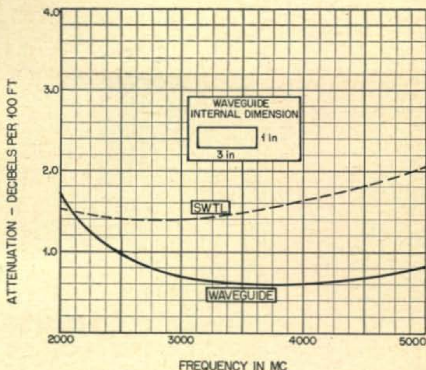
Fig. 5. Comparative curves of the attenuation in a standard copper wave guide, plotted as a function of frequency, versus attenuation in a "G-String."
