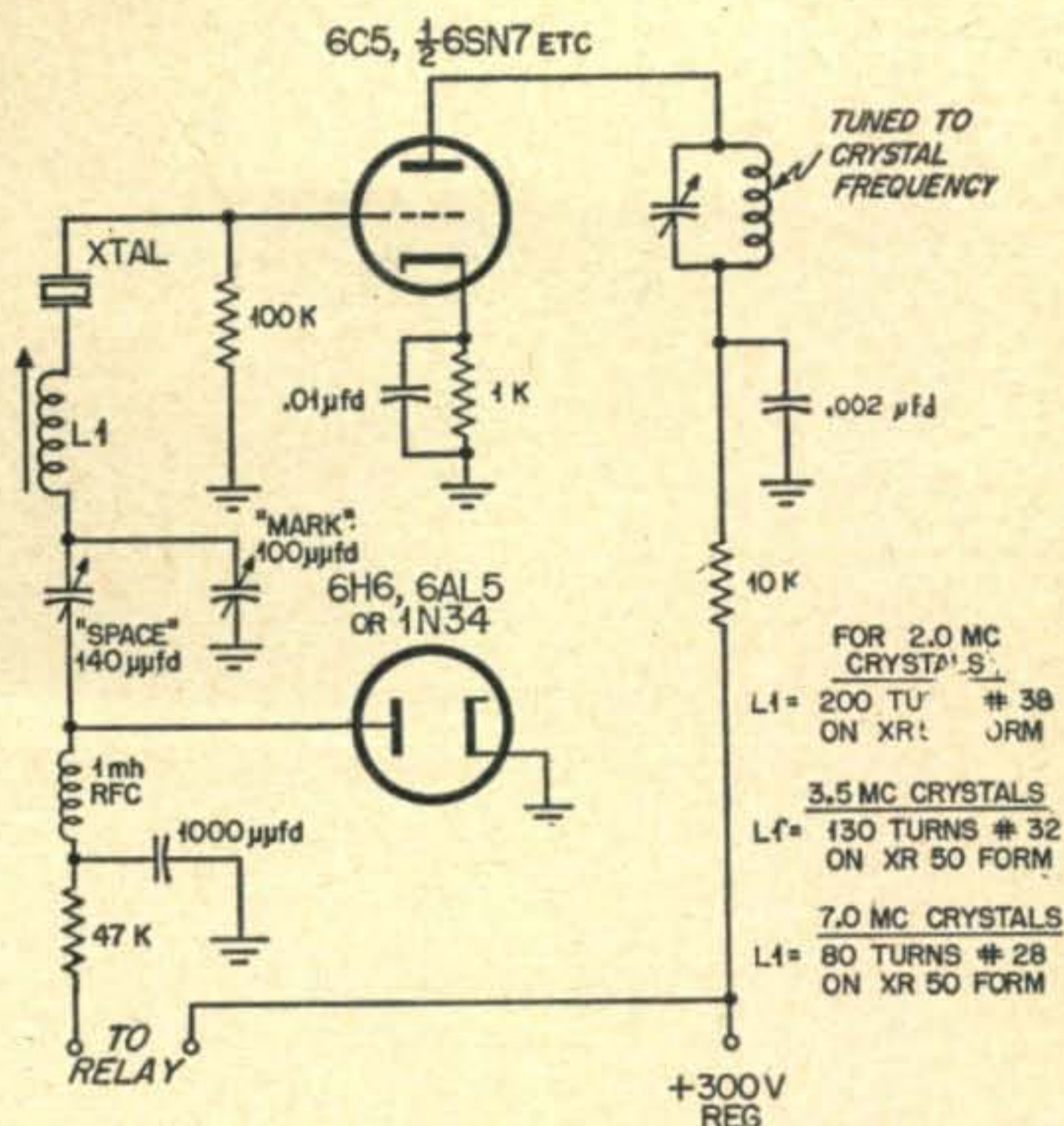
Fig. 2. The W4OLL crystal stretcher circuit.
