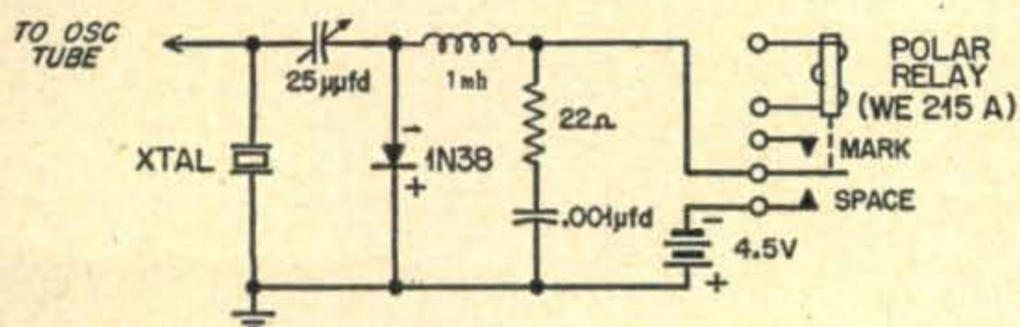
Fig. 1. W6ITH's crystal-crystal f-s-k circuit.
