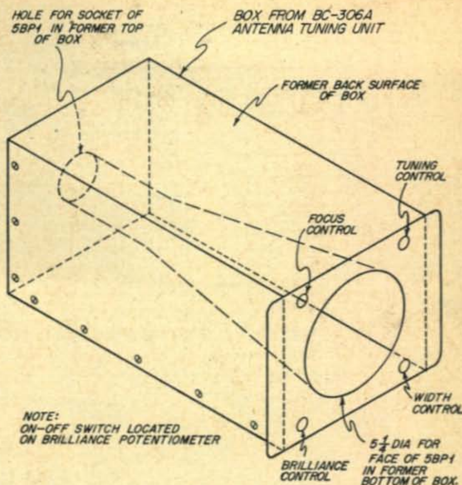
Fig. 3. This is the approximate layout using a surplus cabinet from a BC-306A unit.
