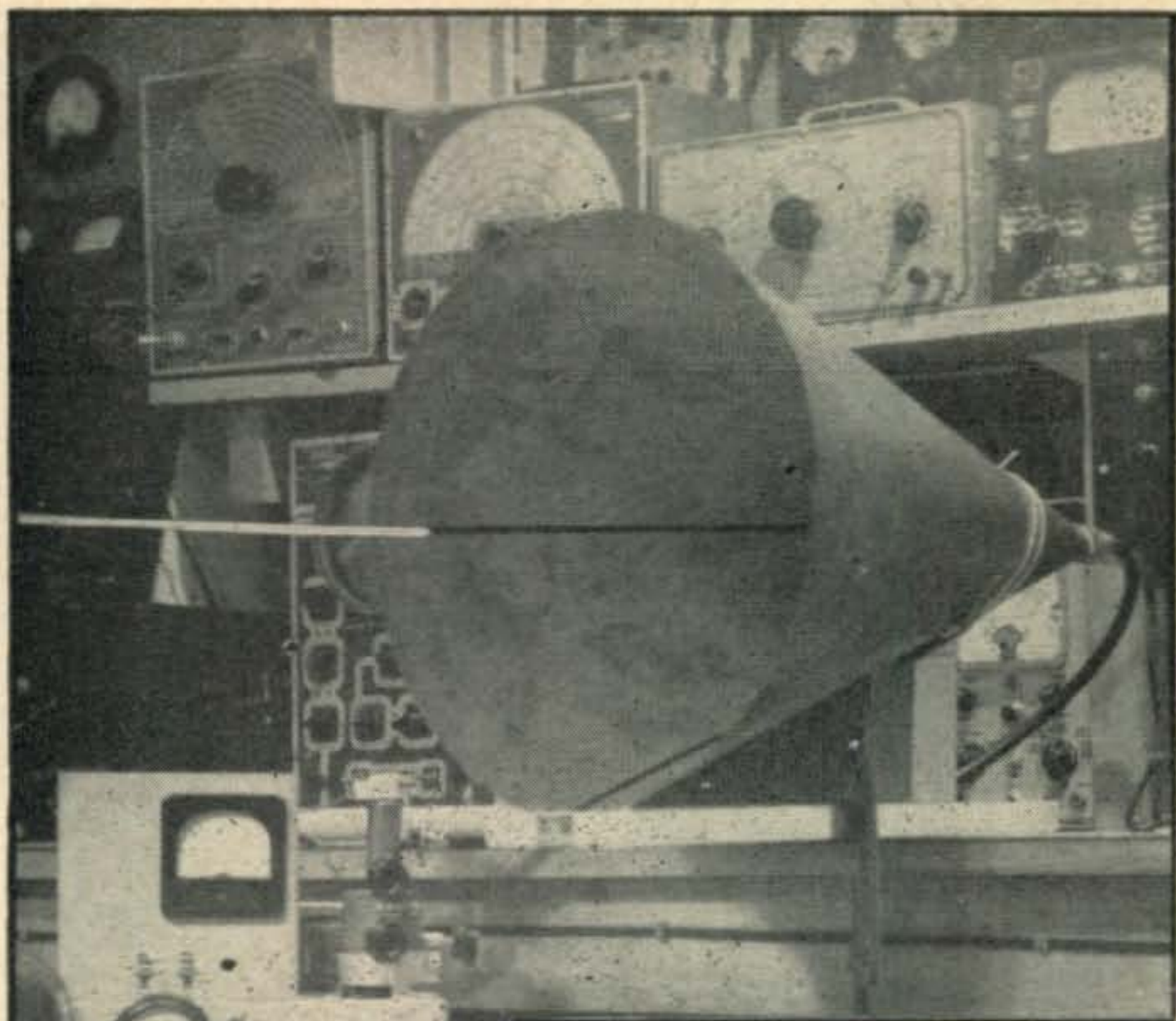
Fig. 2. Experimental setup used by the author showing the u-h-f oscillator connected to one end of a Surface Wave Transmission Line by means of a short length of coaxial cable. Microwaves are effectively "launched" down the center conductor.
