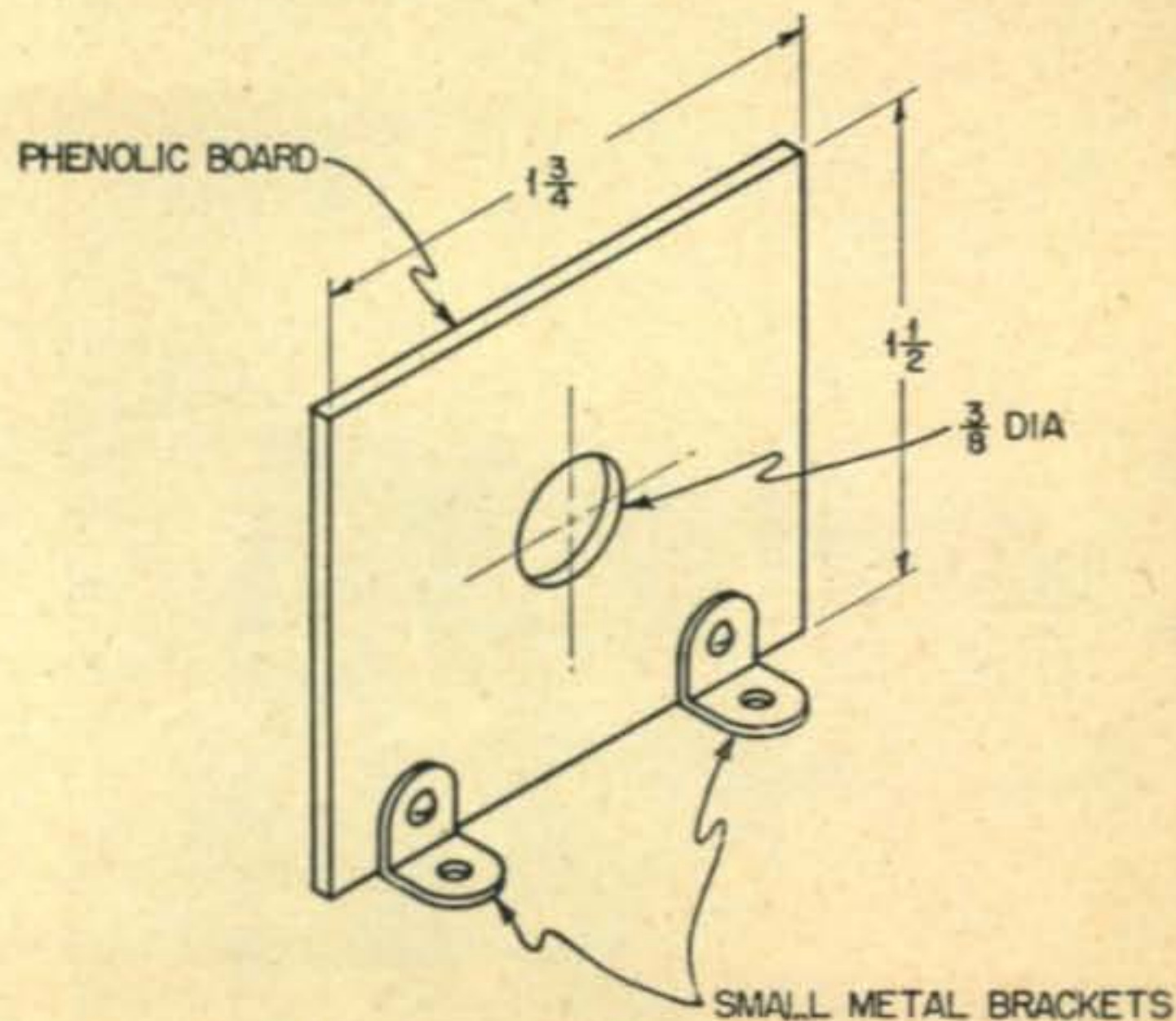
Fig. 4. Insulated potentiometer mounting bracket. If the BC-306A cabinet is used several of these are required for the potentiometers.
