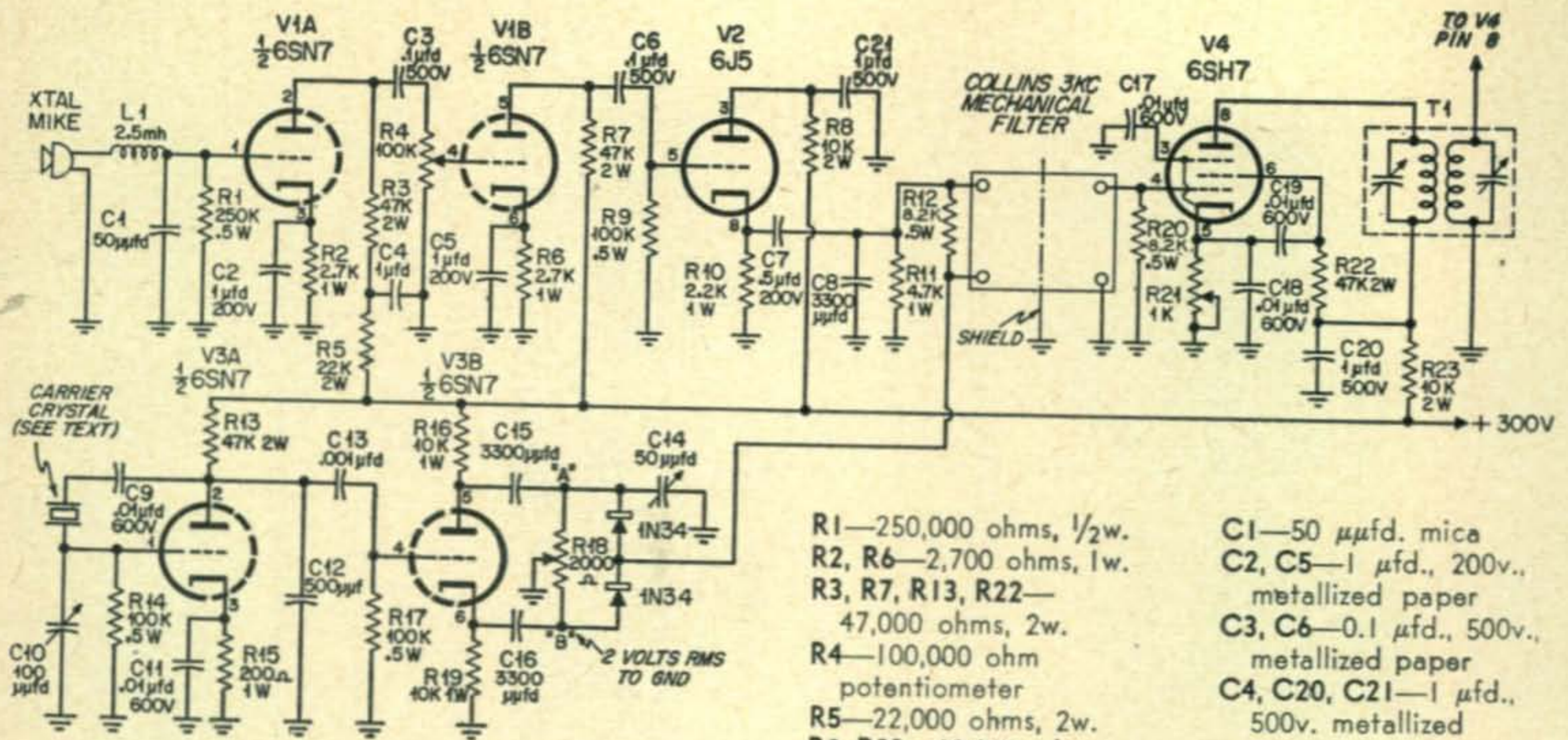
Fig. 3. The exciter shown in Fig. 2 may be adapted to use a COLLINS mechanical i-f filter if the constructor finds the appropriate crystals are not available.
