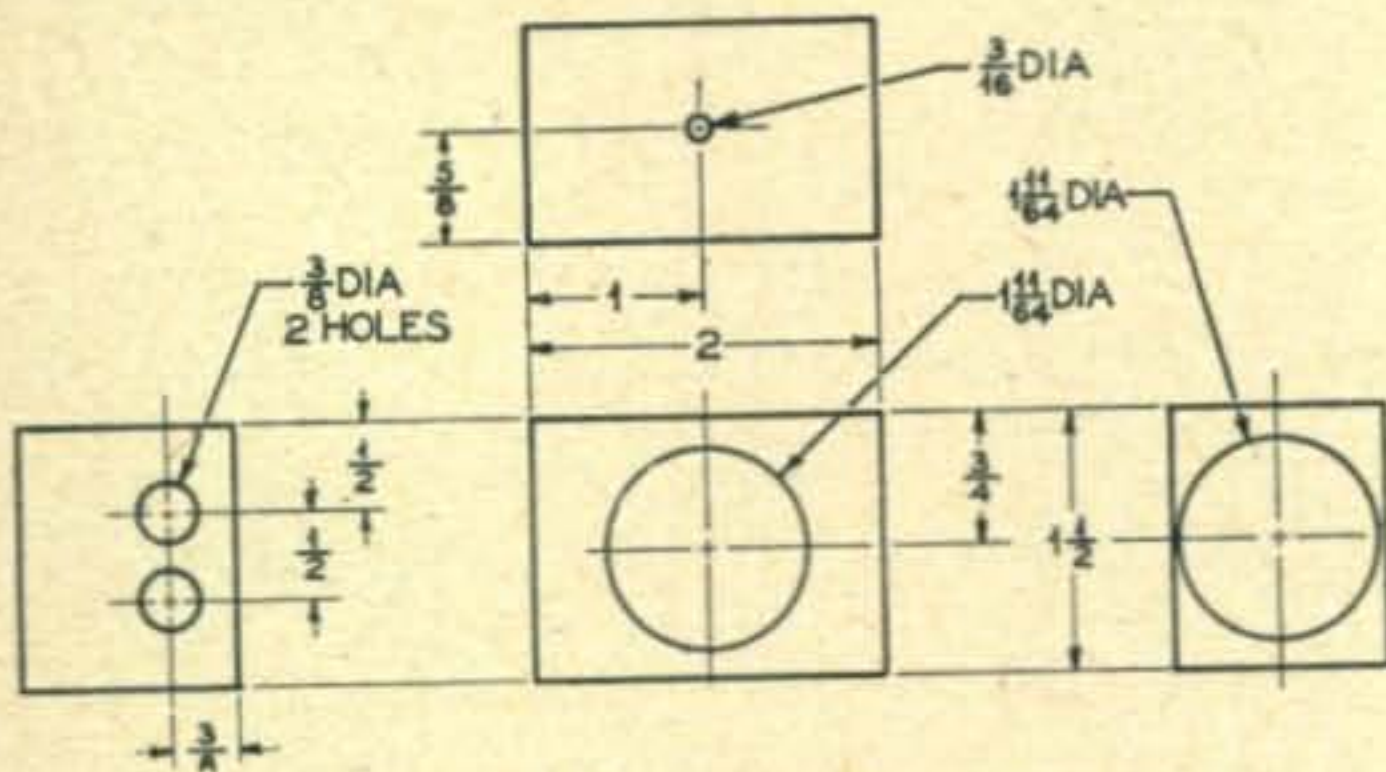
Suggested adapter chassis layout.
