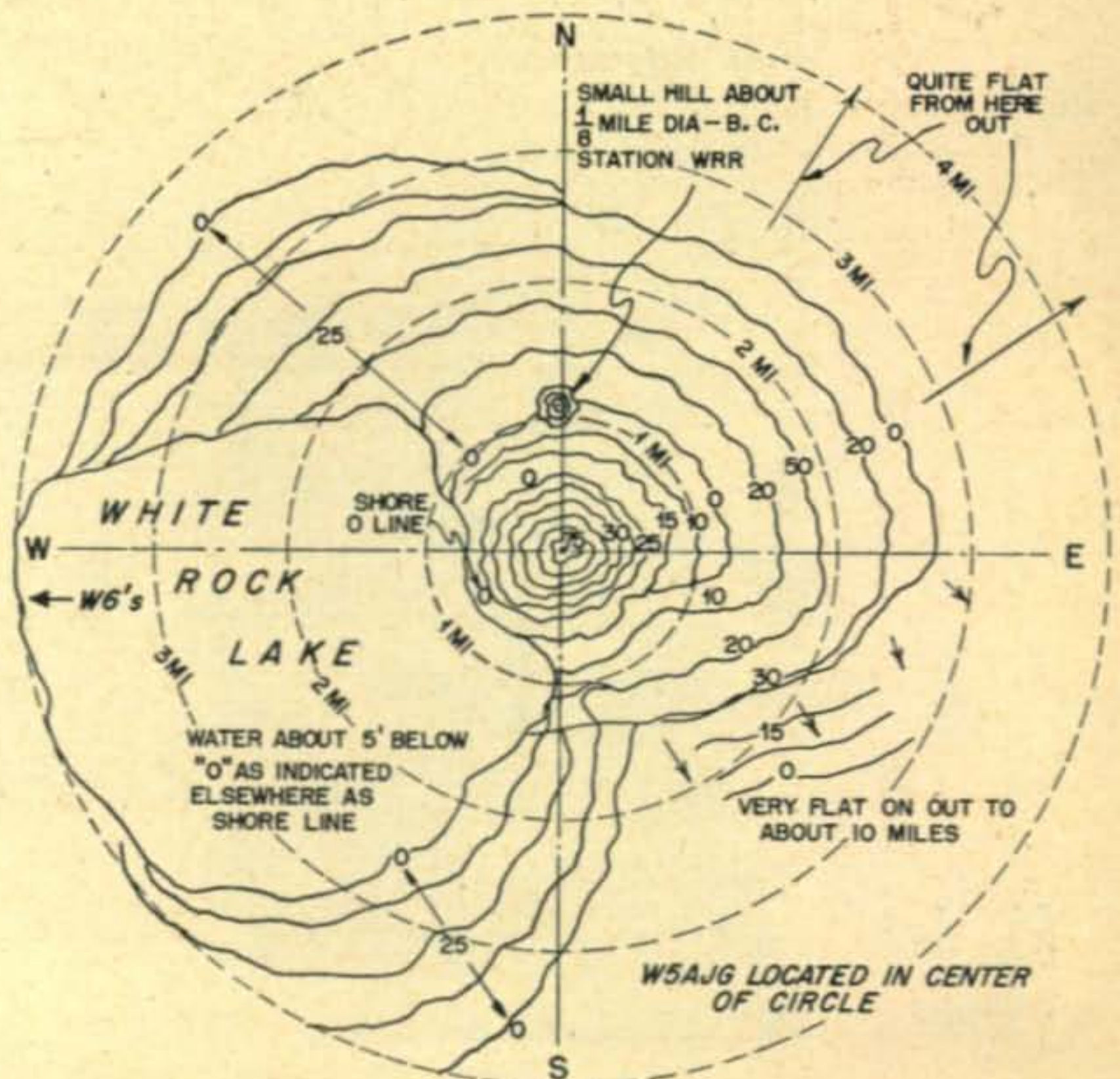
Fig. 1. W5AJG has been fortunate in the choice of a site that is slightly higher than any ground within the first ten miles from the antenna. Most of the skip DX worked on 6 meters has been in the first quadrant (north through east). It is difficult to determine if the lake behind the antenna has any effect on the angle of radiation. The view from the top of the tower shown at the top of this page is towards the west.
