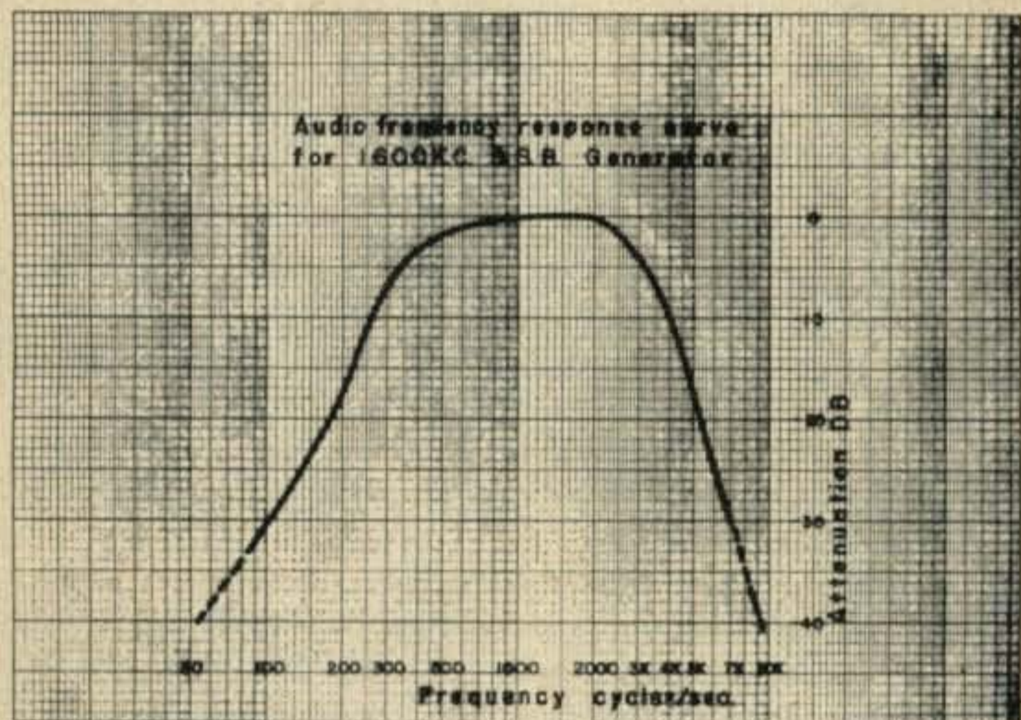
Fig. 8—The audio response curve of the SSB generator described in the article. The text explains how this was plotted.
