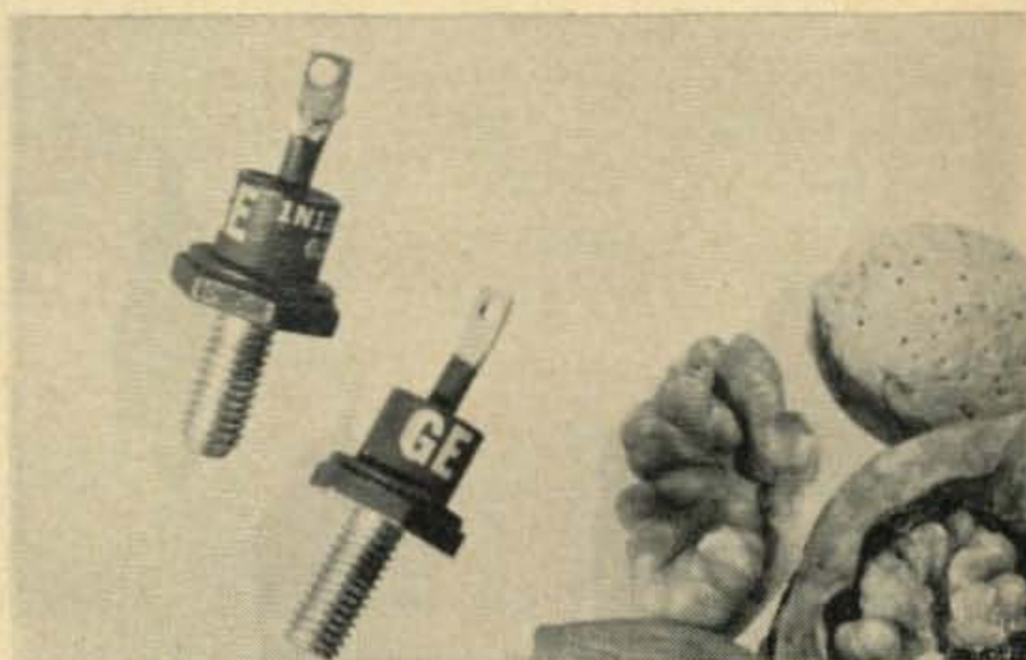
General Electric's new group of 16 medium current silicon rectifiers feature a high temperature hard solder design for maximum thermal fatigue-free operation.
