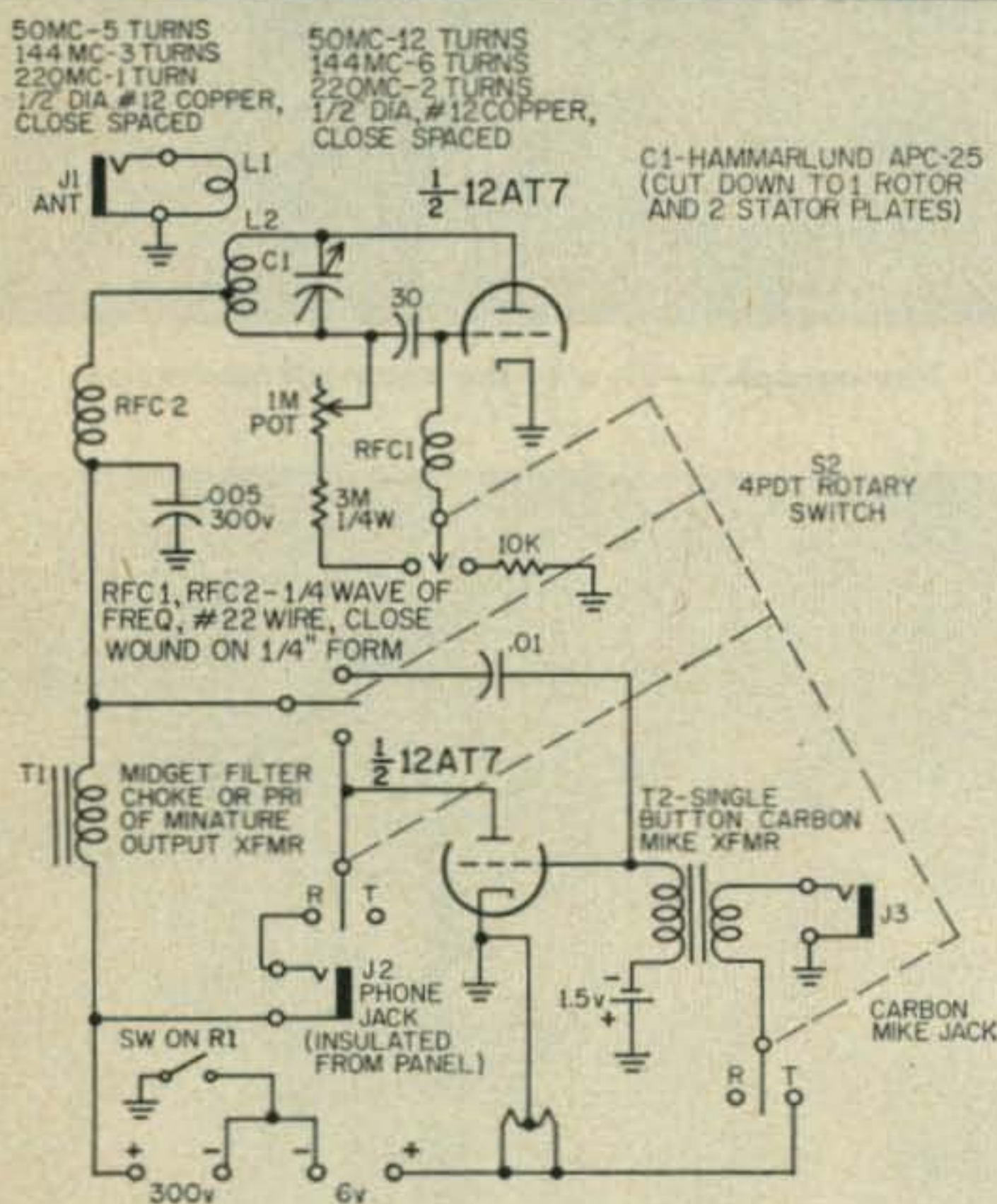
Fig. 1—Circuit of a simple transceiver for 6, 2 and 1 1/4 meters.
