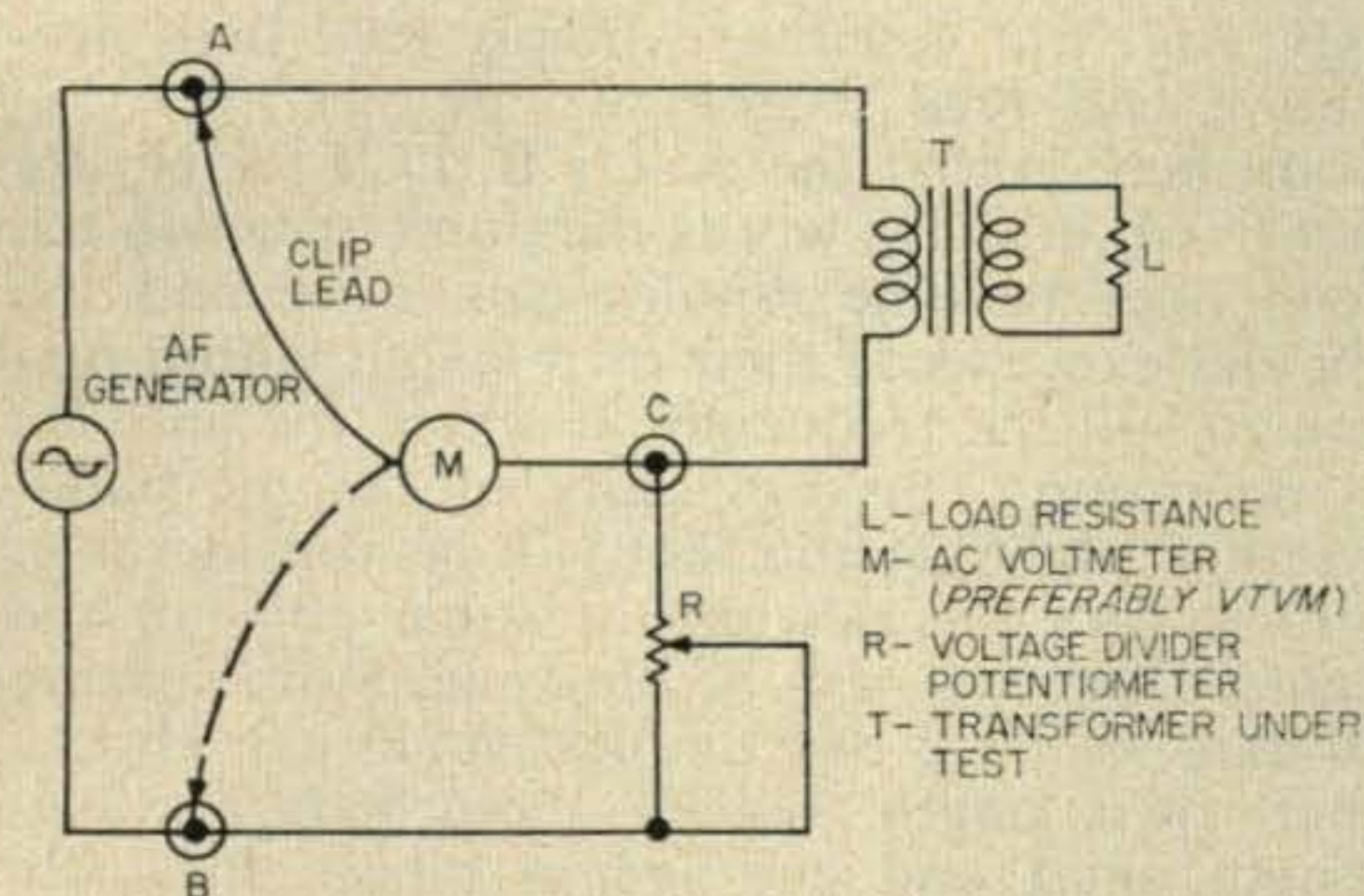
Fig. 1—Schematic of a voltage divider method of determining transformer impedances. See text for a description of L and R .
