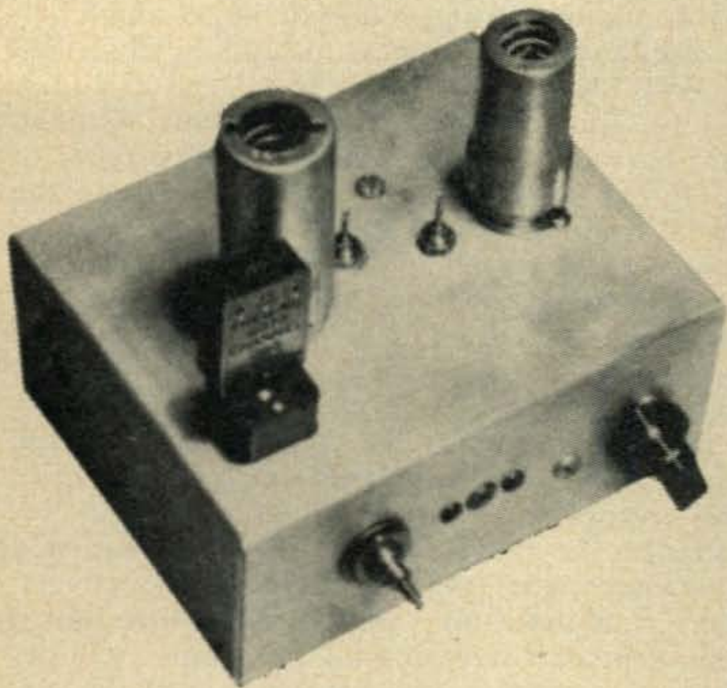
The simple two meter transmitter is built on a standard 2x4x5 inch chassis. At the left on the front is the screwdriver adjustment for L_1 and next to it is C_6 . The knob tunes C_{12} . The screws for tuning L_3 and L_5 are between the tubes.
