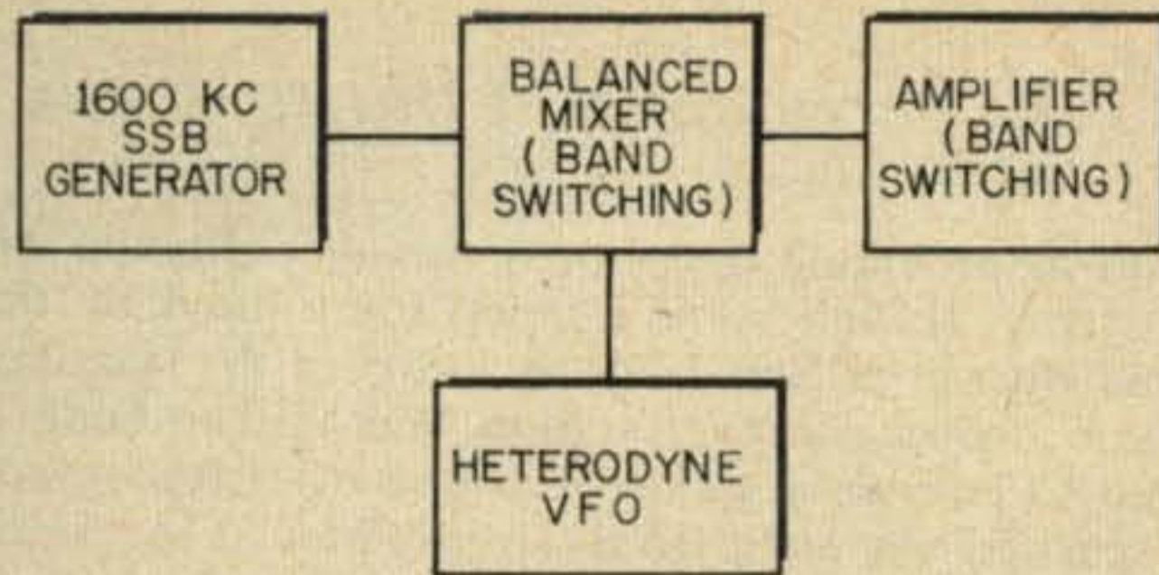
Fig. 9—Block diagram of an all band exciter that may be used with the generator.
