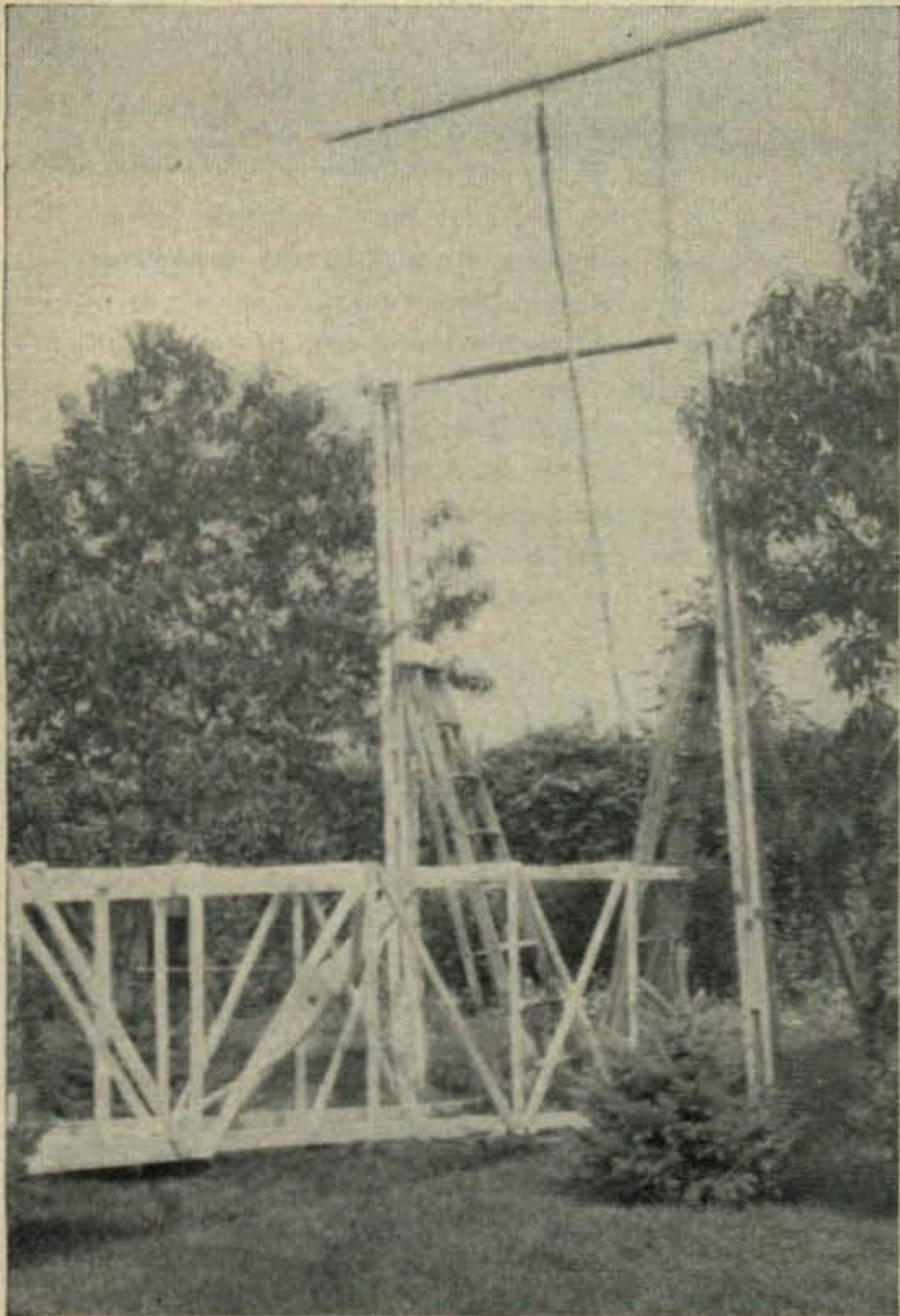
Right—View of the completed tower. Note the marine plywood hinge plate. Tower bottom is loaded with concrete to provide a counterbalance.
