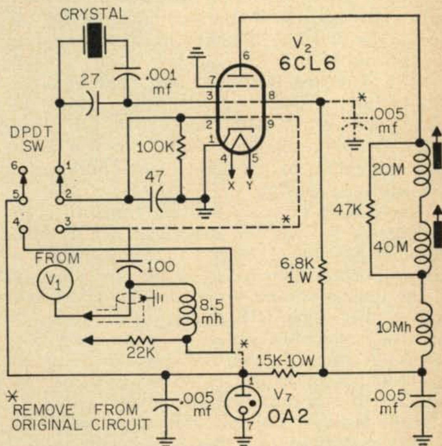
Fig. 2—Circuit modification to permit crystal controlled operation of the Heath MT-1.
