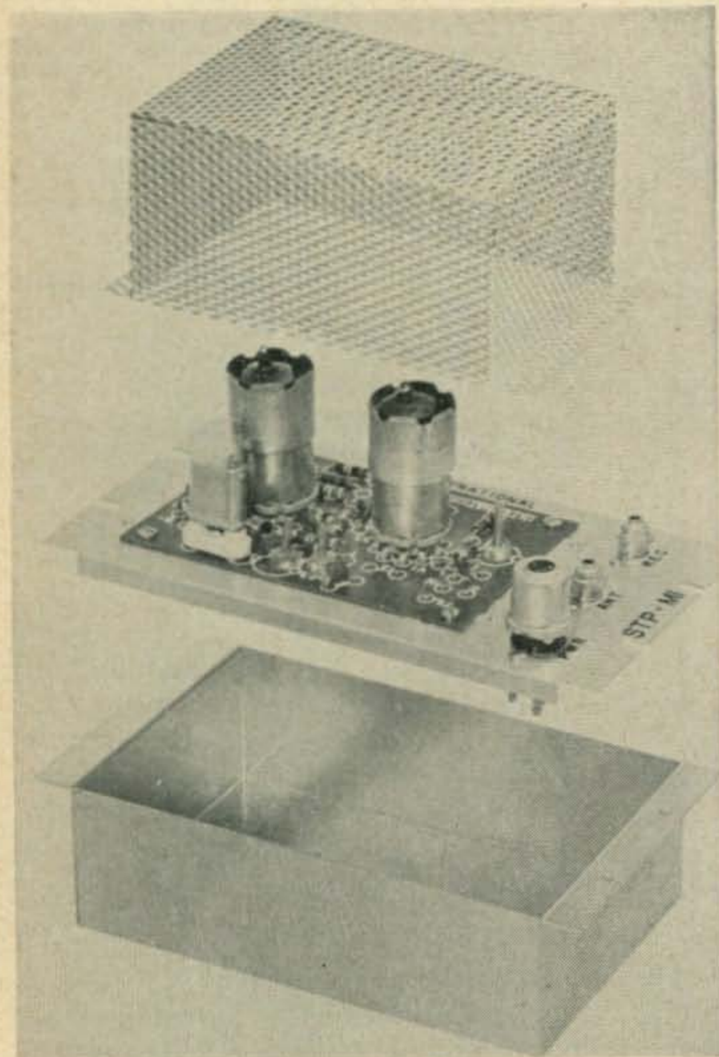
FCV-2 converter and STP-M1 shielded mounting chassis.
