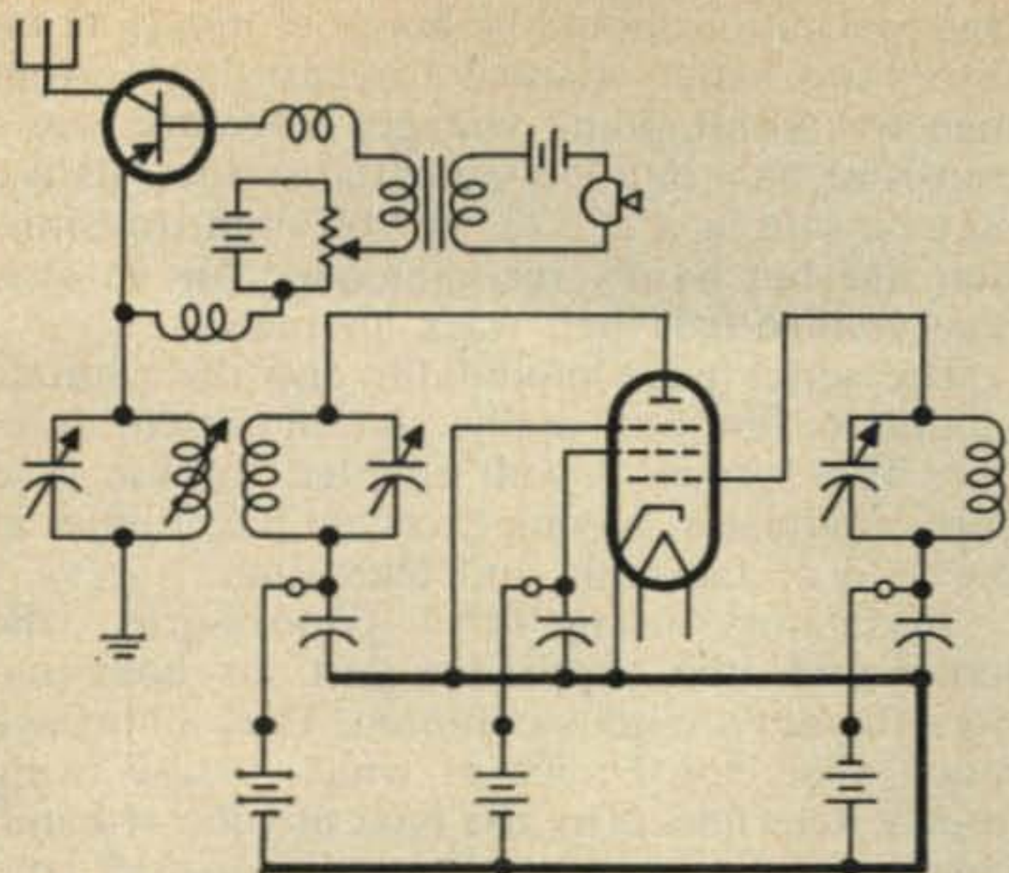
Fig. 3—Transistor antenna modulator. A practical application of this circuit is shown in the Semiconductor Column, December 1959, page 81.
