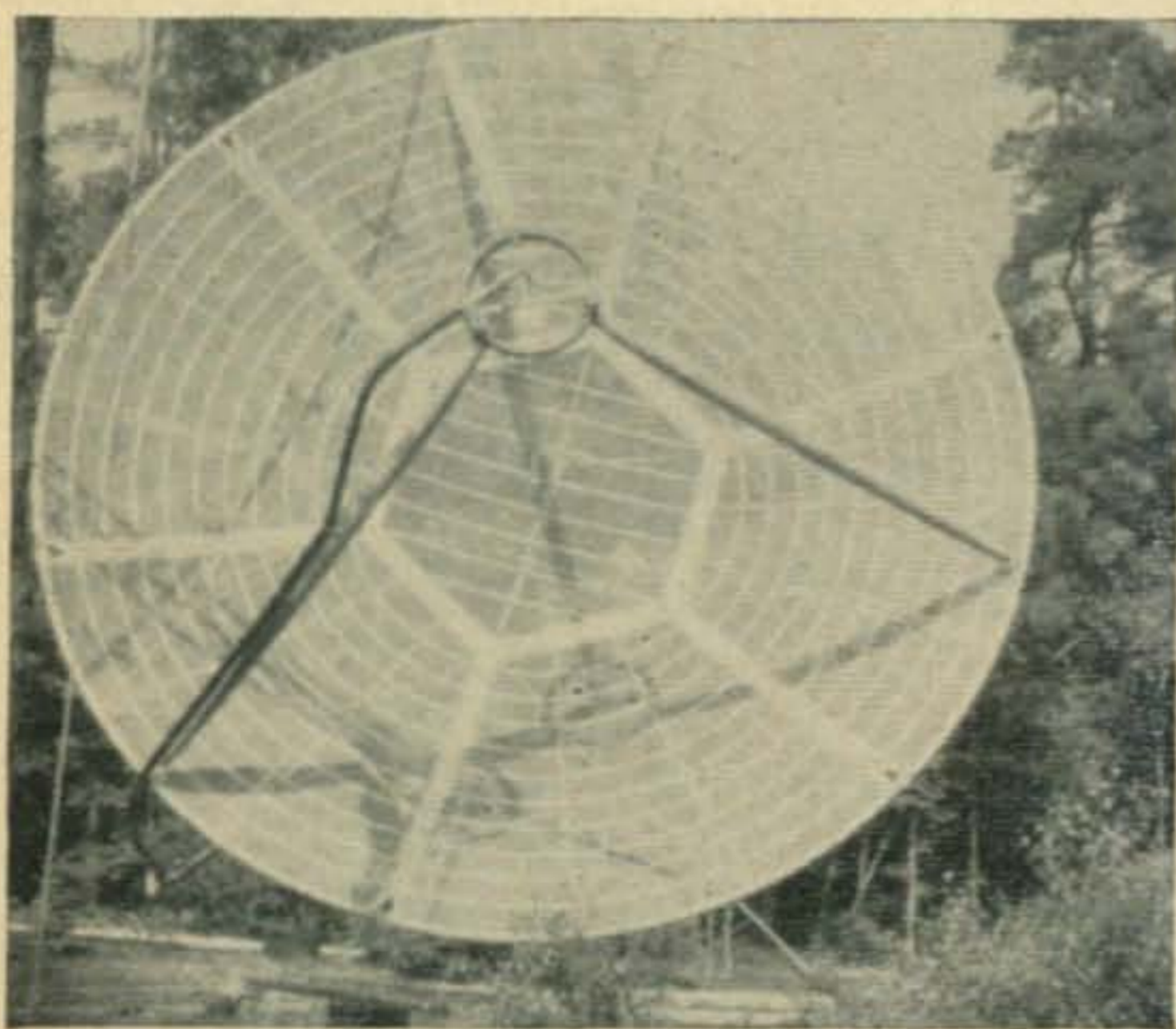
18' parabolic reflector in use at the R.S.V.H.F.S. for 1296 mc Moonbounce project.
