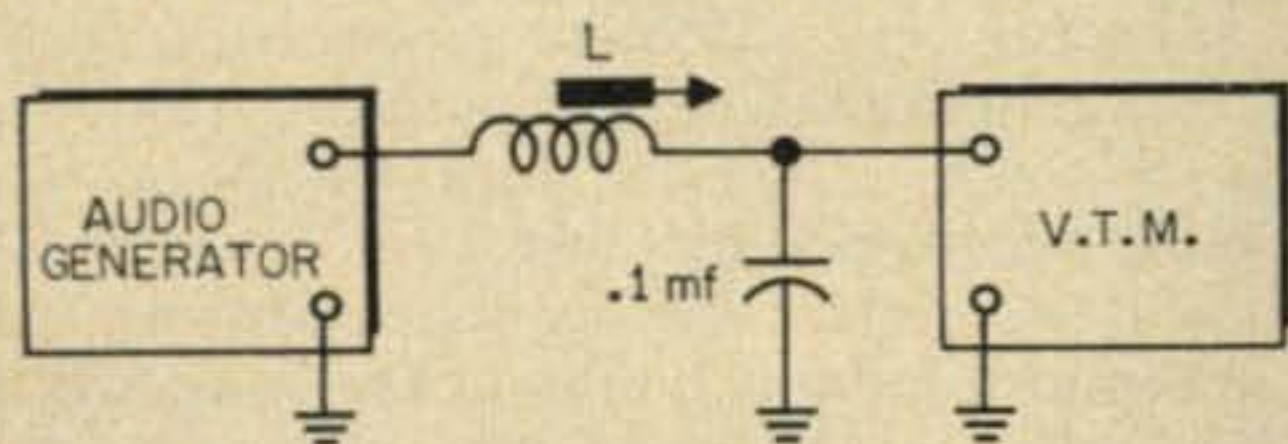
Fig. 6—Test set up used to adjust the inductances in the low pass filter.
