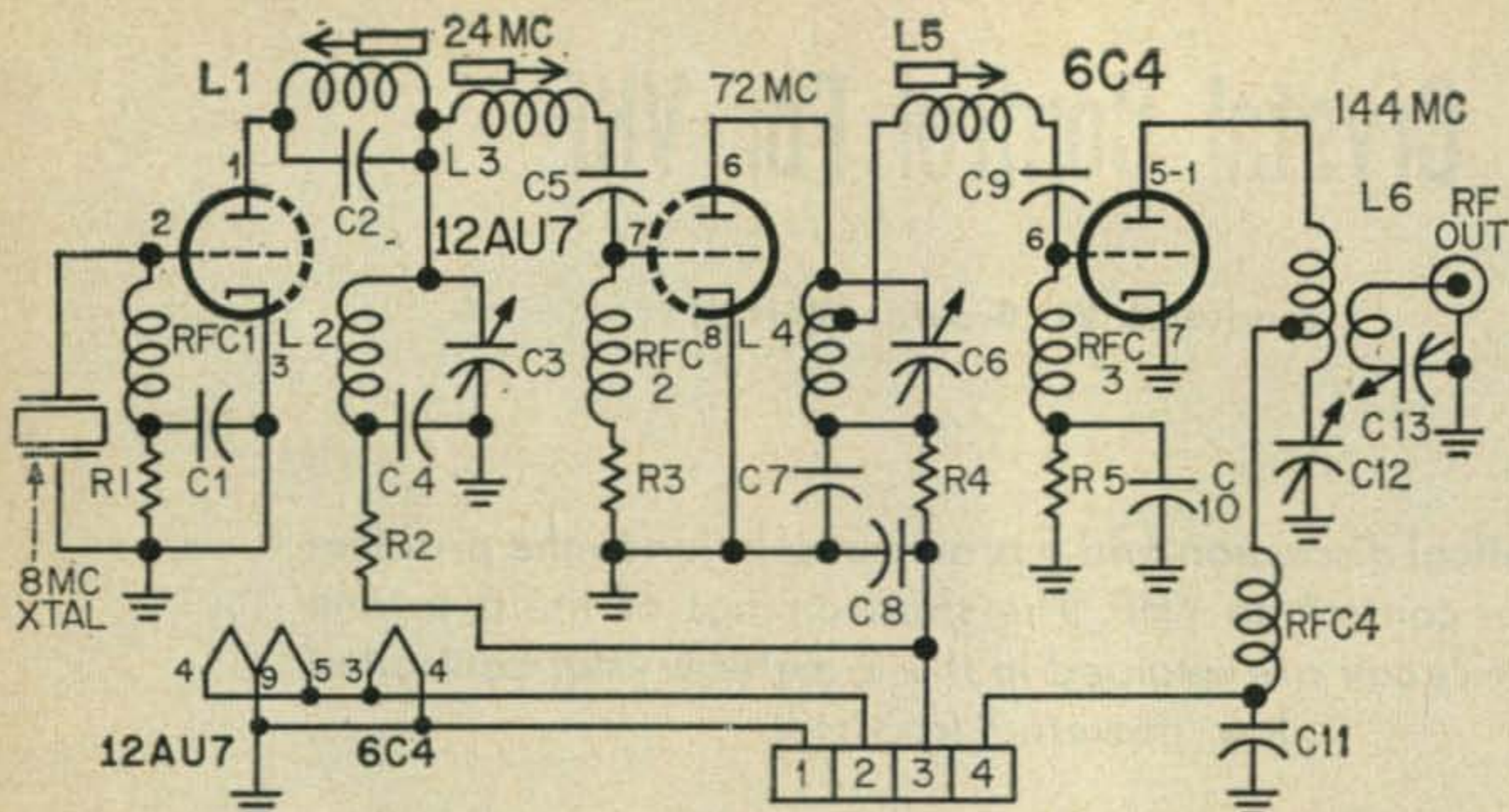
Fig. 1 — Circuit of the low powered 2 meter transmitter. The author used a B+ of 215 volts for all the stages as explained in the text.
