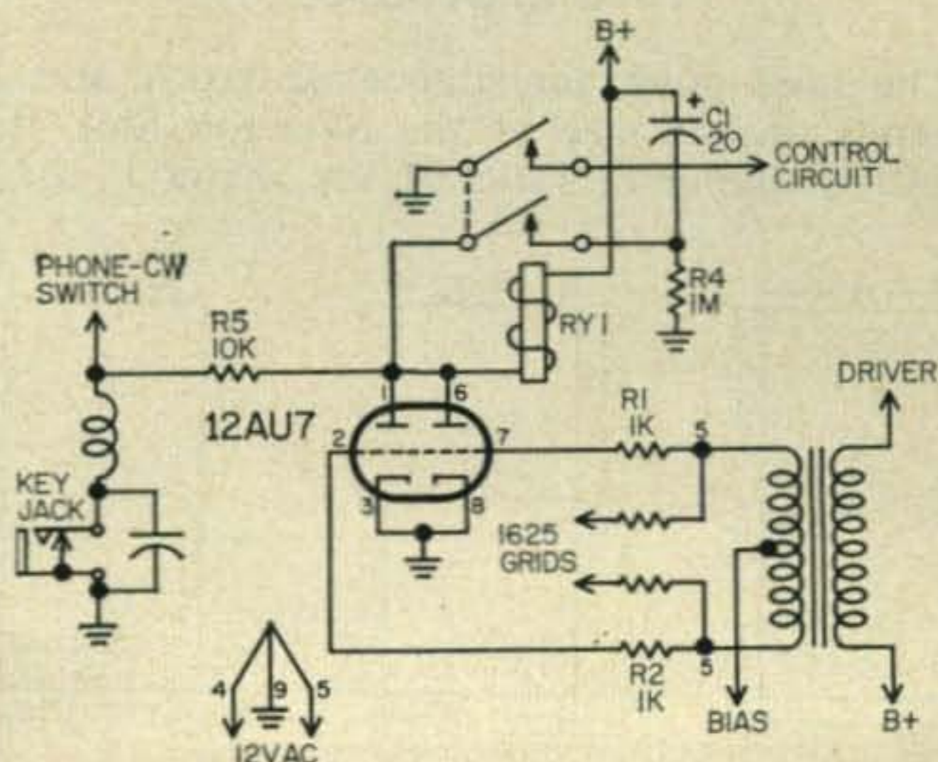
Fig.1—VOX circuit added to the DX-100.
