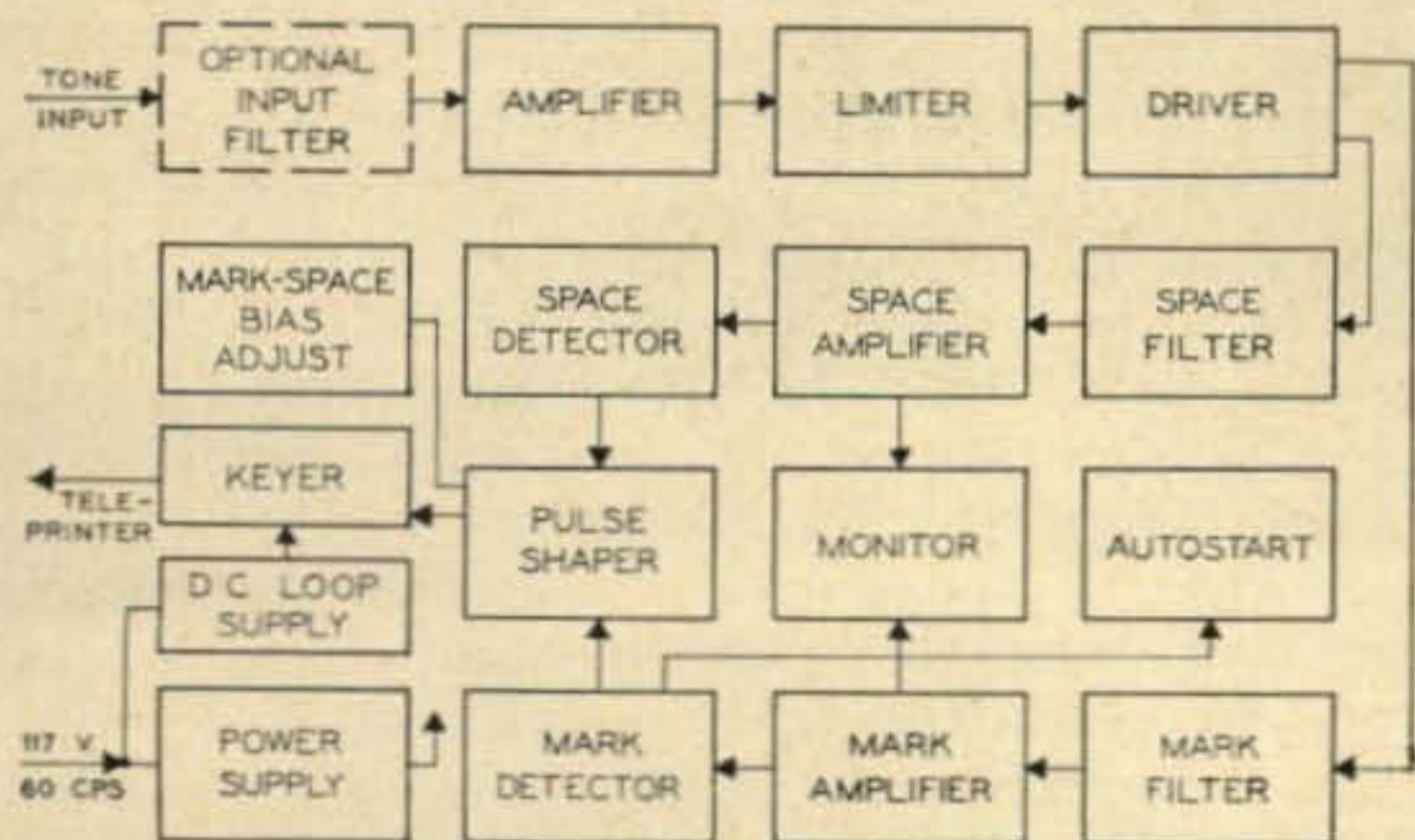
Fig. 1—Block Diagram, Model FSC-250 Frequency Shift Converter.
