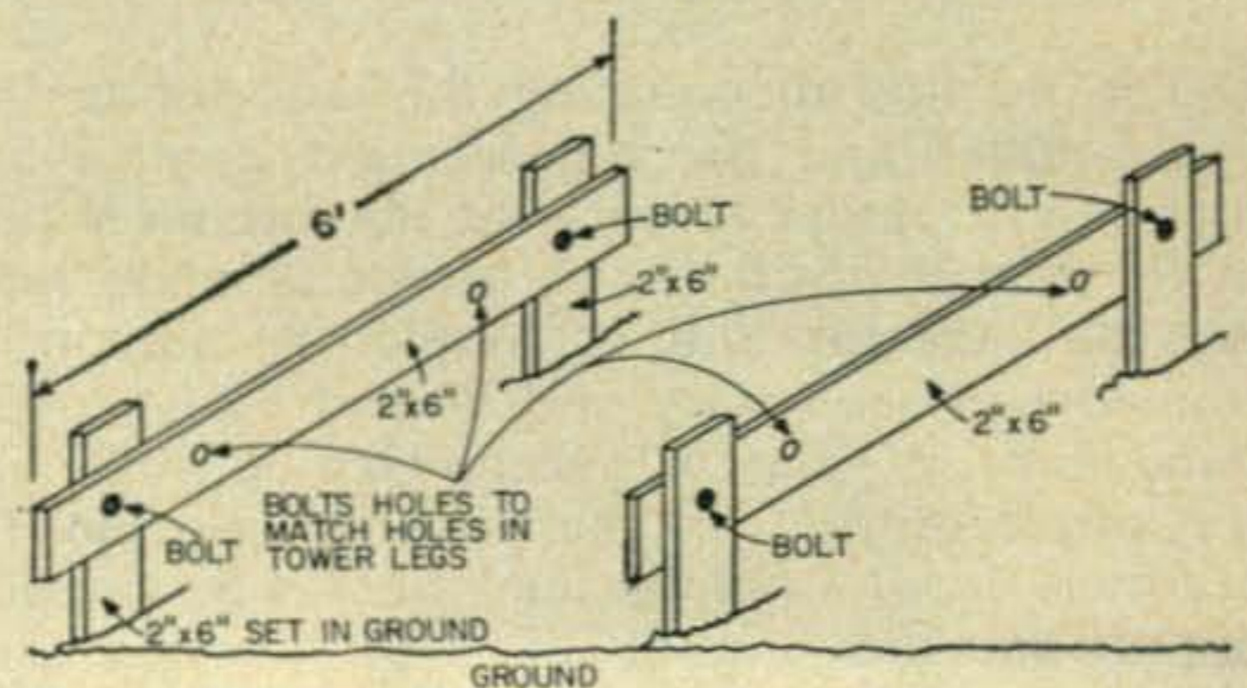
Fig. 2—Details of tower base. When the antenna is in place it may serve to remove the weight from the pivot hinge.
