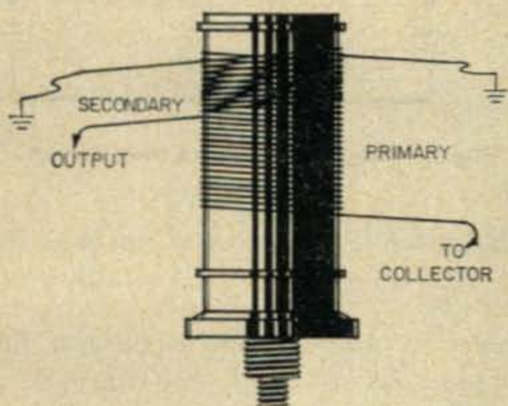
Fig. 2—Construction details for L_3 . Further information is given in the Coil Data in fig. 1. In tuning L_3 , the powdered iron slug is varied so that it meshes only the collector end.
