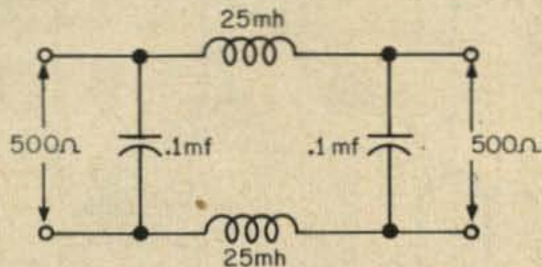
Fig. 2—Lowpass constant K filter.
