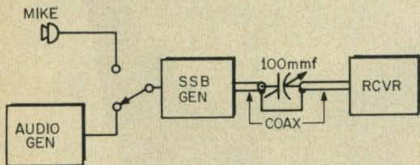
Fig. 7—Block diagram of the test set up used to align the generator.
