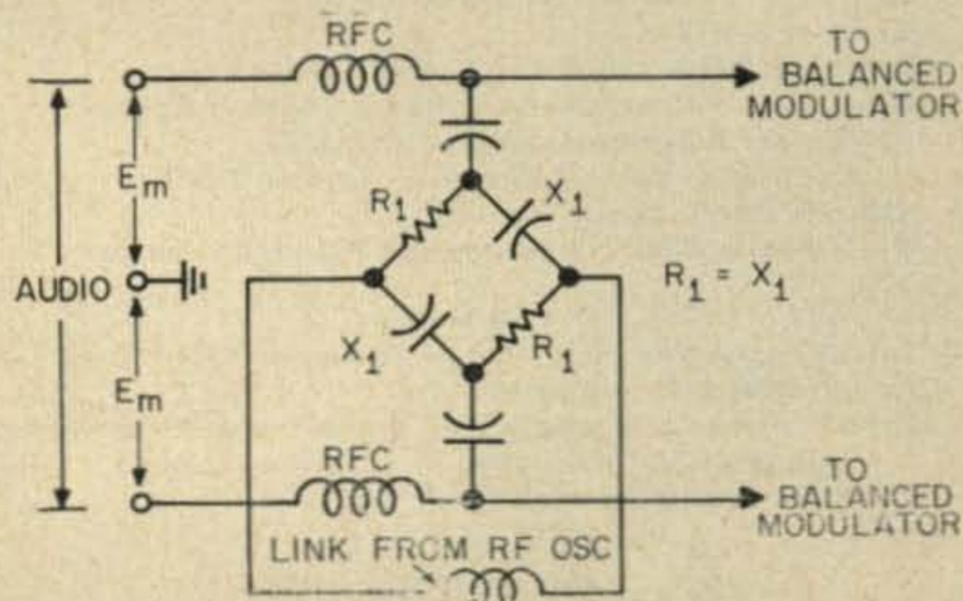
Fig. 1—Basic rf phasing network.
