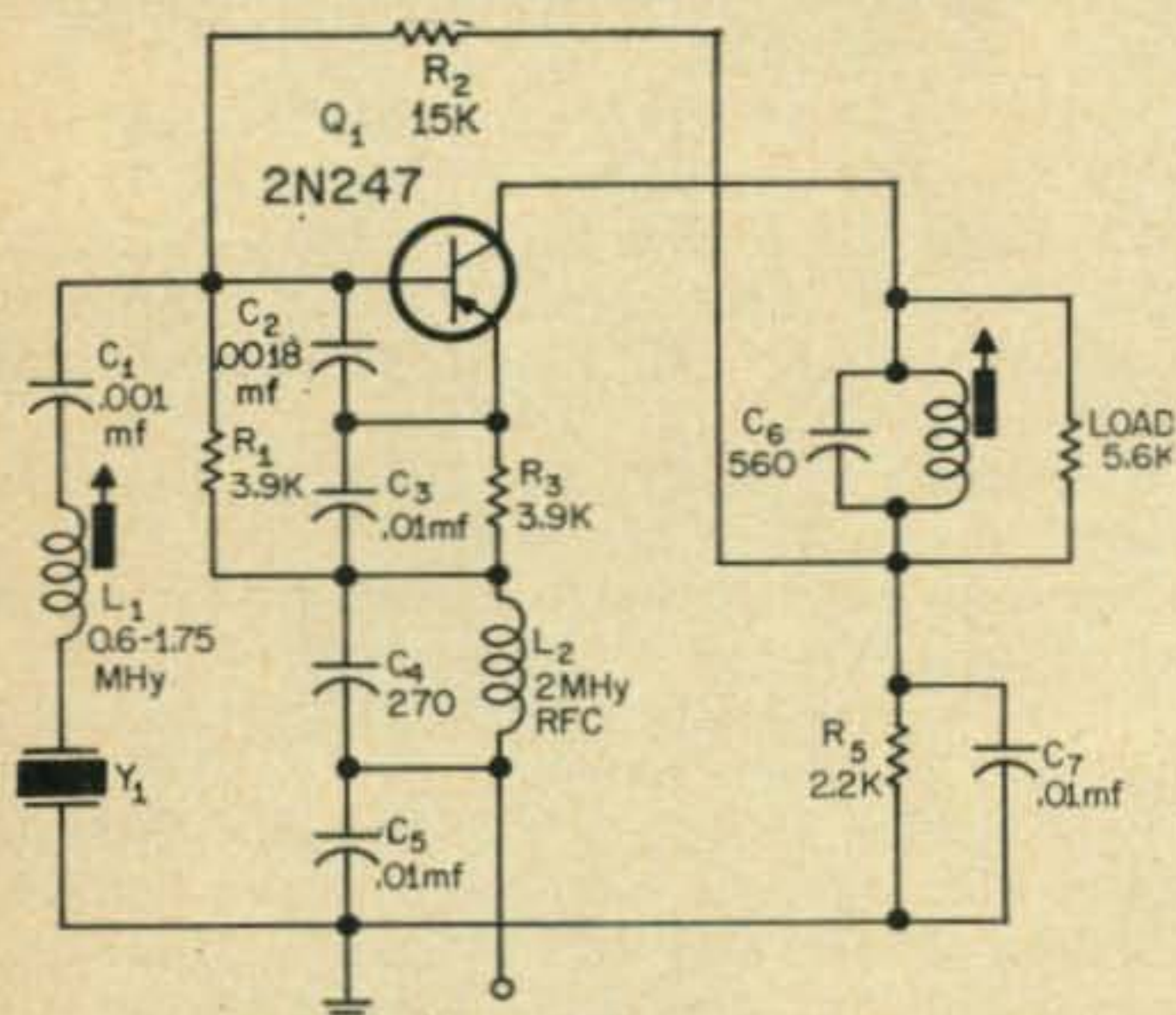
Fig. 1—A 450 kc crystal oscillator suitable for use in transistor receivers as a bfo or in a transmitter as a carrier generator.
