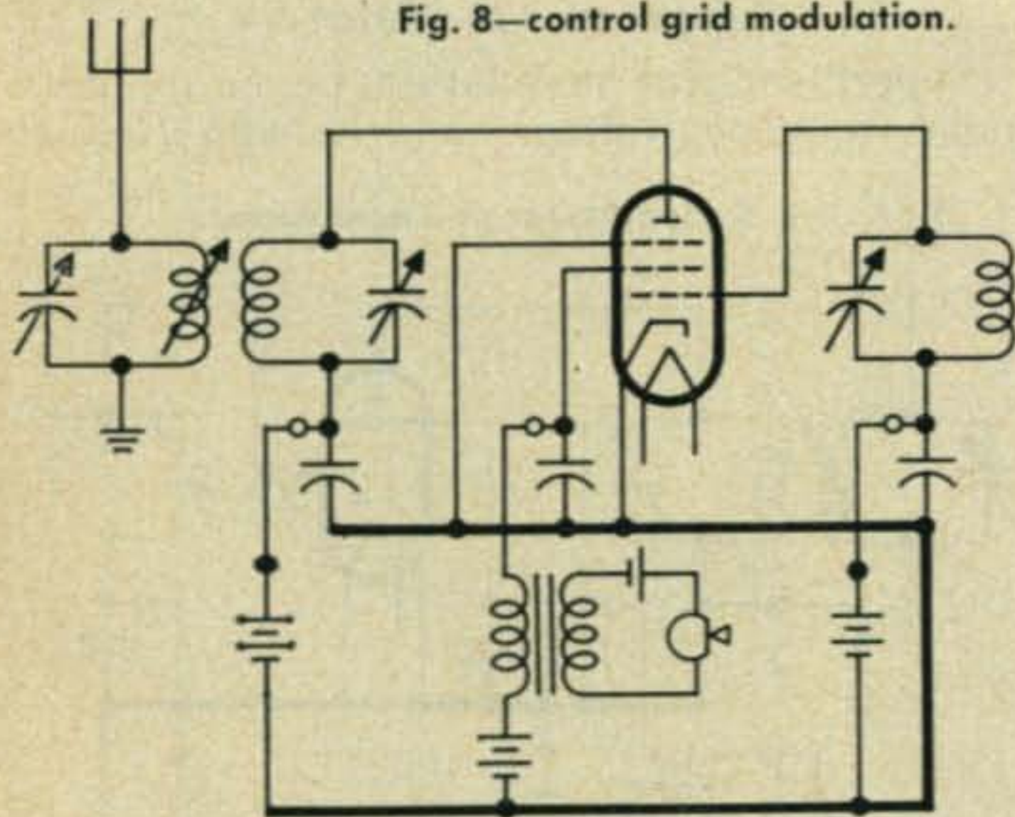
Fig. 8—control grid modulation.
