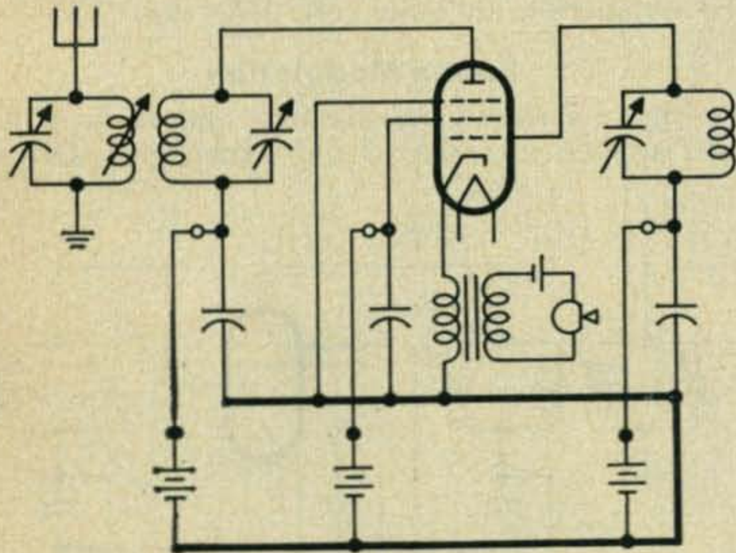
Fig. 9—Cathode modulation.
