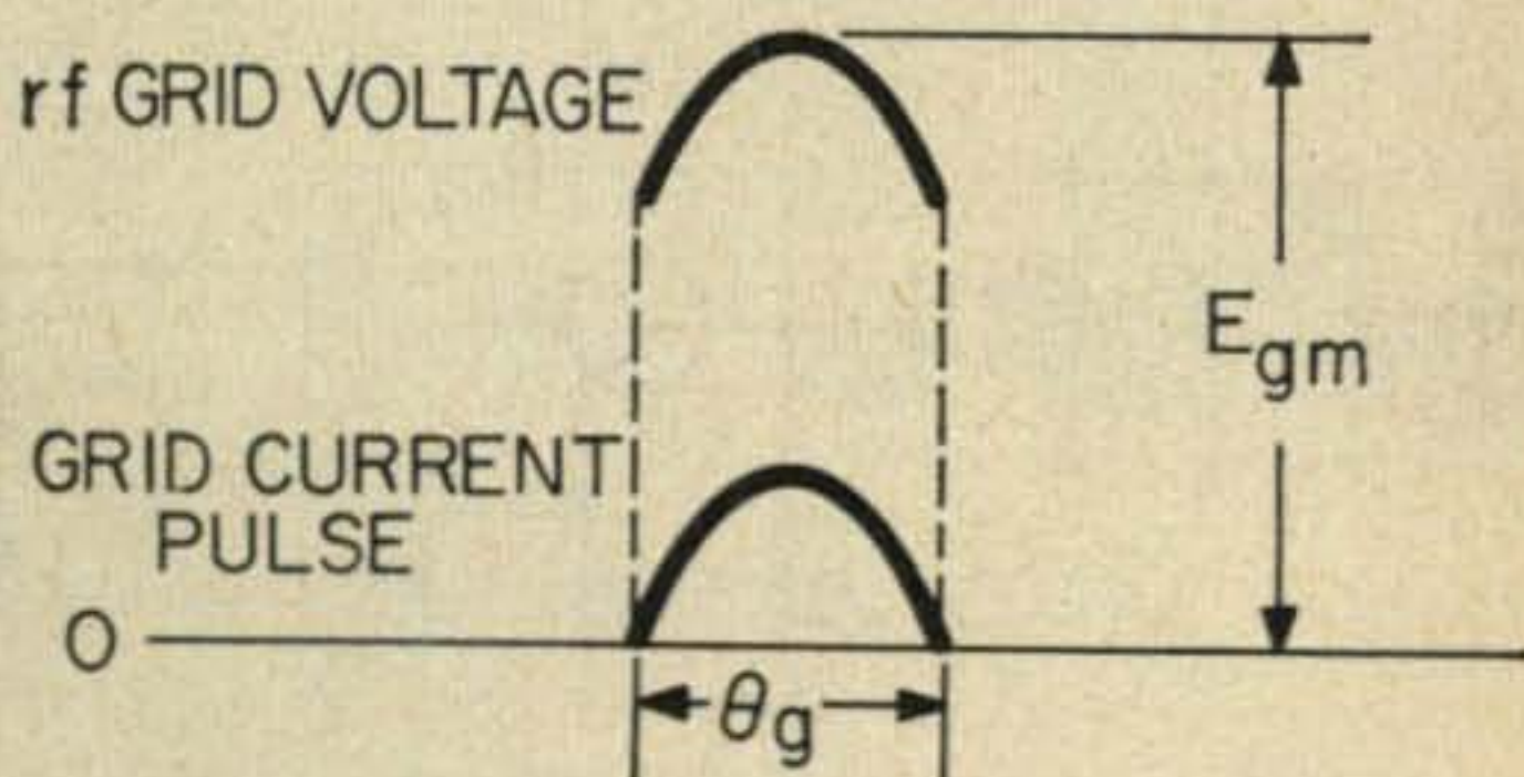
Fig. 3—The grid voltage and its corresponding pulse of grid current.
