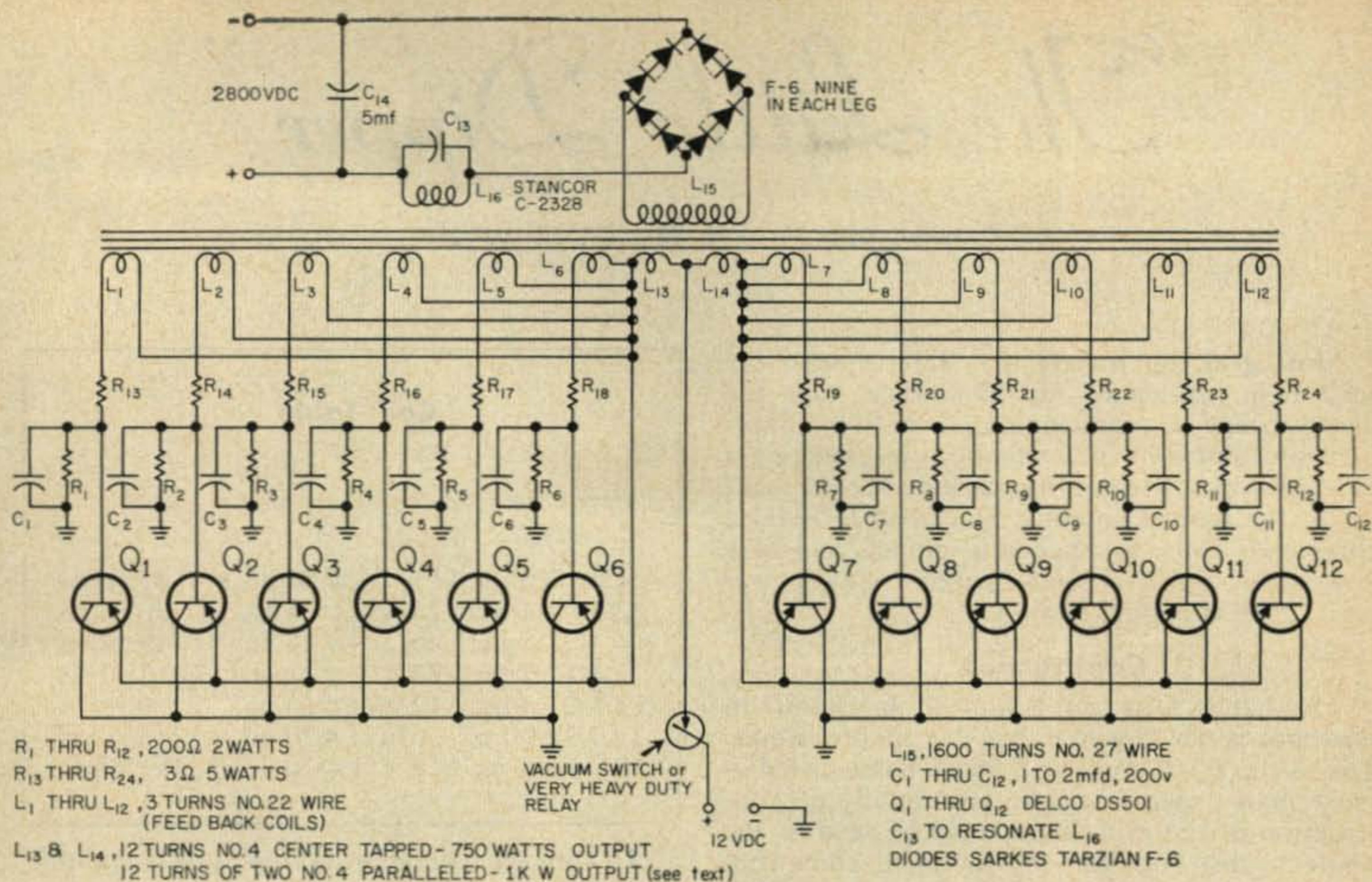
Fig. 1—Schematic of a 1 kw plate supply. The transformer is discussed in the text.
