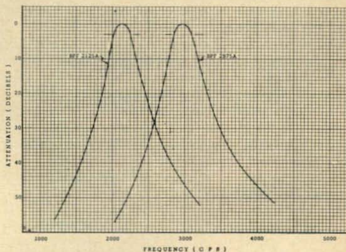
Fig. 2—Response Curves, 850 cycle Shift Channel Filters.
