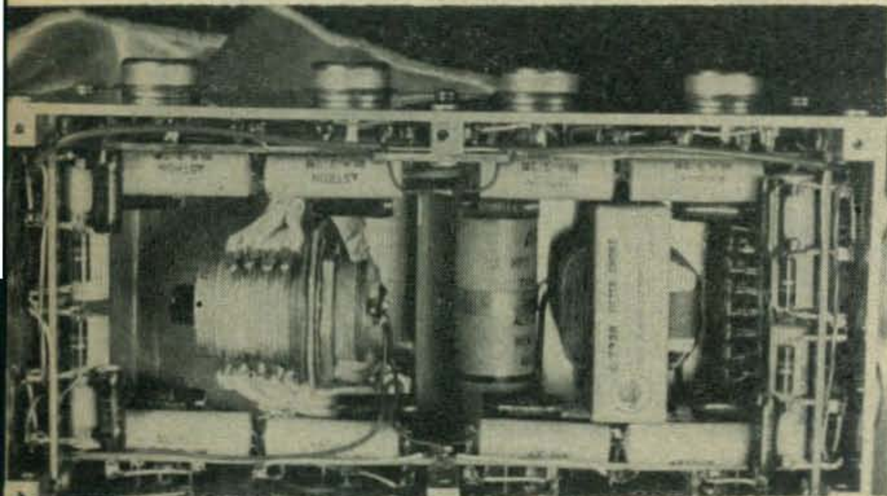
Top view with cover removed showing parts location and sheet metal work. The F6 rectifiers are mounted on an insulated board to the right of the choke. The high power Jennings vacuum switch is mounted above the toroidal transformer and occupies the major portion of the left side of the supply.
