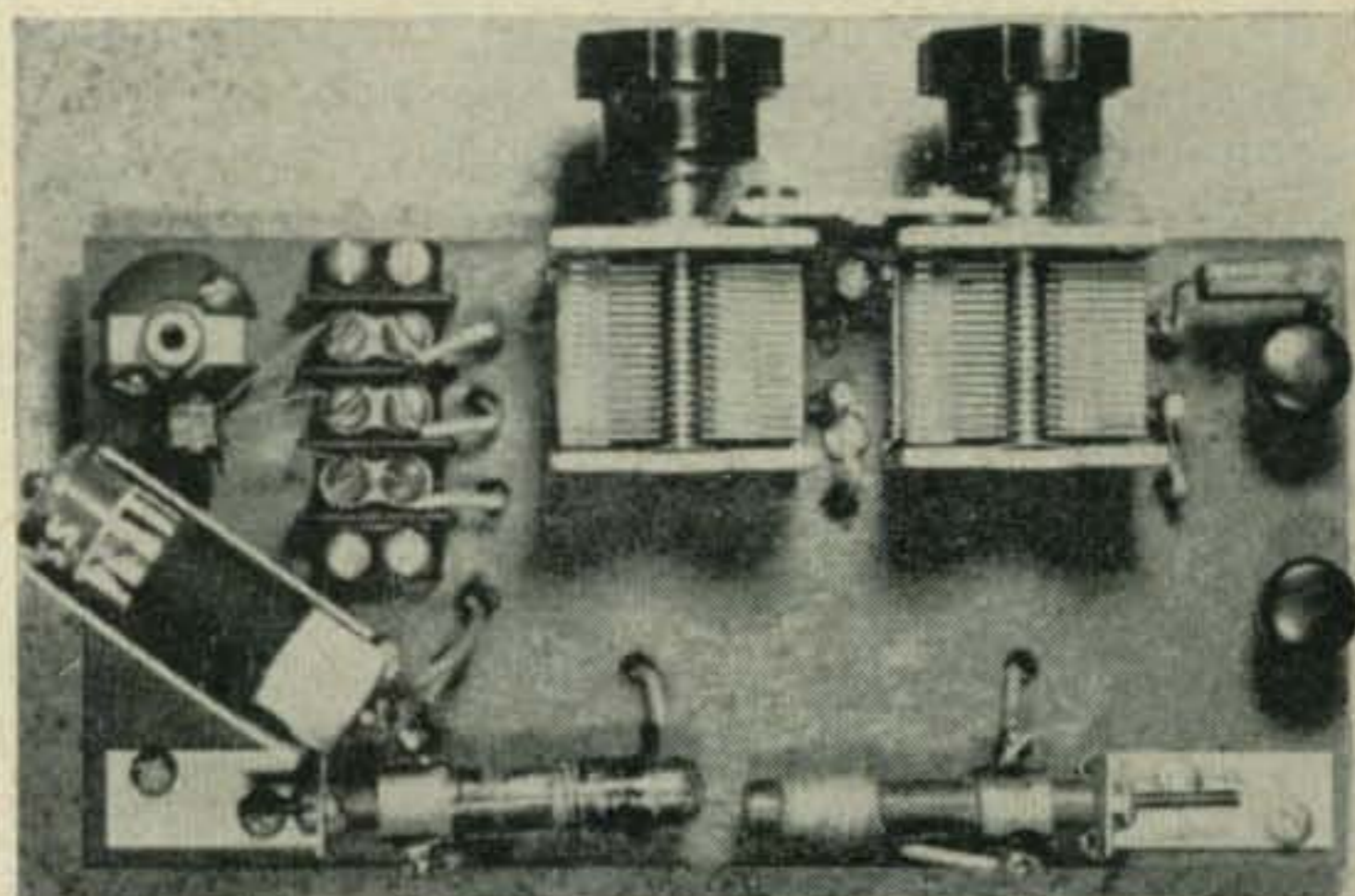
Layout and wiring view of the Transistor Tattle-Tale Conelrad receiver. Note that the transistor is secured to a Kulka block type terminal strip. Posts for antenna and ground are at the right, while the speaker line is near the transistor. The coils should be mounted as shown, back-to-back, near the rear of the chassis. If a metal chassis used, bend the coil brackets so the coils clear the chassis by one inch or more. (Photo by Ray Welch, K9ISQ)
