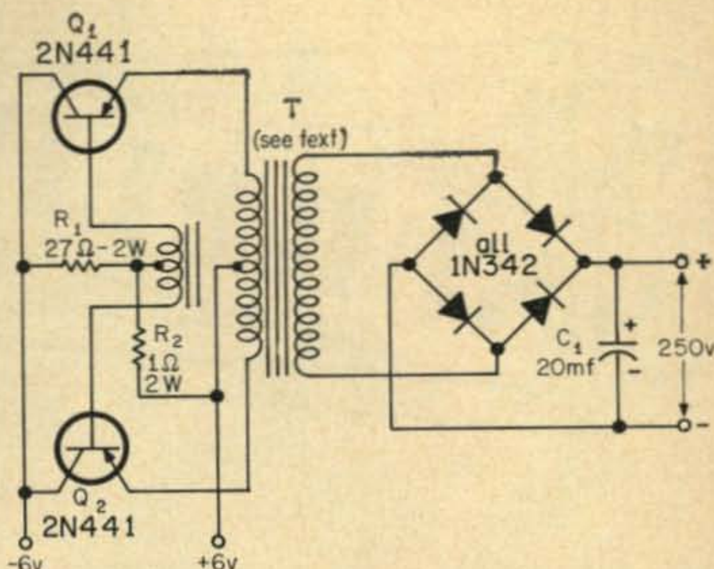
Fig. 4—Power supply circuit submitted by Delco intended to supply 250 volts at 200 ma for a 6 volt source.
