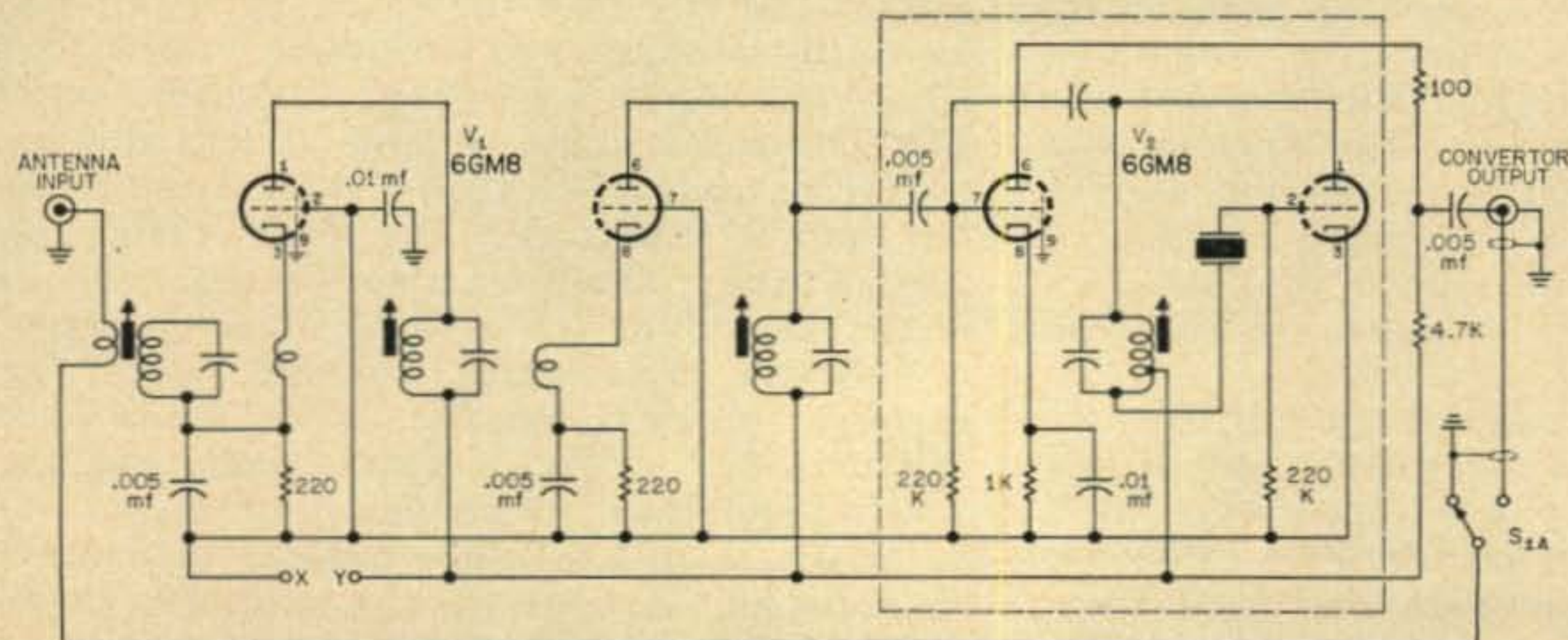
Fig. 1—Schematic of the Aircor converters. All models use the same circuit.
