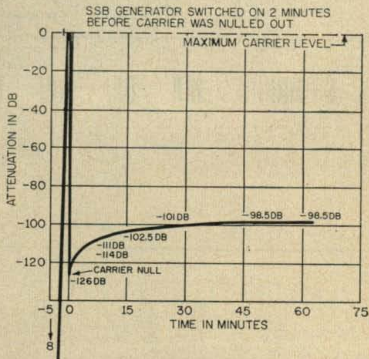
Fig. 11—Carrier suppression drift curve.
