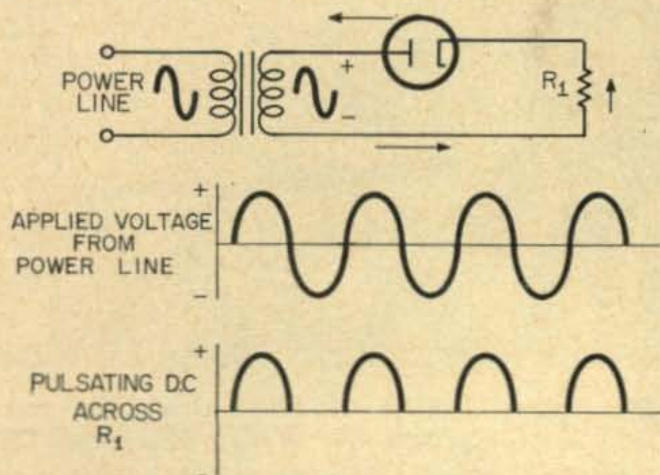
Fig. 1—A simple half-wave rectifier circuit
