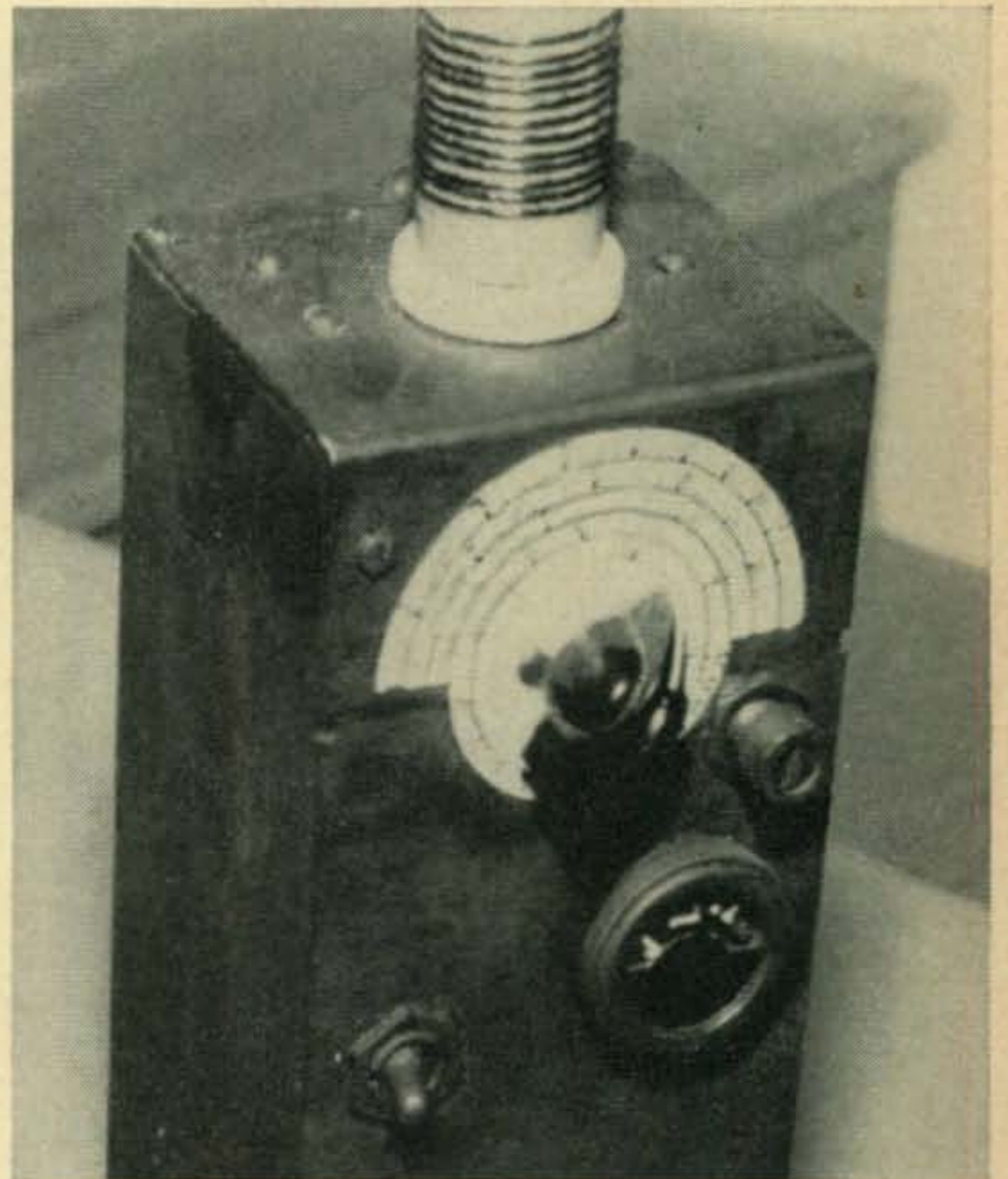
Details of the front panel showing control layout. The small knob above the meter is R_2 meter adjust.
