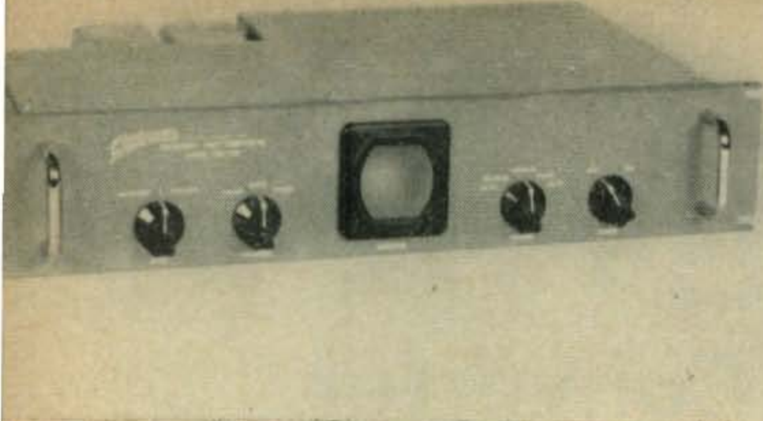
Top—Electrocom Model FSC-250 Frequency Shift Converter. Controls from l to r.; Bias, Channel, Monitor Scope, Keying Selector, and Power Switch. Right—Inside the FSC-250 Converter. The entire unit is constructed on a 3½" rack panel. Power supply components are to the right. Plug-in band pass filters can be seen at the upper left.
