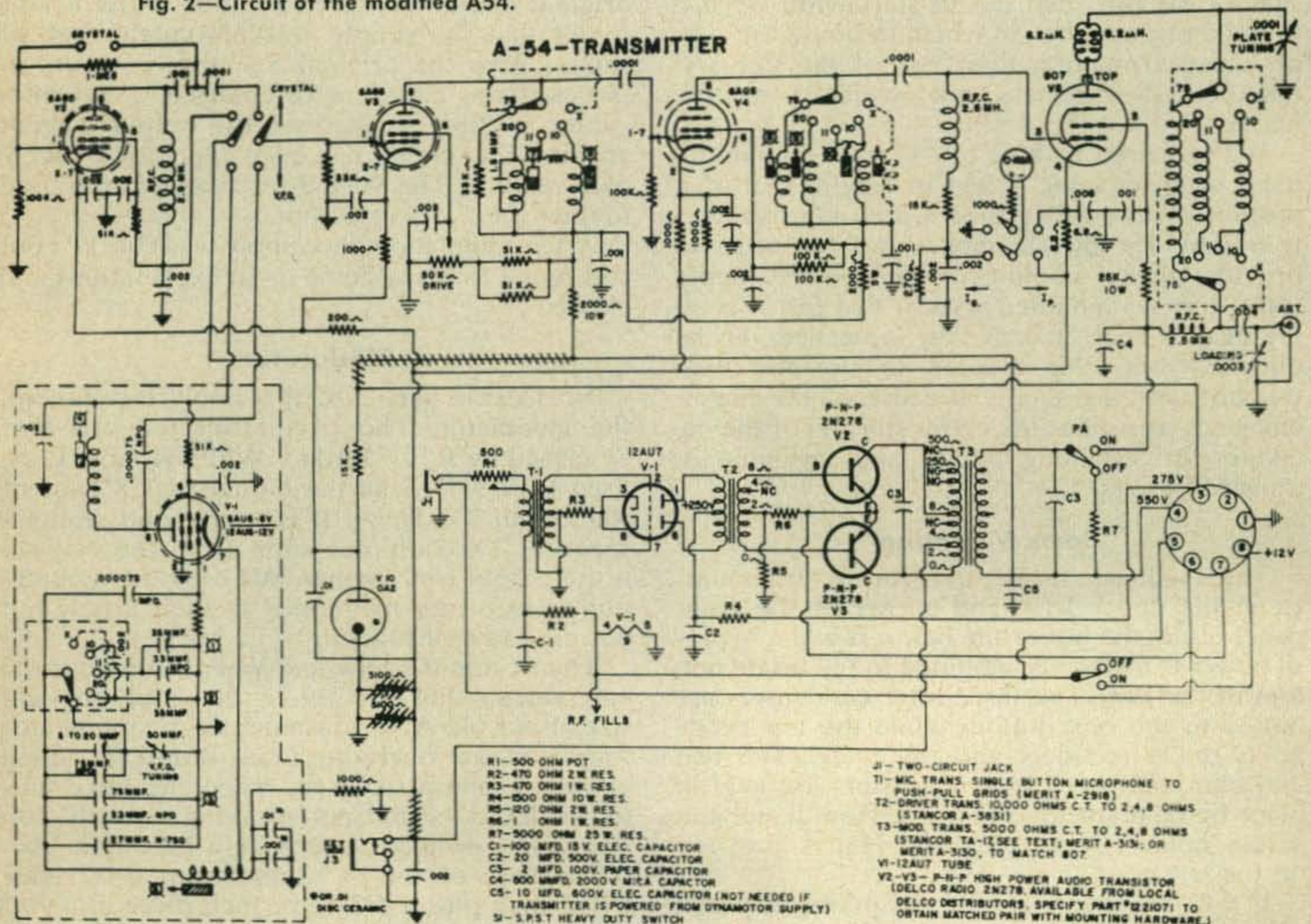
Fig. 2—Circuit of the modified A54.
