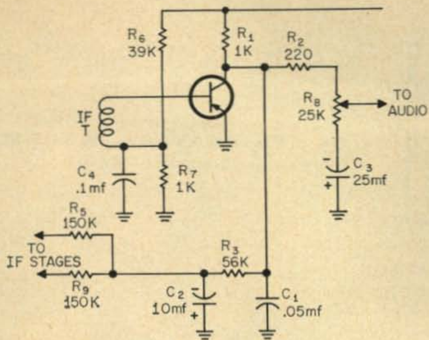
Fig. 3—Detector circuit designed by W. E. Sheehan and J. H. Ivers of Raytheon Mfg. Co. Operation is explained in the text.
