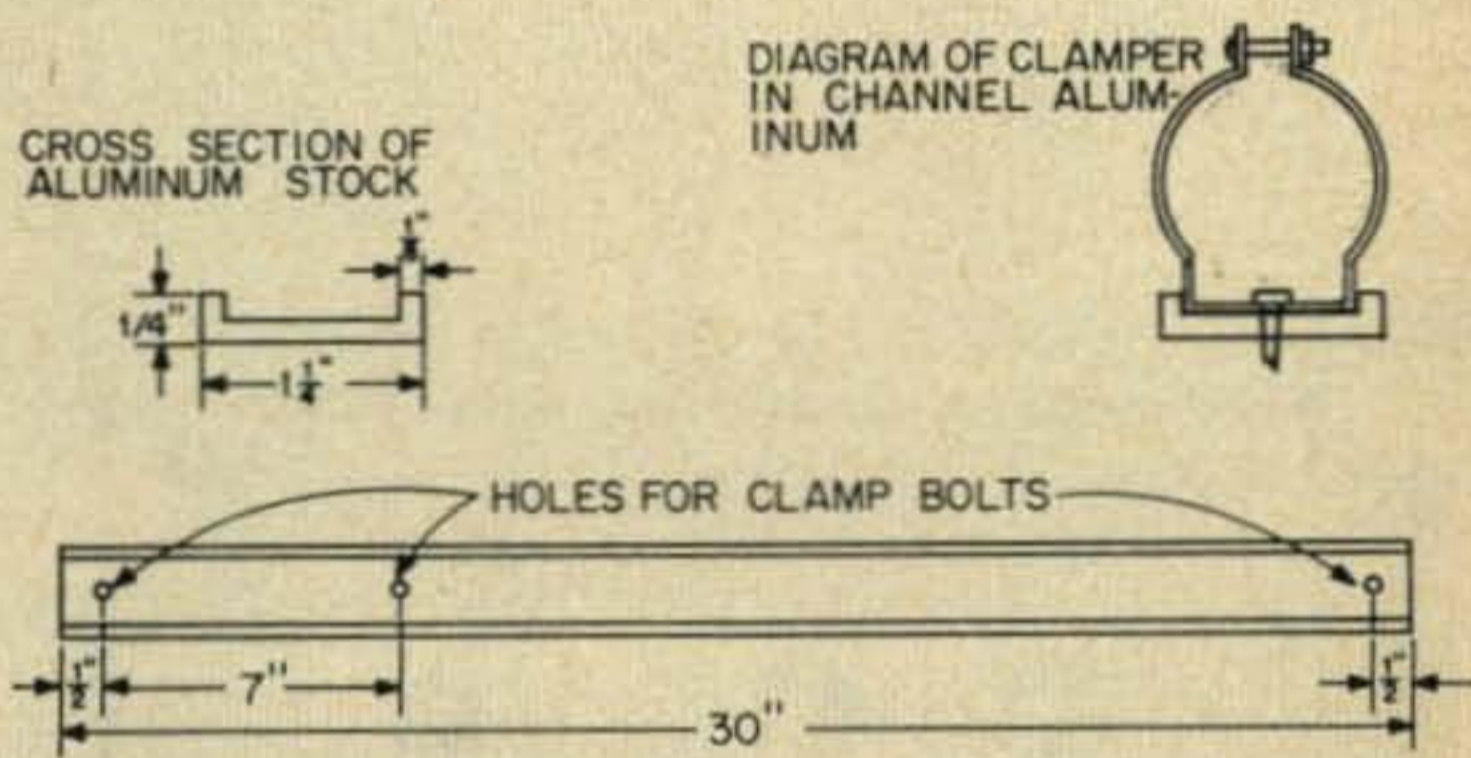
Fig. 1—Measurements of the element support rods.
