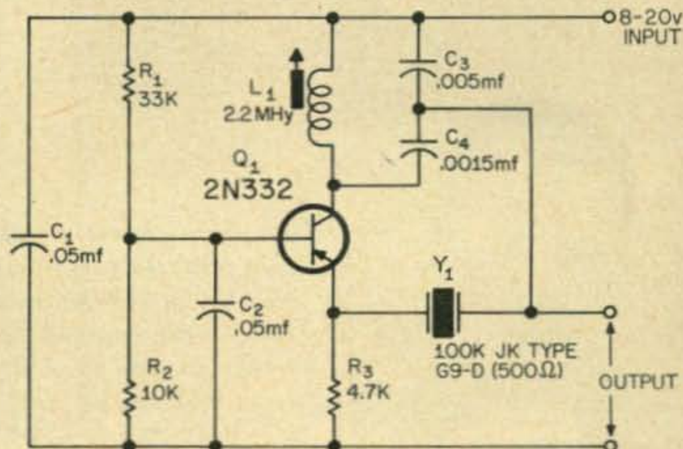
Fig. 2—Circuit useful as a 100 kc frequency standard.
