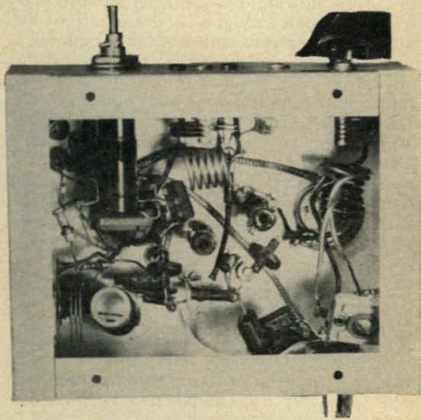
Underside view of the transmitter. C_3 and L_2 are at the lower left and C_{13} can be seen at the lower right.
