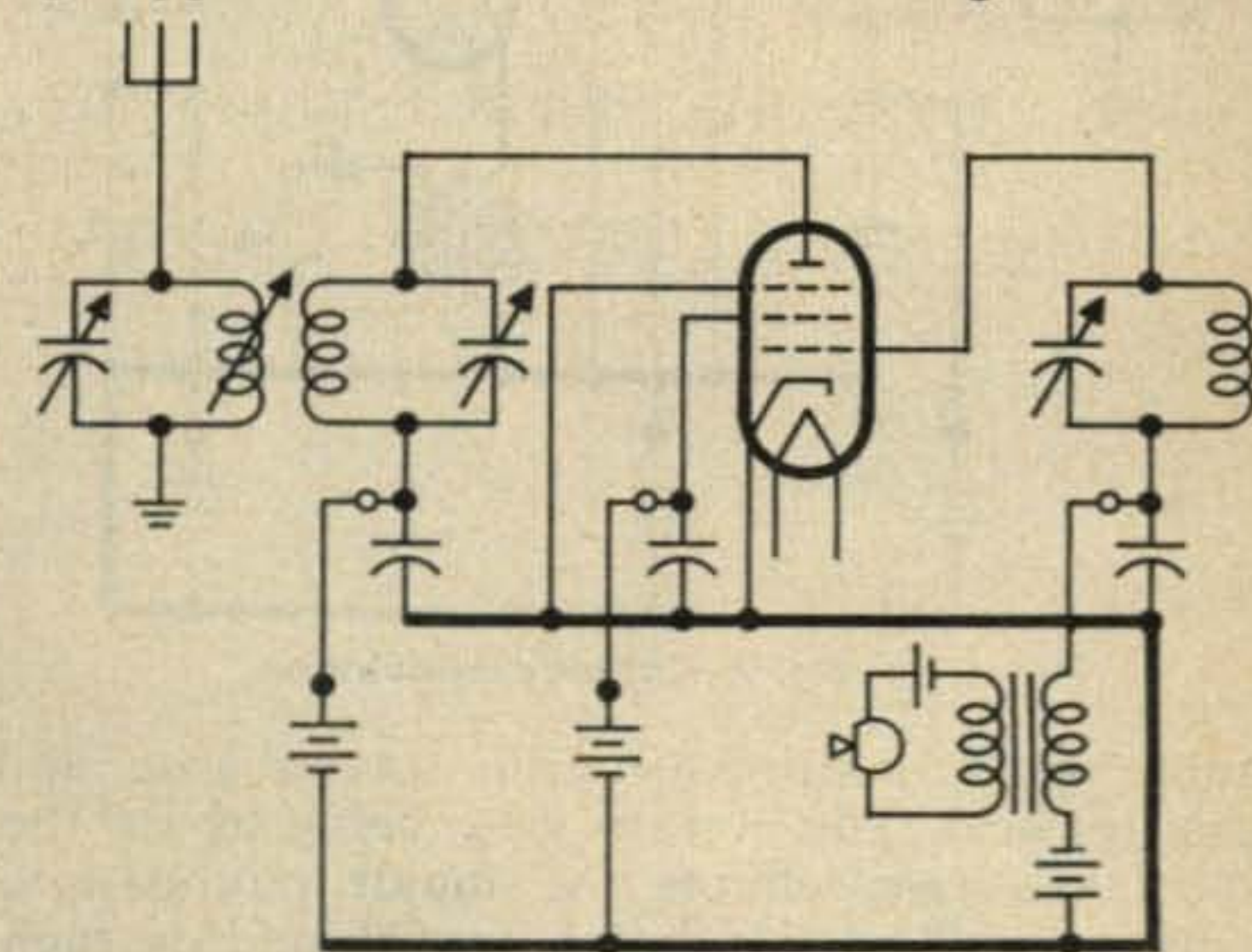
Fig. 7—Screen grid modulation.
