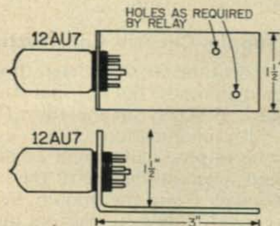
Fig. 2—12AU7 mounting bracket details.
