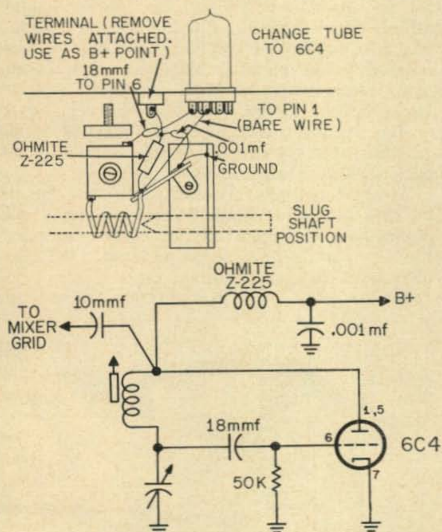
Fig. 2—Revised ARR2 oscillator schematic and pictorial.
