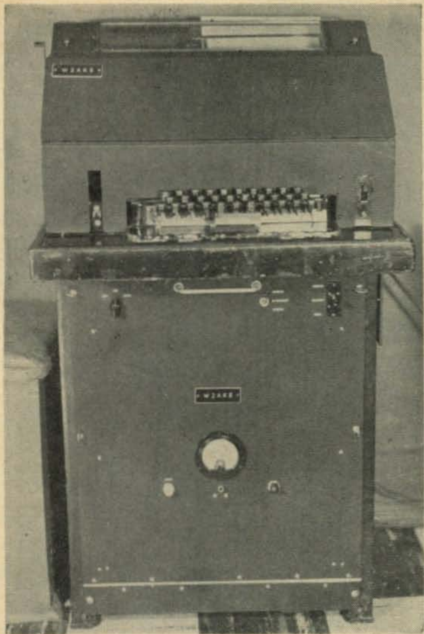
Model 12 Page Printer with Keyboard (with converter built into table).
