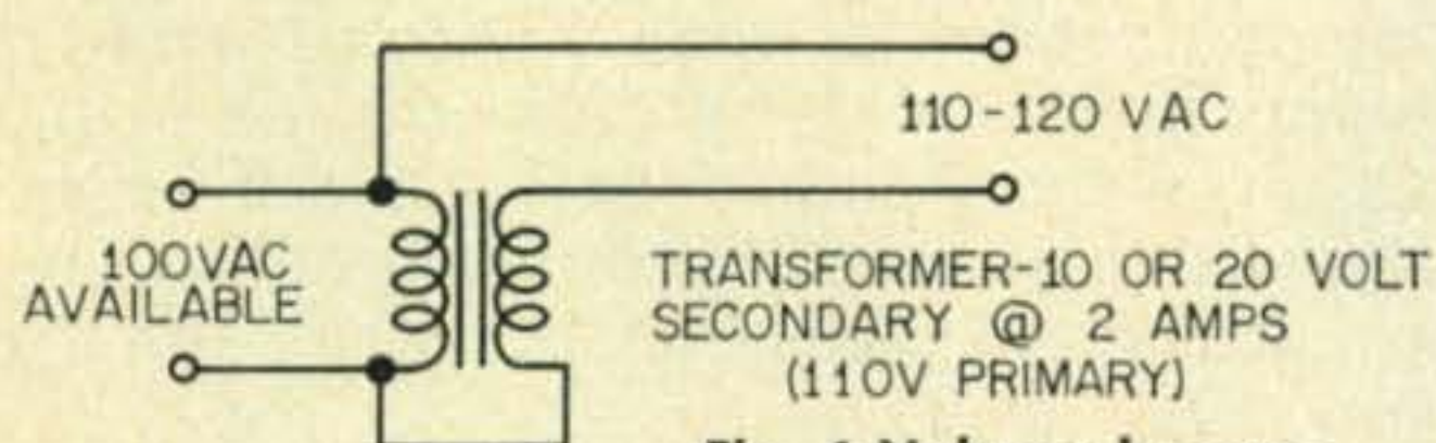
Fig. 6 Voltage booster
