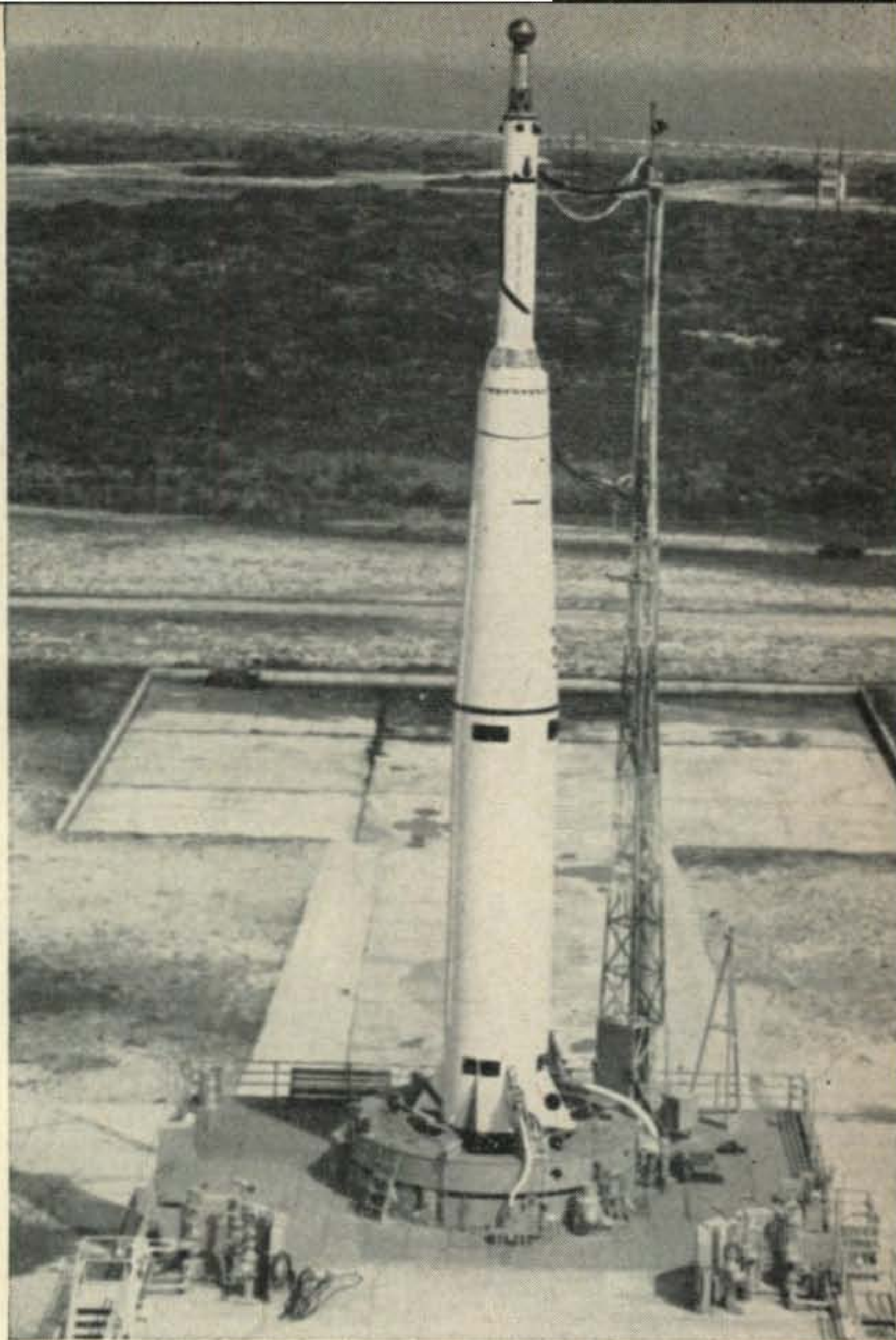
Fig. 2—Project Echo sphere container atop a Delta launch vehicle on the pad at Cape Canaveral, Fla. The next attempt for launching the 100 foot radio wave reflecting sphere is planned for the late fall of 1960 or early 1961. Official NASA Photo.
