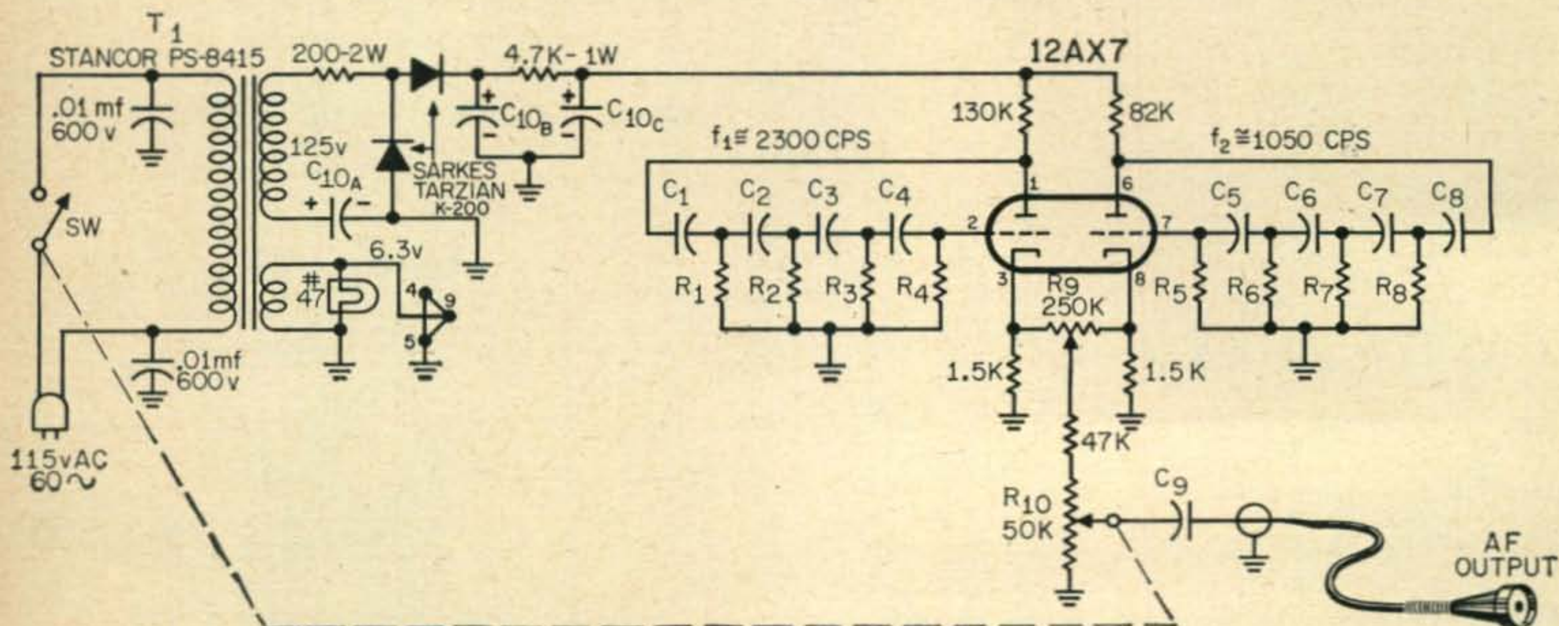
Fig. 1—Circuit of the Two-Tone generator.
