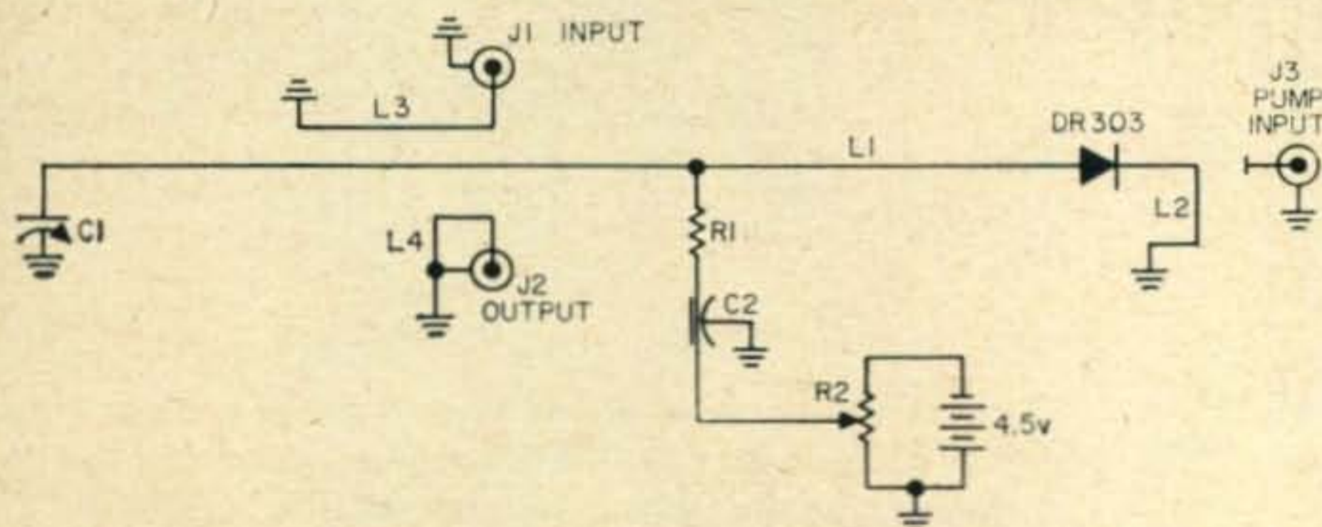
Fig. 1—Circuit of the 1/4 meter parametric amplifier.
