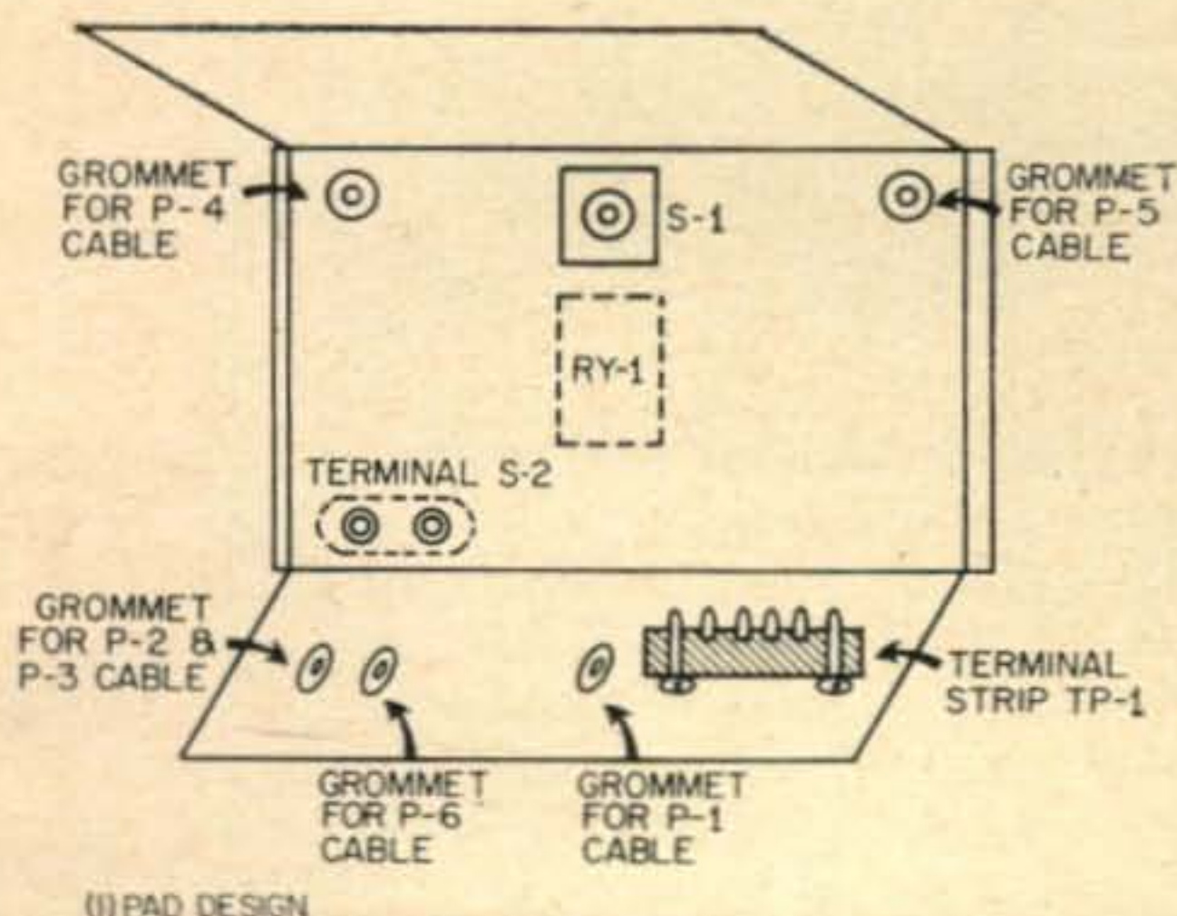
Fig. 2—Interior view of Control Central showing placement of major components.
