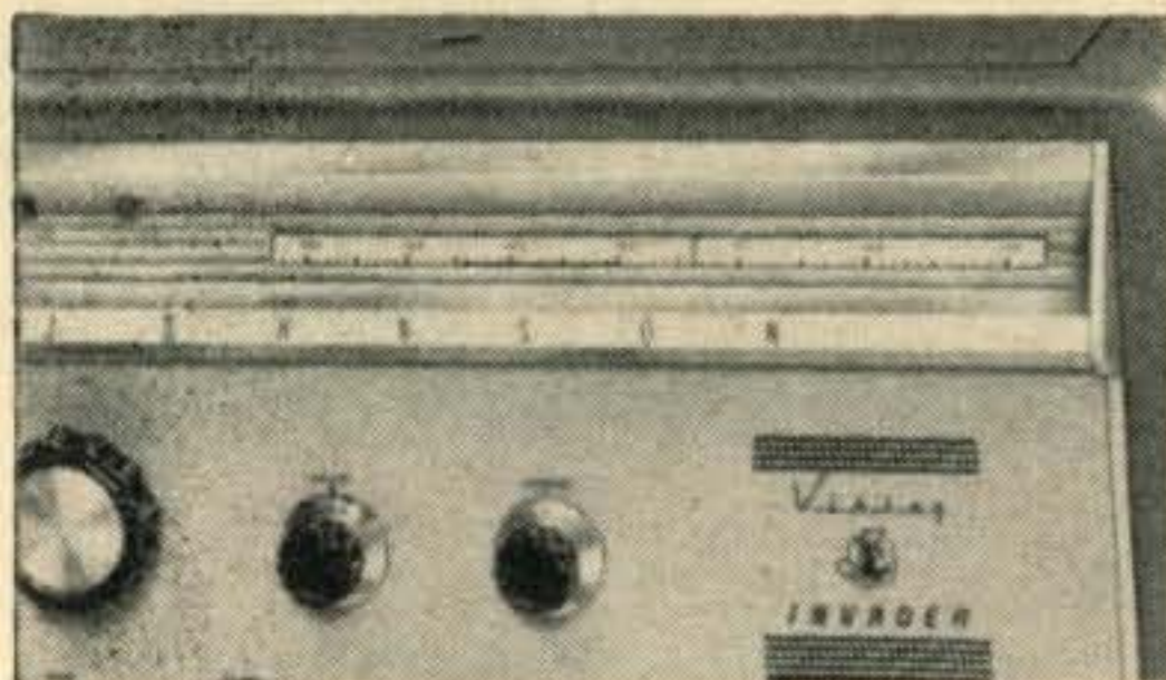
FREQUENCY CONTROL —Instant bandswitching coverage of the full 80, 40, 20, 15 and 10 meter bands... no extra crystals or retuning required. Highly stable, built-in VFO is differentially compensated and factory adjusted for maximum stability—exclusive "keep warm" heater element keeps VFO at operating temperature even with equipment turned off... NO WARM-UP DRIFT!
