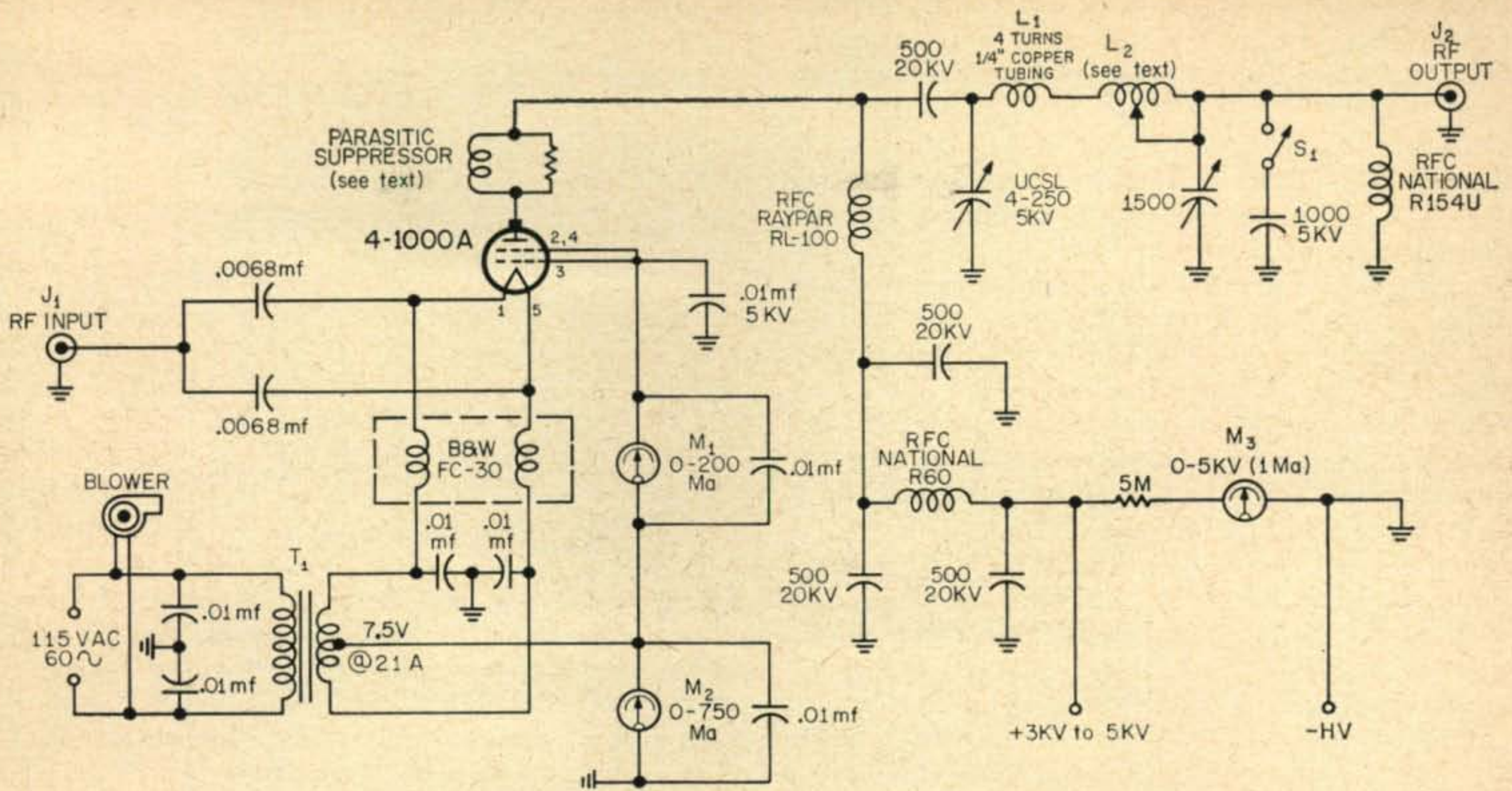
Fig. 1—Schematic of a grounded grid 4-1000A kilowatt amplifier. Drive required is in the neighborhood of 100 watts.
