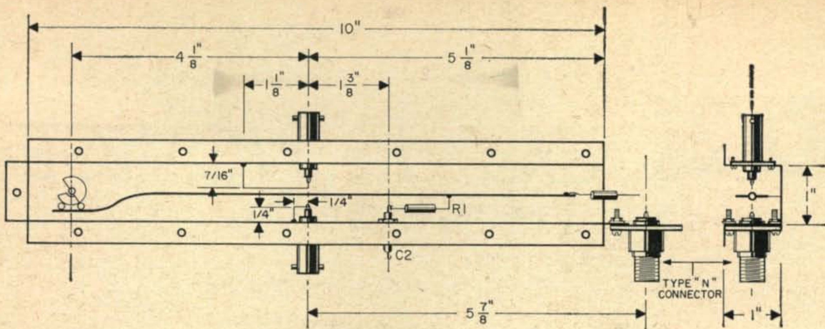
Fig. 2—Construction details of the 1/4 meter parametric amplifier.
