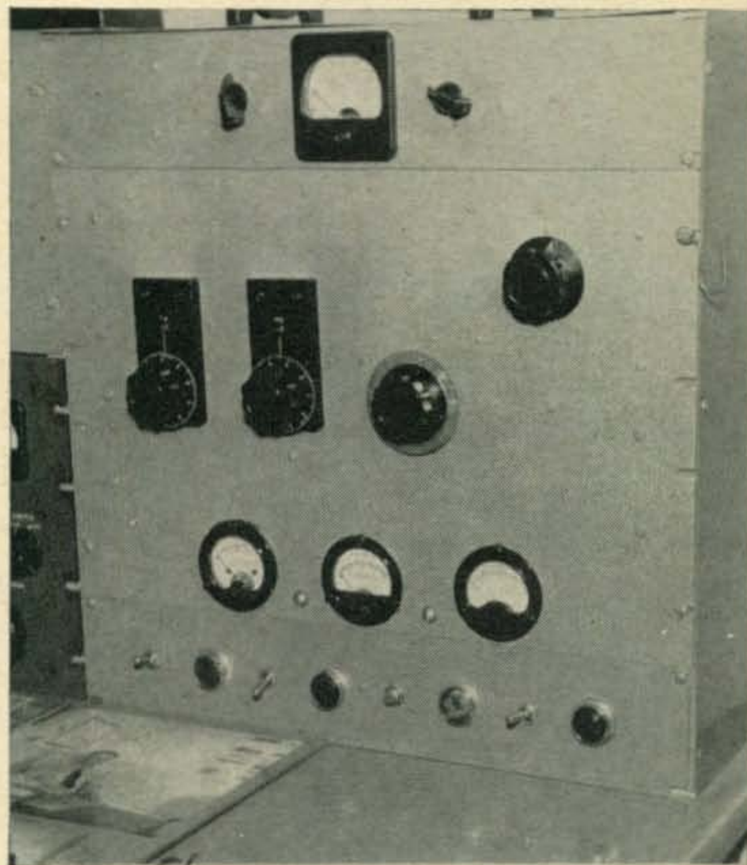
On top of the kw linear sits a swr bridge and below are the switches, circuit breakers and associated pilot lights. The turns counter on the left of the 19 inch panel tunes inductance L^2 while the other controls the vacuum variable plate capacitor. The larger skirted knob twiddles the Cardwell 8013, antenna loading capacitor while the smaller knob is used to switch in extra capacity for 80 meters.
