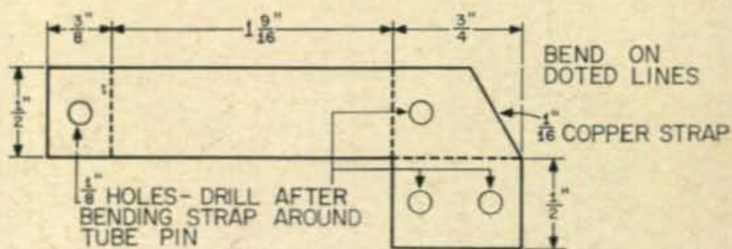
Fig. 2—Drawing illustrating the fabrication of the pin connectors of the 4-1000A. After the copper has been cut and bent it should be formed tight around the pins of the 4-1000A and the nut, together with a solder lug should be securely soldered, preferably with silver solder.
