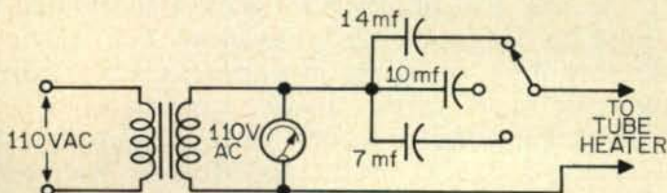
Fig. 3—Low voltage constant current supply.
