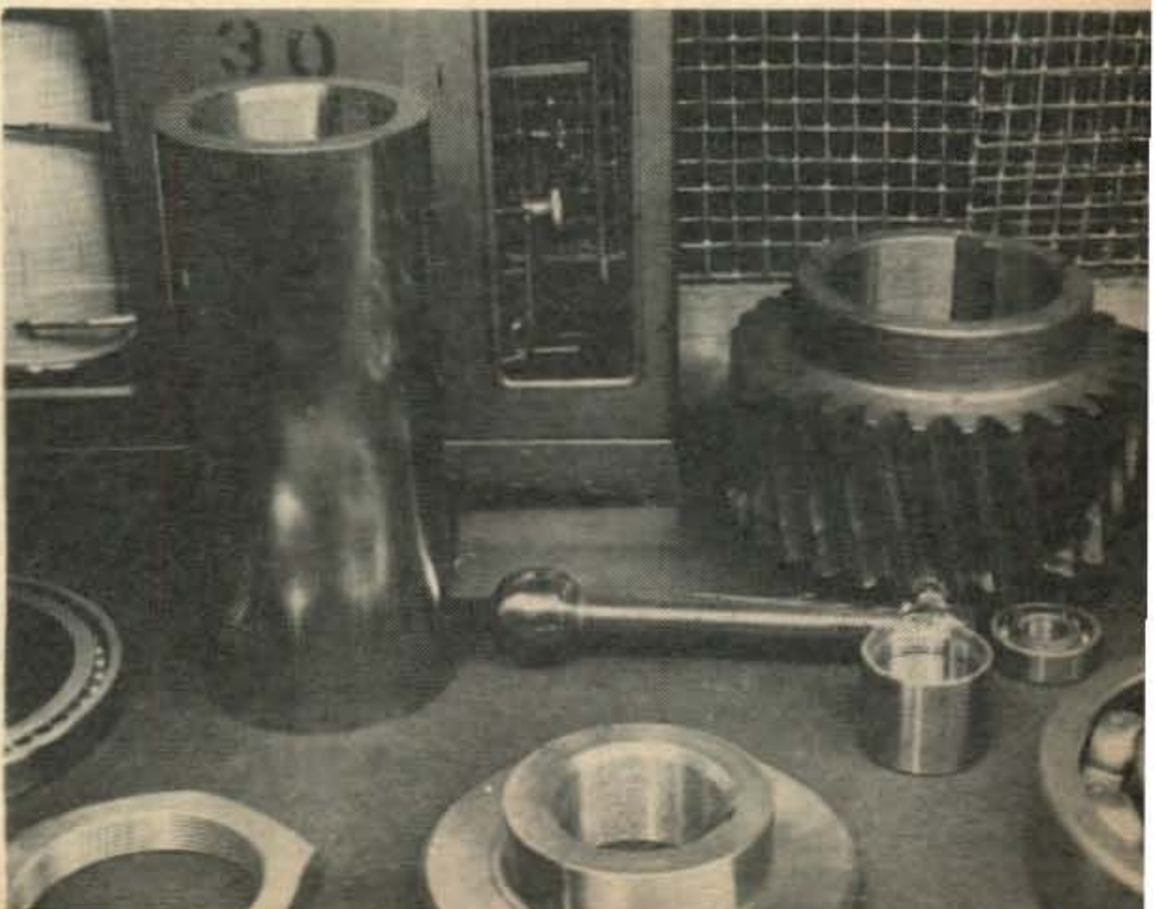
Fig. 3—Specimens exposed to 38 to 40% relative humidity, in "Controlled Humidity Storage" warehouse. These remain bright, unruined, uncorroded. Organic specimens (not shown) were free of rot or mildew.
