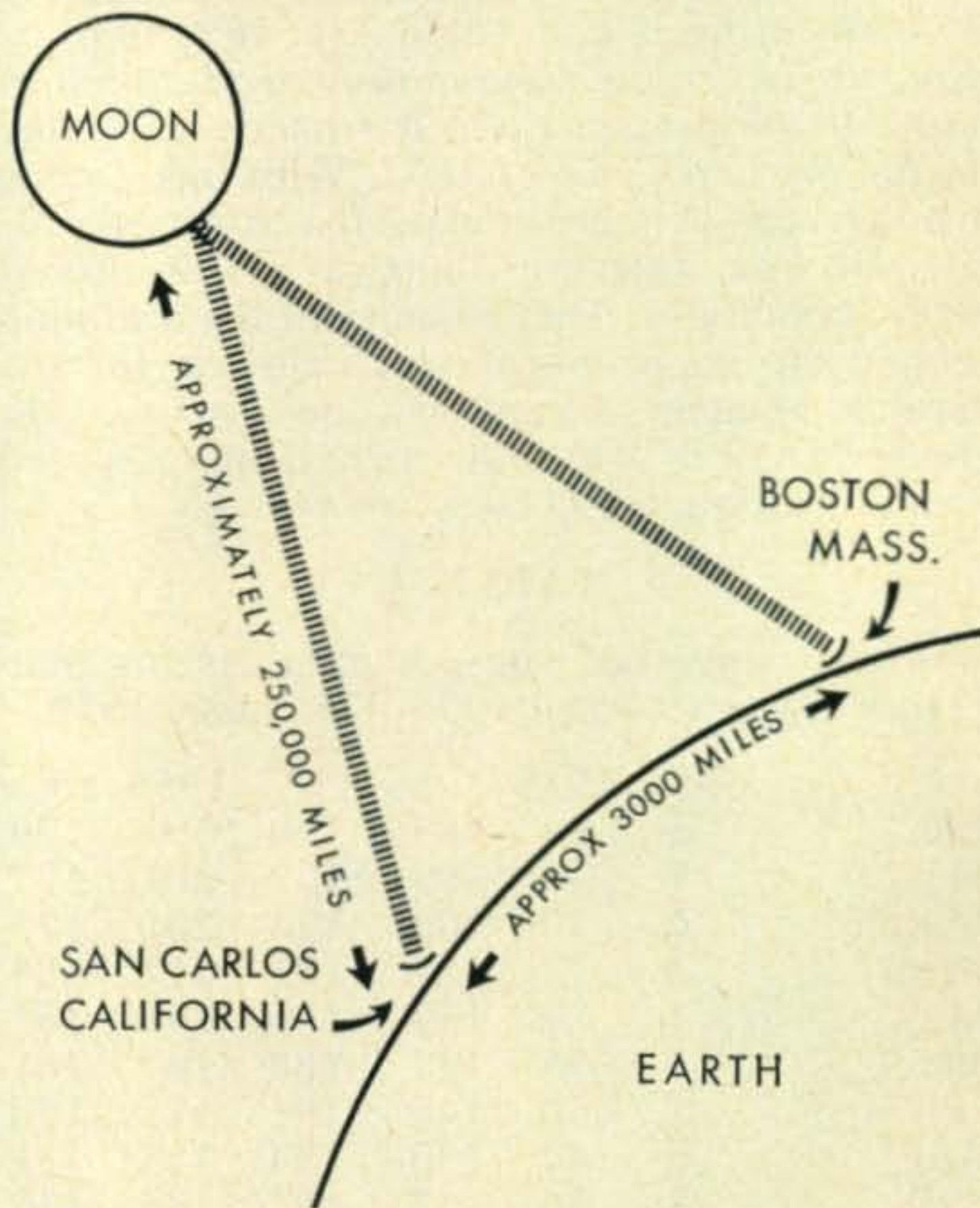
Path of the 1296 mc signal of W1FZJ-W6HB. The moon characteristics are: Mean distance from earth, 238,000 miles; Diameter, 2,160 miles; Radar cross section, 10^{12} square meters.
