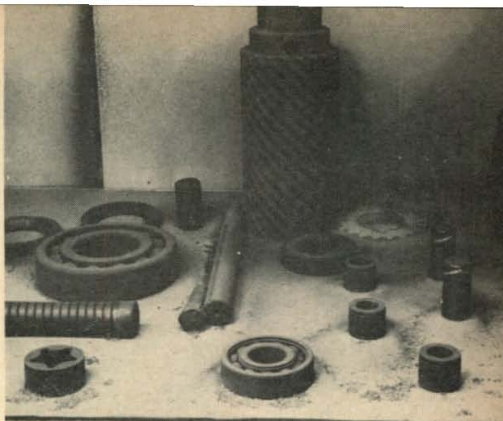
Fig. 1—Specimens exposed to outdoor air continuously. Steel specimens have a complete covering of fine grained rust.
