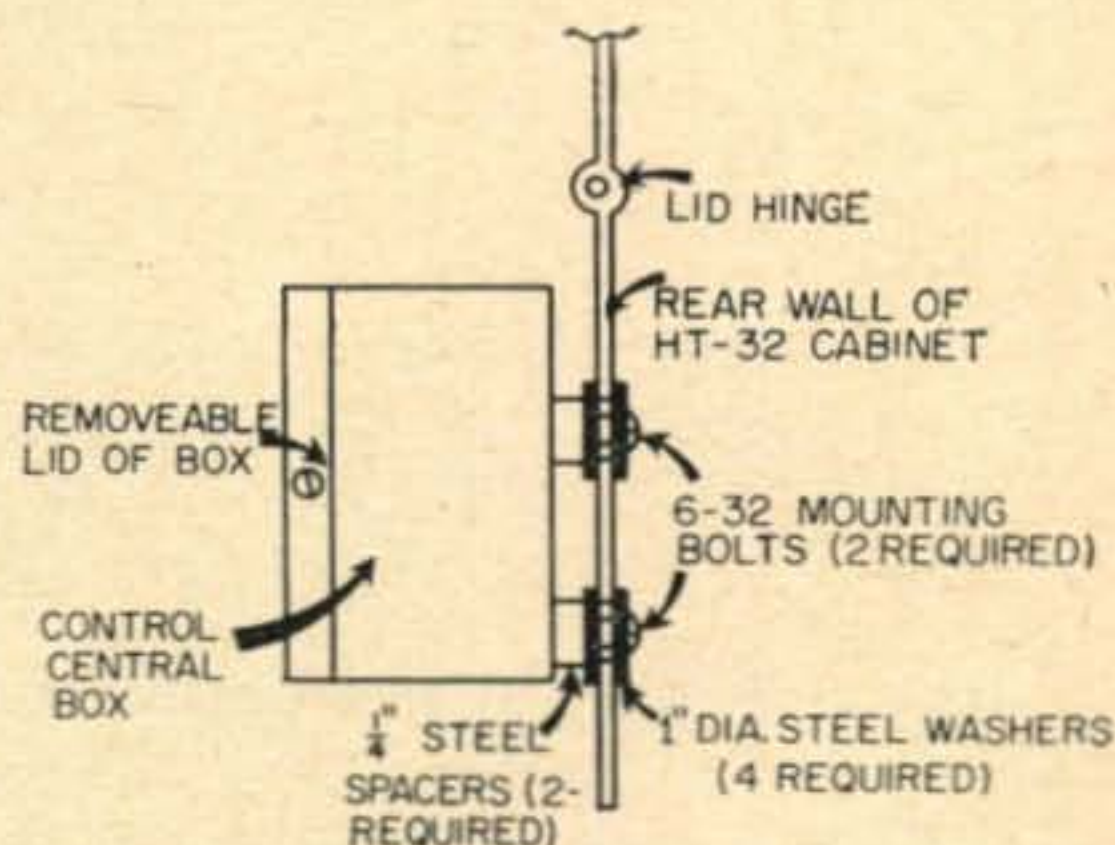
Fig. 3—Method of mounting Control Central to rear wall of HT-32 transmitter cabinet.
