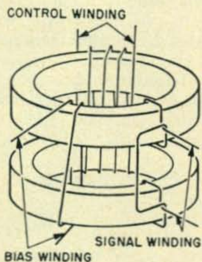
Fig. 1—Simple variable inductor—current controlled.
