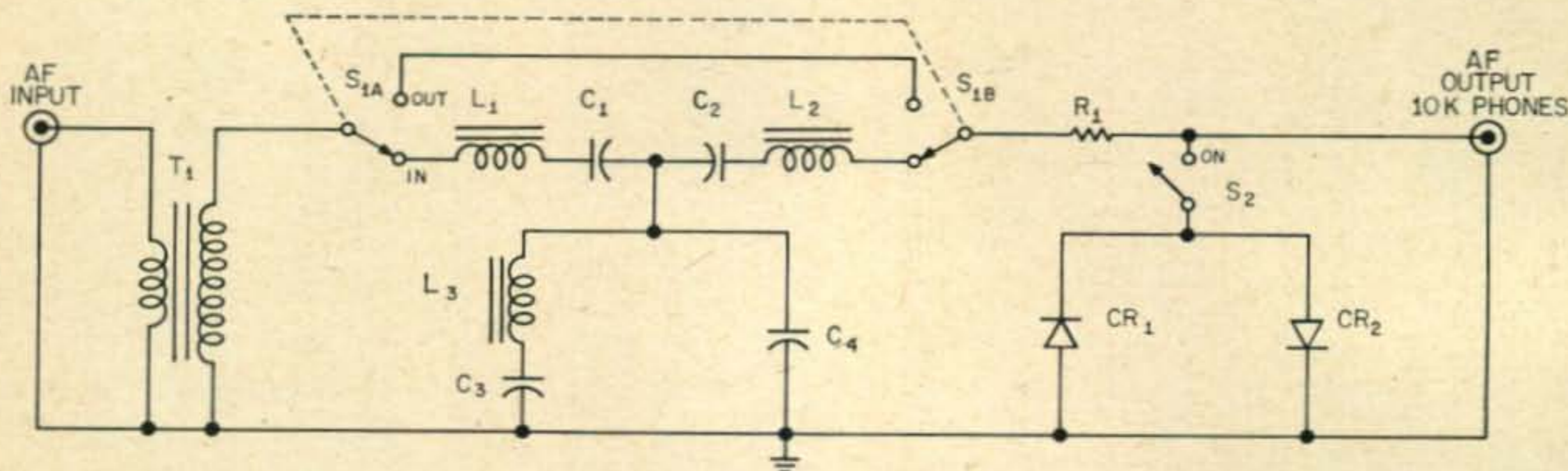
Fig. 1—Schematic of the filter. This unit has an insertion loss of approximately 2.5 db.
