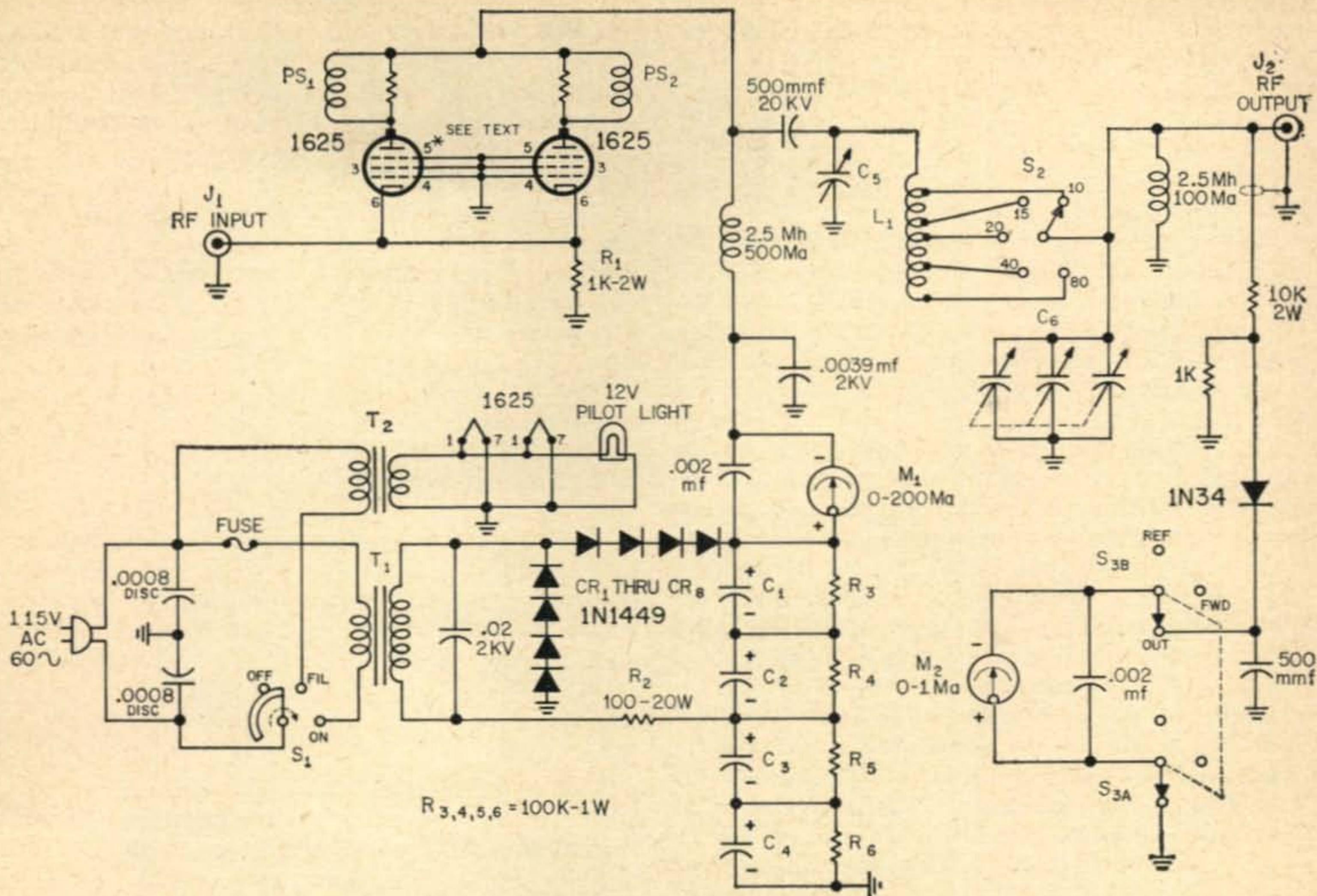
Fig. 1—The circuit of the 1625 grounded grid linear amplifier.
