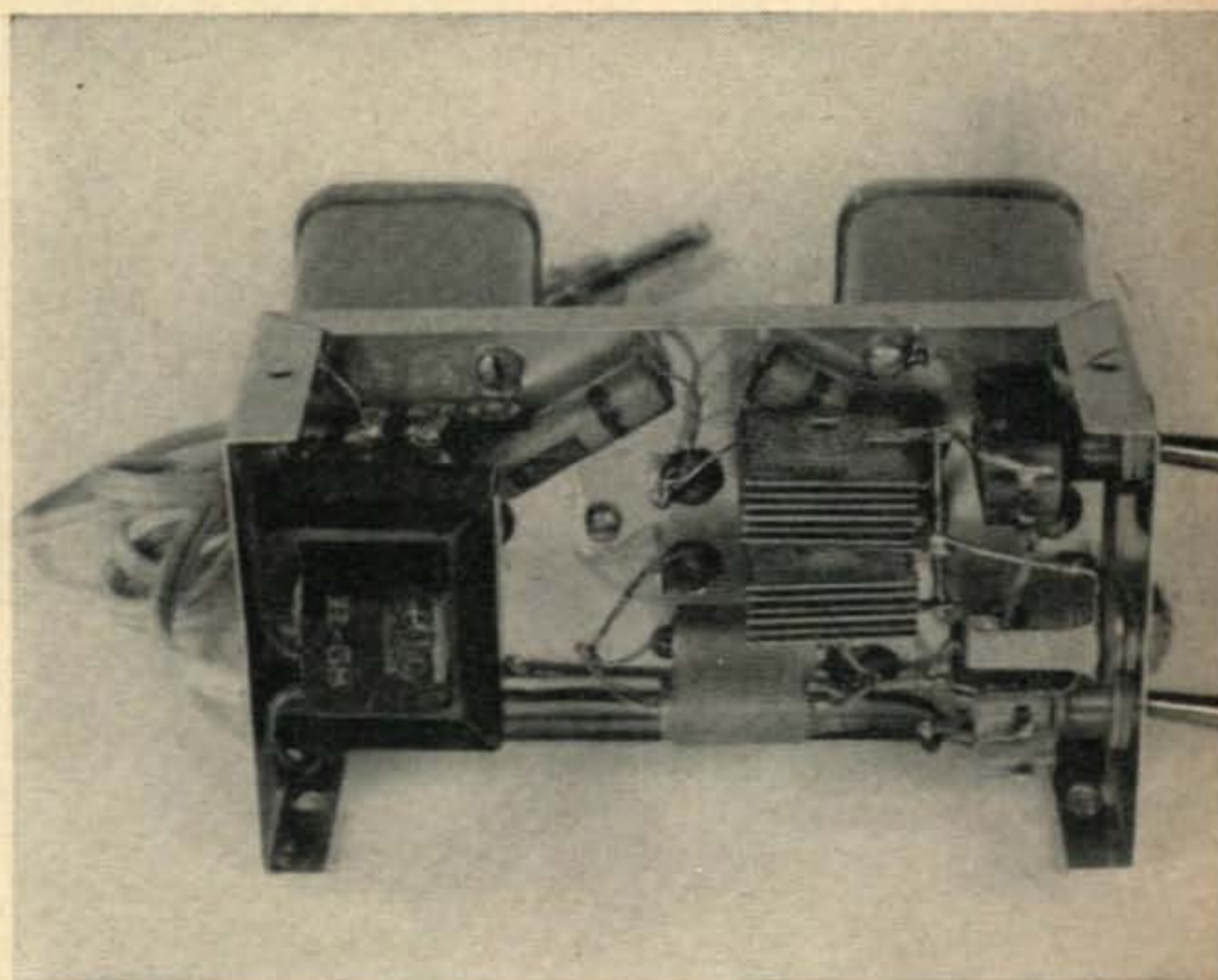
Under chassis view of the filter built on a home made 5 1/4 x 2 x 3 inch aluminum chassis. T_1 is mounted on the left skirt and the selenium rectifiers CR_1 and CR_2 can be seen behind the toggle switches.
