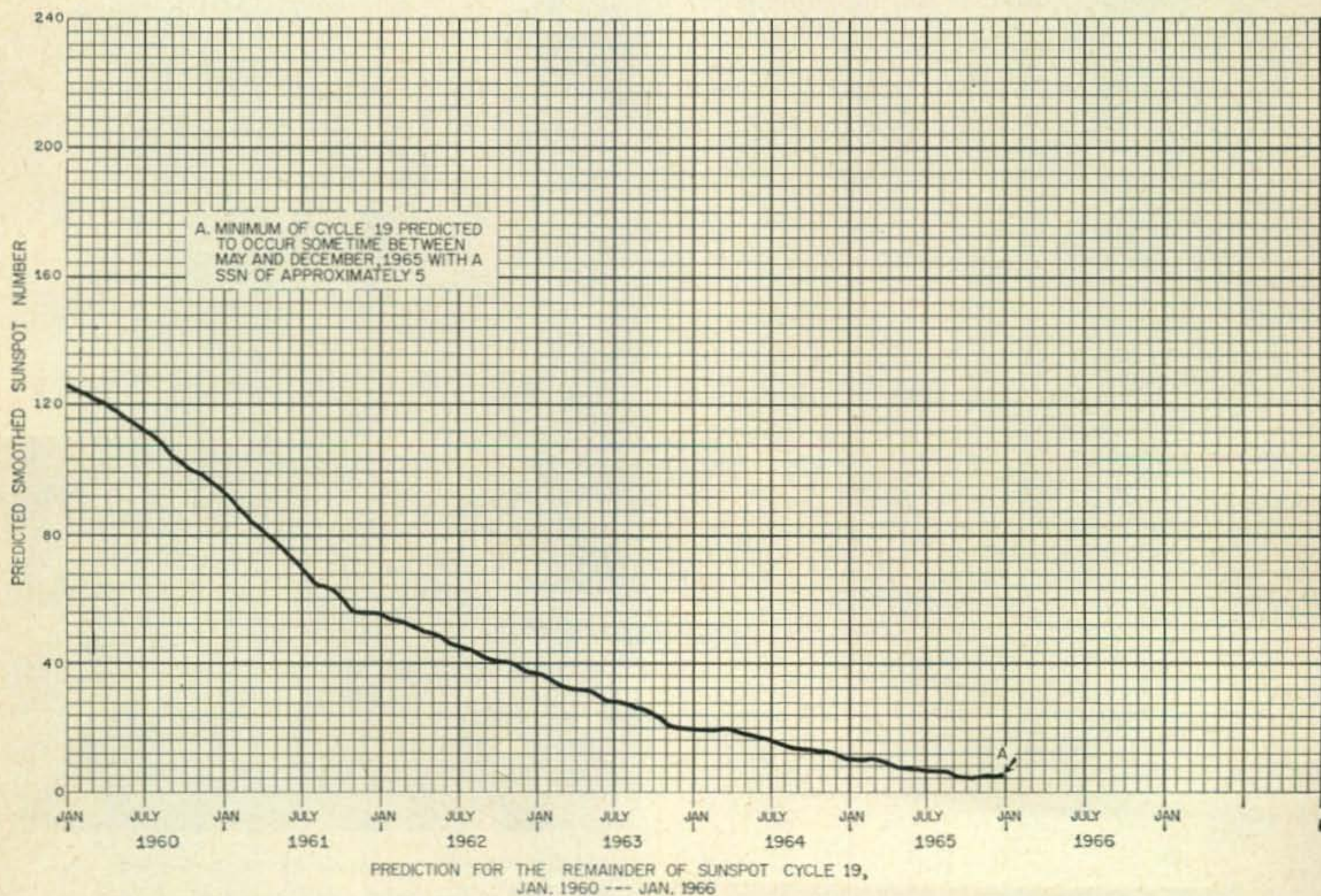
Fig. 2—Graphic presentation of the predicted behavior of the remainder of Sunspot Cycle 19 listed in Table 2.
