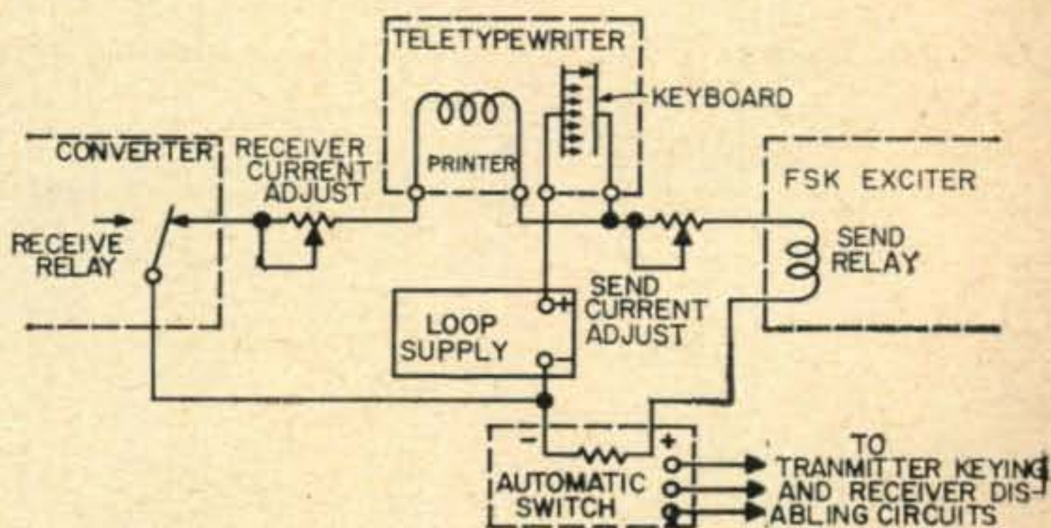
Fig. 2—Block diagram demonstrating a loop arrangement for printing local copy while sending.
