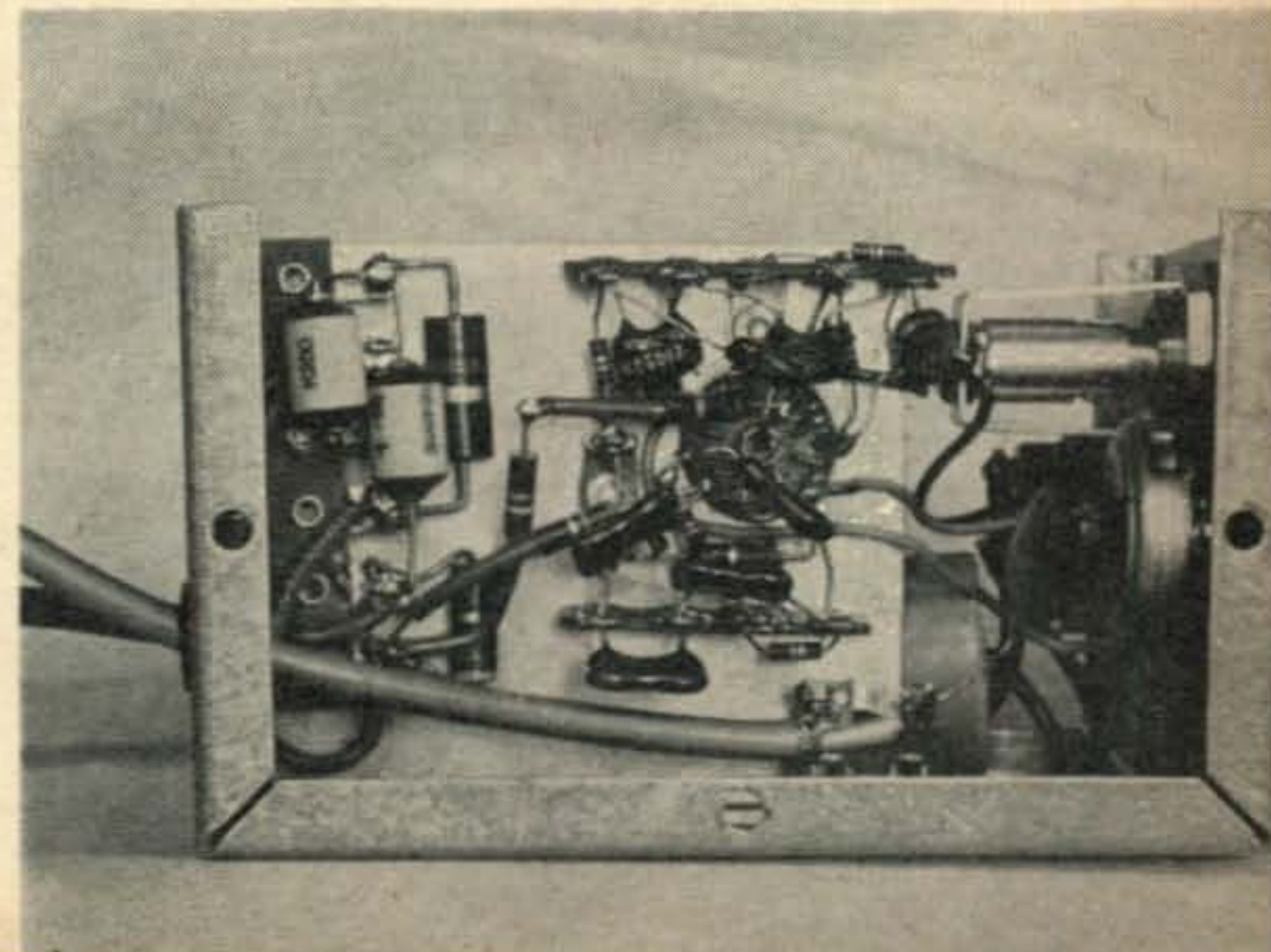
Bottom view of the vertical bracket showing parts location. The audio output can be seen coupled through C 9 to a piece of shielded mike cable.
