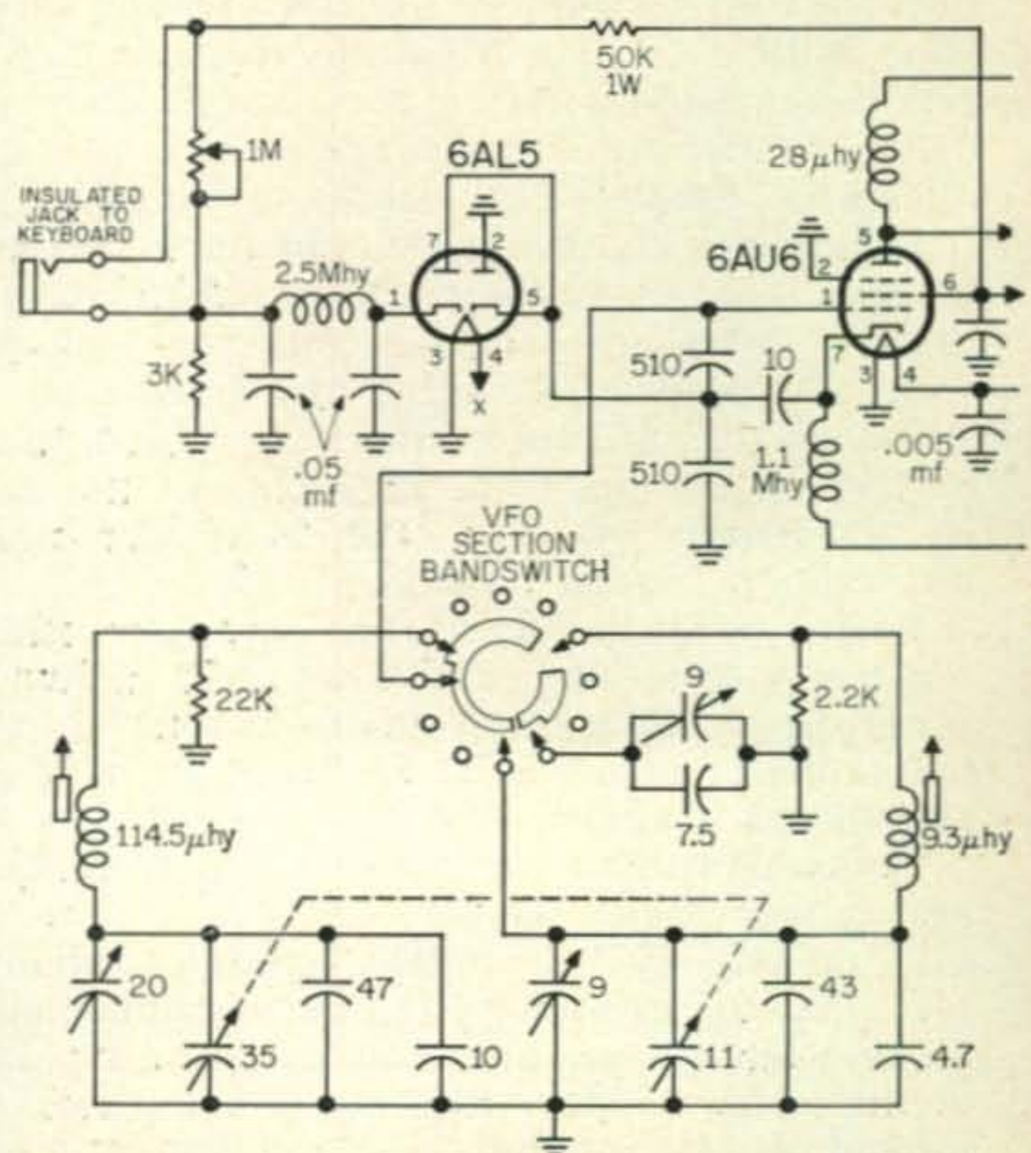
Fig. 1—DX-100 FSK Circuit of W6AEE.
