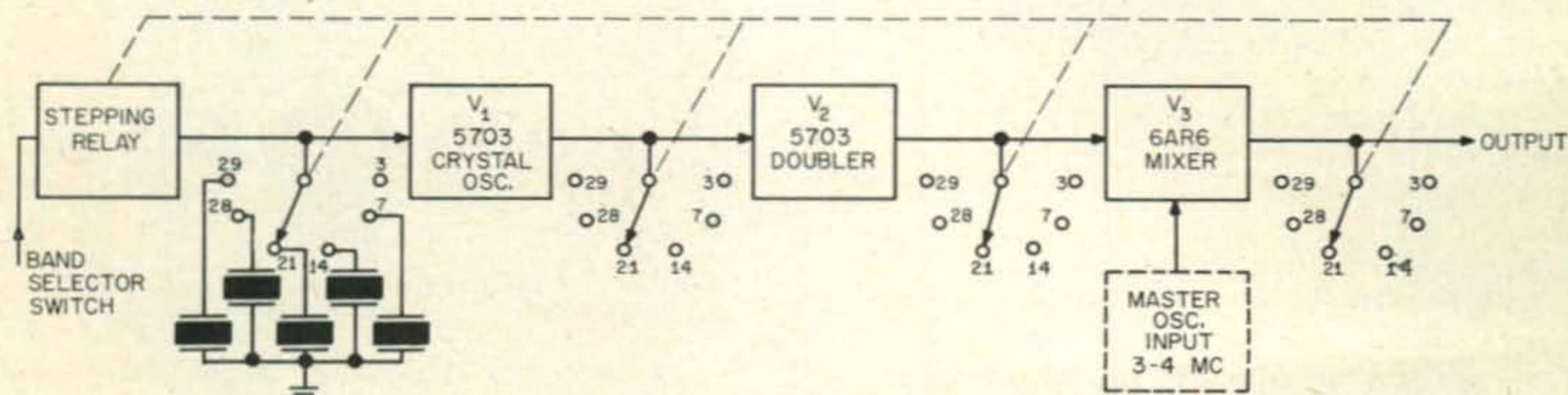
Fig. 1—Block diagram of the Frequency Coupler showing relationship of stepping relay to band-switching. The master Oscillator was described by the author in a previous article.
