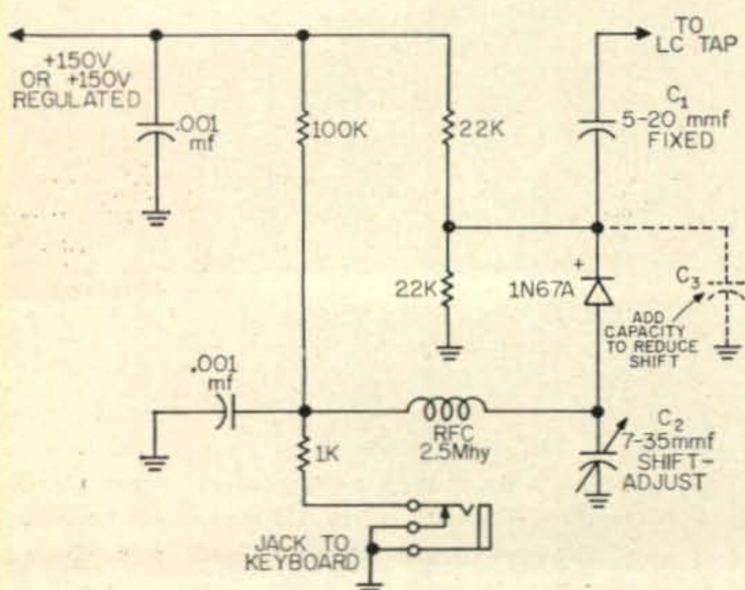
Fig. 2—Diode Switch FSK Circuit of WØACV.
