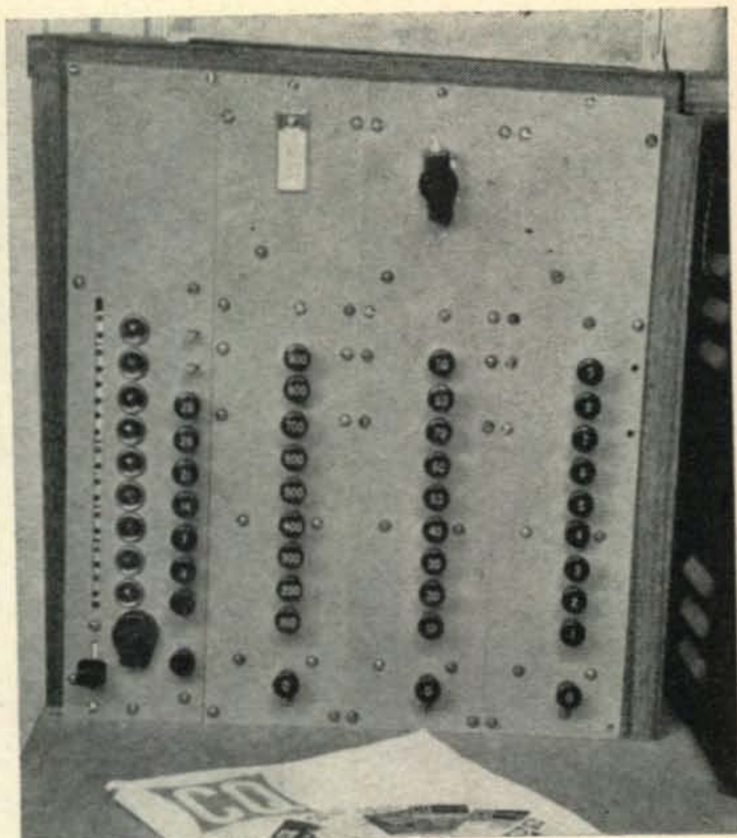
Push button consol at W2JKH. By actuating appropriate buttons, choice of frequency is made instantaneously. For example; 7+100+20+8=7128 kc.
