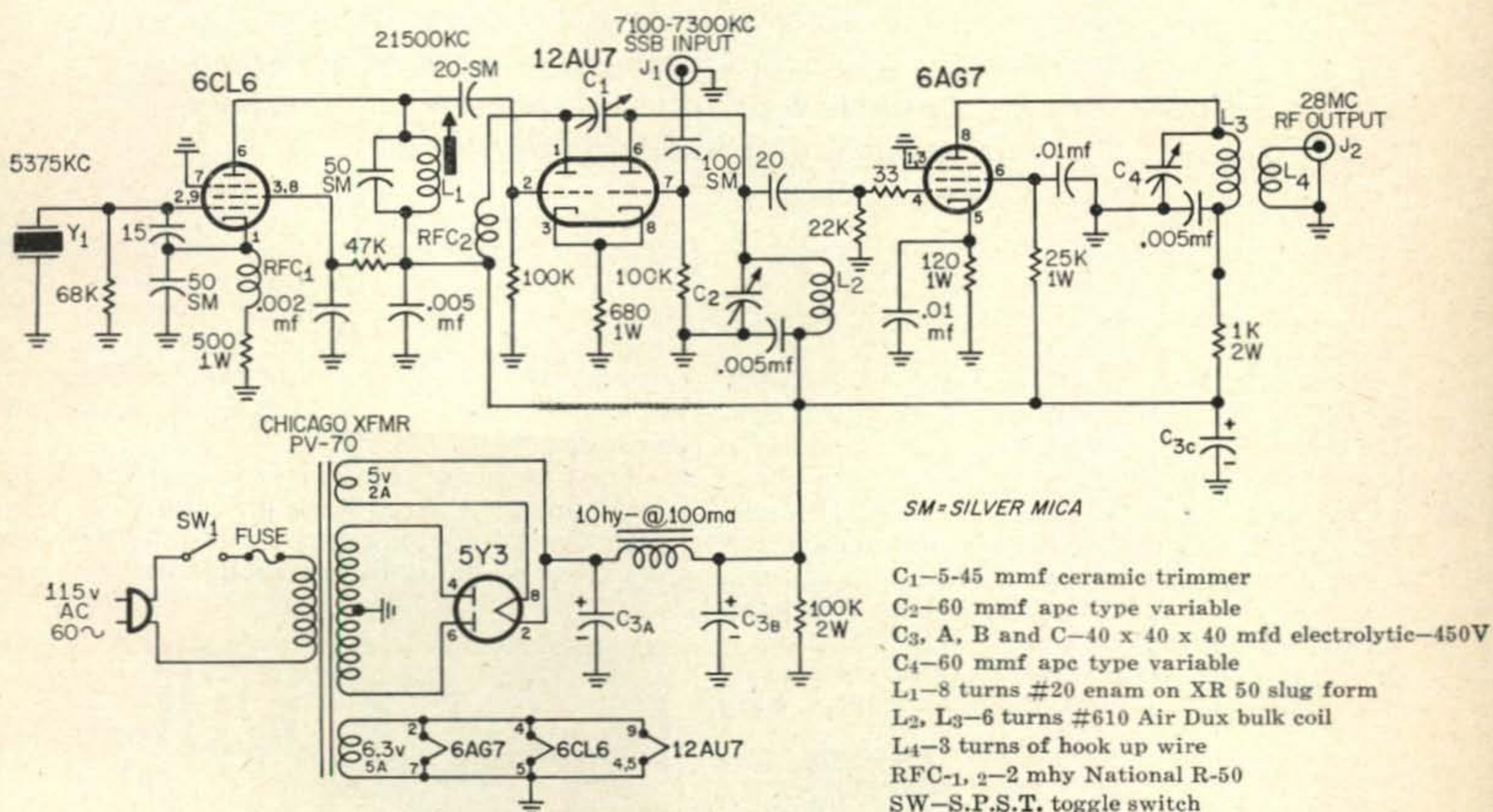
Fig. 1—Schematic of an SSB Ten Meter Mixer. All resistors are 1/2 watt unless otherwise specified. All fixed capacitors are silvered mica with the exception of the decimal values which are disc ceramic.
