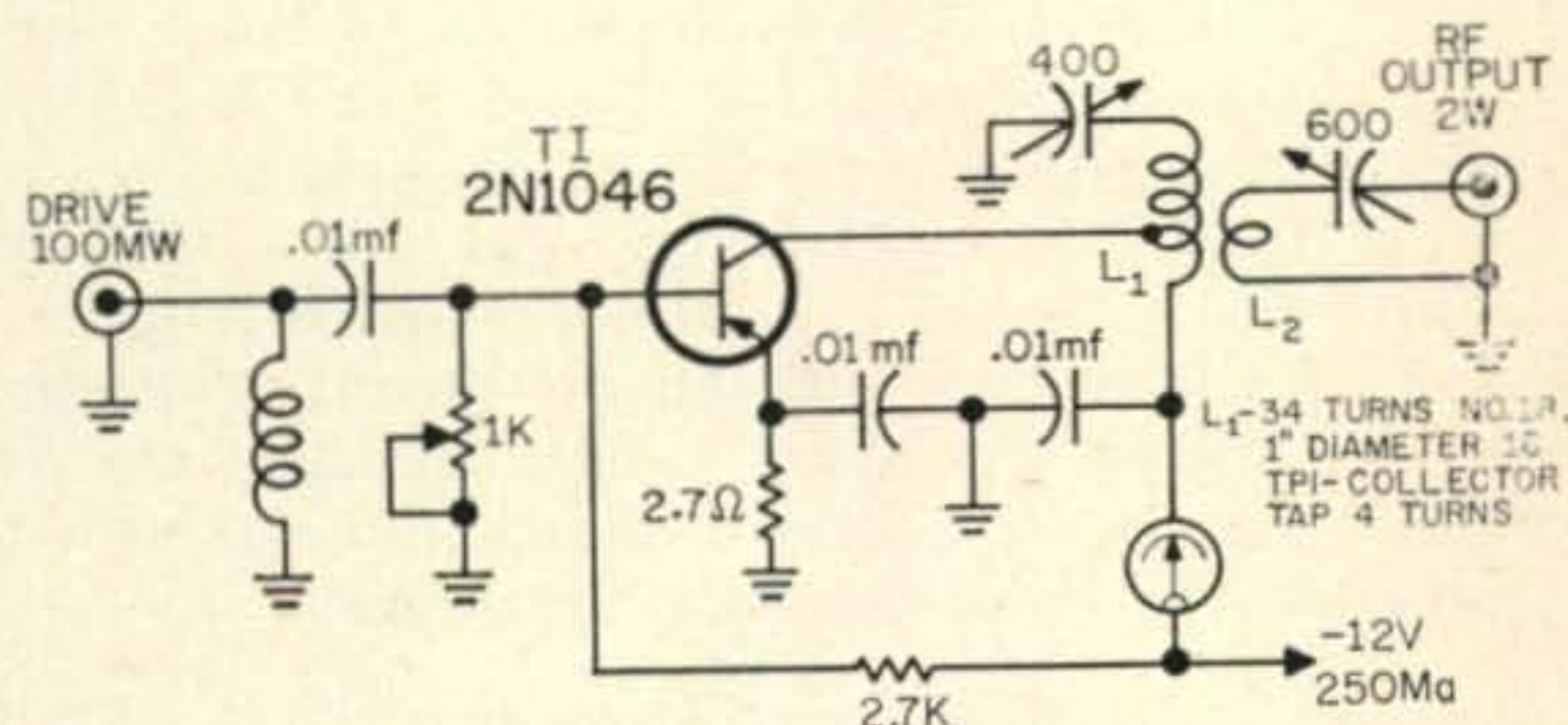
Fig. 2—Linear amplifier for 40 and 80 meters.
