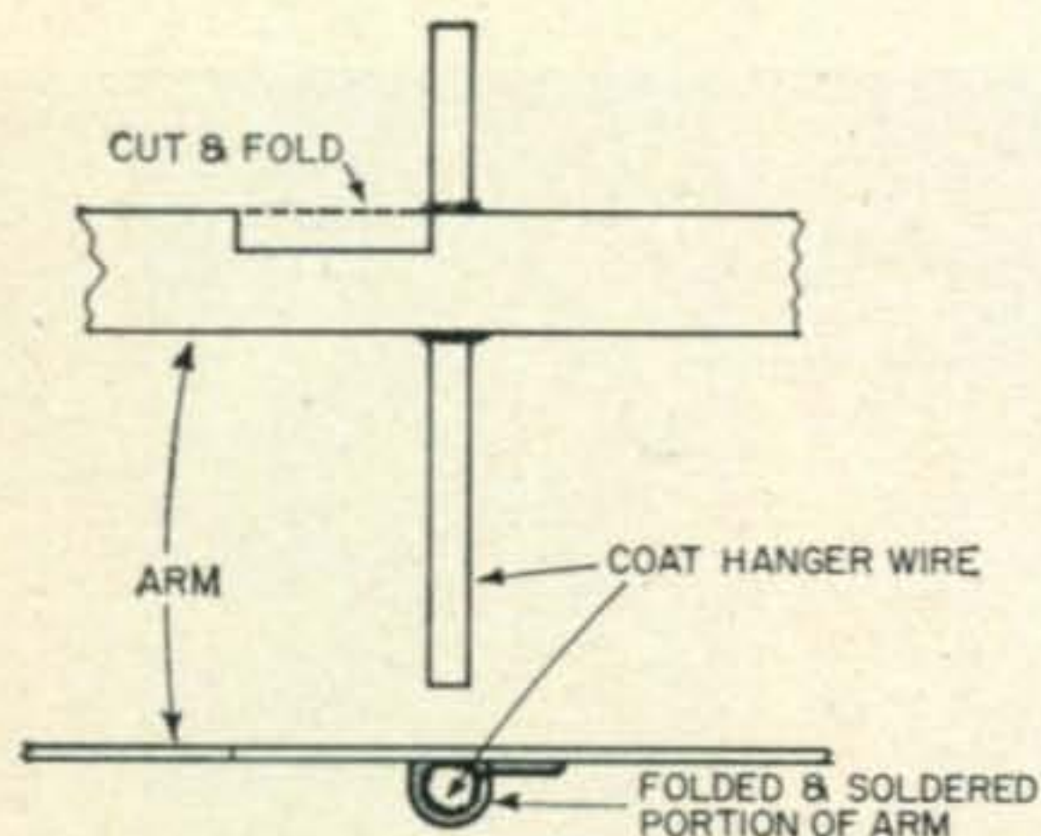
Fig. 2—Side and top detail of pivot construction.
