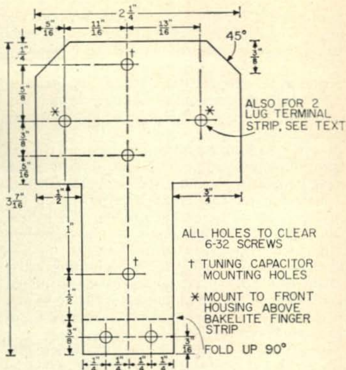
Fig. 5—PLATE A—This plate mounts the main tuning capacitor for the dipper. In this case the dimensions fit the Hammarlund HFD-50.
