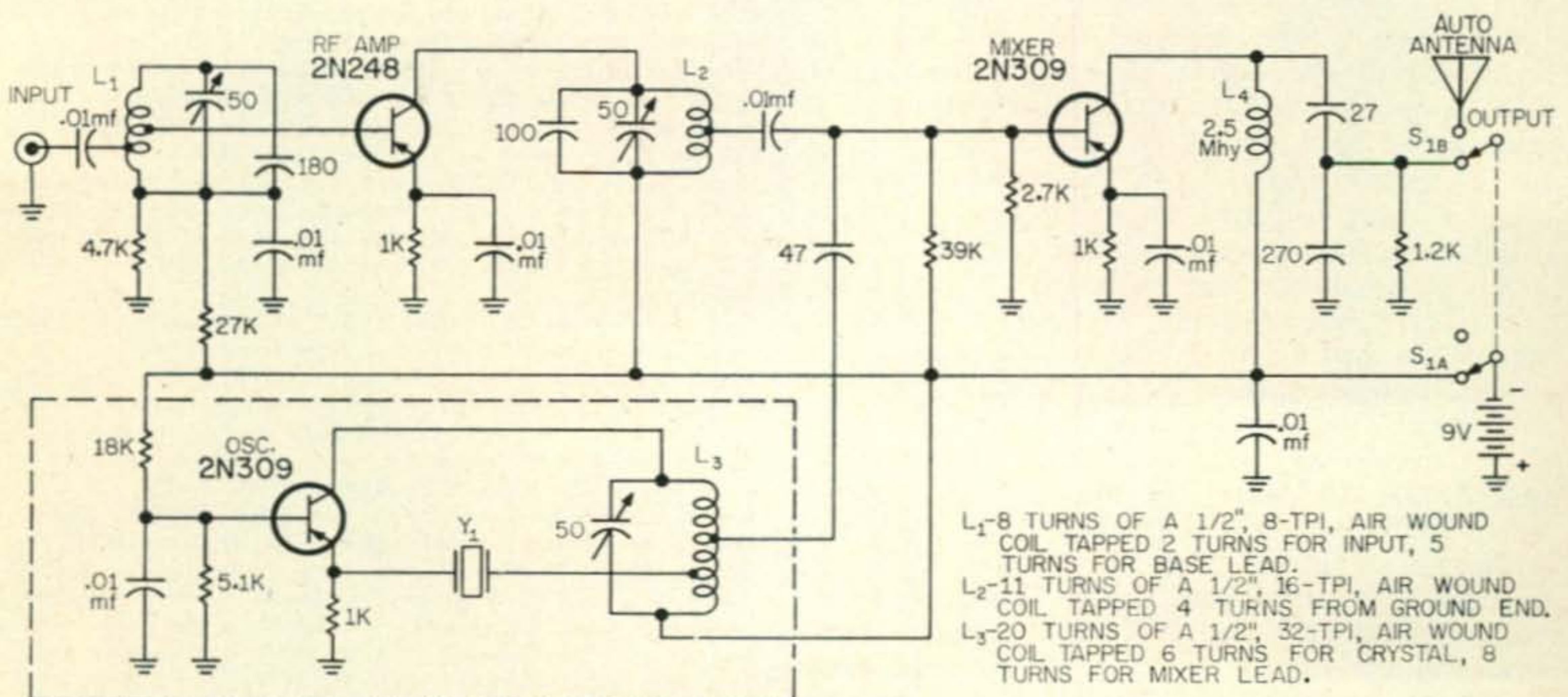
Fig. 1—Schematic diagram for the Texas Instruments transistorized 20 meter converter.
