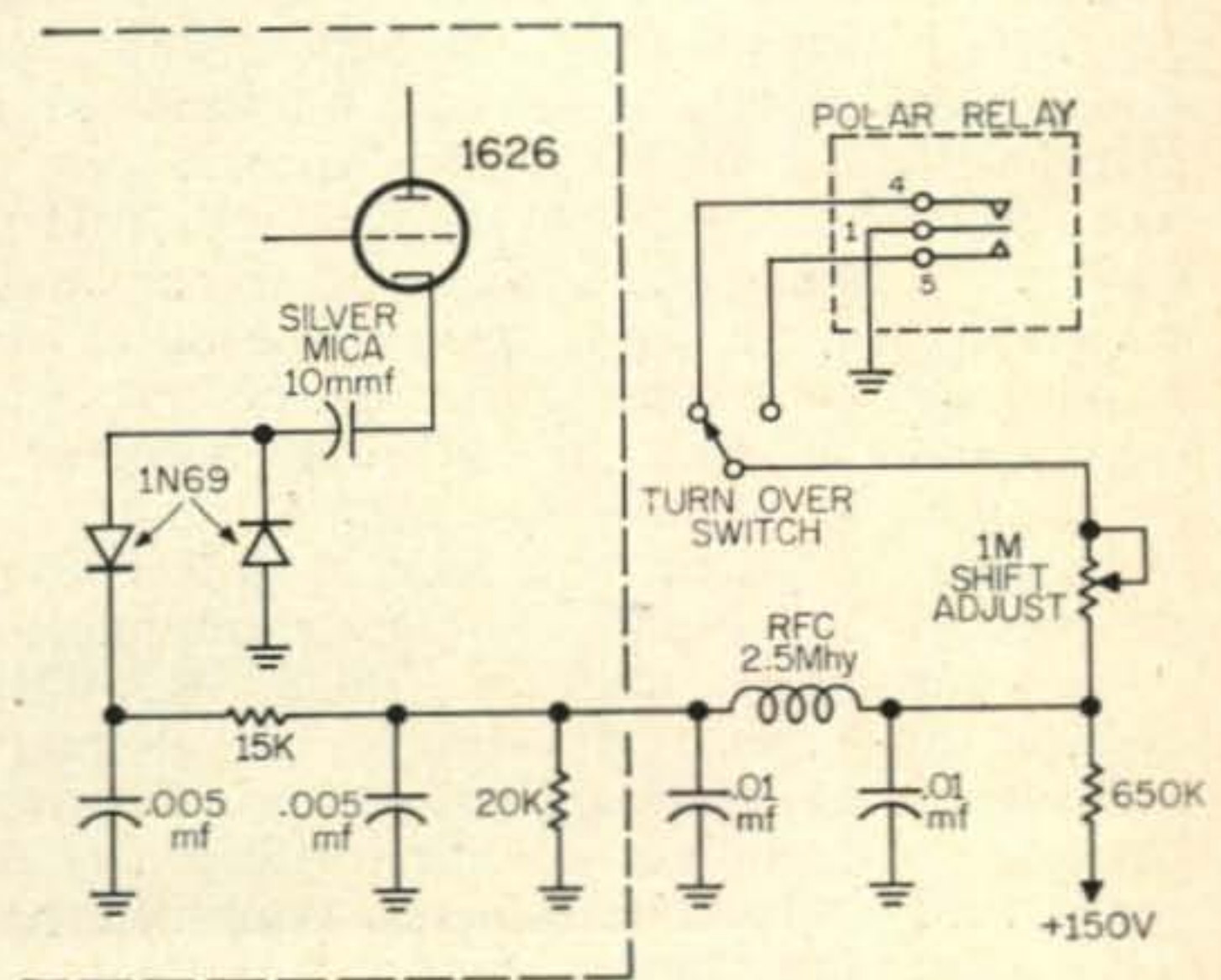
Fig. 3—CE 458 VFO FSK Circuit of K9CNG.
