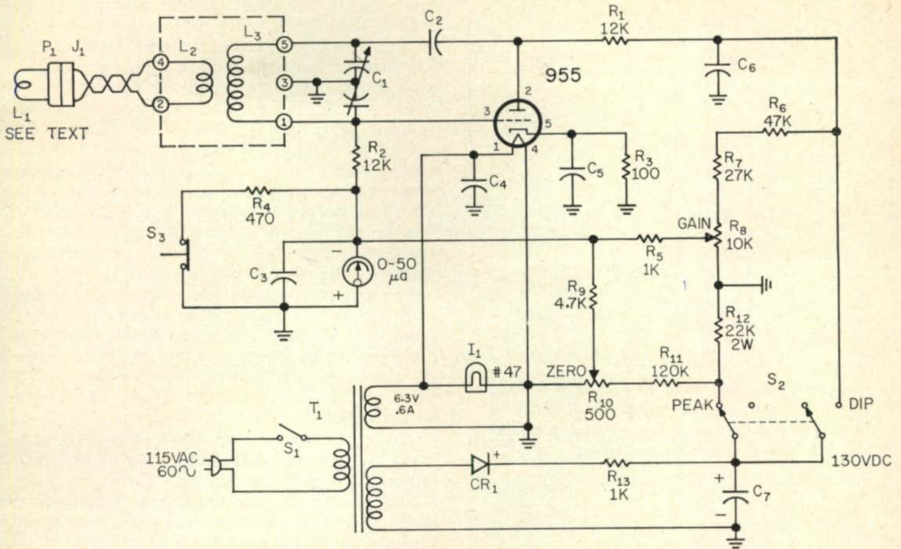
Fig. 1—Circuit of the Uno-Dipper. All resistors are 1/2 watt unless otherwise specified.
