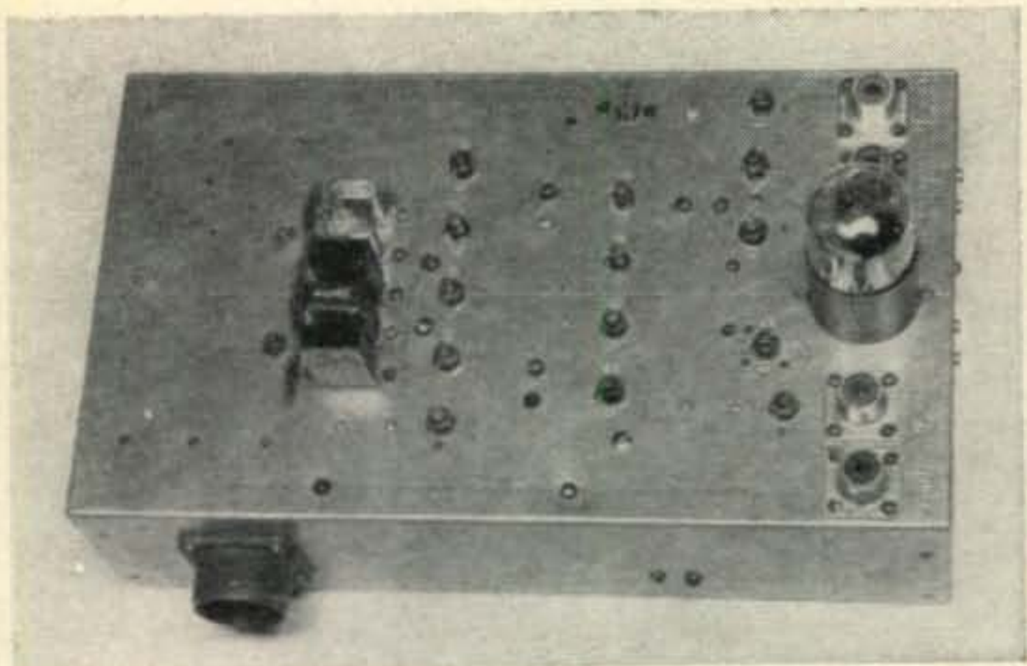
Top of the frequency coupler showing crystal and capacitor arrangement. The AN connector, J 5 , supplies power and switching signals from the push-button consol. The coaxial connectors are, from bottom to top, J 1 master oscillator input, J 2 80 and 40 meter output, J 3 (partially hidden by the 6AR6) 20 and 10 meter output and J 4 15 meter output.
