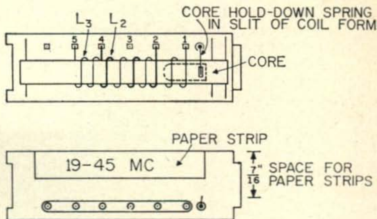
Fig. 6—Drawing illustrating the points used when fabricating the coils. All coil winding data may be found in the Coil Table.
