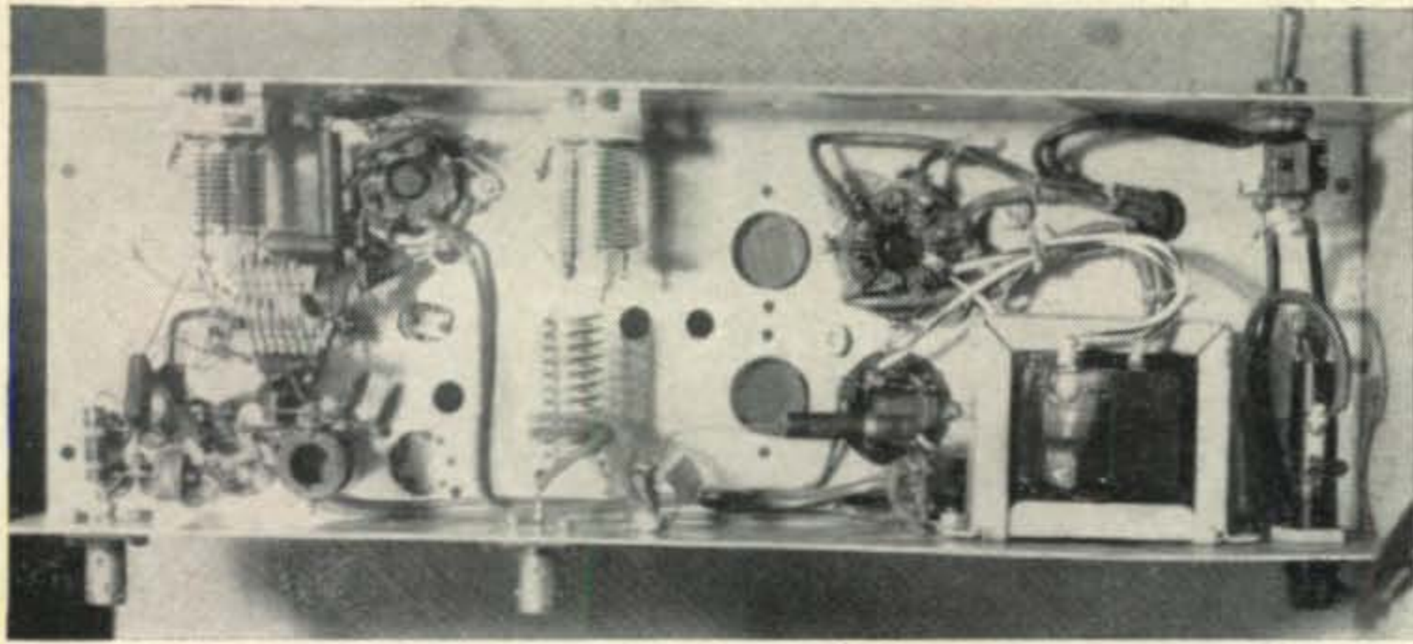
Bottom view of the 10 meter mixer. J 1 exciter input is mounted at the bottom left and J 2 , RF out is almost in the center. L 1 can be seen mounted on the main chassis between the BNC coaxial connectors.
